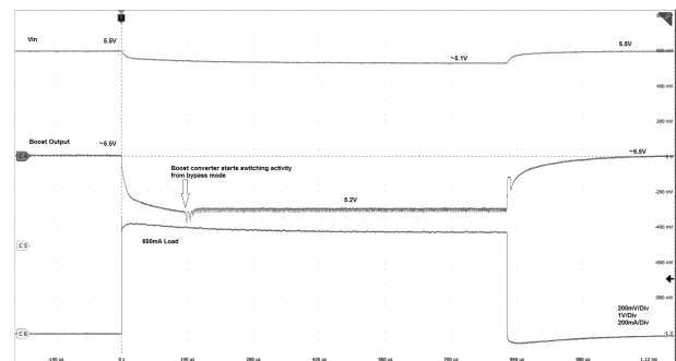
Figure 8. Boost powered by 5 V supply having poor performance
