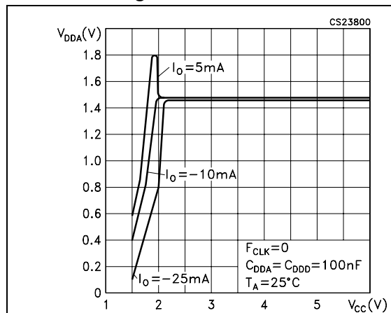
Figure 7. Digital voltage regulator: line - load regulation
