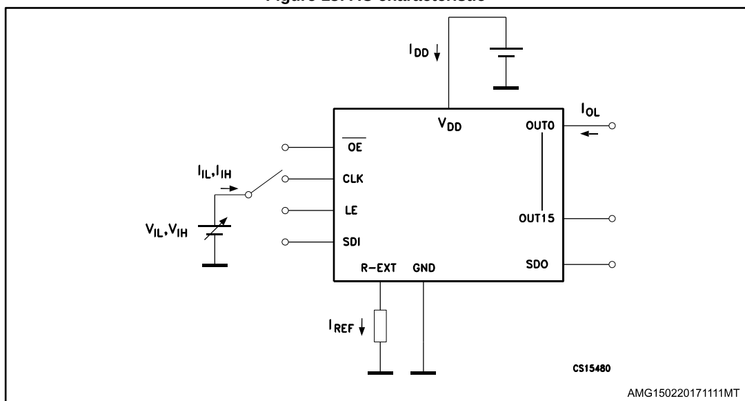
Figure 18: AC characteristic
