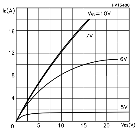
Figure 5. Output Characteristics
