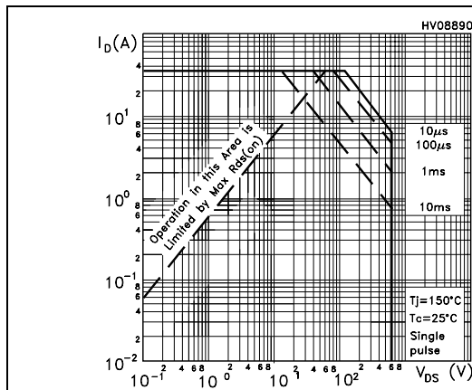
Figure 1. Safe operating area for TO-220 / I 2 PAK / D 2 PAK
