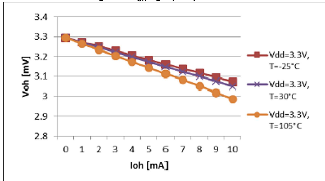
Figure 29. V_{OH} high speed pad at 3.3 V
