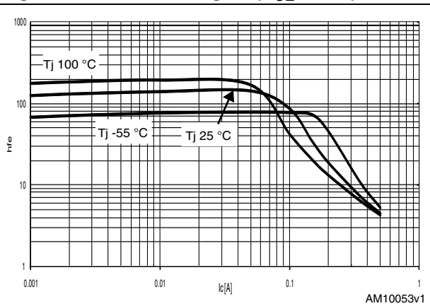
Figure 7. DC current gain ( V_{CE} = -5 V)
