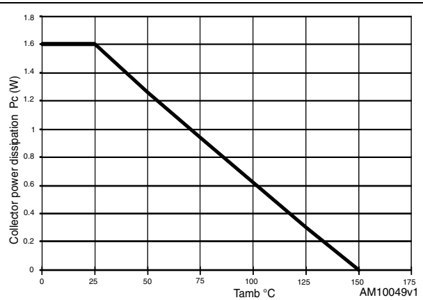
Figure 3. Derating curve
