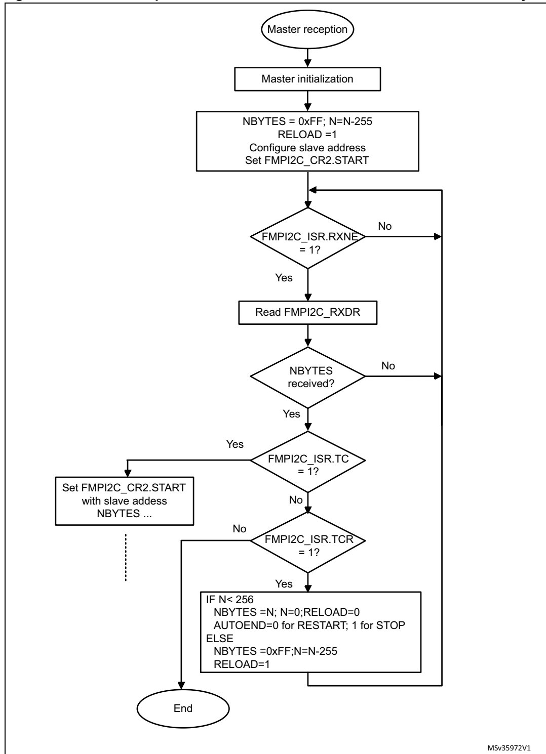
Figure 229. Transfer sequence flowchart for FMPI2C master receiver for N &gt; 255 bytes
