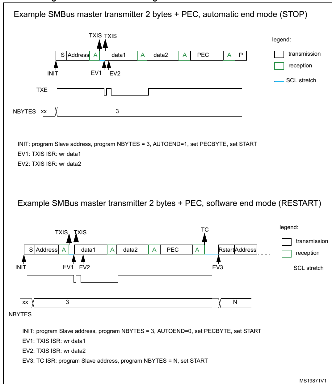
Figure 236. Bus transfer diagrams for SMBus master transmitter
