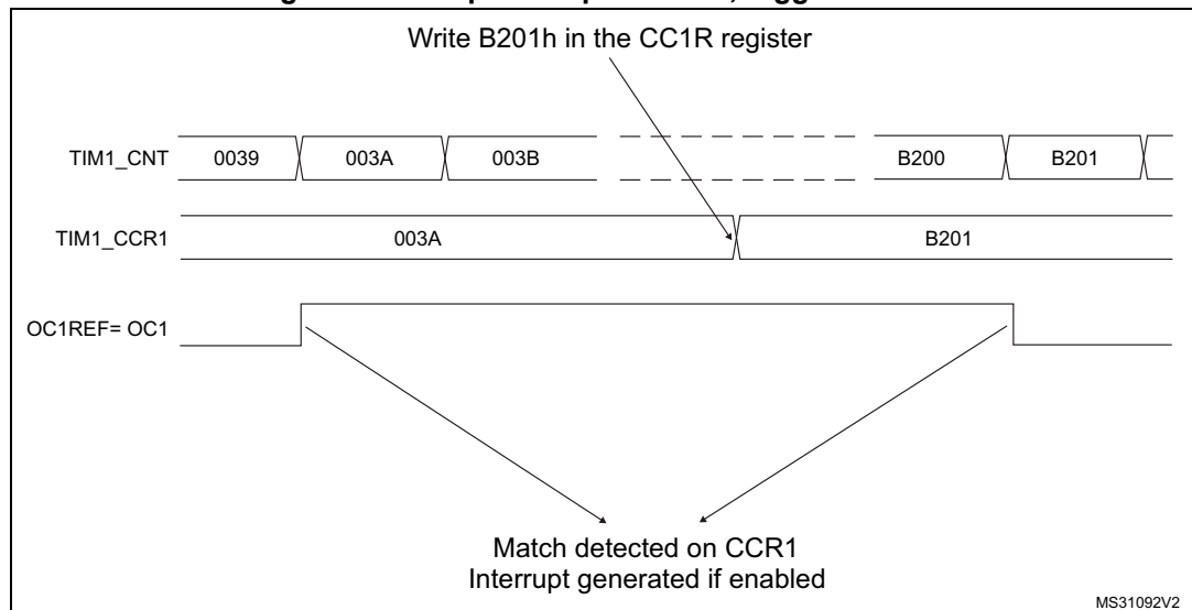
Figure 188. Output compare mode, toggle on OC1.
