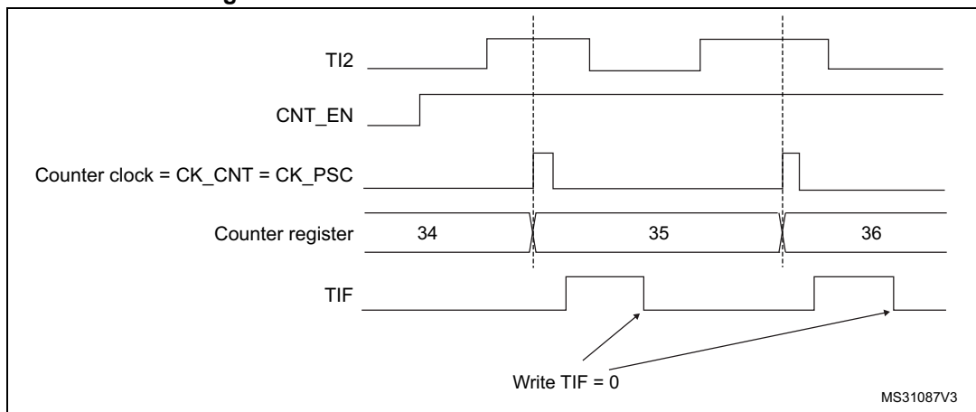
Figure 183. Control circuit in external clock mode 1
