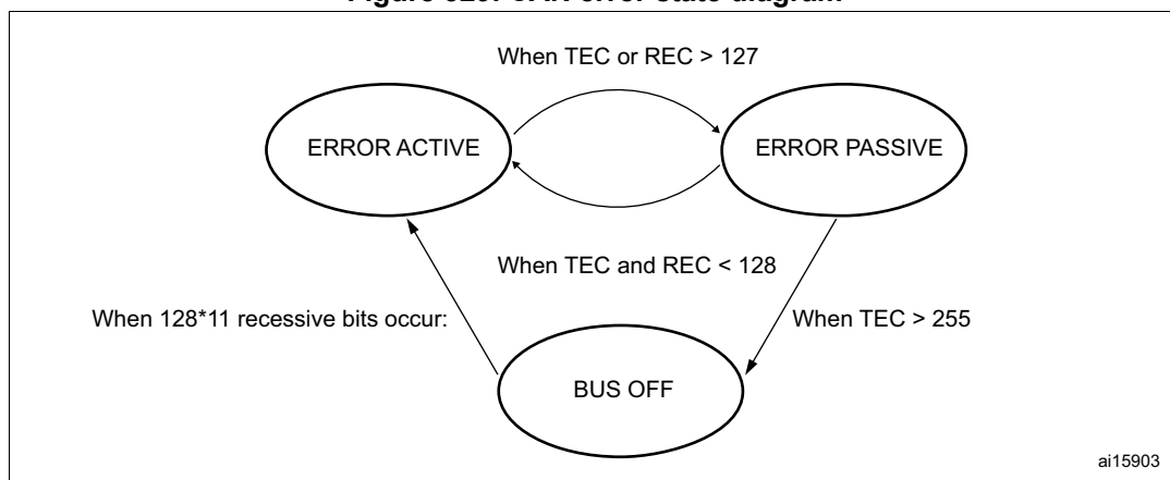
Figure 329. CAN error state diagram
