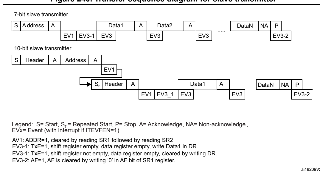
Figure 240. Transfer sequence diagram for slave transmitter
