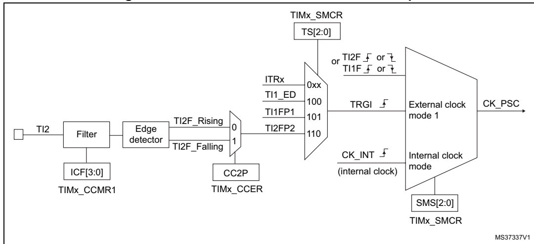
Figure 182. TI2 external clock connection example
