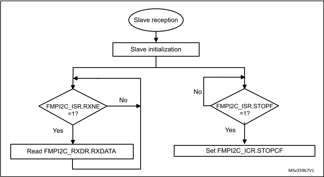
Figure 219. Transfer sequence flowchart for slave receiver with NOSTRETCH=1
