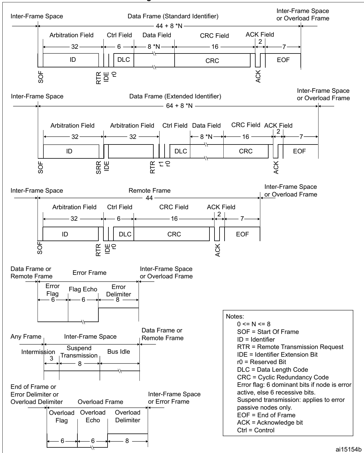
Figure 331. CAN frames
