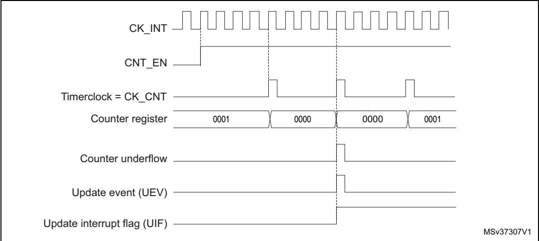
Figure 108. Counter timing diagram, internal clock divided by 4
