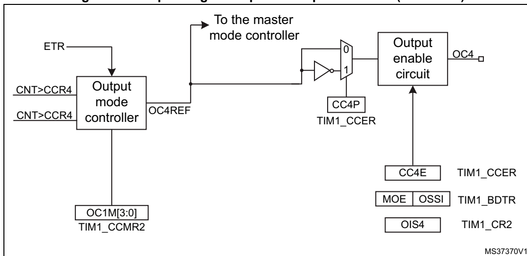
Figure 78. Output stage of capture/compare channel (channel 4)
