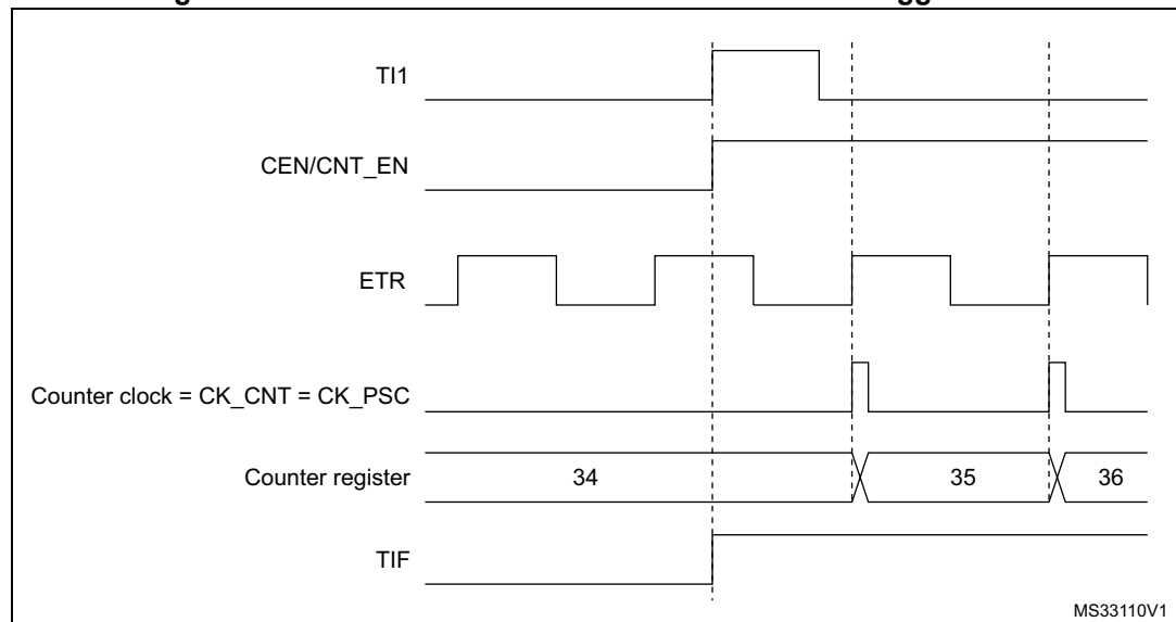
Figure 96. Control circuit in external clock mode 2 + trigger mode
