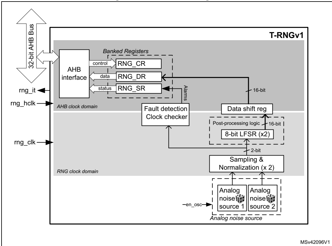
Figure 47. RNG block diagram
