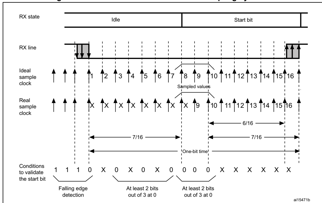
Figure 218. Start bit detection when oversampling by 16 or 8
