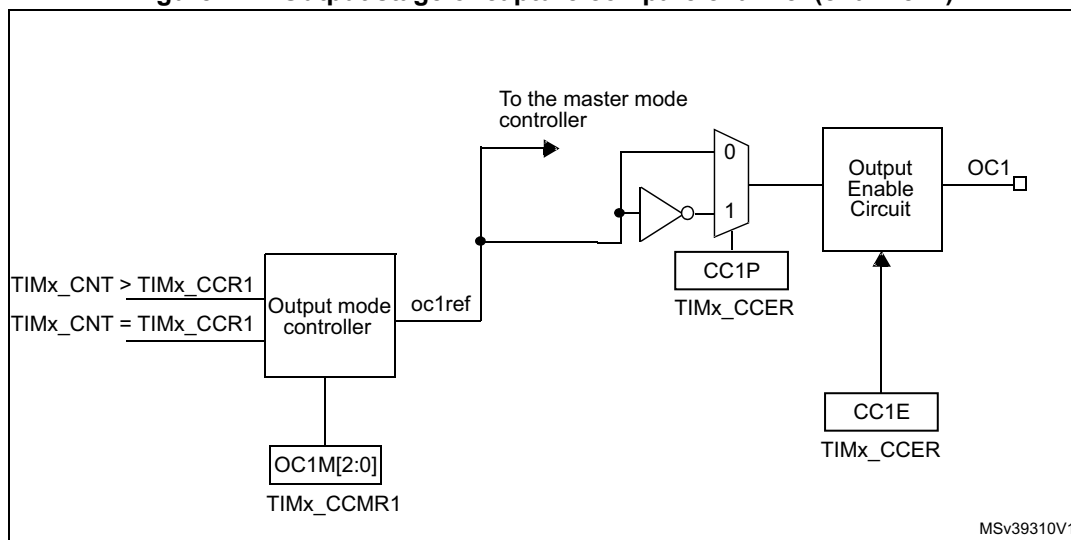
Figure 122. Output stage of capture/compare channel (channel 1)
