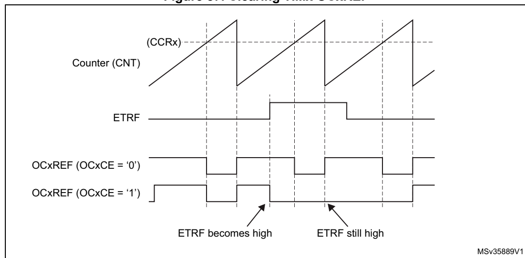
Figure 87. Clearing TIMx OCxREF
