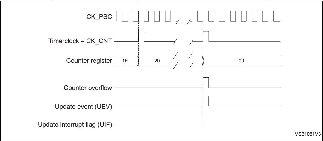
Figure 55. Counter timing diagram, internal clock divided by N
