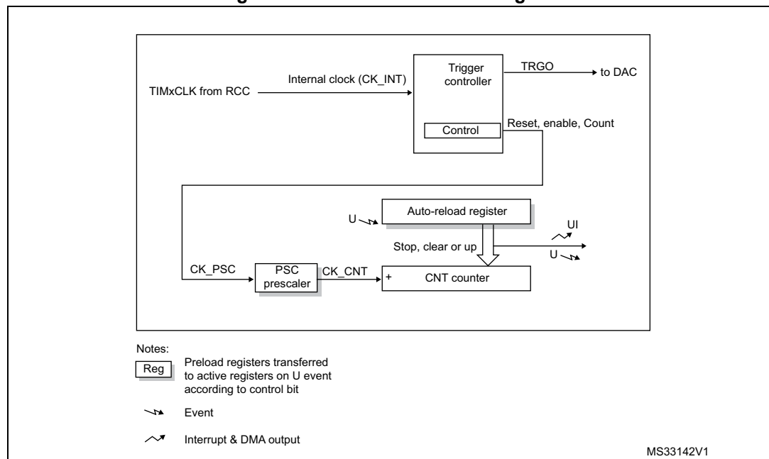
Figure 156. Basic timer block diagram
