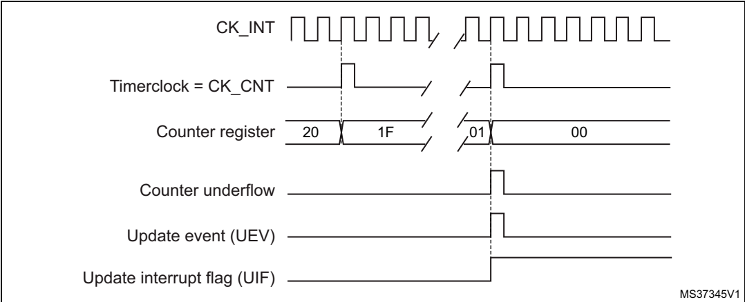
Figure 114. Counter timing diagram, internal clock divided by N
