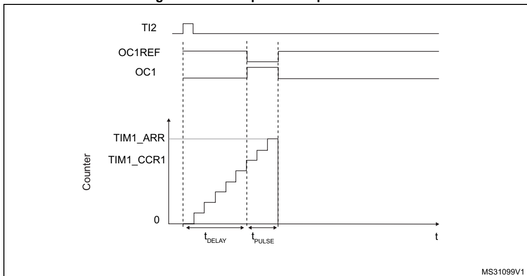
Figure 127. Example of one-pulse mode
