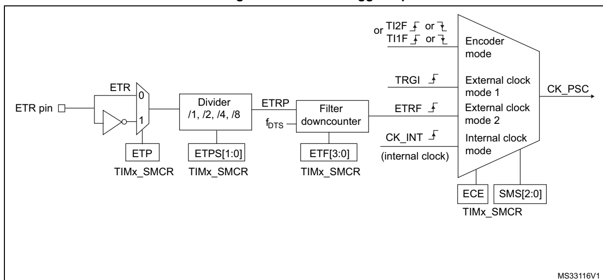
Figure 73. External trigger input block
