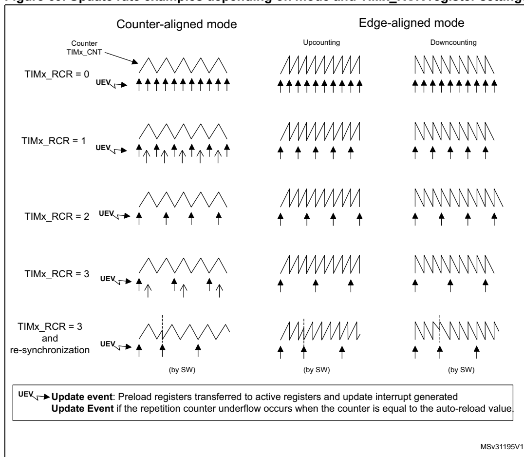
Figure 69. Update rate examples depending on mode and TIMx_RCR register settings
