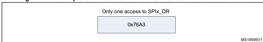
Figure 259. Example of 16-bit data frame extended to 32-bit channel frame
