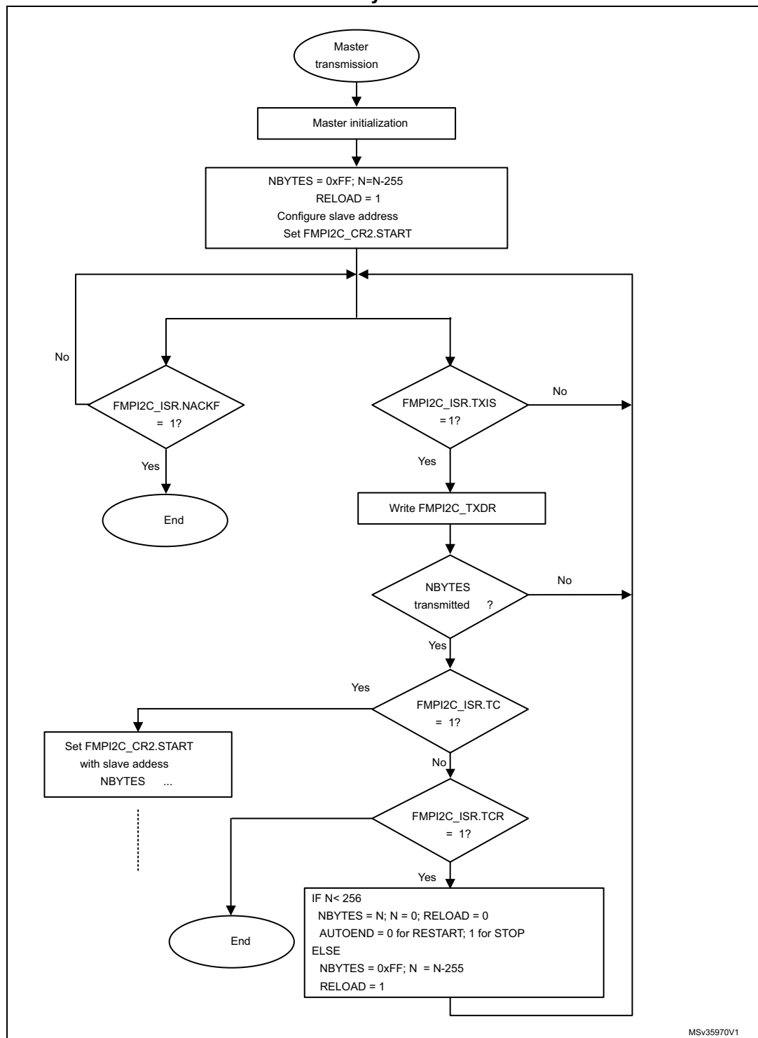
Figure 195. Transfer sequence flowchart for FMPI2C master transmitter for N>255 bytes
