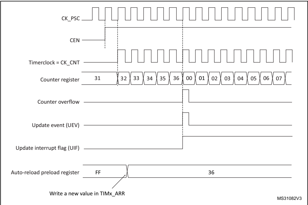
Figure 56. Counter timing diagram, update event when ARPE=0 (TIMx_ARR not preloaded)
