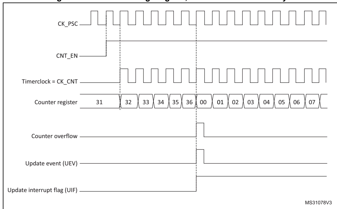
Figure 52. Counter timing diagram, internal clock divided by 1
