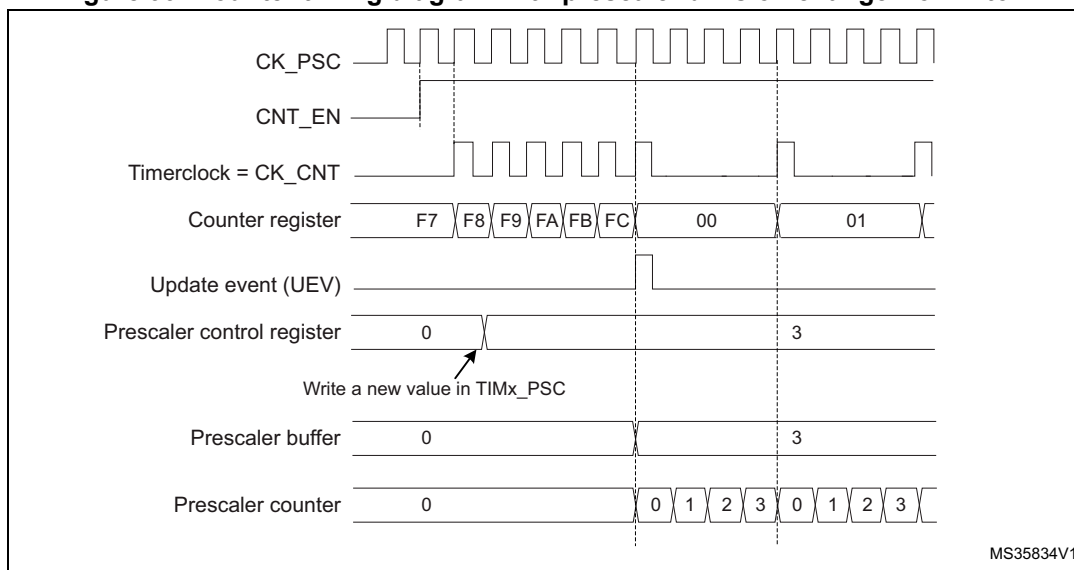
Figure 99. Counter timing diagram with prescaler division change from 1 to 4
