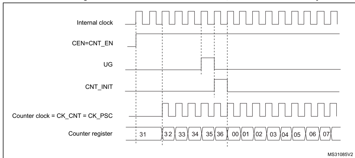
Figure 70. Control circuit in normal mode, internal clock divided by 1
