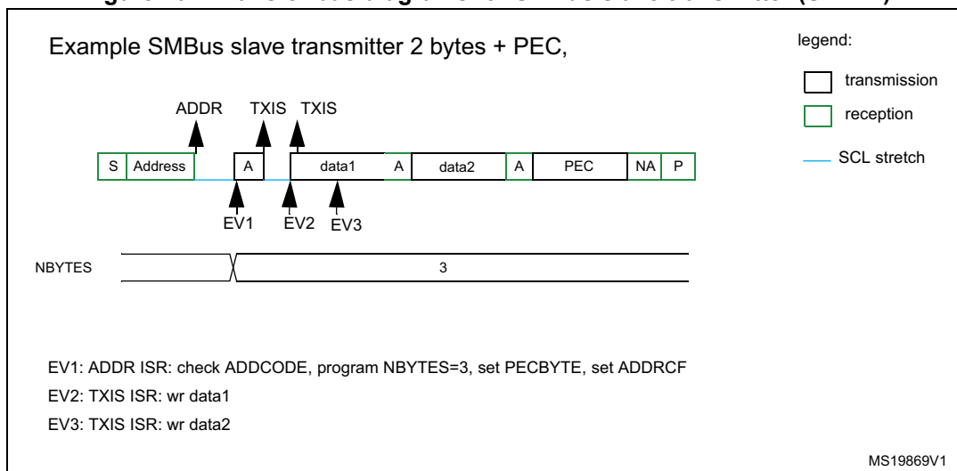
Figure 202. Transfer bus diagrams for SMBus slave transmitter (SBC=1)
