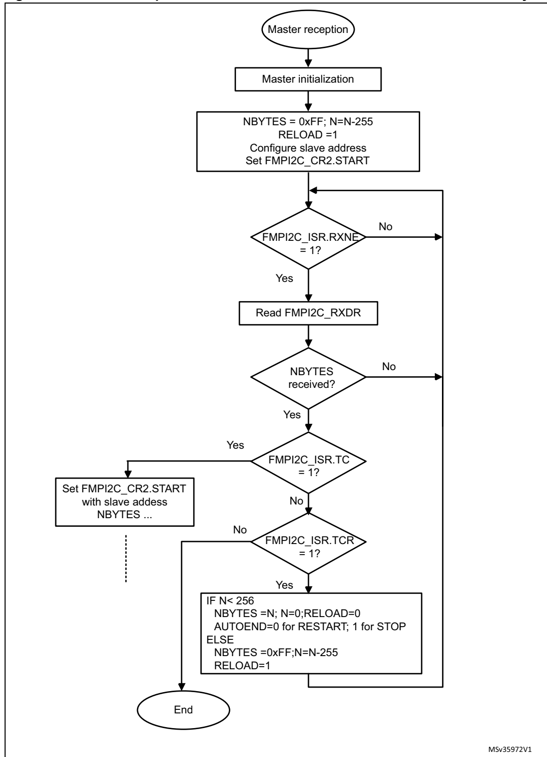
Figure 198. Transfer sequence flowchart for FMPI2C master receiver for N > 255 bytes
