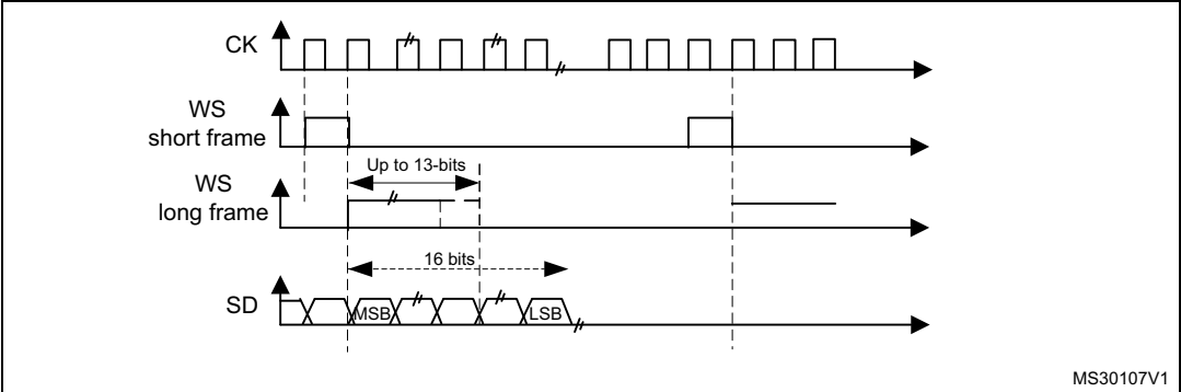
Figure 270. PCM standard waveforms (16-bit extended to 32-bit packet frame)
