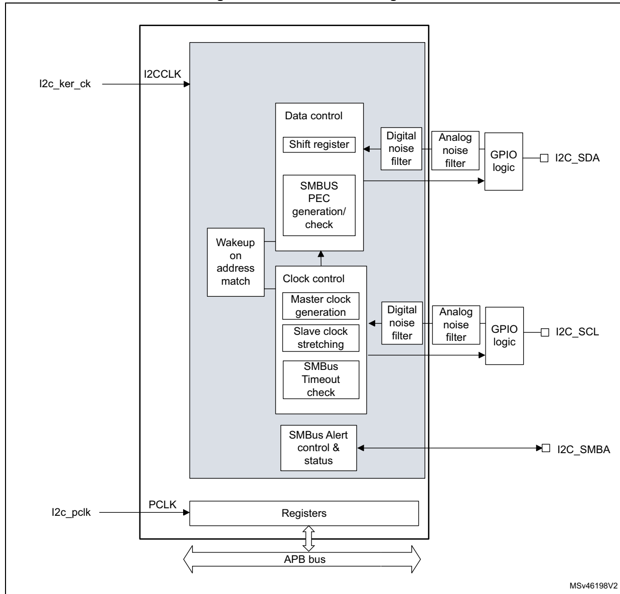
Figure 177. FMPI2C block diagram
