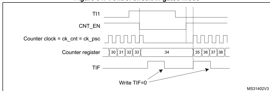
Figure 94. Control circuit in gated mode
