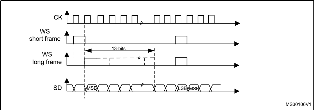
Figure 269. PCM standard waveforms (16-bit)
