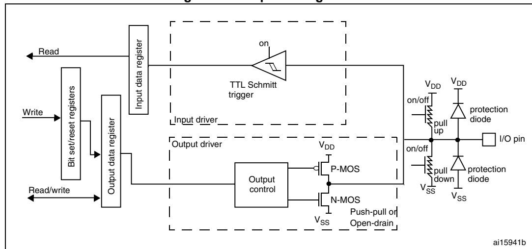
Figure 19. Output configuration
