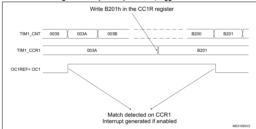
Figure 80. Output compare mode, toggle on OC1.
