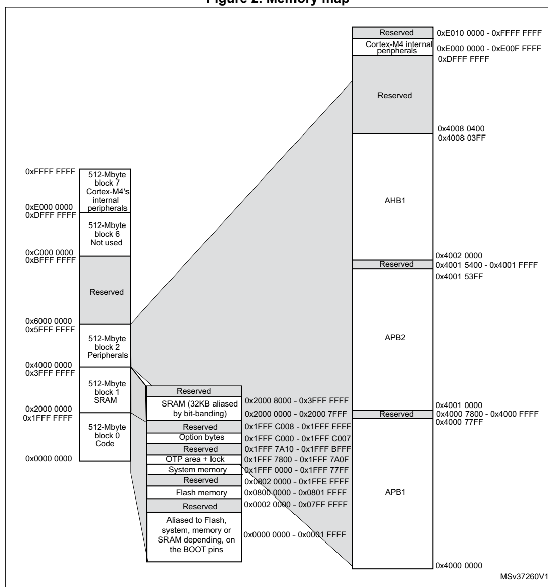
Figure 2. Memory map
