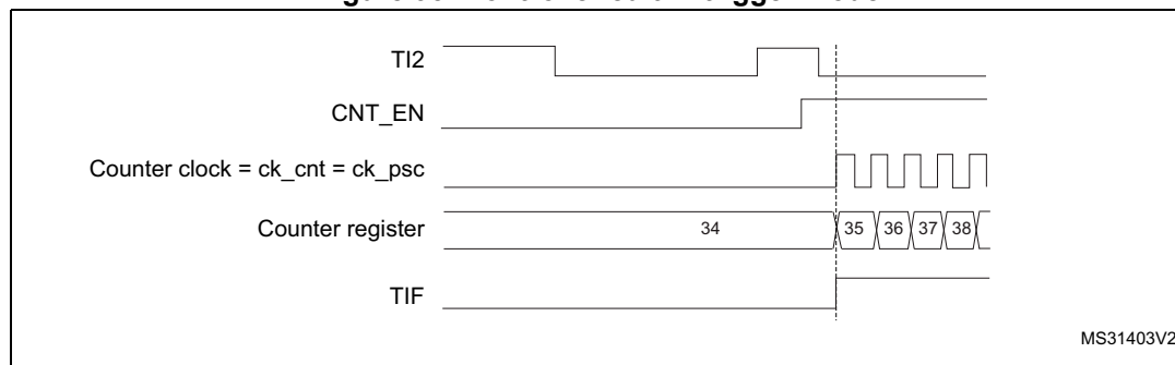
Figure 95. Control circuit in trigger mode
