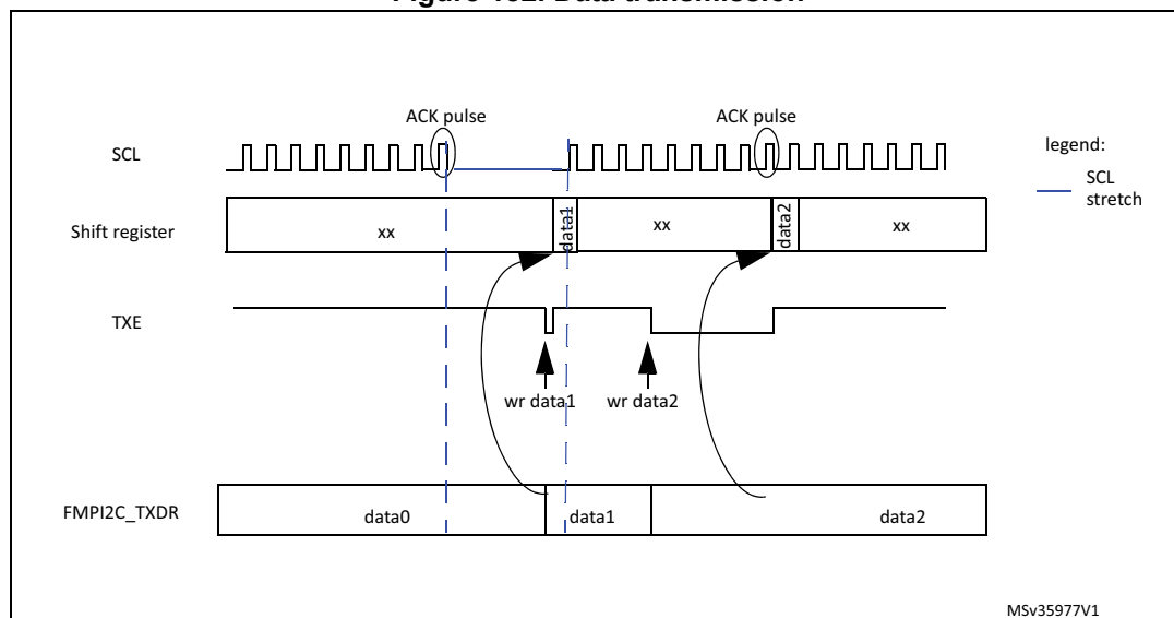
Figure 182. Data transmission
