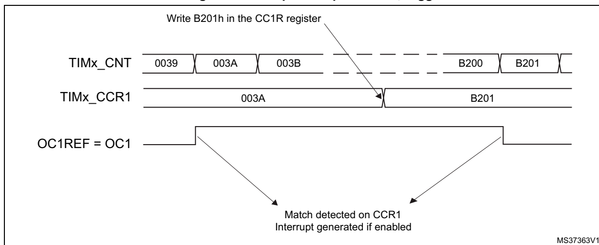
Figure 124. Output compare mode, toggle on OC1
