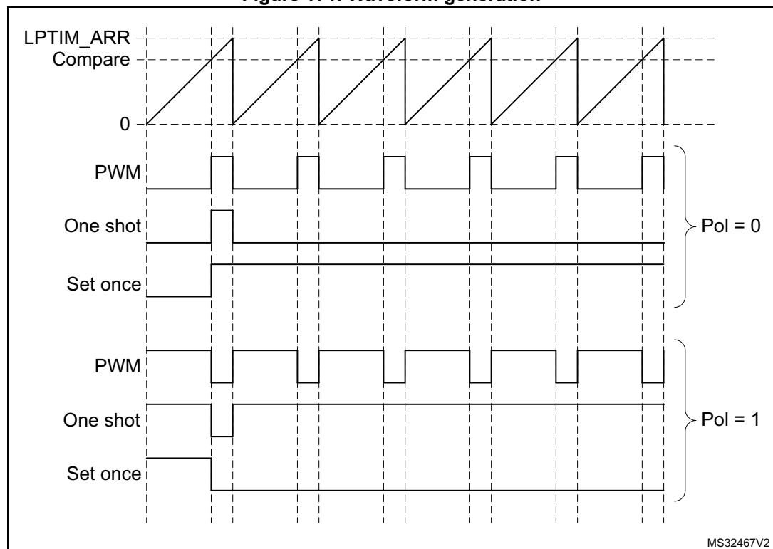
Figure 171. Waveform generation
