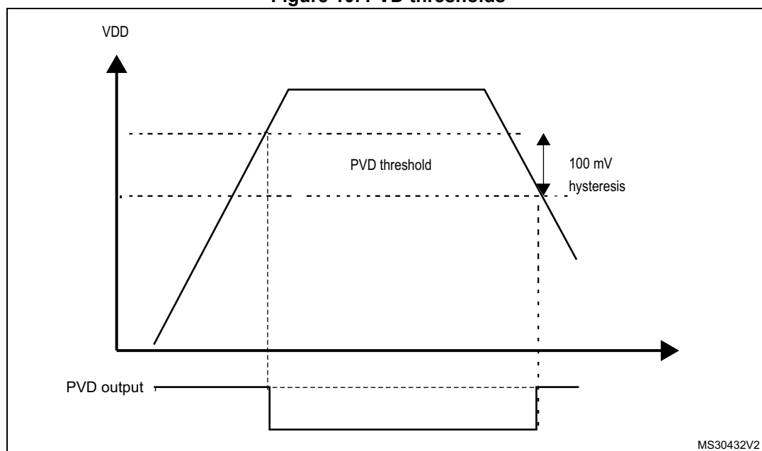
Figure 10. PVD thresholds
