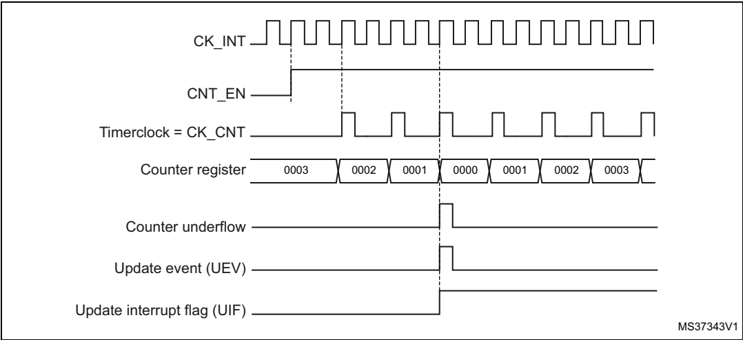
Figure 112. Counter timing diagram, internal clock divided by 2
