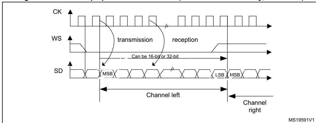
Figure 254. I 2 S Philips protocol waveforms (16/32-bit full accuracy, CPOL = 0)
