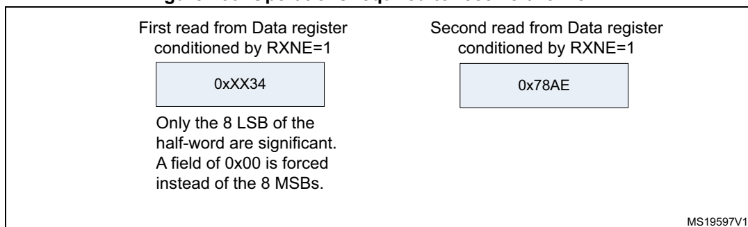
Figure 266. Operations required to receive 0x3478AE
