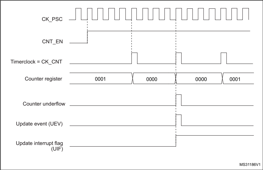
Figure 60. Counter timing diagram, internal clock divided by 4
