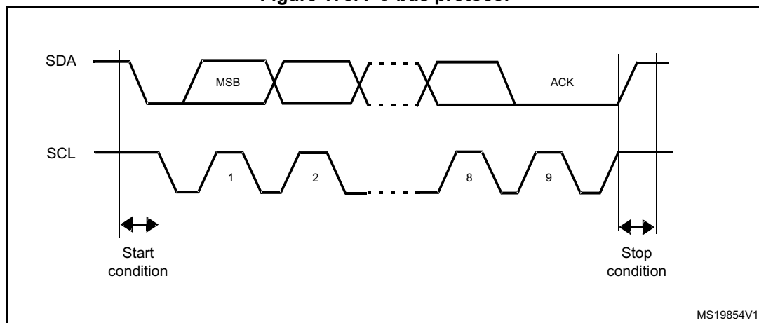
Figure 178. I 2 C bus protocol
