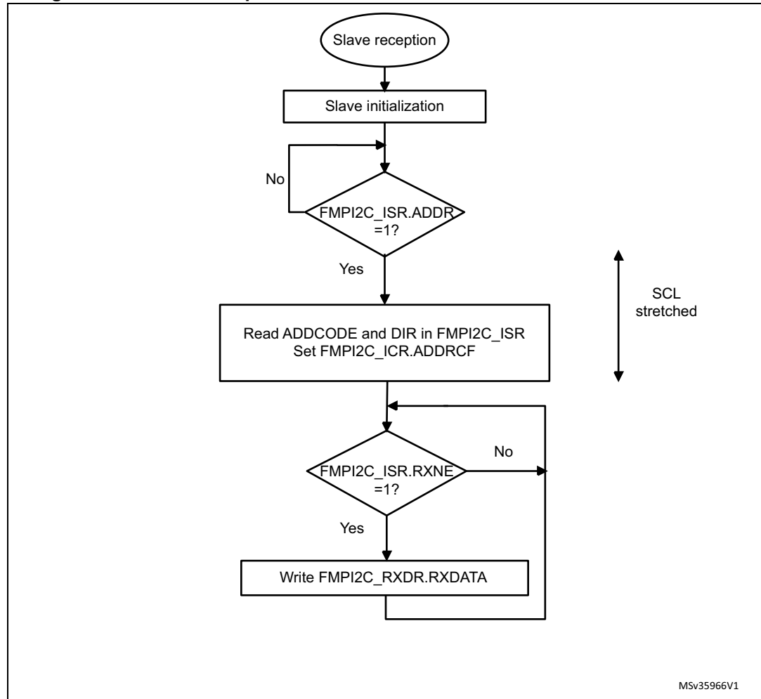
Figure 187. Transfer sequence flowchart for slave receiver with NOSTRETCH=0
