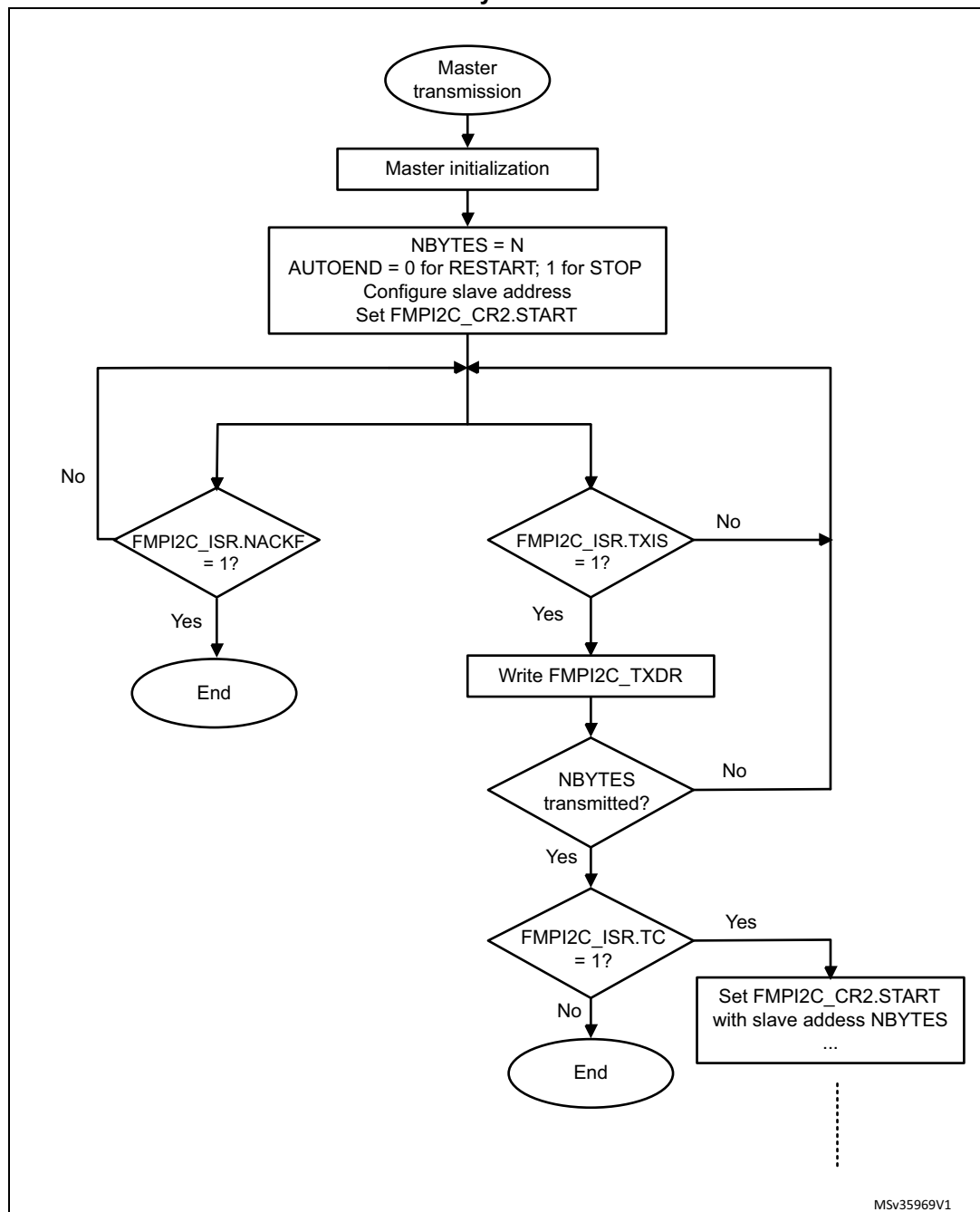
Figure 194. Transfer sequence flowchart for FMPI2C master transmitter for N \leq 255 bytes
