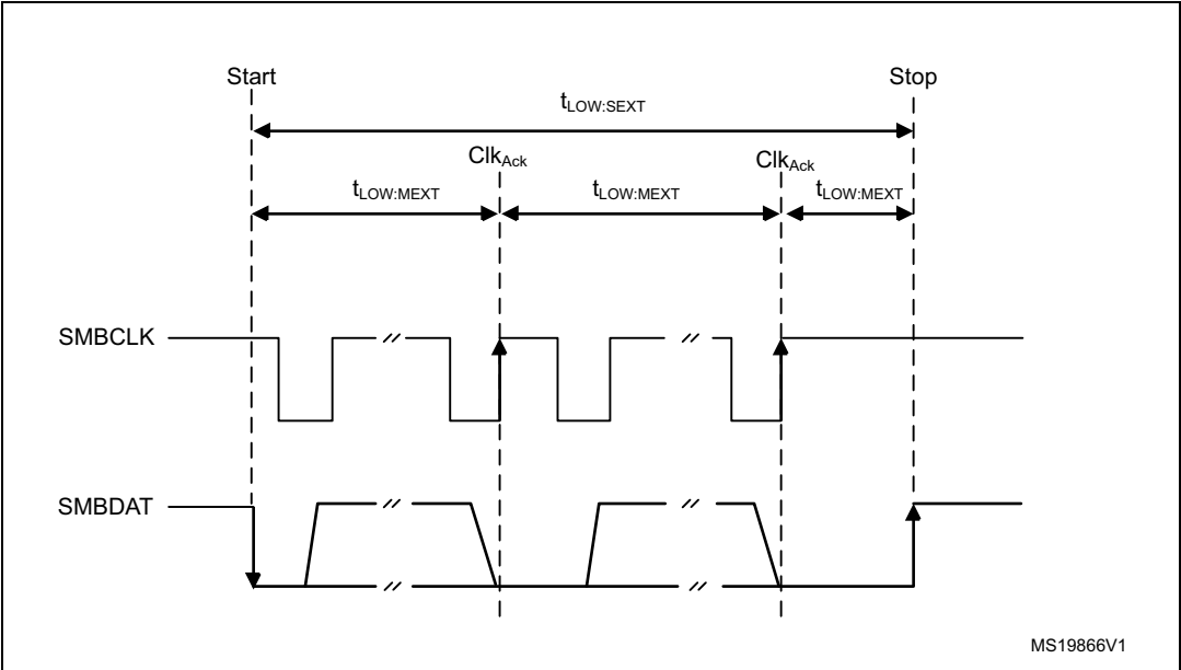
Figure 200. Timeout intervals for t_{\text{LOW:SEXT}} , t_{\text{LOW:MEXT}}
