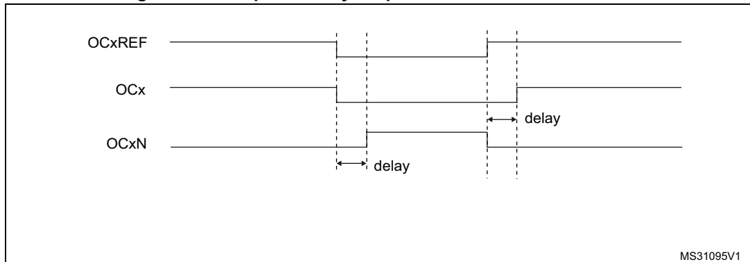
Figure 83. Complementary output with dead-time insertion.
