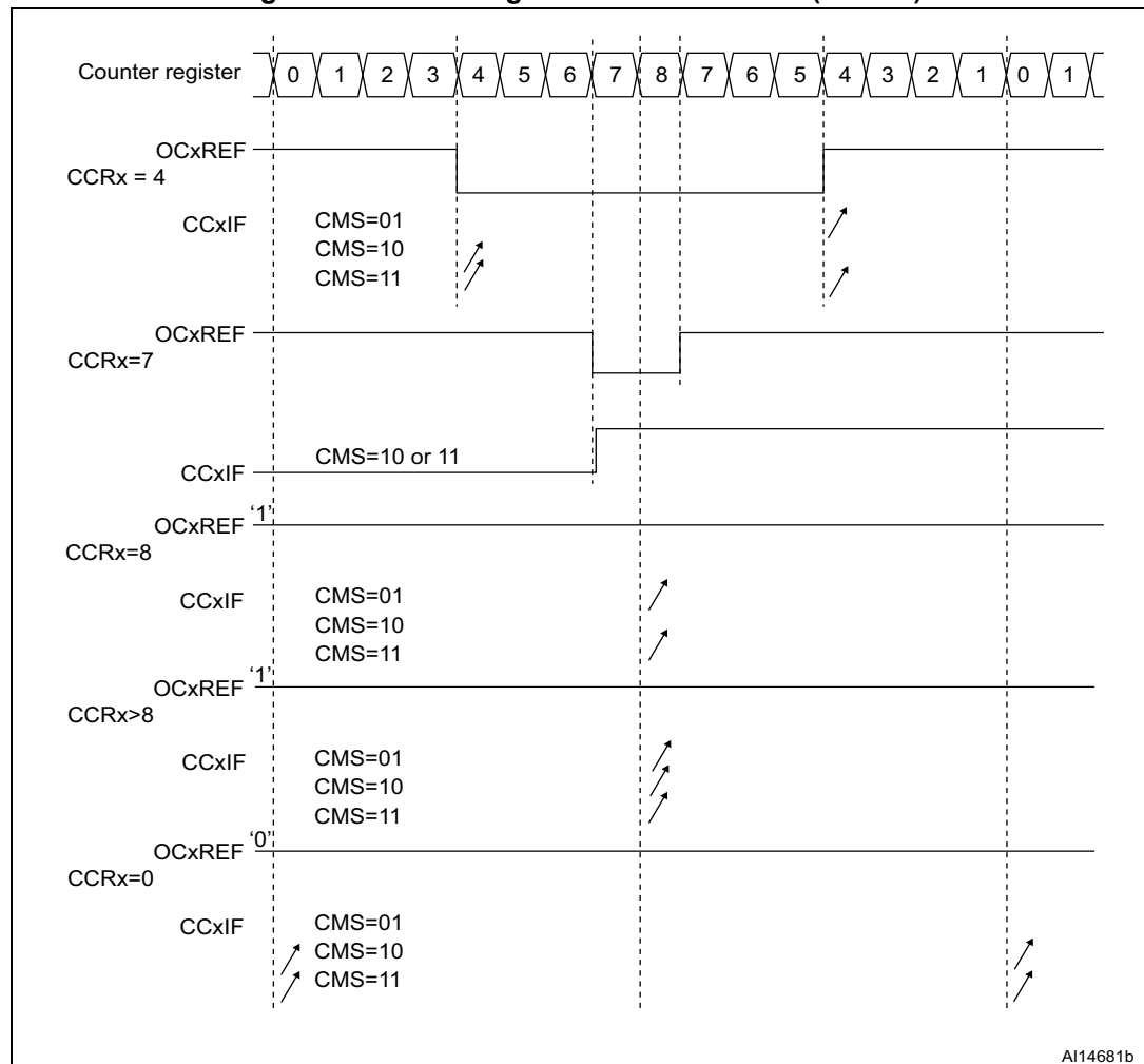
Figure 82. Center-aligned PWM waveforms (ARR=8)
