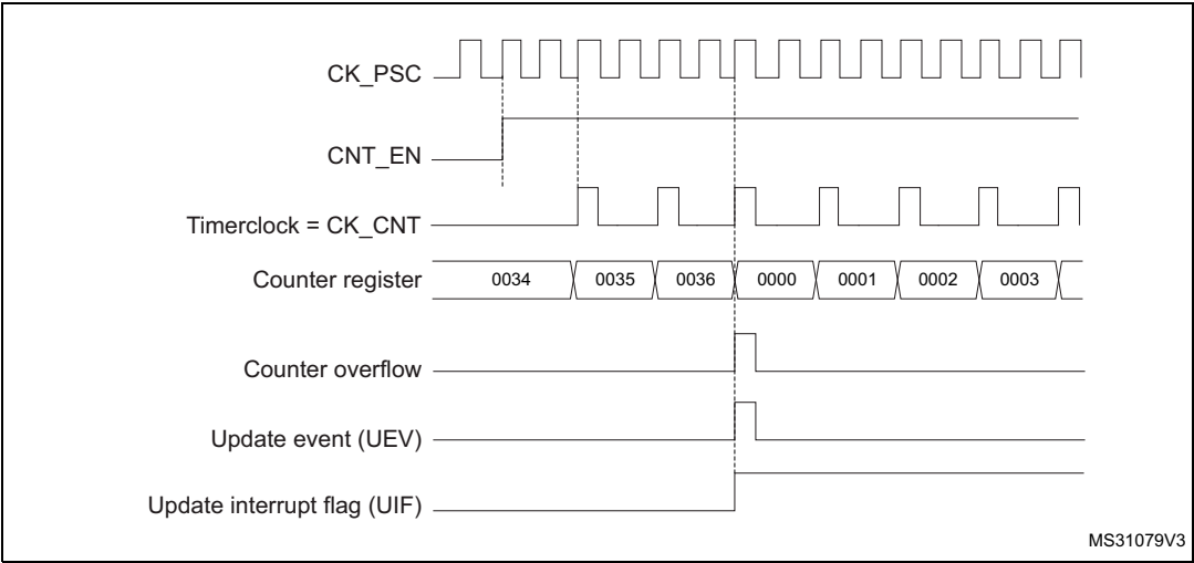
Figure 53. Counter timing diagram, internal clock divided by 2
