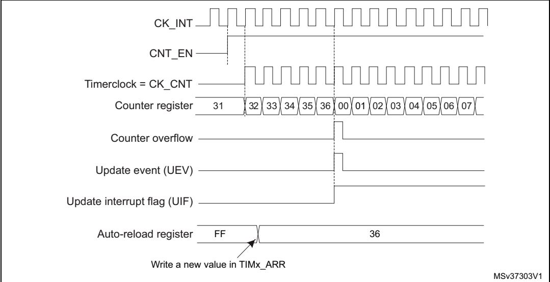
Figure 104. Counter timing diagram, Update event when ARPE=0 (TIMx_ARR not preloaded)
