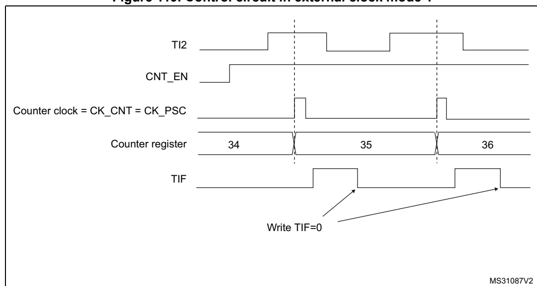
Figure 119. Control circuit in external clock mode 1
