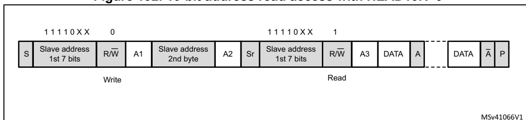
Figure 192. 10-bit address read access with HEAD10R=0
