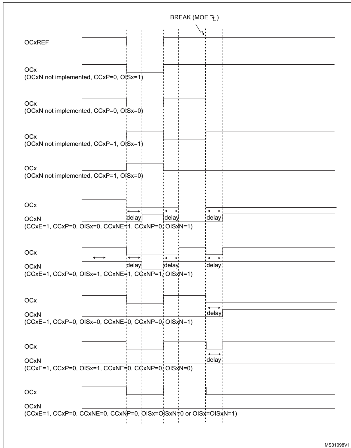
Figure 86. Output behavior in response to a break.
