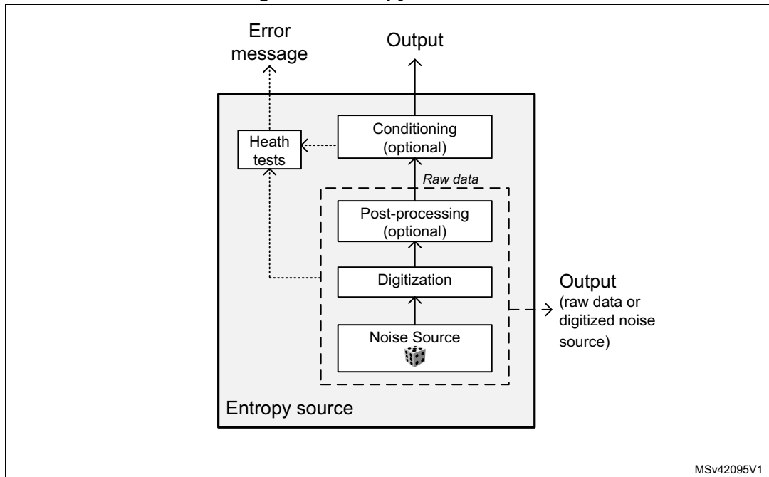
Figure 48. Entropy source model
