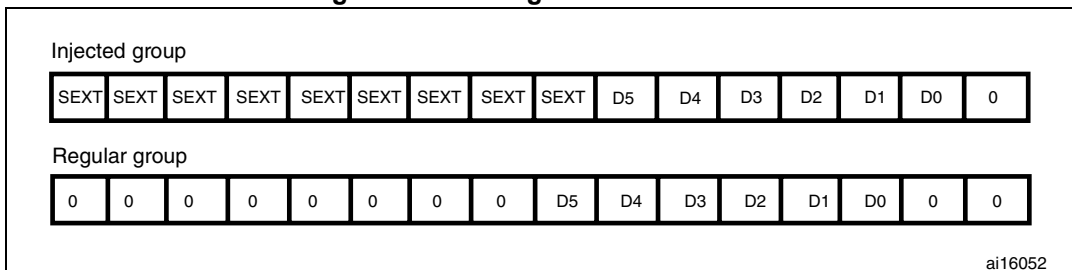
Figure 38. Left alignment of 6-bit data
