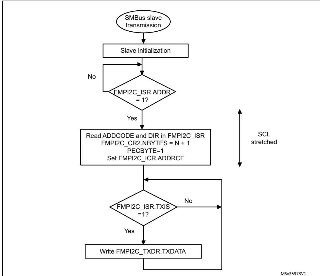
Figure 201. Transfer sequence flowchart for SMBus slave transmitter N bytes + PEC
