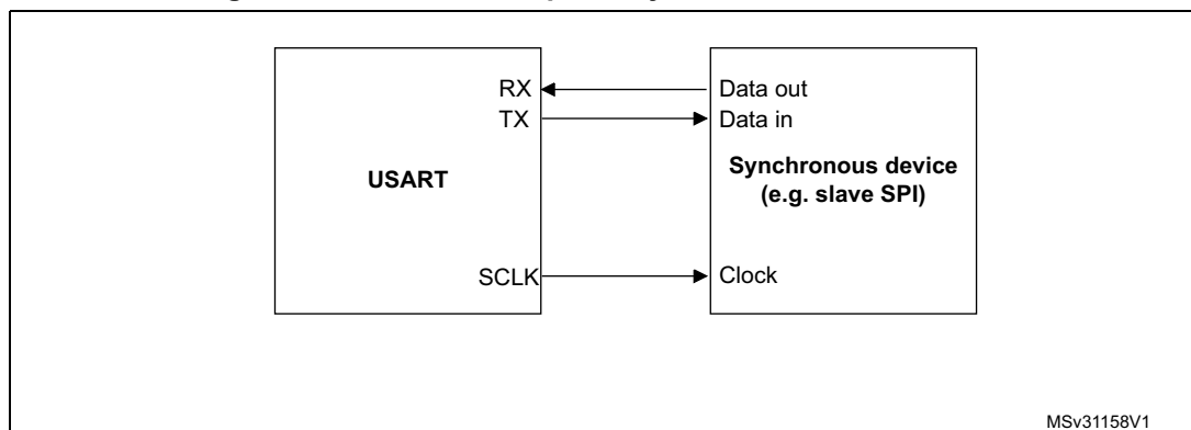
Figure 225. USART example of synchronous transmission
