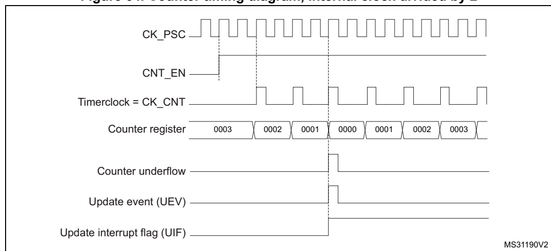
Figure 64. Counter timing diagram, internal clock divided by 2
