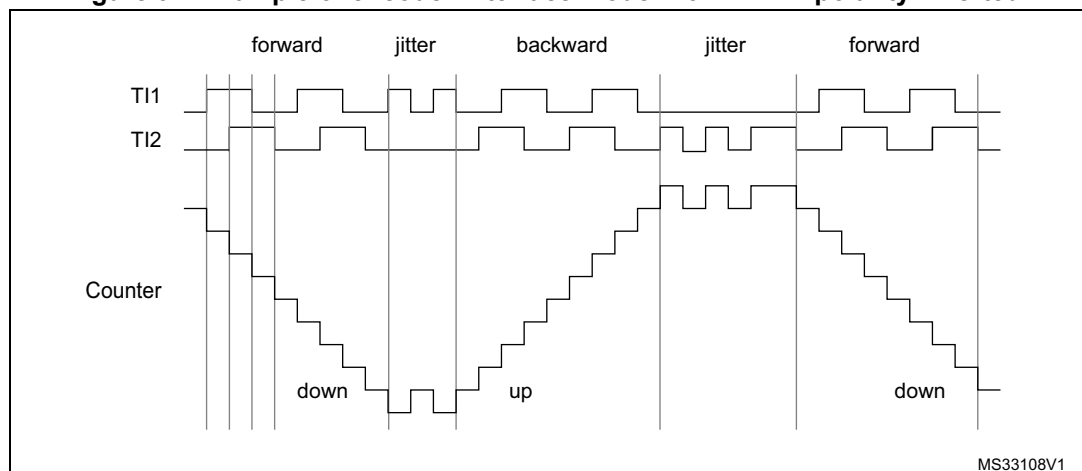
Figure 91. Example of encoder interface mode with TI1FP1 polarity inverted.
