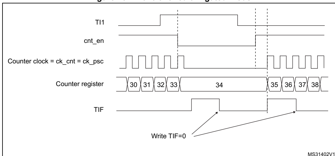
Figure 154. Control circuit in gated mode
