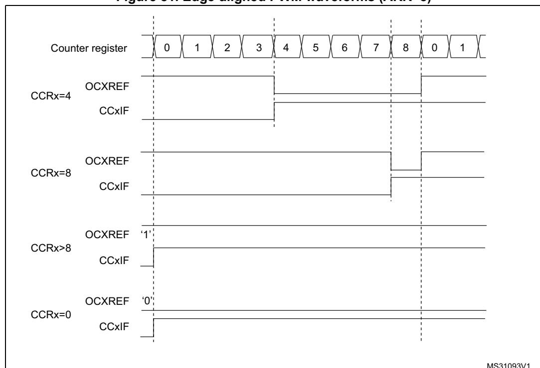
Figure 81. Edge-aligned PWM waveforms (ARR=8)
