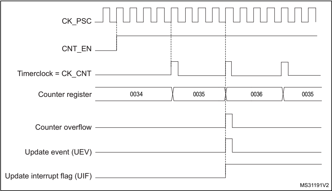
Figure 65. Counter timing diagram, internal clock divided by 4, TIMx_ARR=0x36
