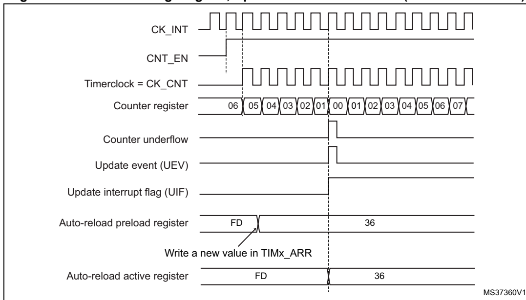
Figure 115. Counter timing diagram, Update event with ARPE=1 (counter underflow)
