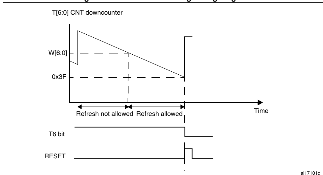
Figure 174. Window watchdog timing diagram
