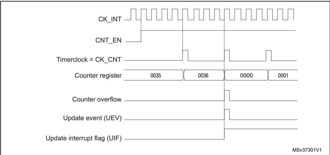
Figure 102. Counter timing diagram, internal clock divided by 4
