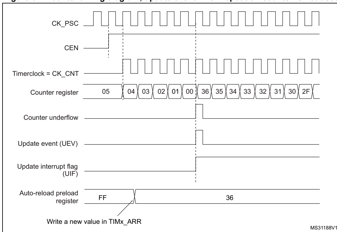
Figure 62. Counter timing diagram, update event when repetition counter is not used
