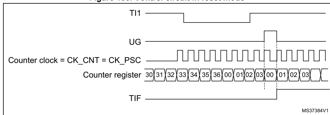
Figure 130. Control circuit in reset mode
