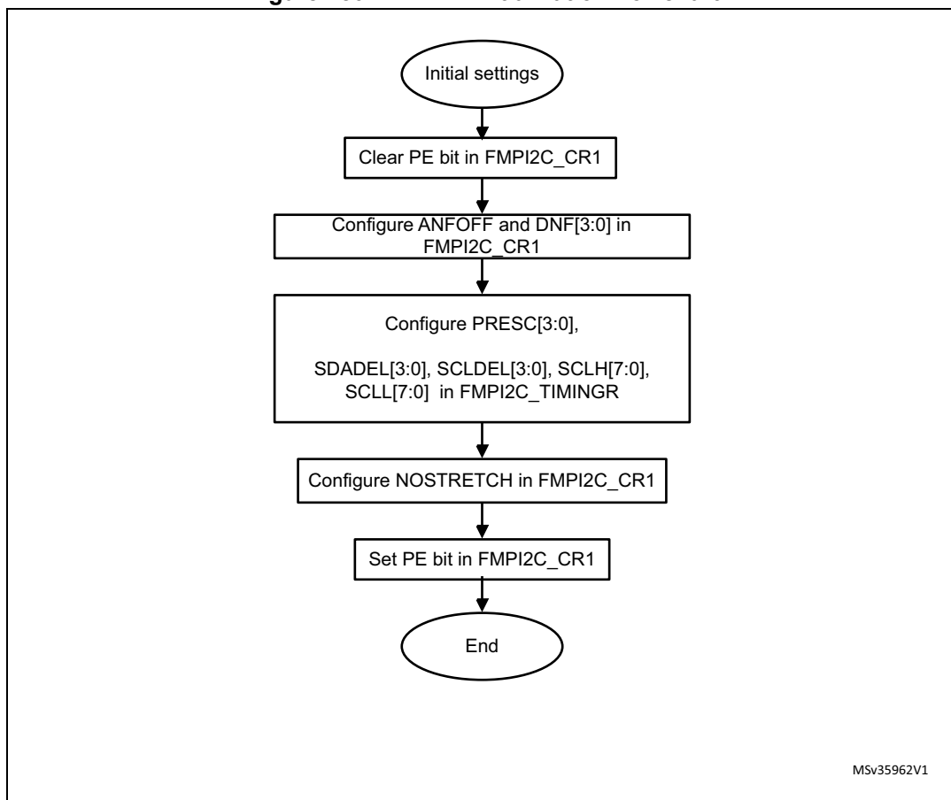
Figure 180. FMPI2C initialization flowchart
