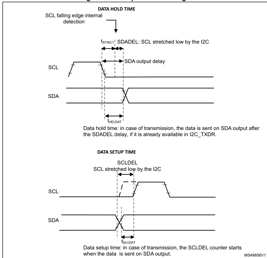
Figure 179. Setup and hold timings
