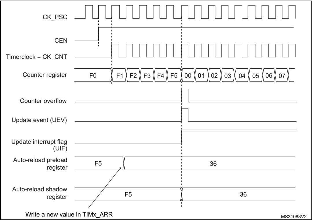
Figure 57. Counter timing diagram, update event when ARPE=1 (TIMx_ARR preloaded)
