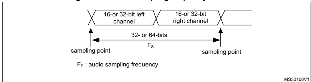
Figure 271. Audio sampling frequency definition
