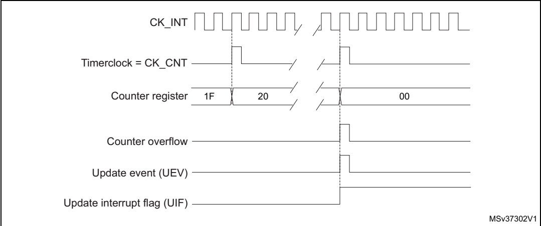
Figure 103. Counter timing diagram, internal clock divided by N
