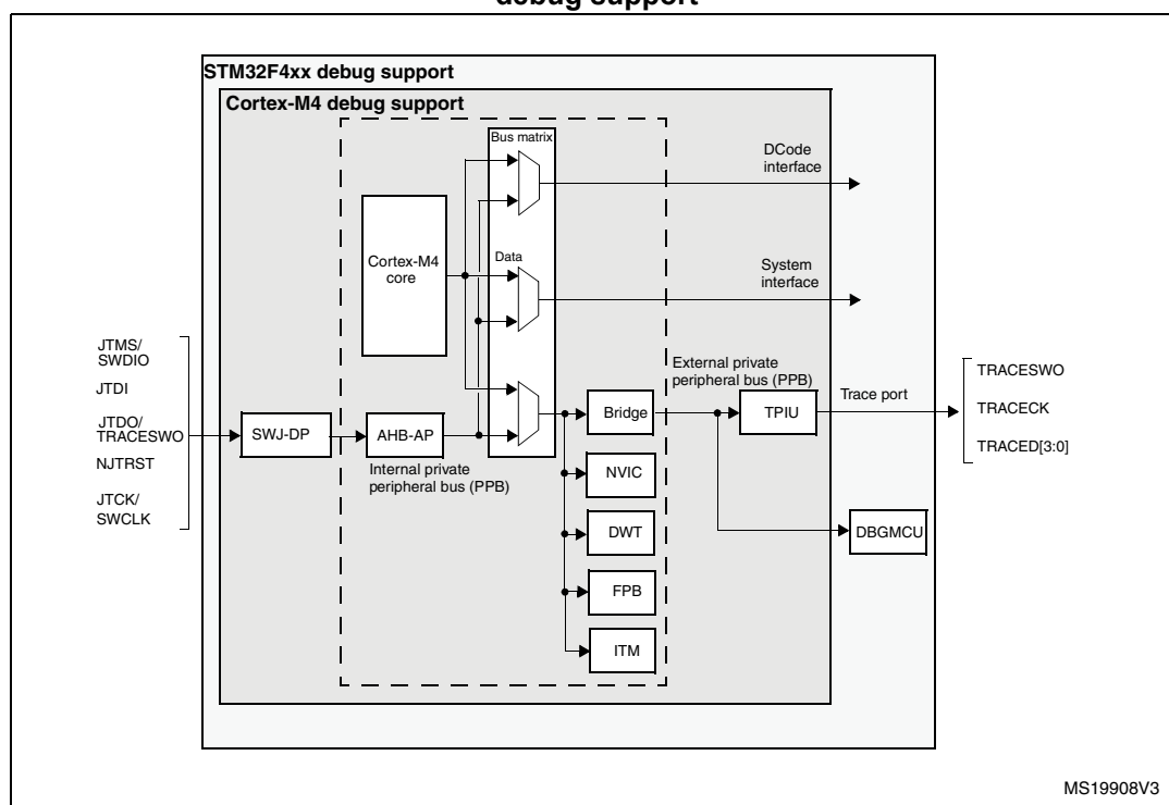
Figure 273. Block diagram of STM32 MCU and Cortex ® -M4 with FPU-level debug support
