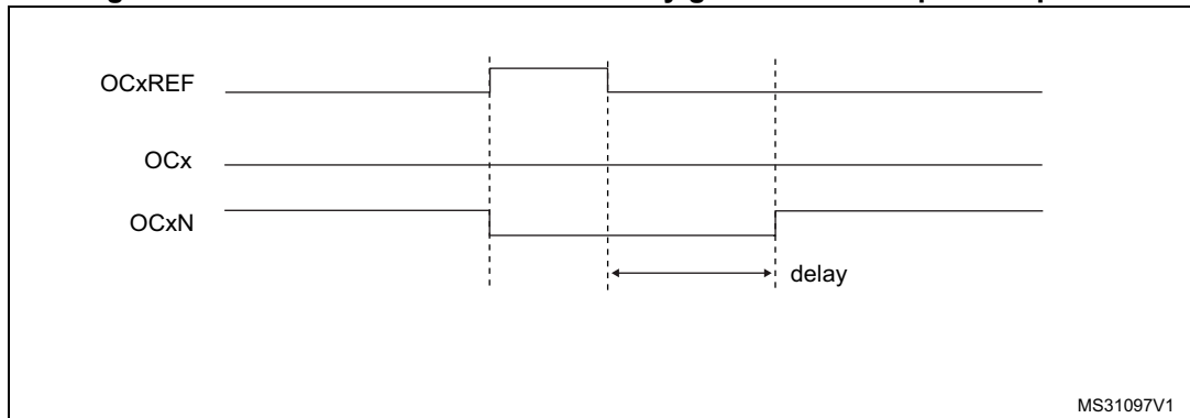
Figure 85. Dead-time waveforms with delay greater than the positive pulse.
