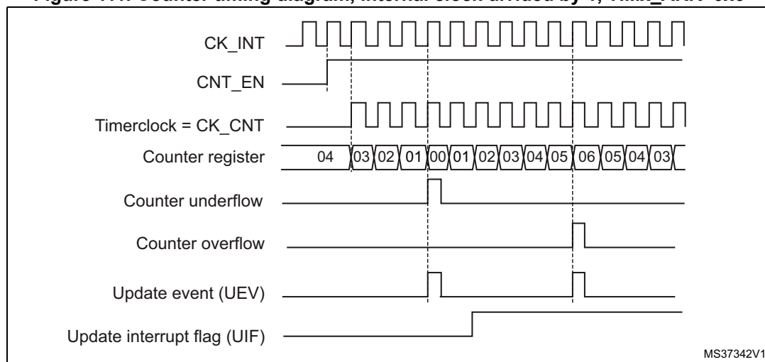
Figure 111. Counter timing diagram, internal clock divided by 1, TIMx_ARR=0x6
