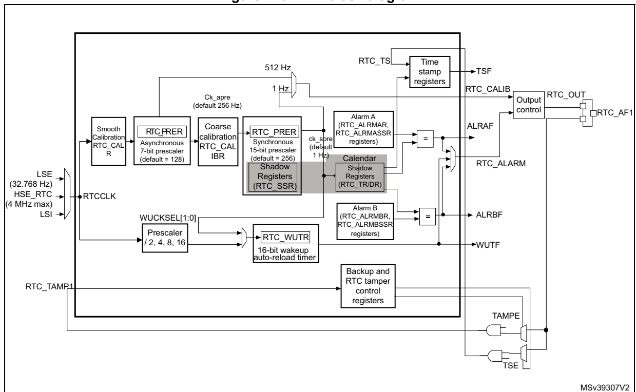
Figure 176. RTC block diagram
