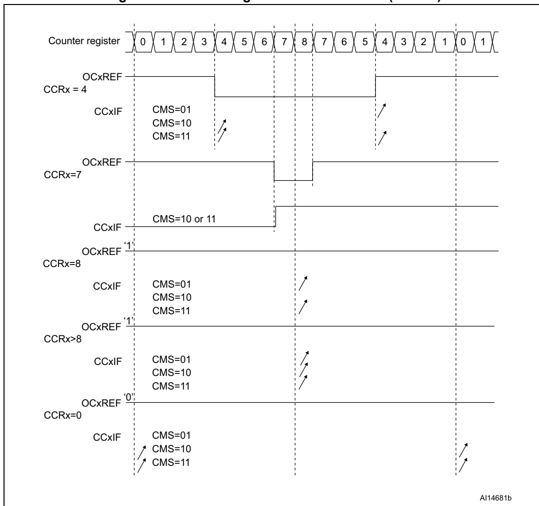
Figure 126. Center-aligned PWM waveforms (ARR=8)
