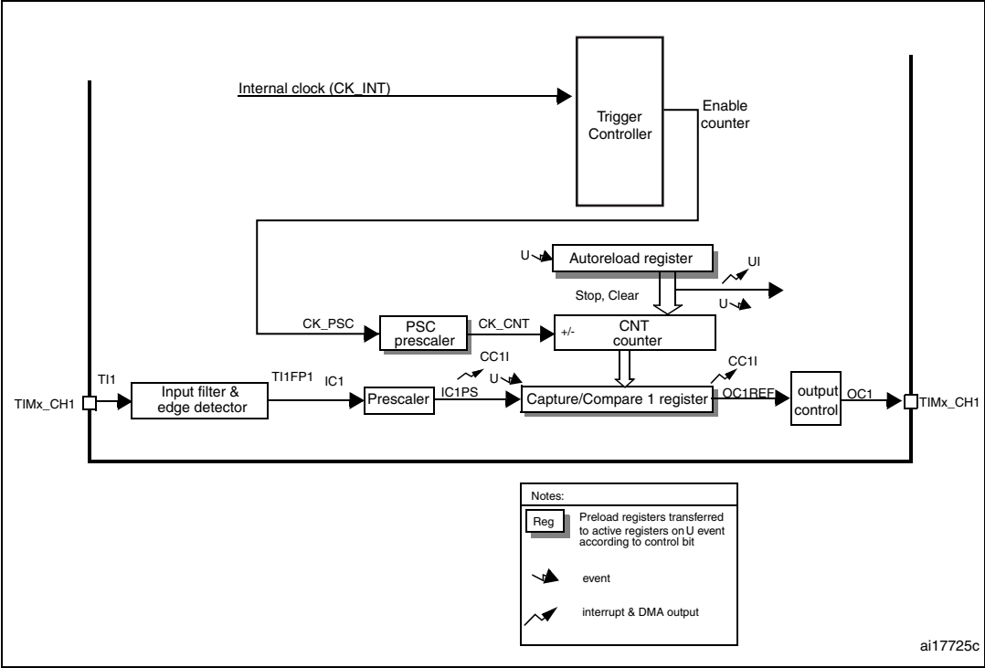
Figure 134. General-purpose timer block diagram (TIM11)
