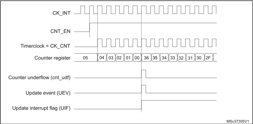
Figure 106. Counter timing diagram, internal clock divided by 1
