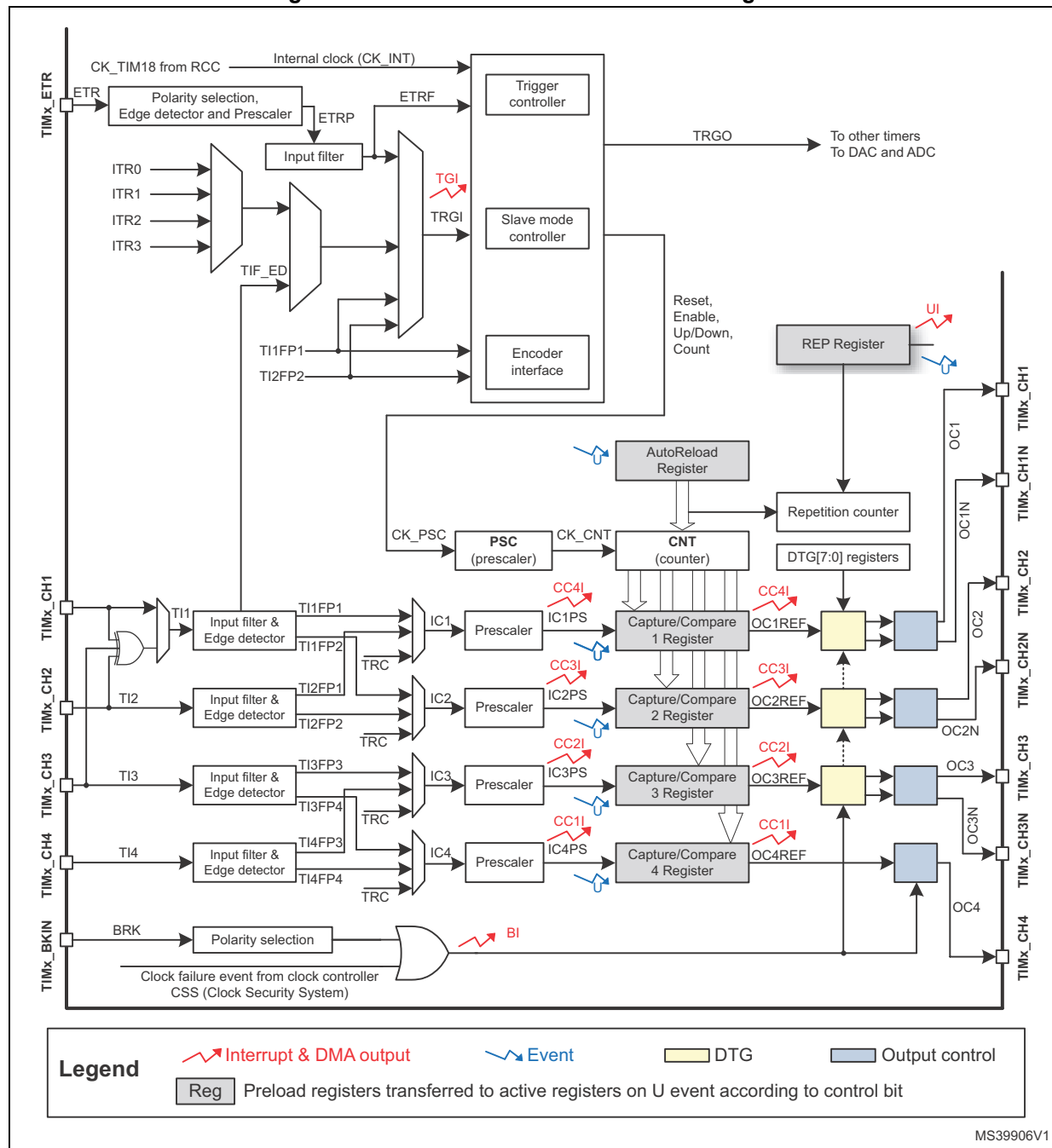
Figure 49. Advanced-control timer block diagram
