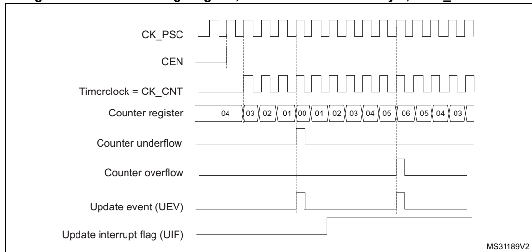
Figure 63. Counter timing diagram, internal clock divided by 1, TIMx_ARR = 0x6
