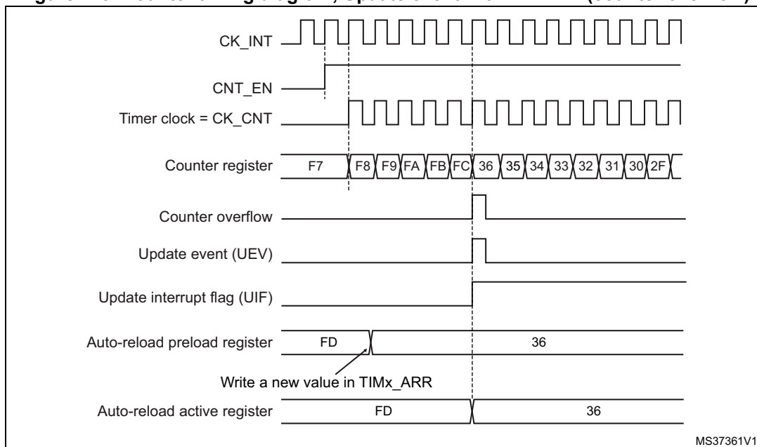
Figure 116. Counter timing diagram, Update event with ARPE=1 (counter overflow)
