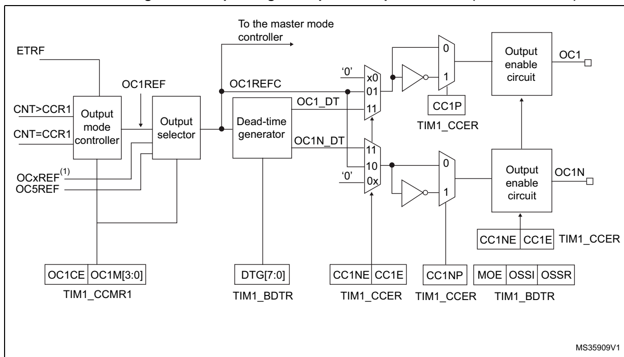
Figure 77. Output stage of capture/compare channel (channels 1 to 3)
