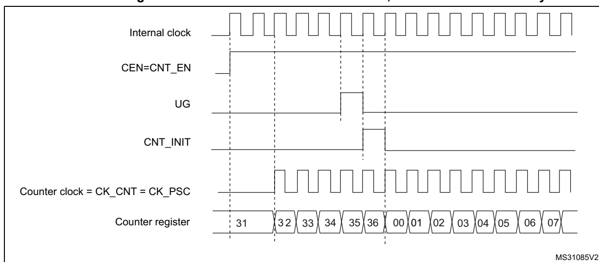
Figure 143. Control circuit in normal mode, internal clock divided by 1
