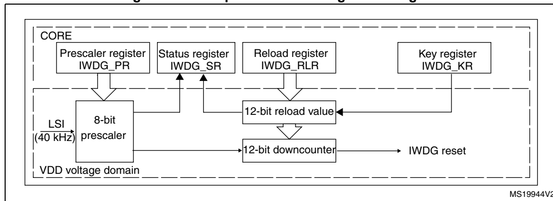
Figure 175. Independent watchdog block diagram
