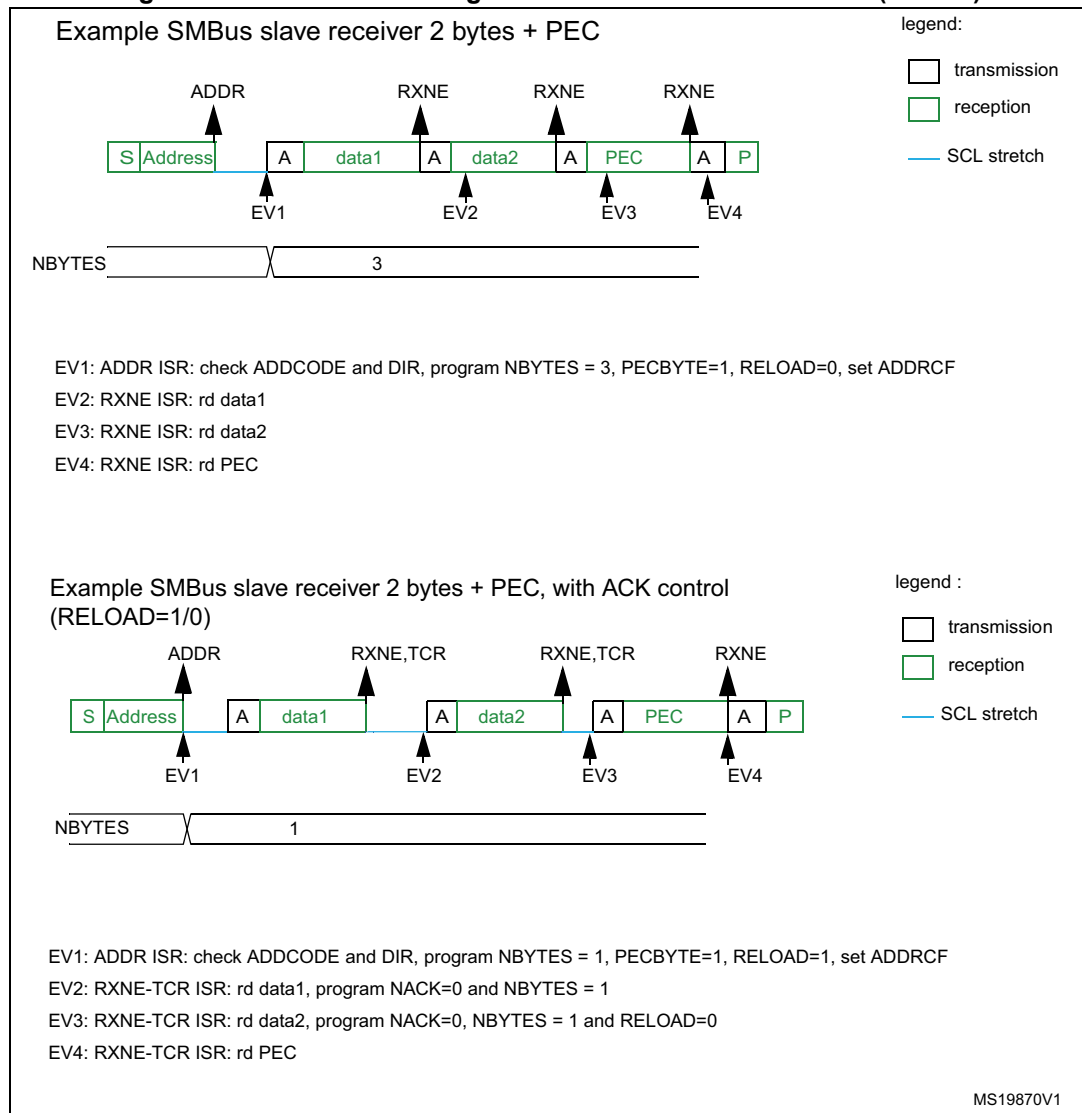
Figure 204. Bus transfer diagrams for SMBus slave receiver (SBC=1)
