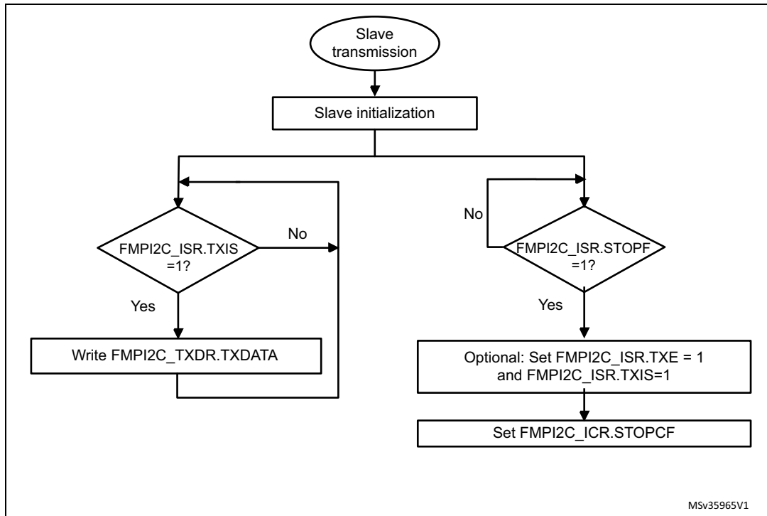
Figure 185. Transfer sequence flowchart for FMPI2C slave transmitter, NOSTRETCH= 1
