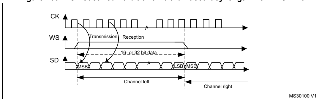
Figure 260. MSB Justified 16-bit or 32-bit full-accuracy length with CPOL = 0
