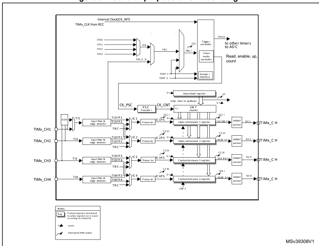
Figure 97. General-purpose timer block diagram
