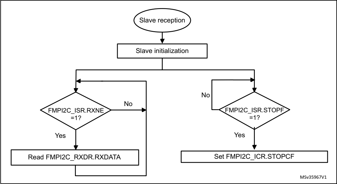
Figure 188. Transfer sequence flowchart for slave receiver with NOSTRETCH=1
