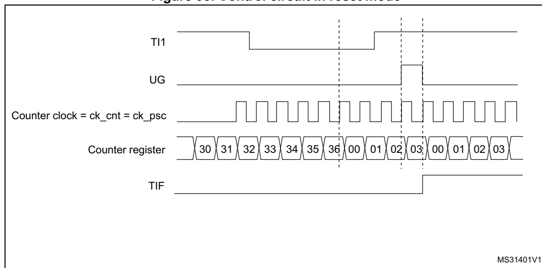
Figure 93. Control circuit in reset mode
