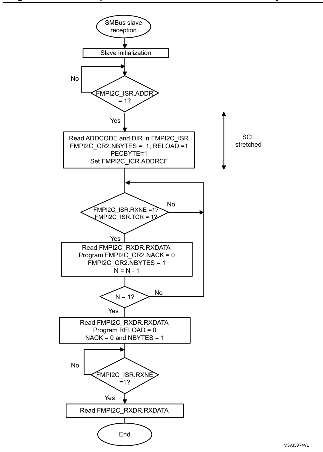
Figure 203. Transfer sequence flowchart for SMBus slave receiver N Bytes + PEC
