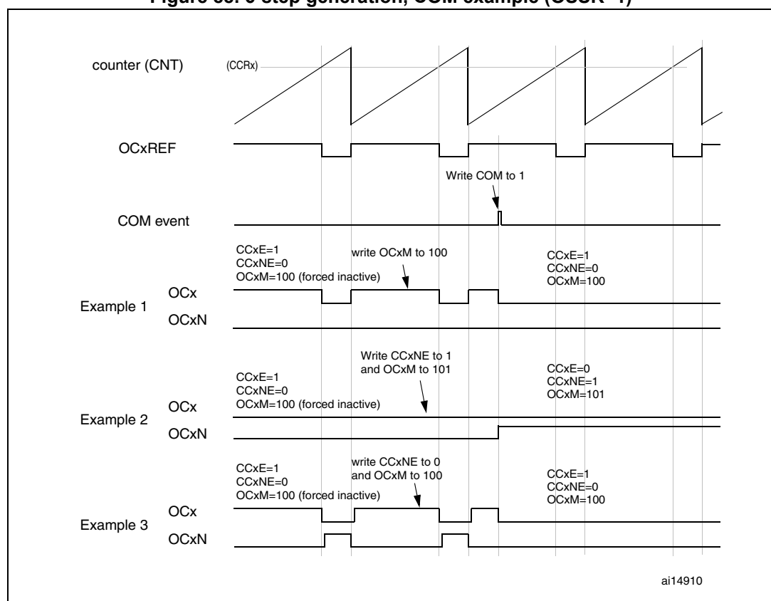
Figure 88. 6-step generation, COM example (OSSR=1)
