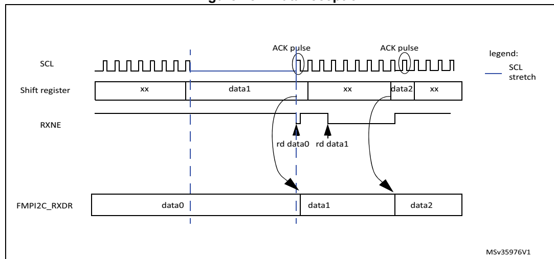
Figure 181. Data reception
