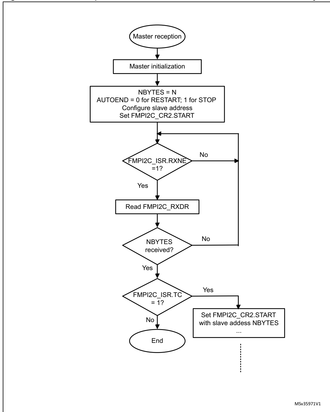
Figure 197. Transfer sequence flowchart for FMPI2C master receiver for N \leq 255 bytes
