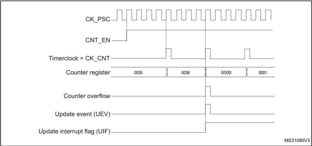
Figure 54. Counter timing diagram, internal clock divided by 4
