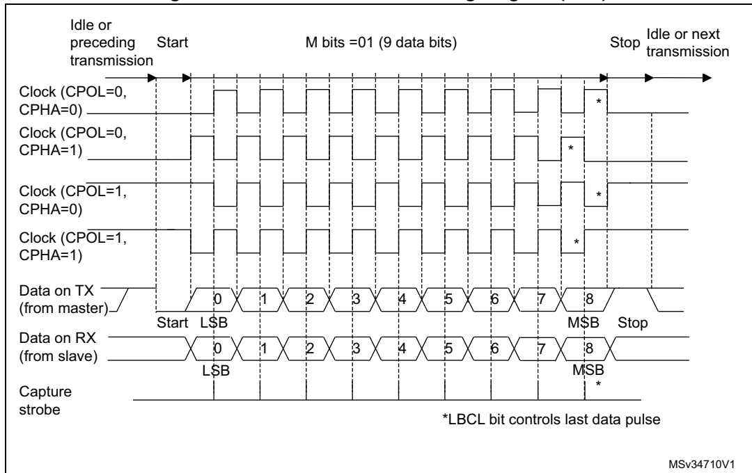
Figure 227. USART data clock timing diagram (M=1)
