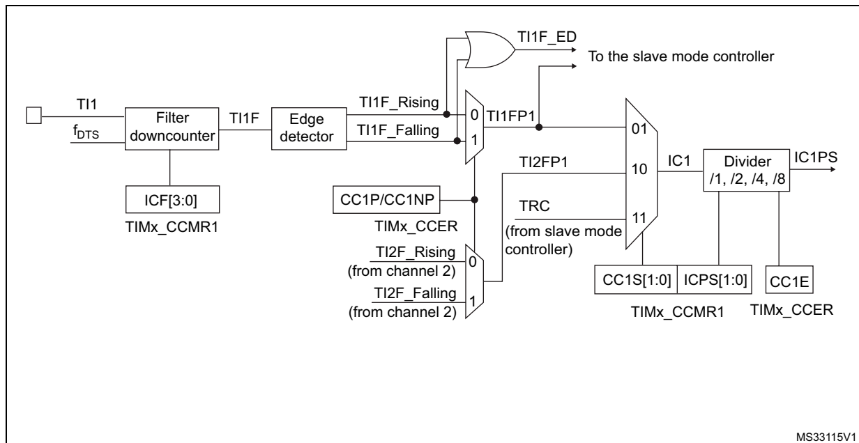
Figure 75. Capture/compare channel (example: channel 1 input stage)
