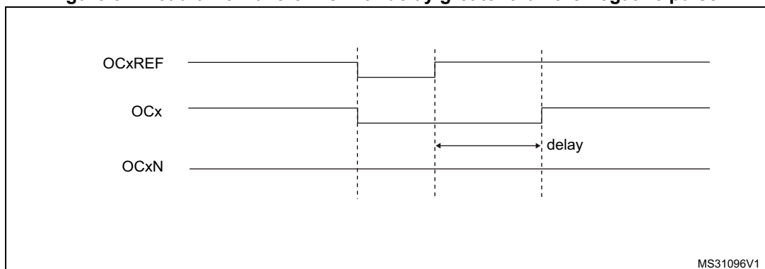
Figure 84. Dead-time waveforms with delay greater than the negative pulse.
