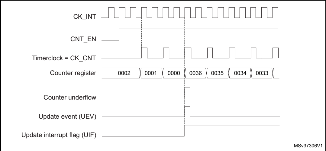
Figure 107. Counter timing diagram, internal clock divided by 2
