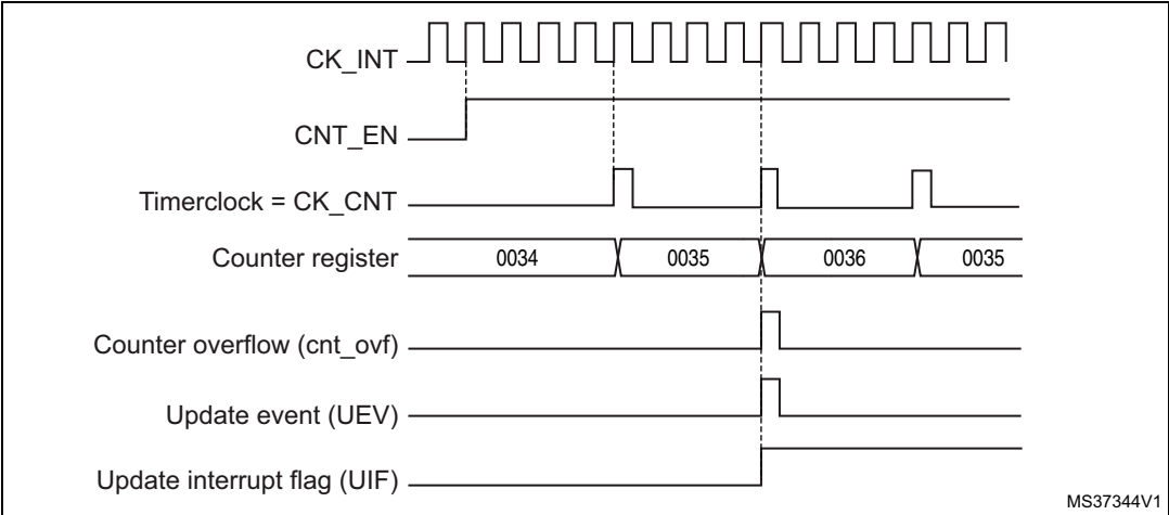
Figure 113. Counter timing diagram, internal clock divided by 4, TIMx_ARR=0x36
