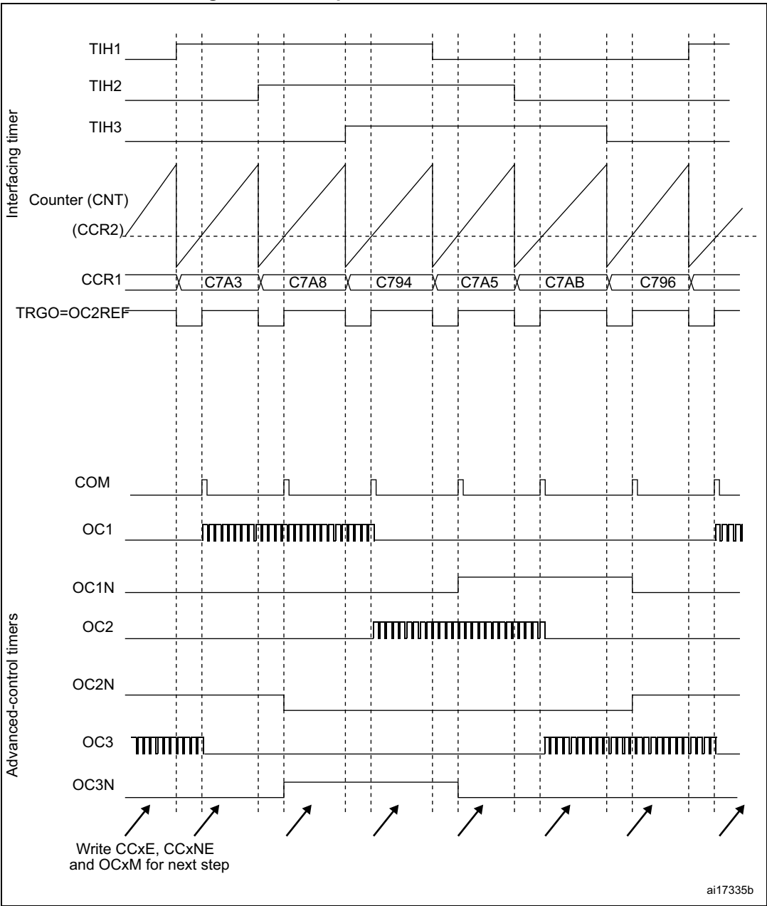
Figure 92. Example of Hall sensor interface
