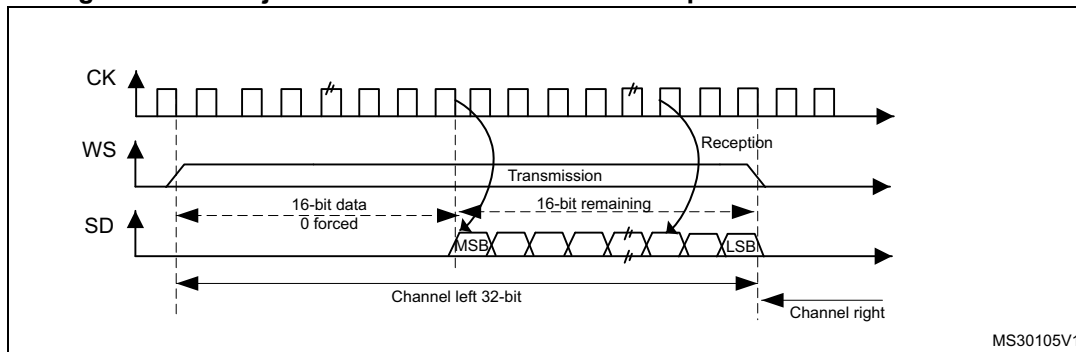
Figure 267. LSB justified 16-bit extended to 32-bit packet frame with CPOL = 0
