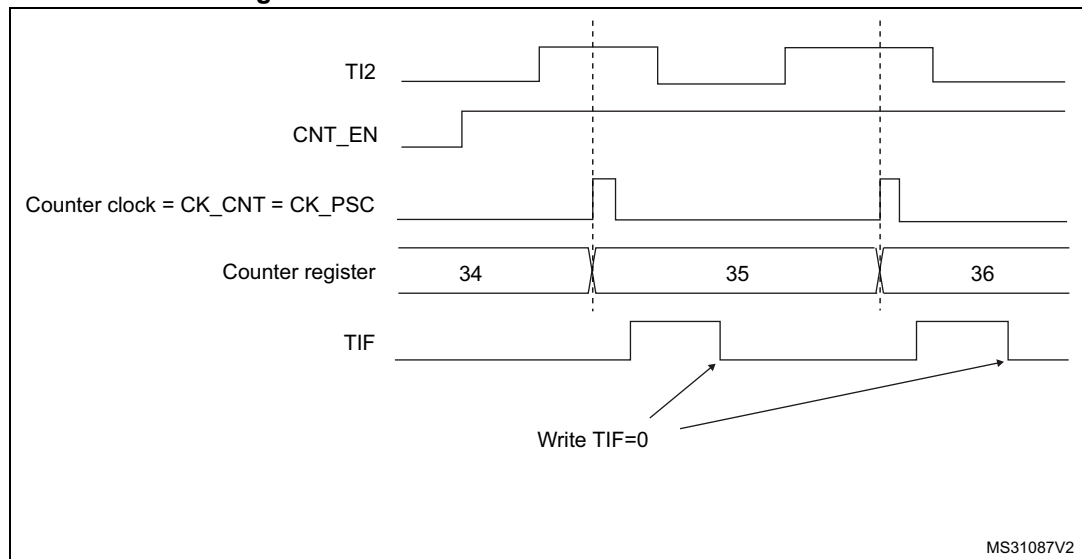
Figure 72. Control circuit in external clock mode 1
