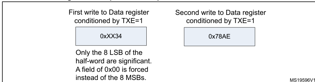
Figure 265. Operations required to transmit 0x3478AE
