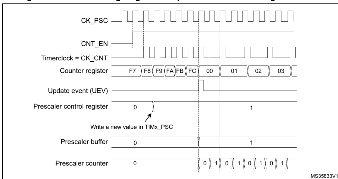
Figure 98. Counter timing diagram with prescaler division change from 1 to 2
