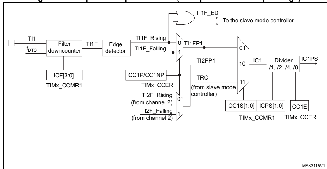
Figure 146. Capture/compare channel (example: channel 1 input stage)
