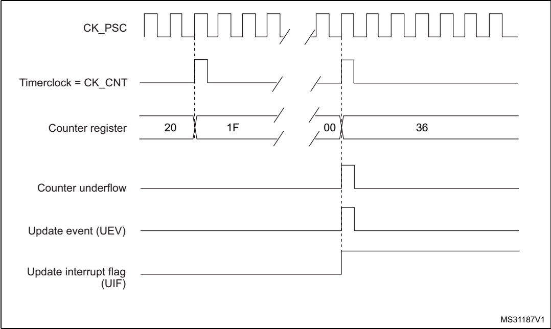
Figure 61. Counter timing diagram, internal clock divided by N
