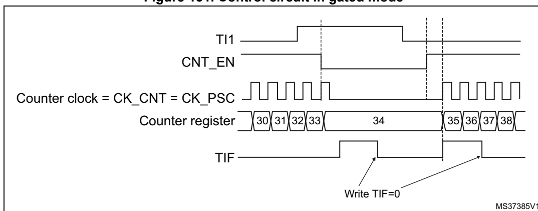
Figure 131. Control circuit in gated mode
