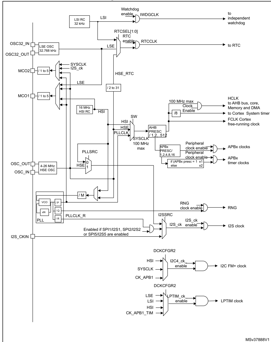
Figure 12. Clock tree
