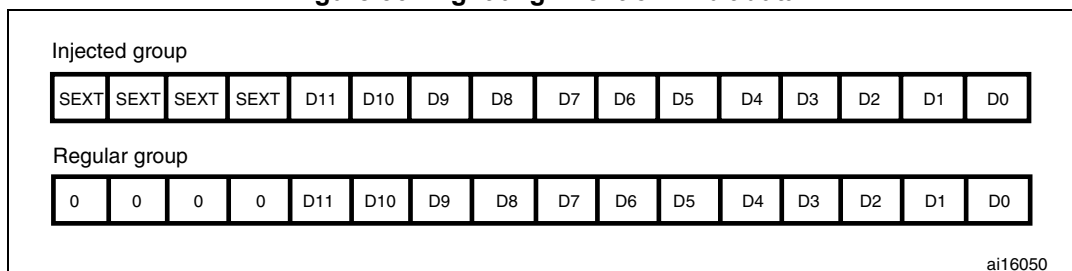
Figure 36. Right alignment of 12-bit data
