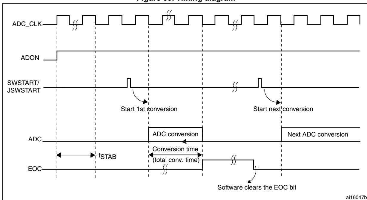
Figure 33. Timing diagram
