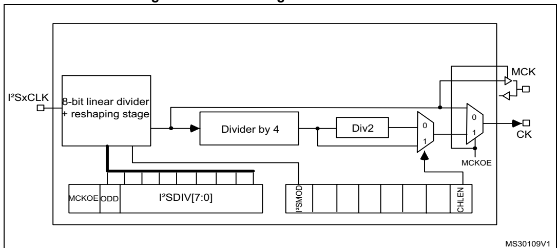
Figure 272. I 2 S clock generator architecture
