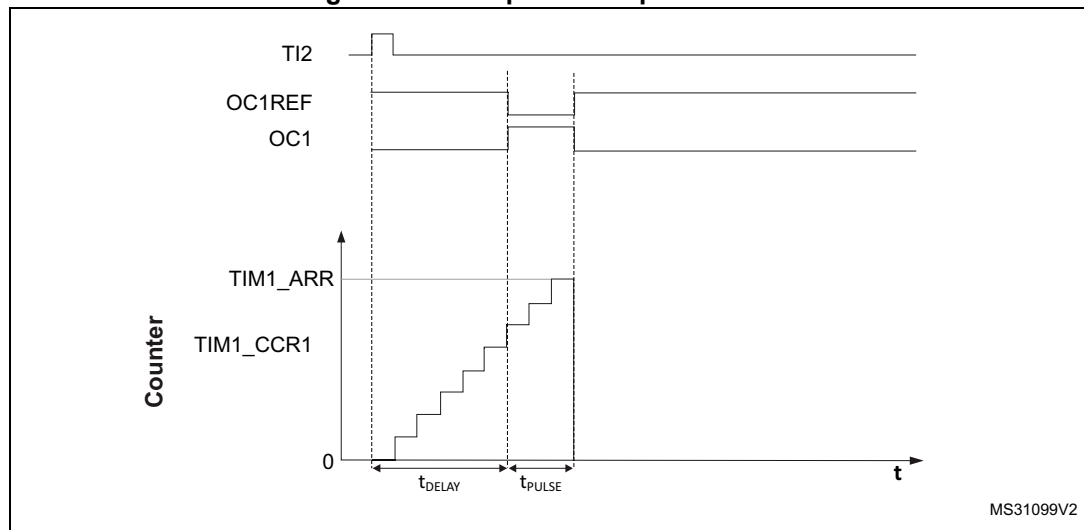
Figure 89. Example of one pulse mode.
