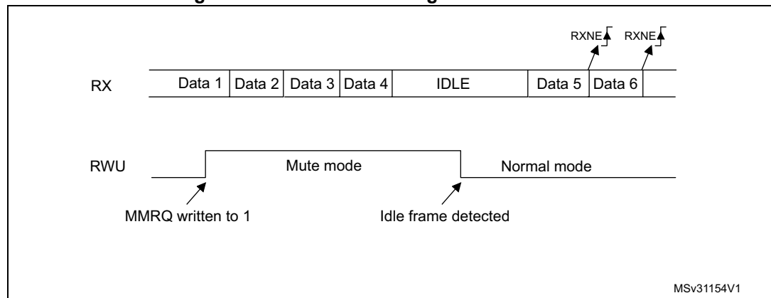
Figure 221. Mute mode using Idle line detection
