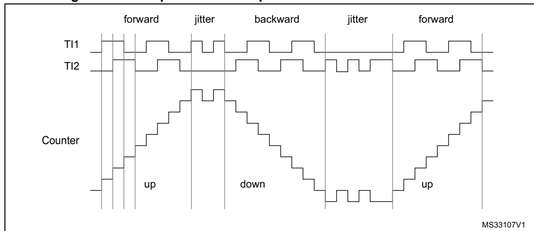
Figure 90. Example of counter operation in encoder interface mode.
