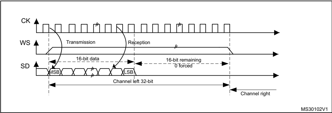
Figure 262. MSB justified 16-bit extended to 32-bit packet frame with CPOL = 0
