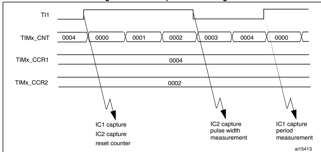
Figure 79. PWM input mode timing
