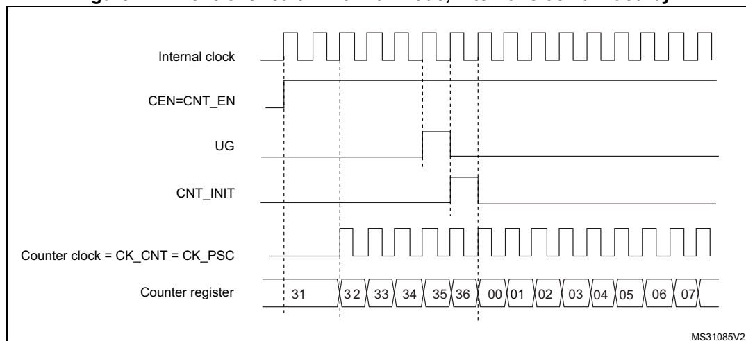
Figure 117. Control circuit in normal mode, internal clock divided by 1
