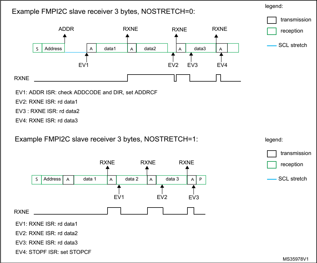
Figure 189. Transfer bus diagrams for FMPI2C slave receiver
