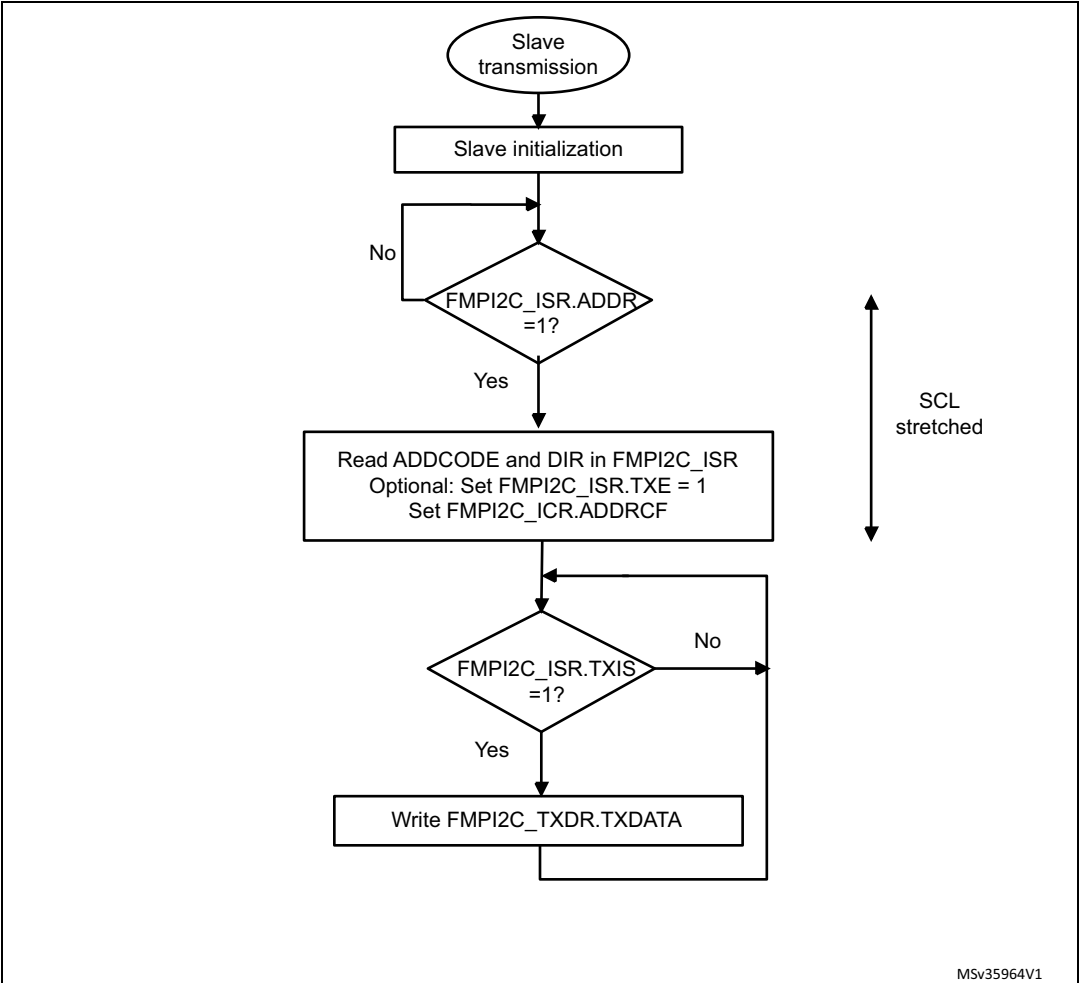
Figure 184. Transfer sequence flowchart for FMPI2C slave transmitter, NOSTRETCH= 0
