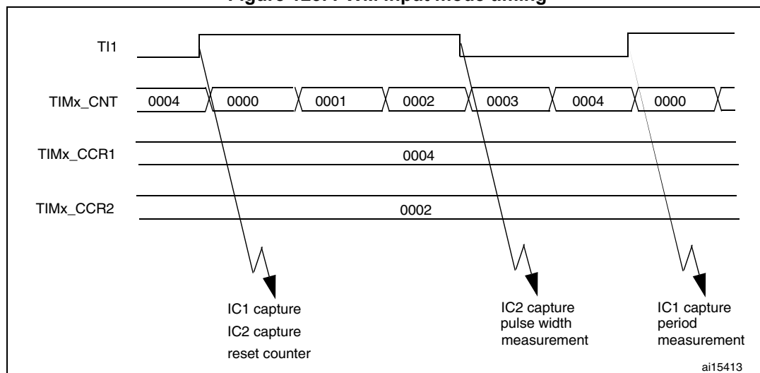
Figure 123. PWM input mode timing
