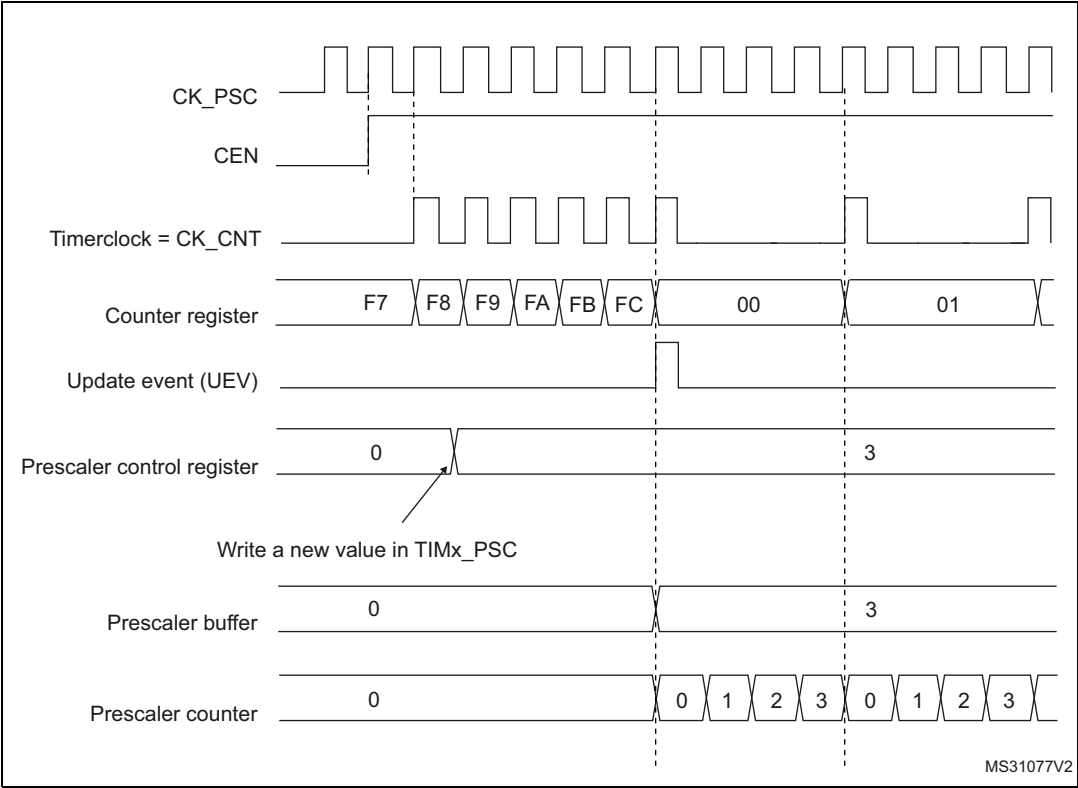
Figure 51. Counter timing diagram with prescaler division change from 1 to 4
