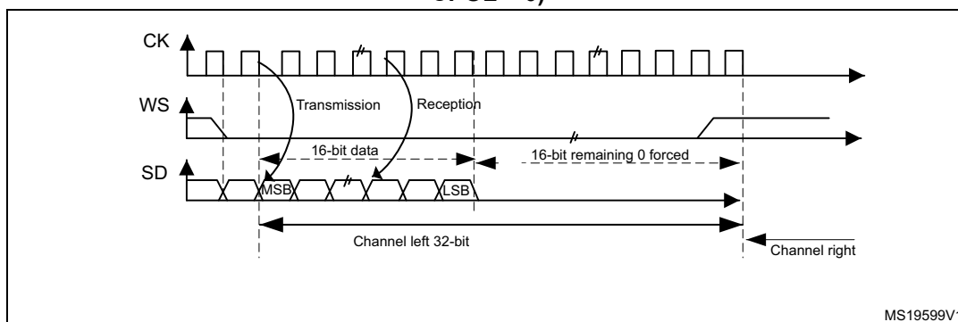
Figure 258. I 2 S Philips standard (16-bit extended to 32-bit packet frame with CPOL = 0)
