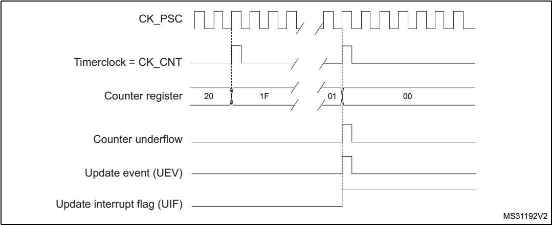
Figure 66. Counter timing diagram, internal clock divided by N
