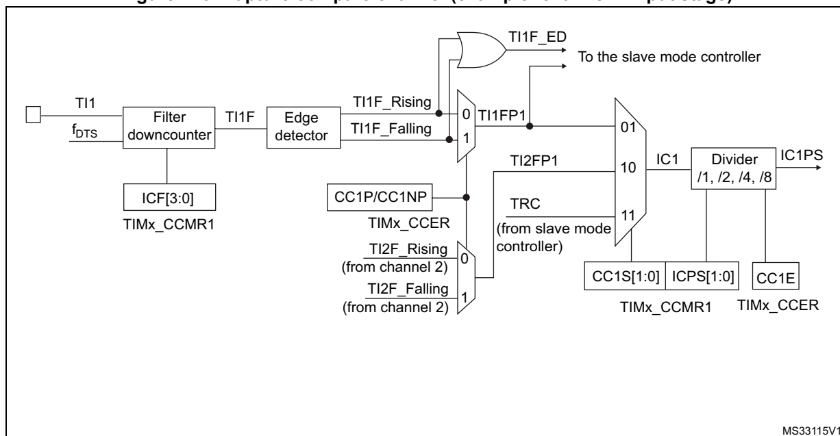
Figure 120. Capture/compare channel (example: channel 1 input stage)
