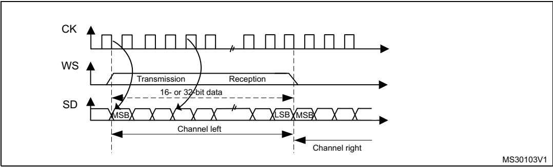
Figure 263. LSB justified 16-bit or 32-bit full-accuracy with CPOL = 0
