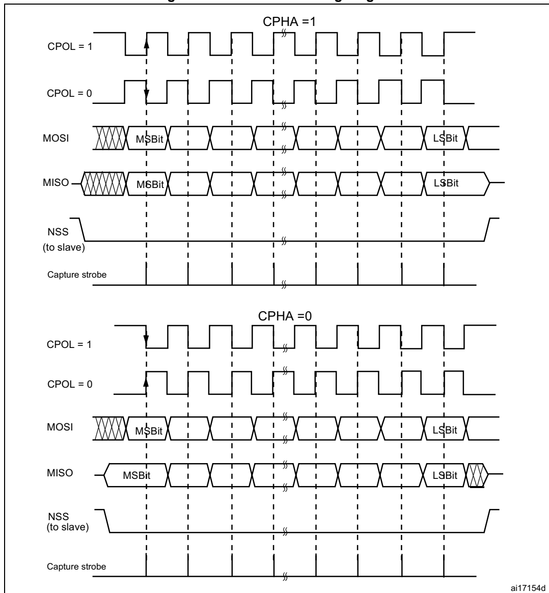
Figure 246. Data clock timing diagram
