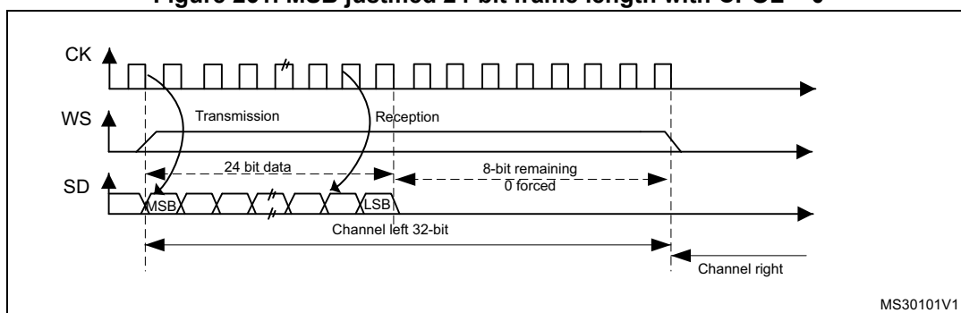
Figure 261. MSB justified 24-bit frame length with CPOL = 0
