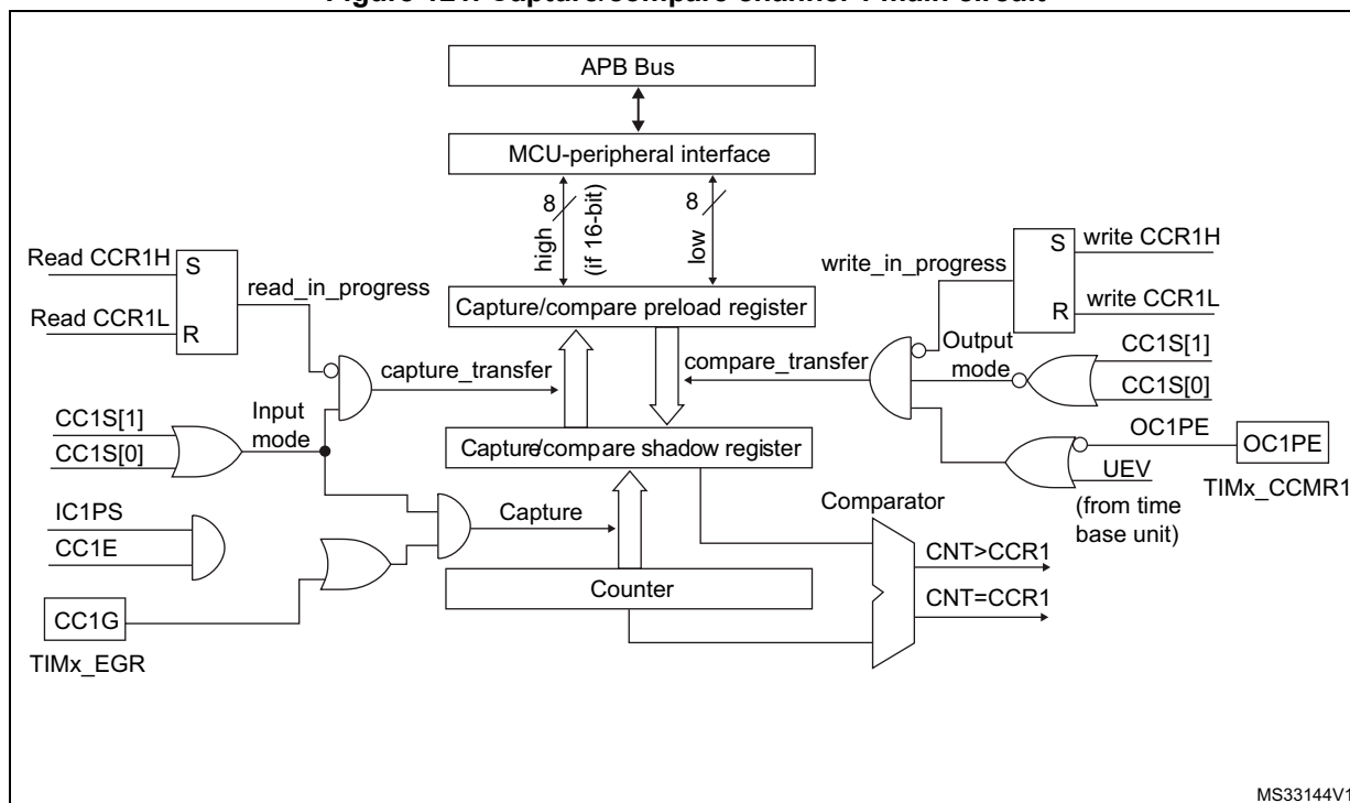
Figure 121. Capture/compare channel 1 main circuit
