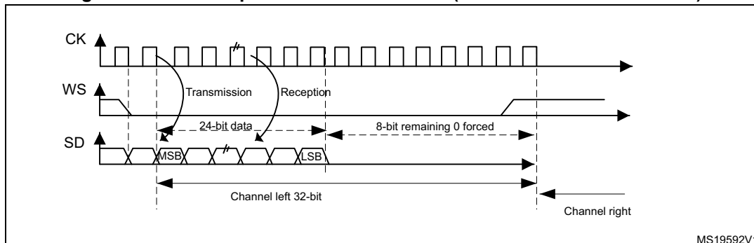
Figure 255. I 2 S Philips standard waveforms (24-bit frame with CPOL = 0)
