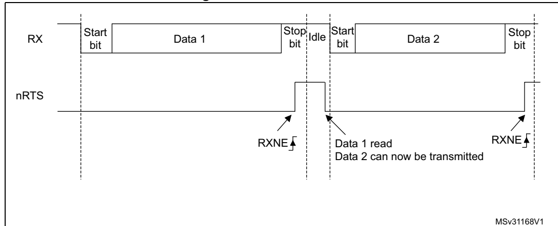
Figure 236. RTS flow control
