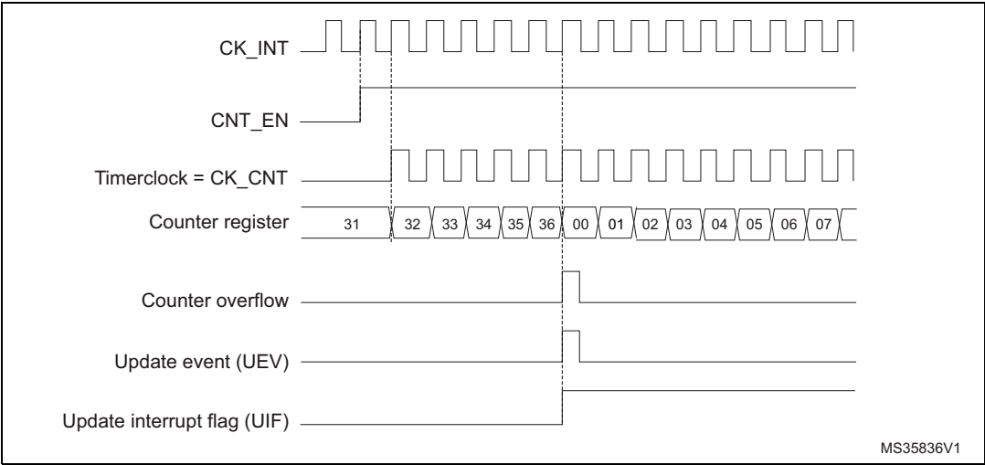
Figure 100. Counter timing diagram, internal clock divided by 1
