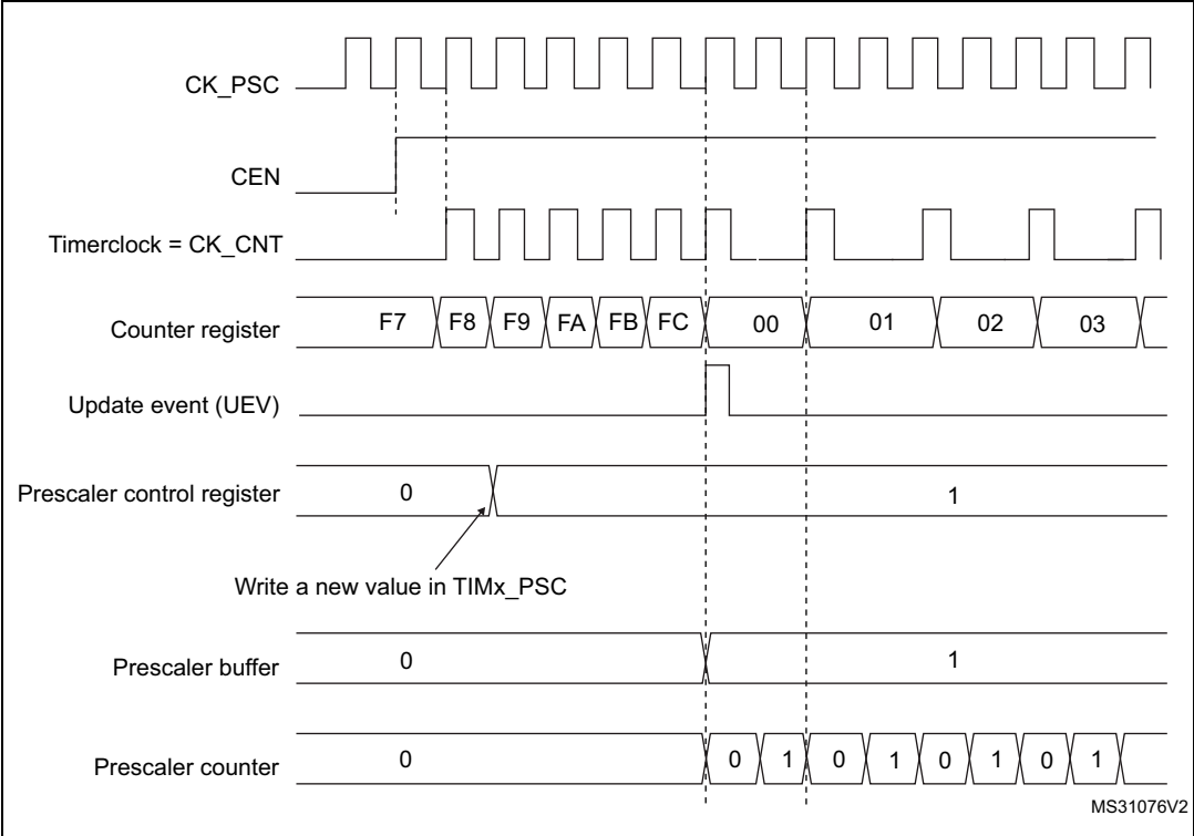
Figure 50. Counter timing diagram with prescaler division change from 1 to 2
