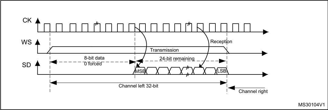
Figure 264. LSB justified 24-bit frame length with CPOL = 0
