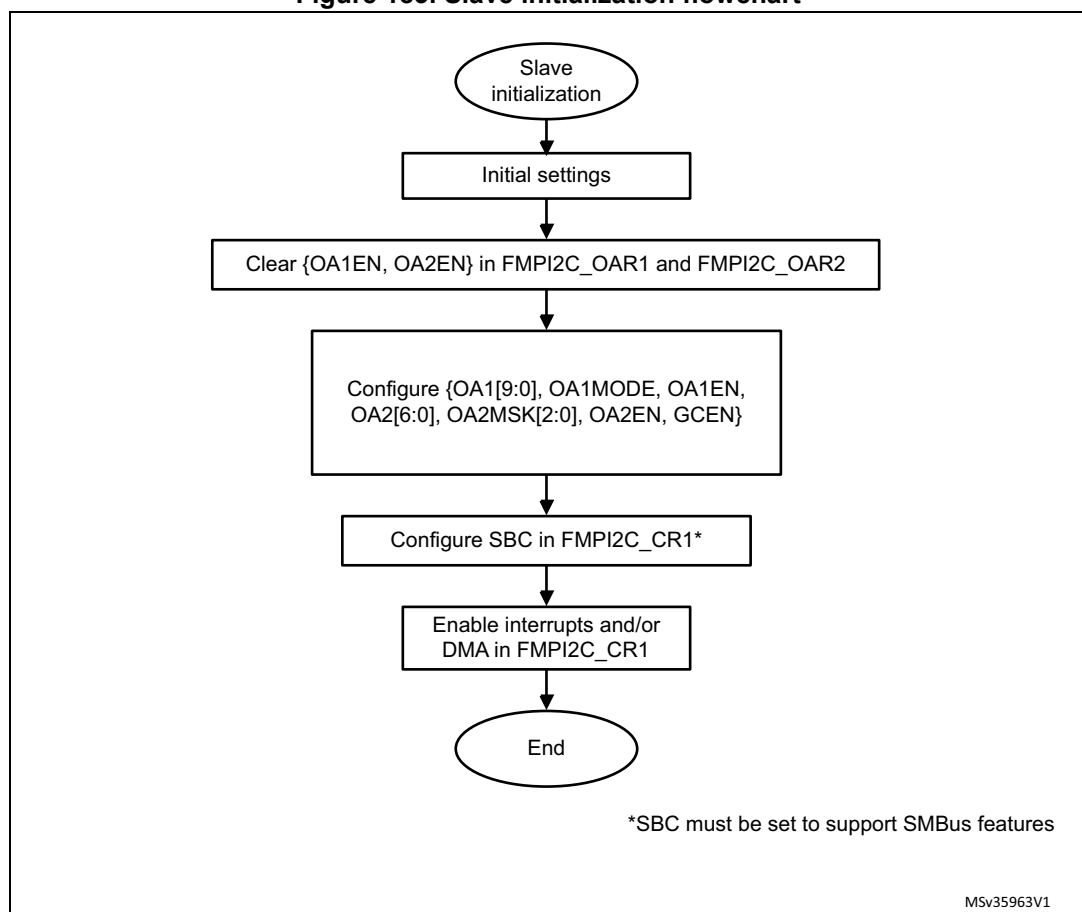
Figure 183. Slave initialization flowchart
