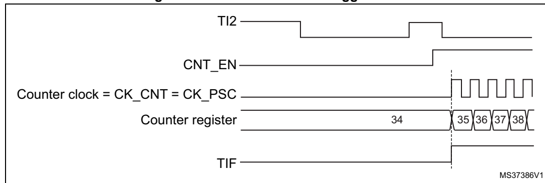
Figure 132. Control circuit in trigger mode
