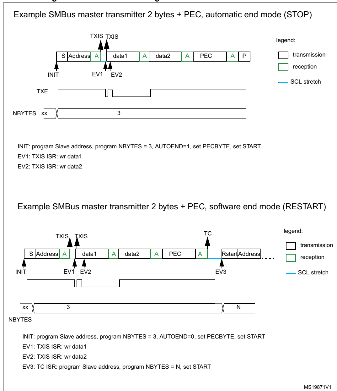
Figure 205. Bus transfer diagrams for SMBus master transmitter
