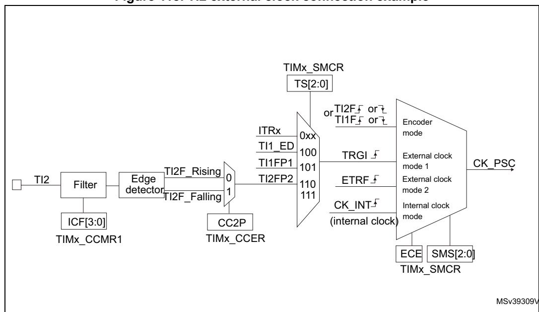
Figure 118. TI2 external clock connection example
