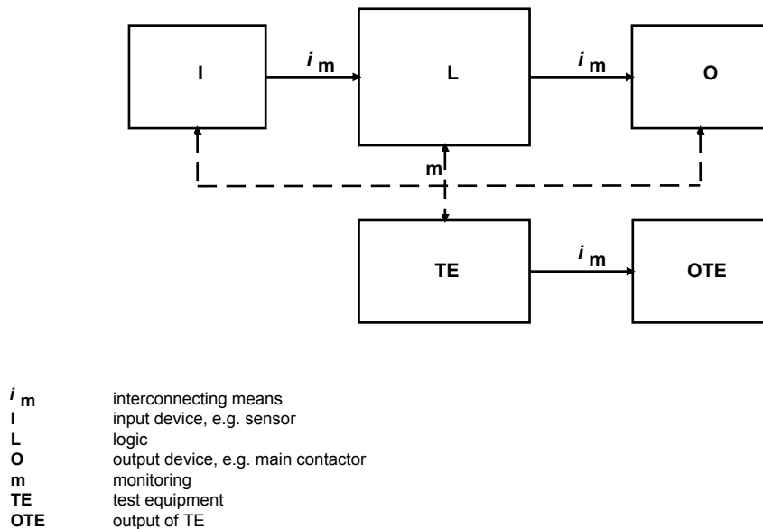
Figure 7. Block diagram for ISO 13849 Cat. 2
