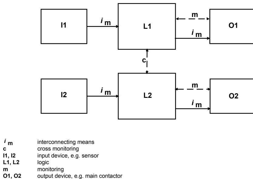
Figure 8. Block diagram for ISO 13849 Cat. 3 and Cat. 4
