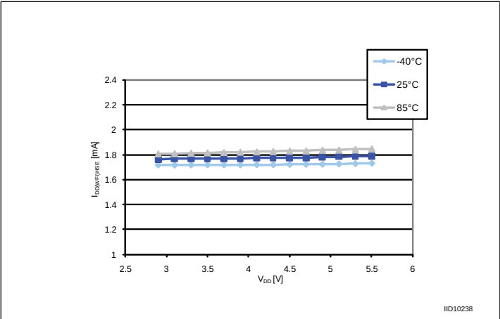
Figure 14: Typ. I_{DD(WFI)} vs. V_{DD} , HSE user external clock, f_{CPU} = 16\text{ MHz}
