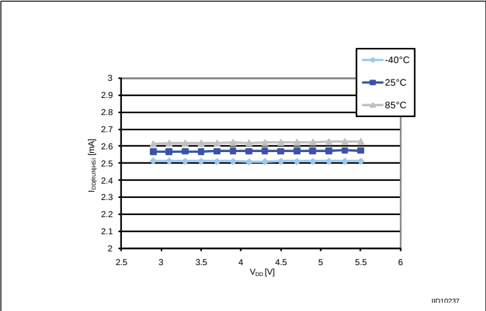
Figure 13: Typ. I_{DD(RUN)} vs. V_{DD} , HSI RC osc, f_{CPU} = 16\text{ MHz}
