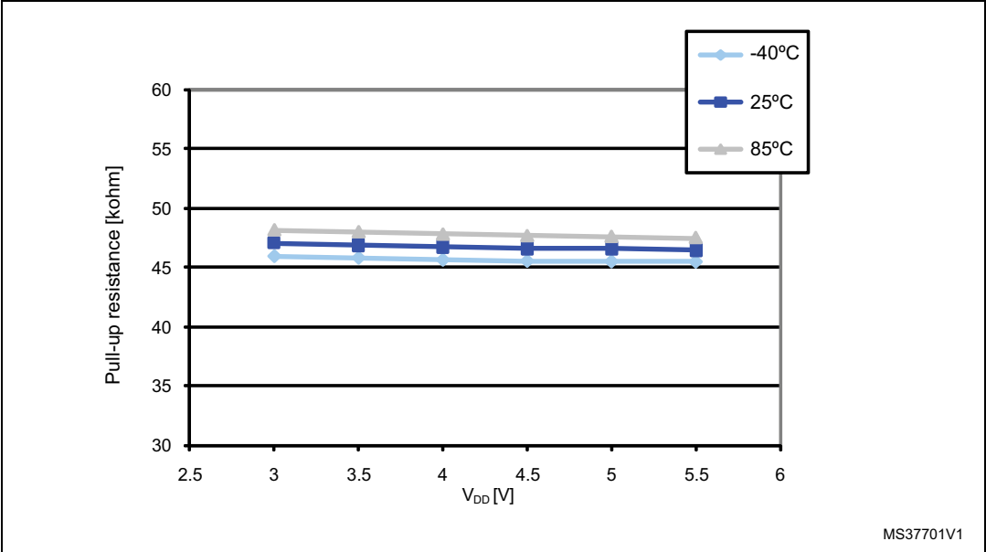
Figure 22. Typical pull-up resistance vs V_{DD} @ 3 temperatures
