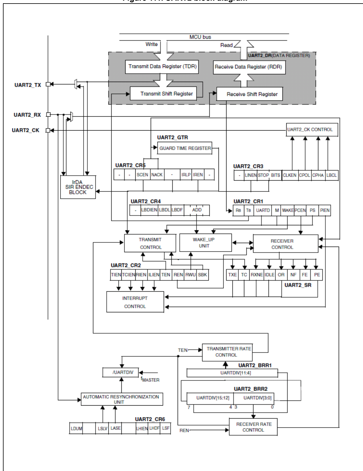
Figure 111. UART2 block diagram
