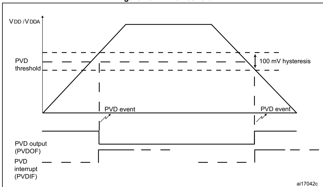
Figure 15. PVD threshold
