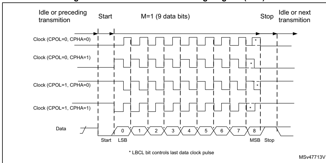
Figure 163. USART data clock timing diagram (M=1)
