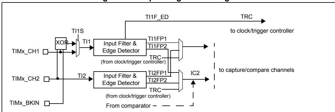
Figure 122. Input stage block diagram
