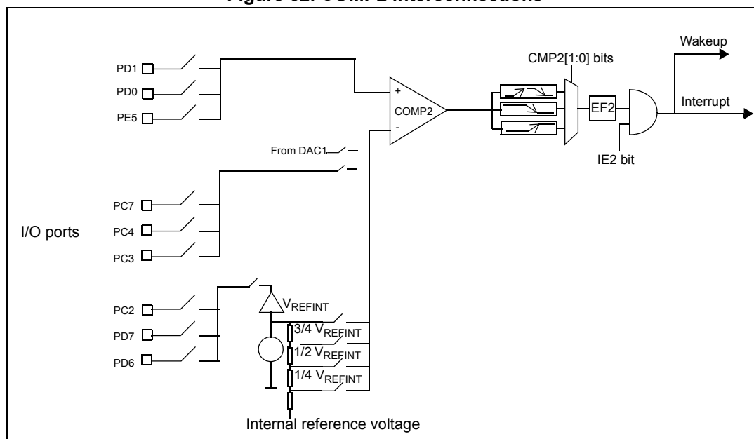
Figure 52. COMP2 interconnections
