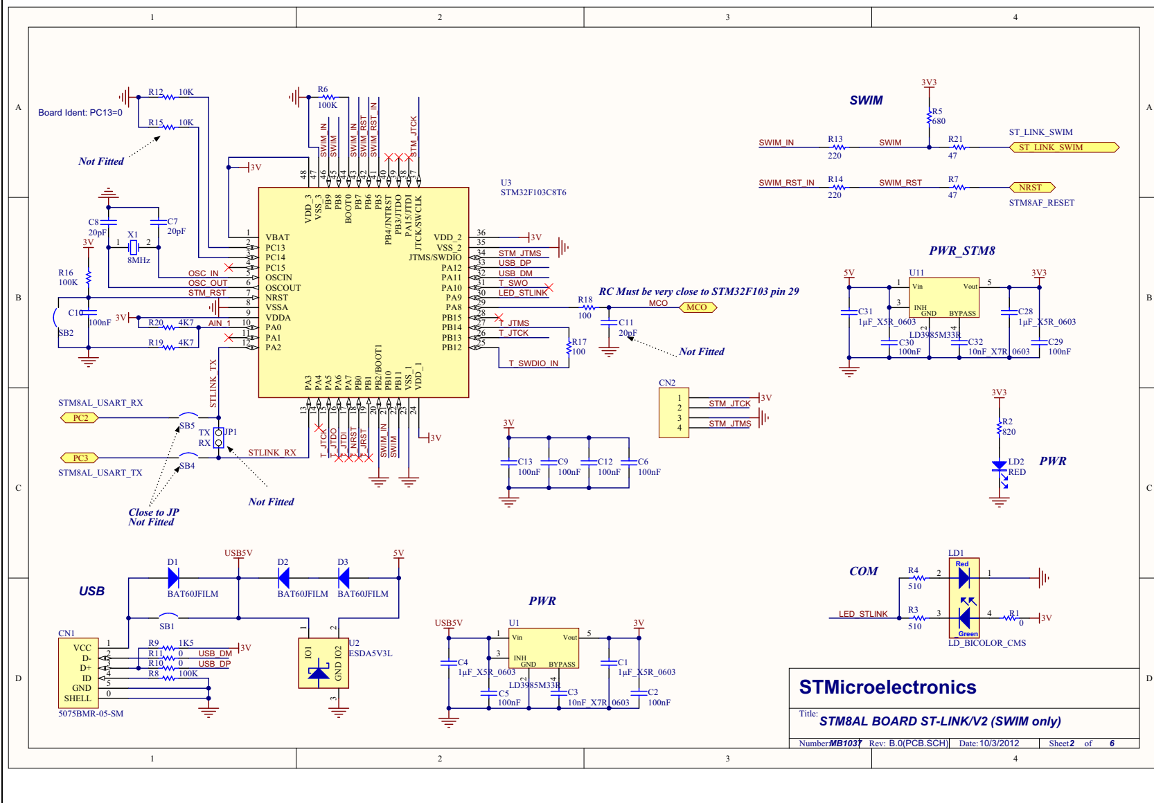
Figure 26. STM8AL board ST-LINK/V2 (SWIM only)
