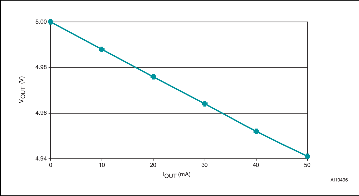
Figure 26. Output voltage vs. load current ( V_{\text{CC}} = 5 \text{ V} ; V_{\text{BAT}} = 2.8 \text{ V} ; T_{\text{A}} = 25^{\circ}\text{C} )
