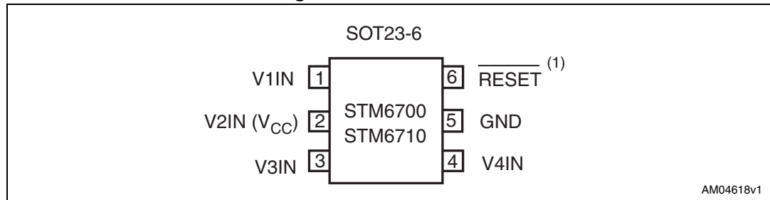
Figure 3. Pinout SOT23-6
