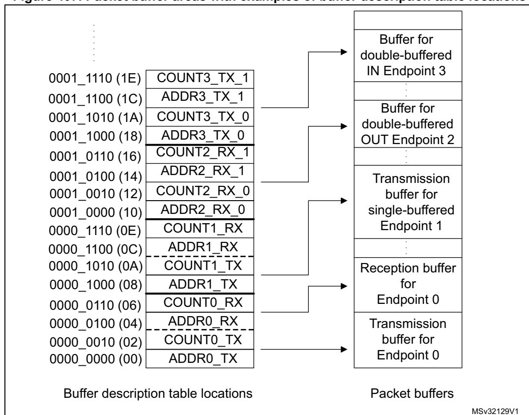
Figure 407. Packet buffer areas with examples of buffer description table locations
