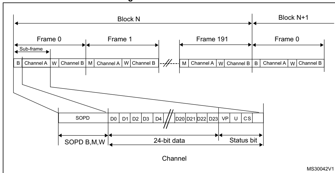
Figure 389. SPDIF format
