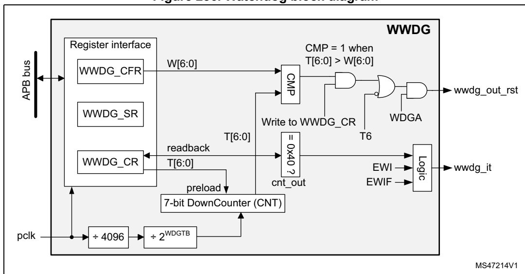
Figure 286. Watchdog block diagram
