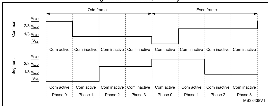
Figure 97. 1/3 bias, 1/4 duty
