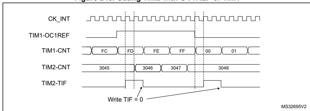
Figure 248. Gating TIM2 with OC1REF of TIM1
