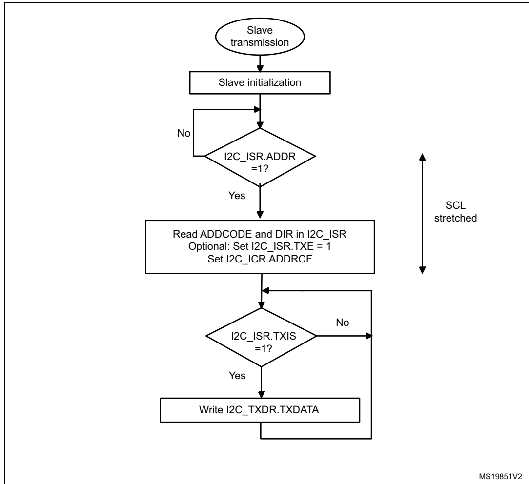
Figure 295. Transfer sequence flowchart for I2C slave transmitter, NOSTRETCH= 0
