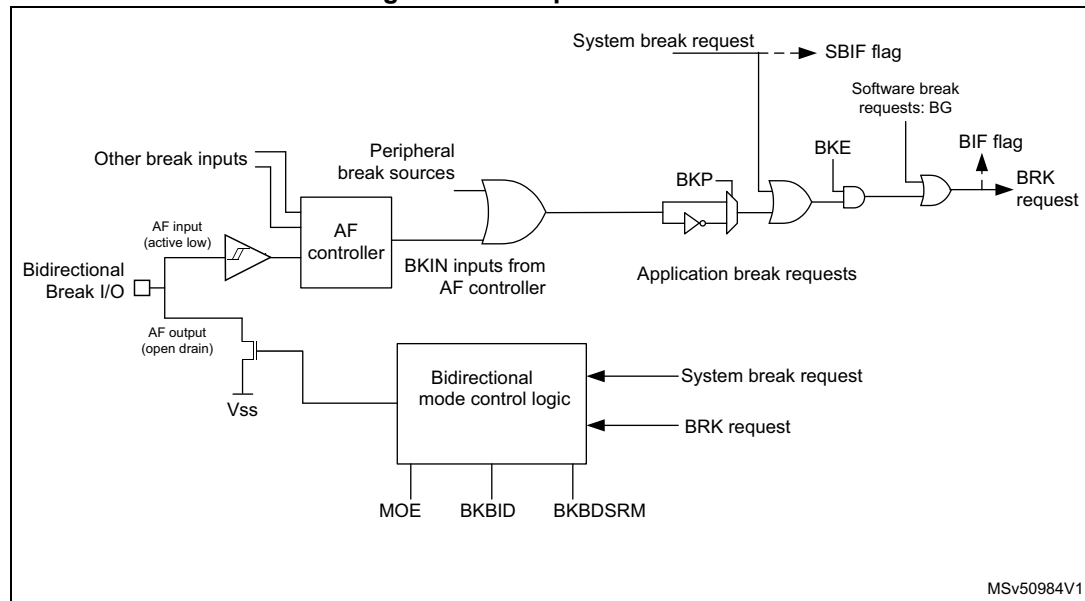
Figure 274. Output redirection
