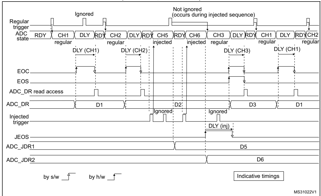
Figure 74. AUTODLY=1, regular HW conversions interrupted by injected conversions (DISCEN=1, JDISCEN=1)
