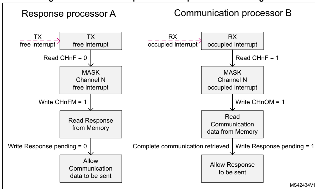
Figure 402. IPCC Half-duplex - Receive procedure state diagram
