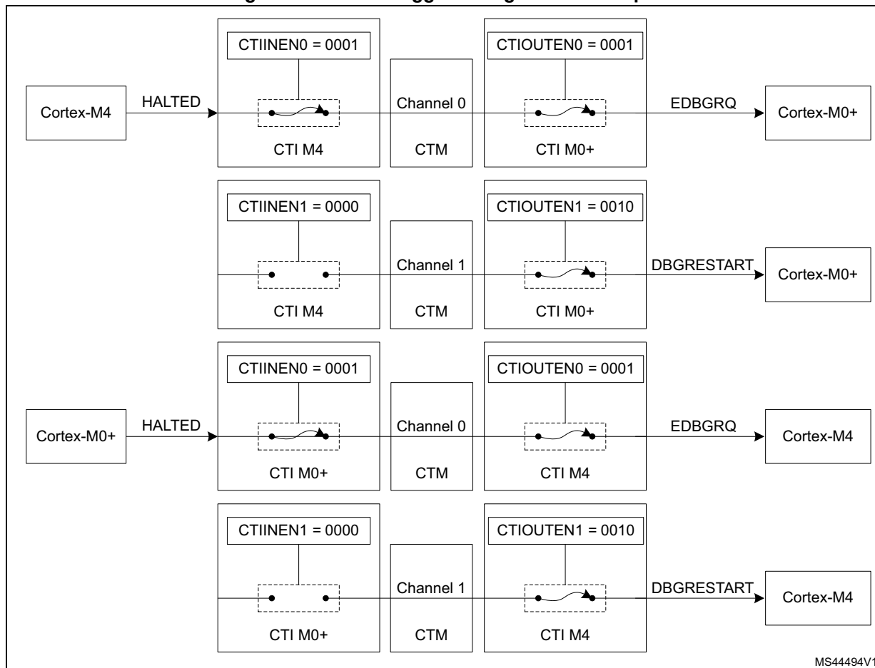
Figure 416. Cross trigger configuration example
