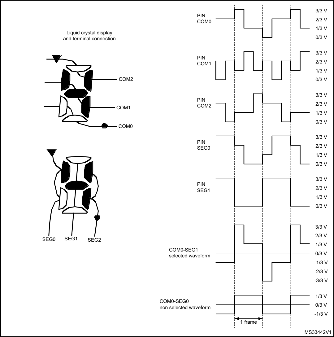
Figure 101. 1/3 duty, 1/3 bias
