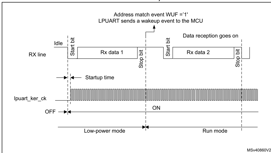
Figure 357. Wakeup event verified (wakeup event = address match, FIFO disabled)
