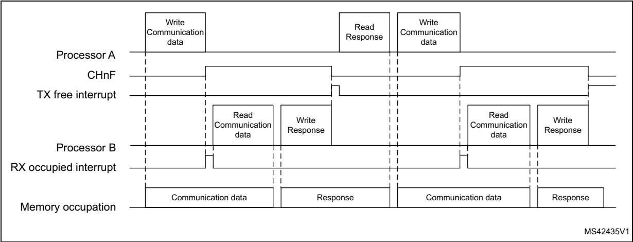
Figure 400. IPCC Half-duplex channel mode transfer timing
