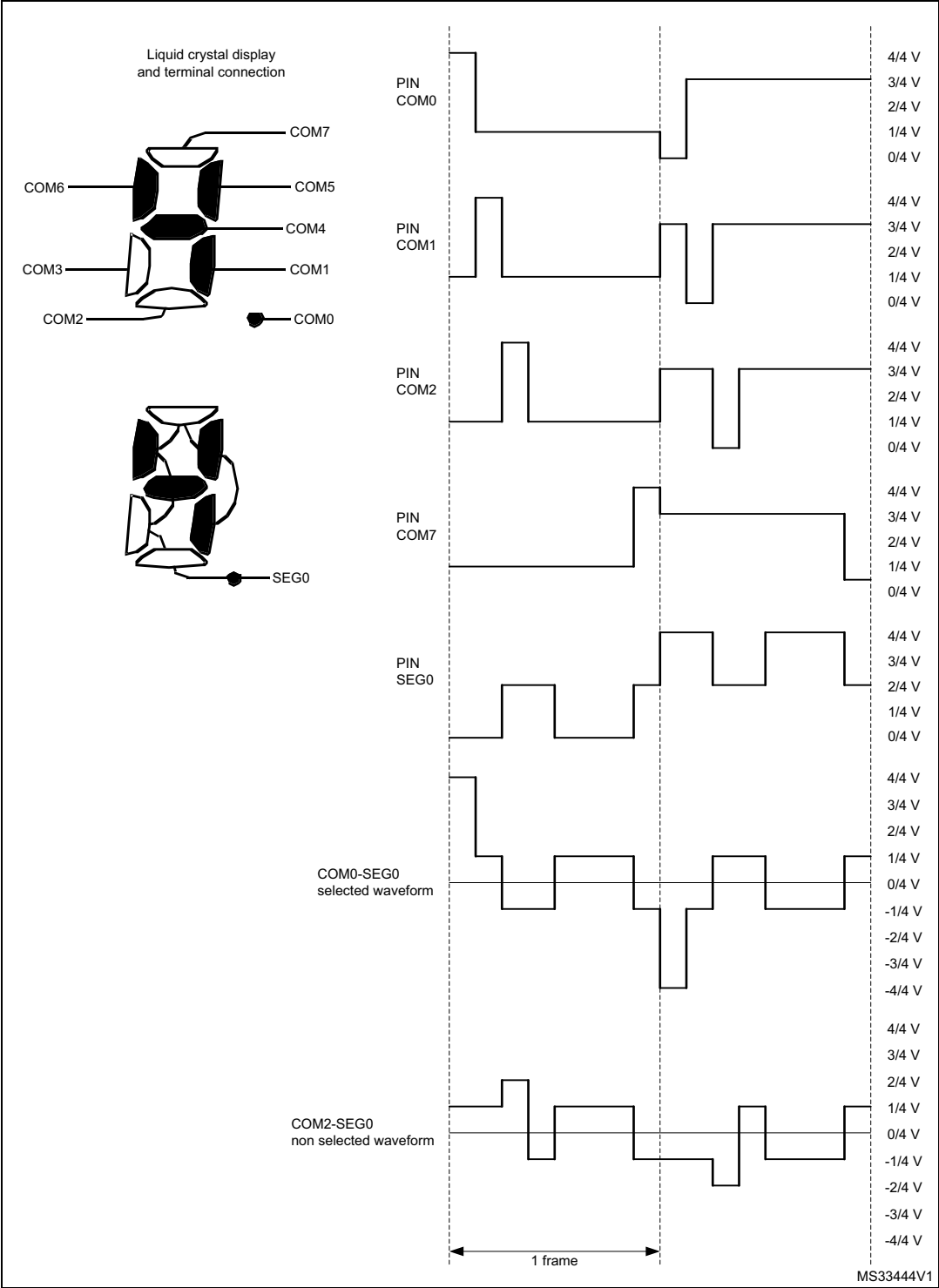
Figure 103. 1/8 duty, 1/4 bias
