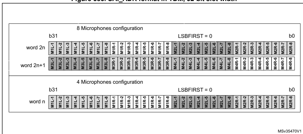
Figure 385. SAI_ADR format in TDM, 32-bit slot width
