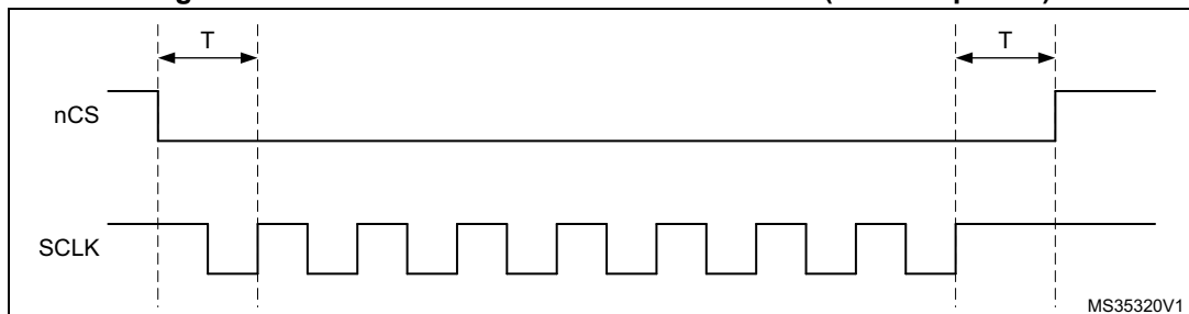
Figure 37. nCS when CKMODE = 1 in SDR mode (T = CLK period)
