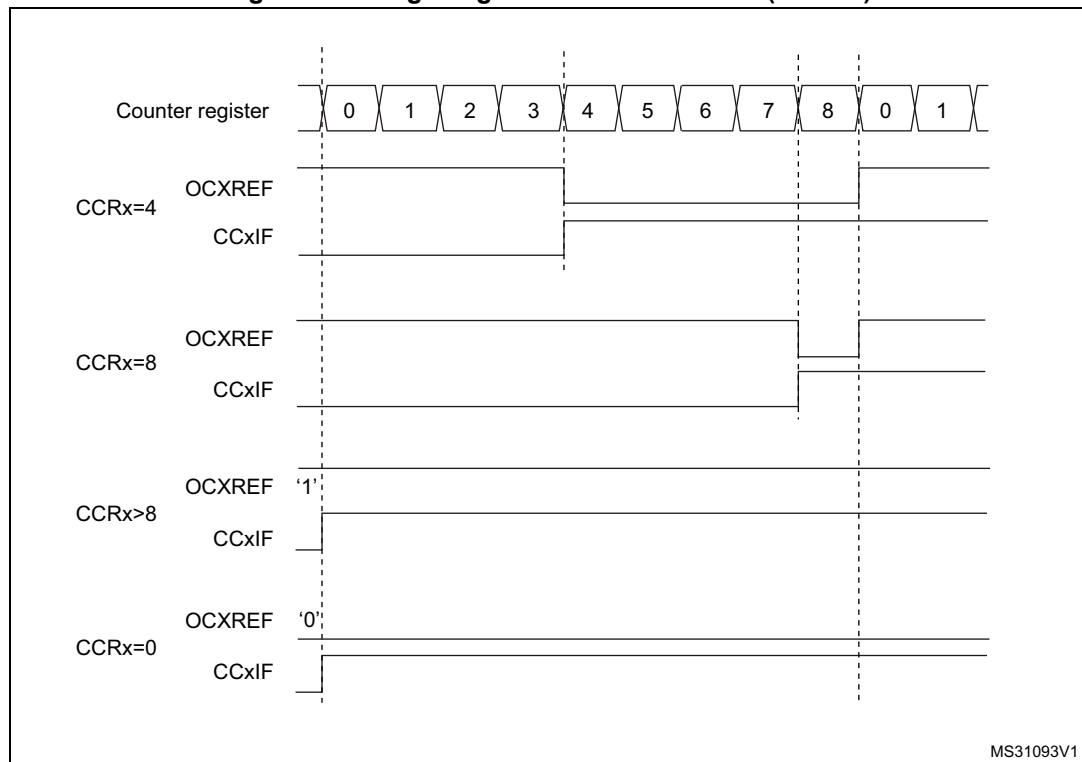
Figure 269. Edge-aligned PWM waveforms (ARR=8)
