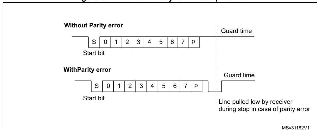
Figure 334. ISO 7816-3 asynchronous protocol
