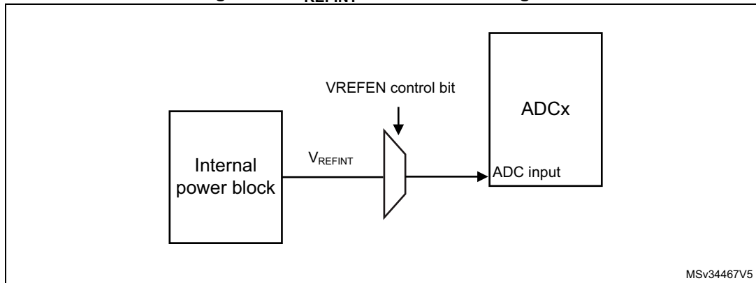
Figure 91. V_{REFINT} channel block diagram
