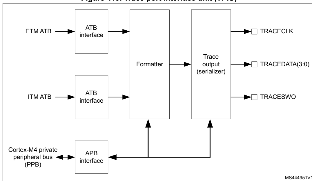
Figure 419. Trace port interface unit (TPIU)
