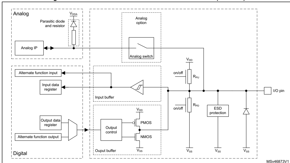
Figure 20. Three-volt or five-volt tolerant GPIO structure (TT or FT)
