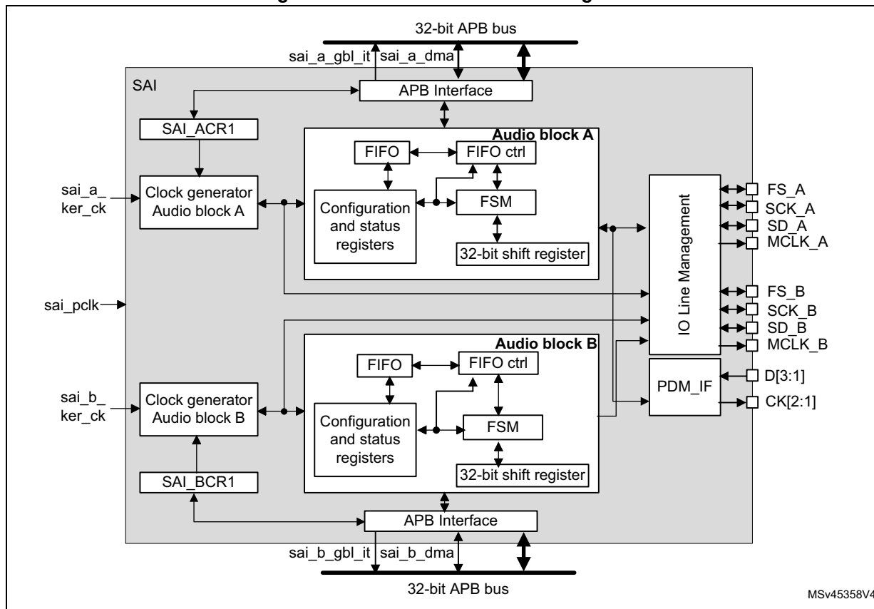
Figure 375. SAI functional block diagram
