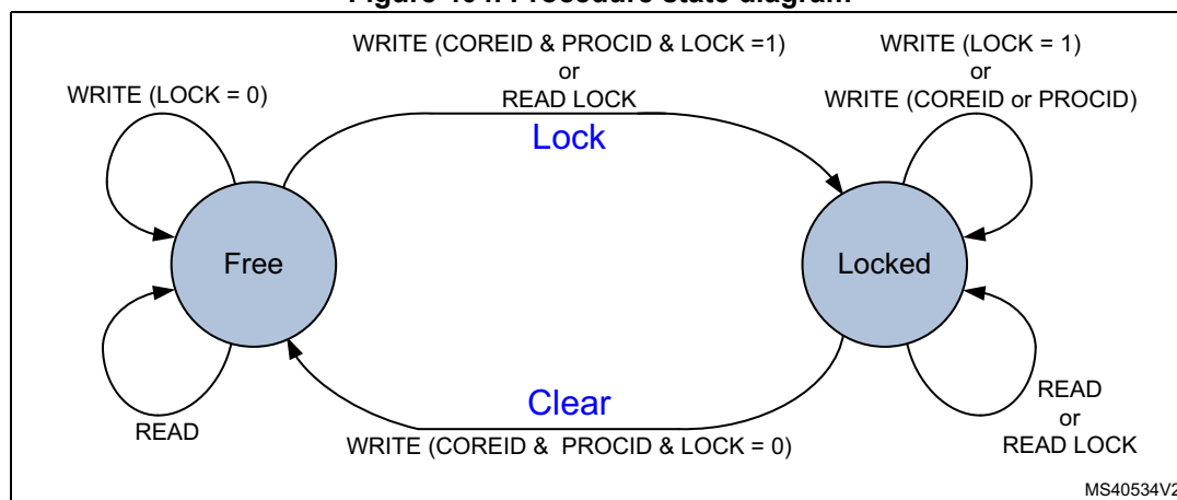
Figure 404. Procedure state diagram
