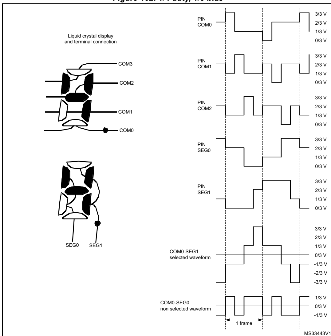
Figure 102. 1/4 duty, 1/3 bias
