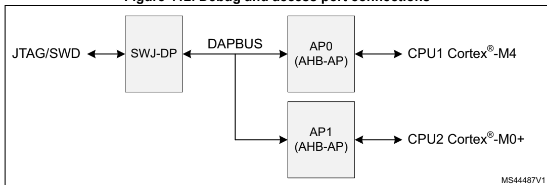
Figure 412. Debug and access port connections
