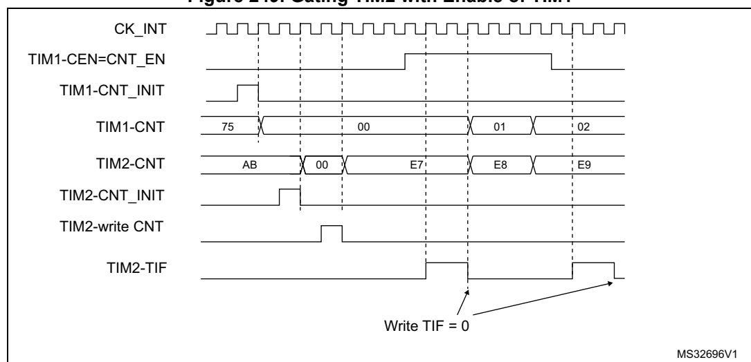
Figure 249. Gating TIM2 with Enable of TIM1
