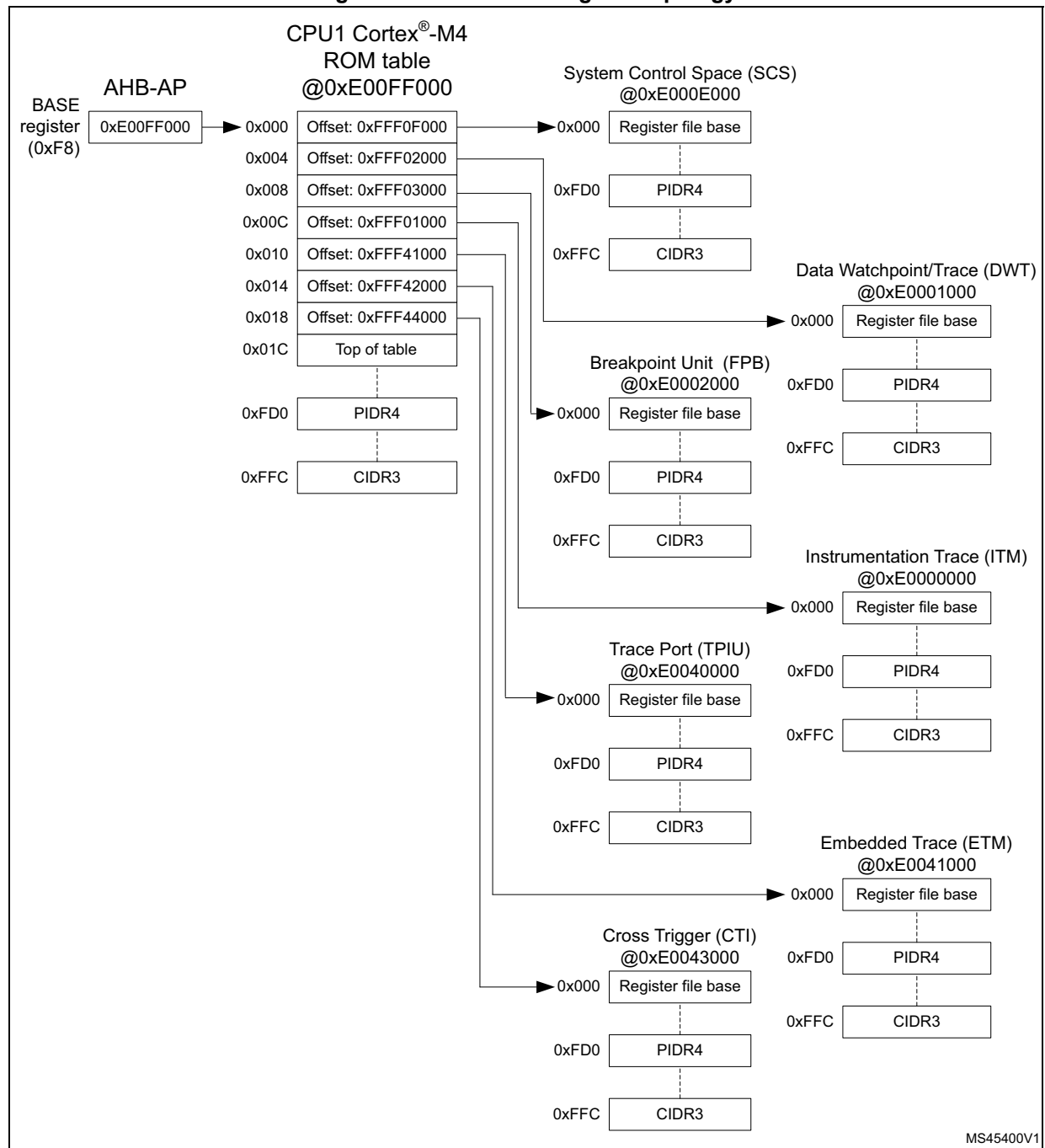
Figure 418. CPU1 CoreSight™ topology
