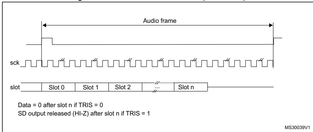
Figure 378. FS role is start of frame (FSDEF = 0)
