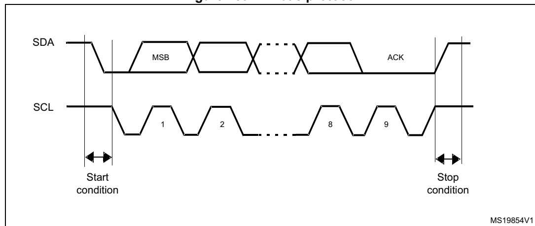
Figure 289. I 2 C bus protocol
