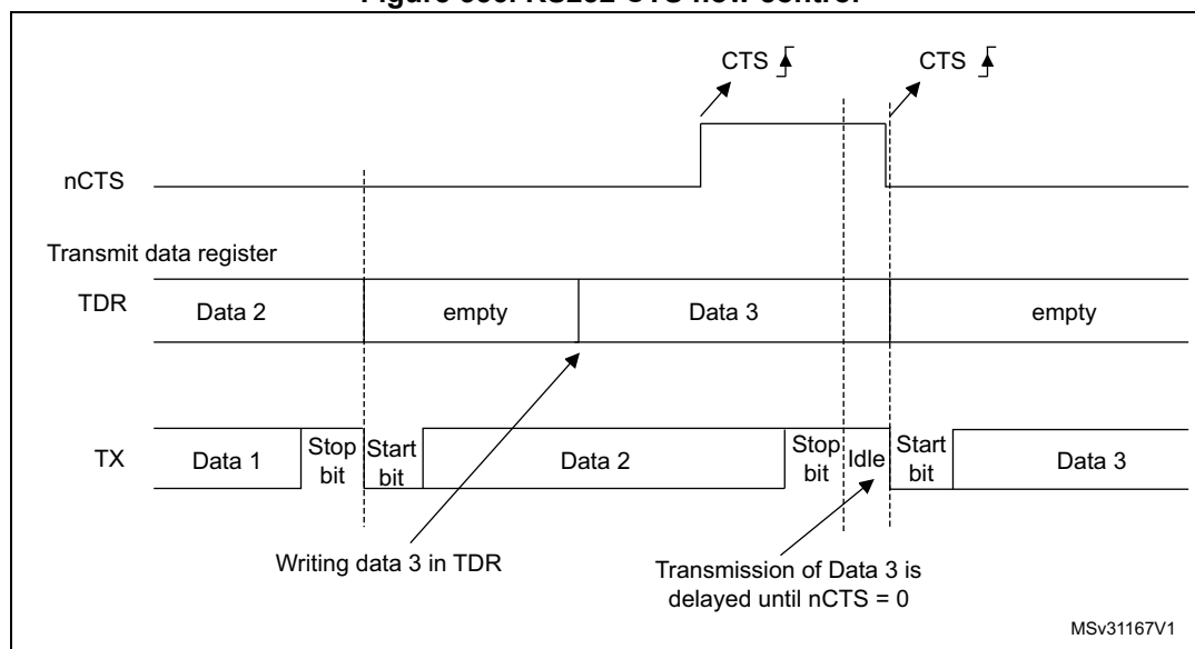
Figure 356. RS232 CTS flow control
