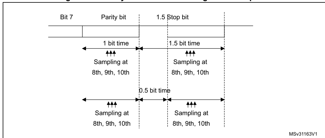
Figure 335. Parity error detection using the 1.5 stop bits
