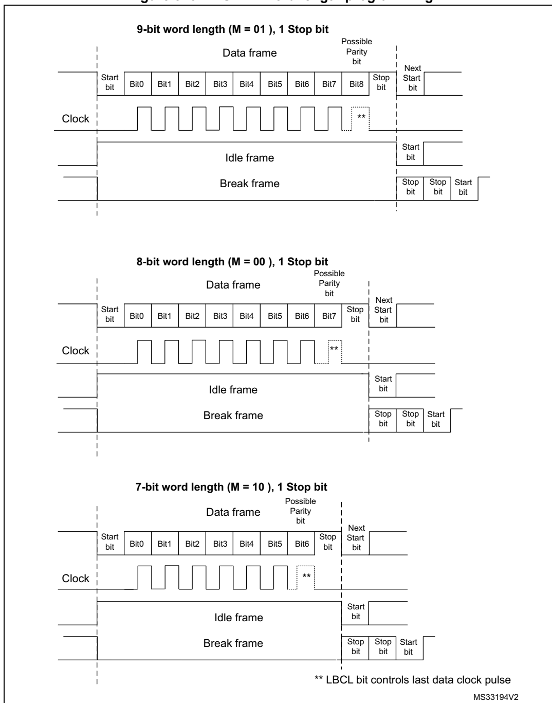
Figure 346. LPUART word length programming
