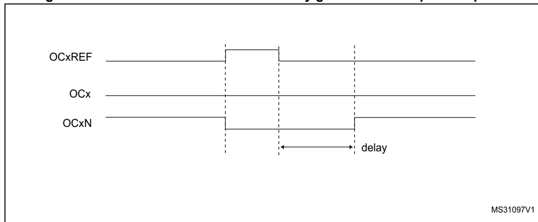
Figure 272. Dead-time waveforms with delay greater than the positive pulse.
