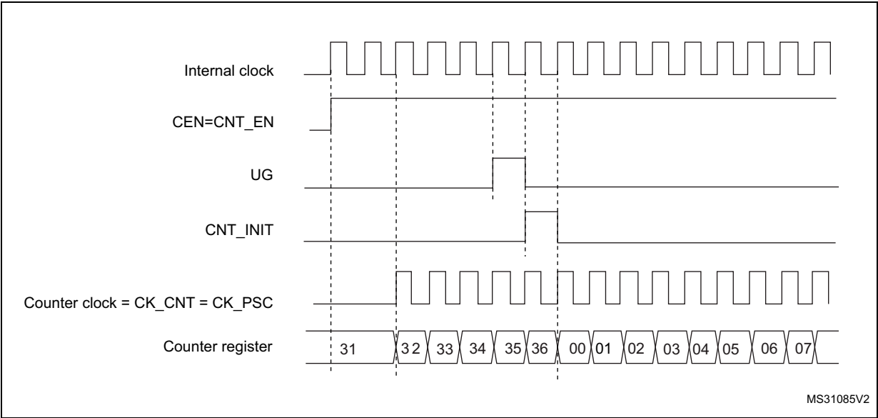
Figure 262. Control circuit in normal mode, internal clock divided by 1
