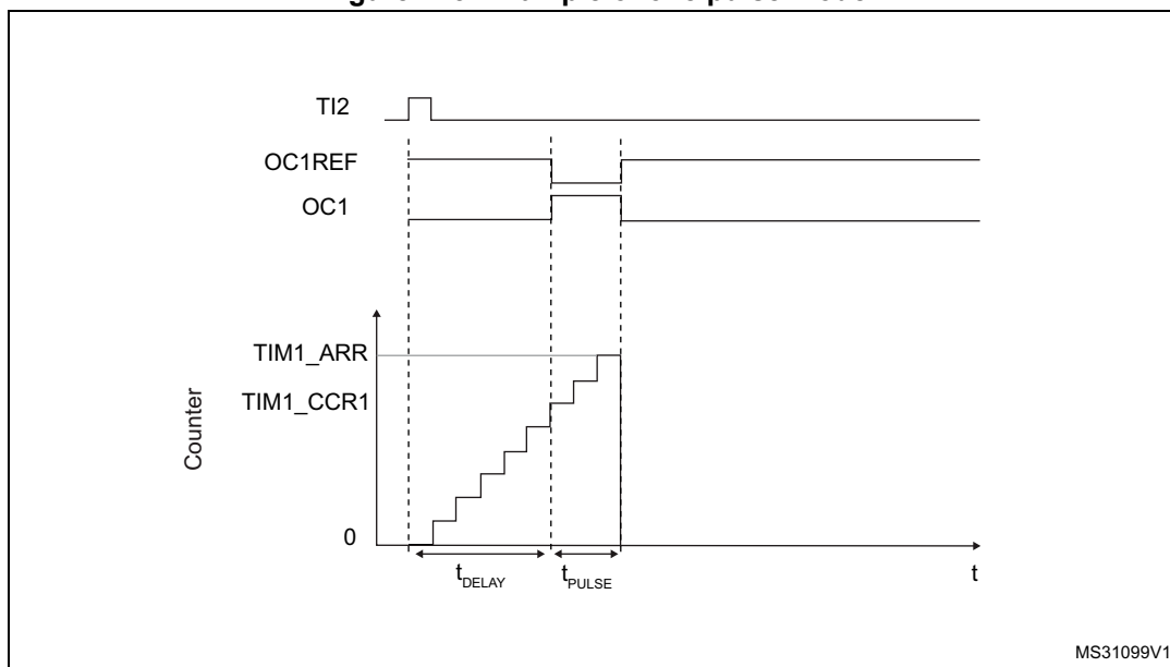
Figure 275. Example of one pulse mode
