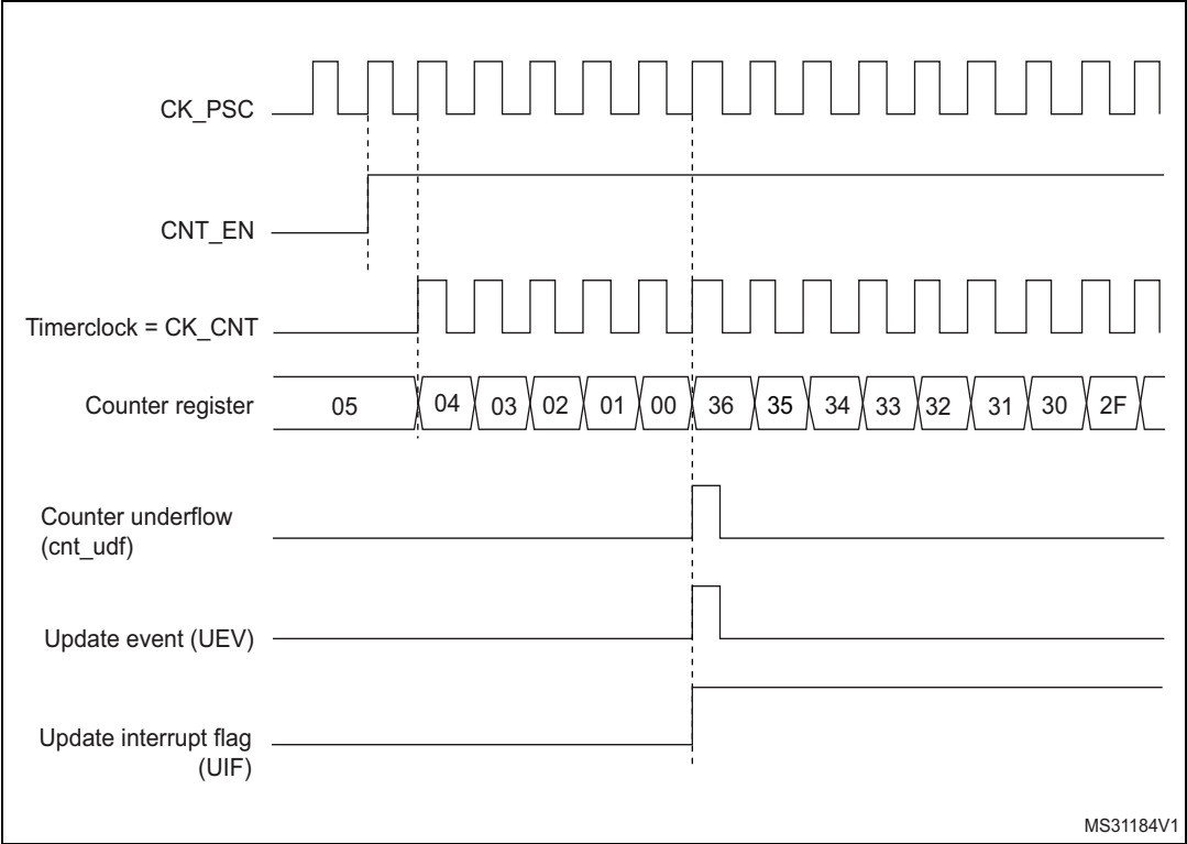
Figure 153. Counter timing diagram, internal clock divided by 1
