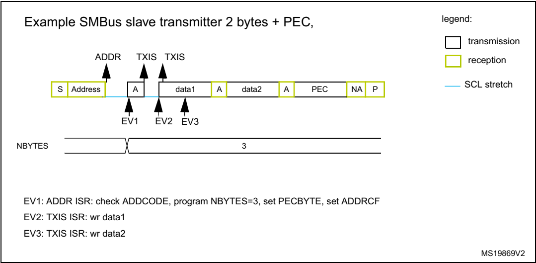
Figure 313. Transfer bus diagrams for SMBus slave transmitter (SBC=1)
