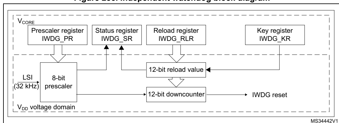
Figure 285. Independent watchdog block diagram
