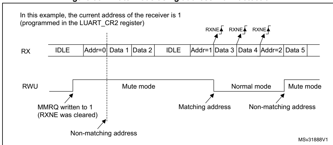
Figure 351. Mute mode using address mark detection
