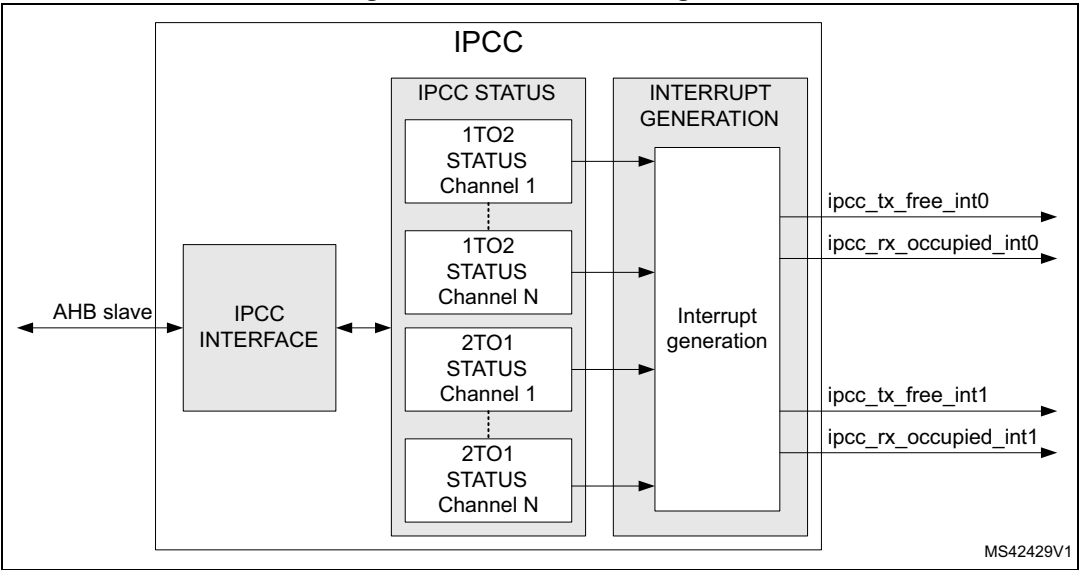
Figure 396. IPCC block diagram
