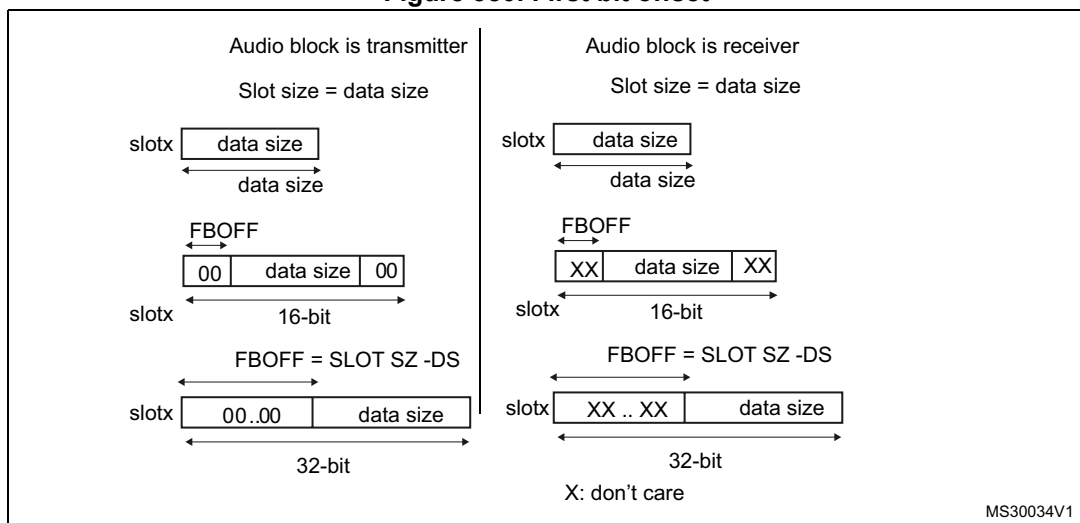
Figure 380. First bit offset
