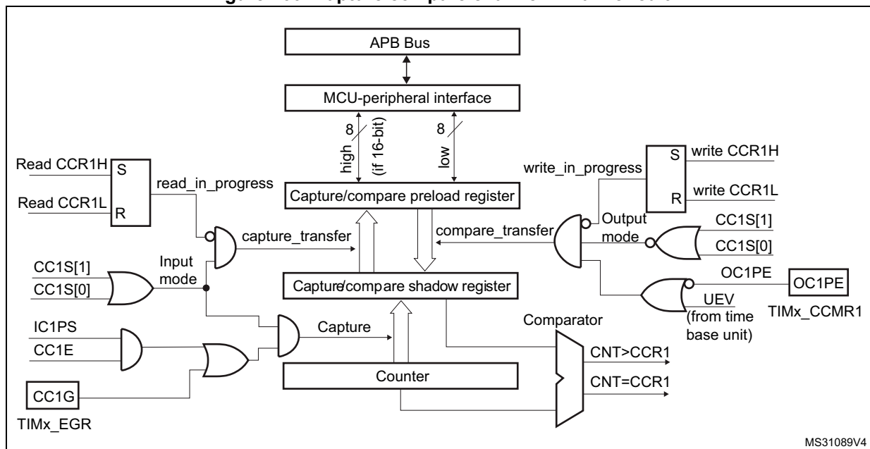
Figure 266. Capture/compare channel 1 main circuit
