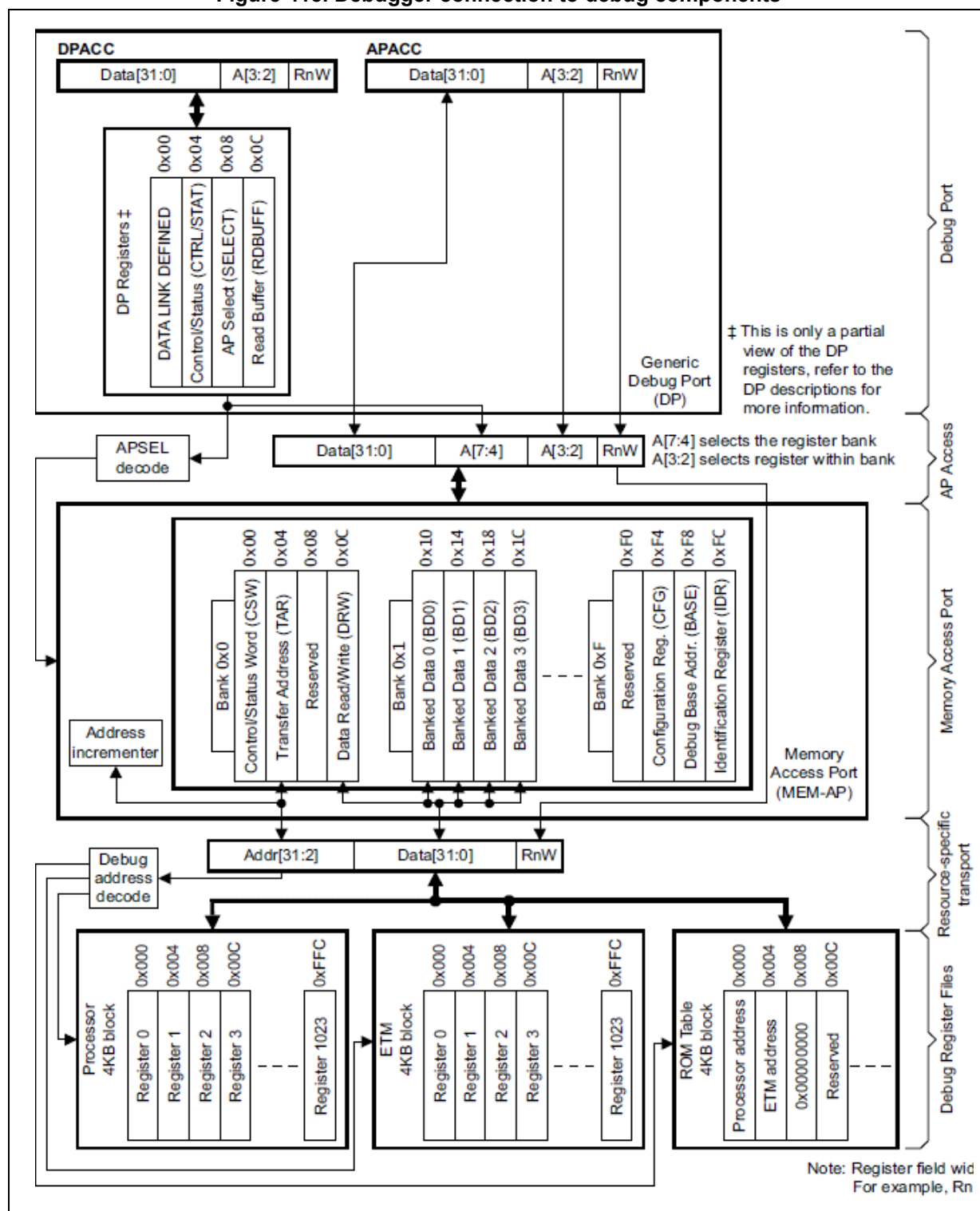
Figure 413. Debugger connection to debug components
