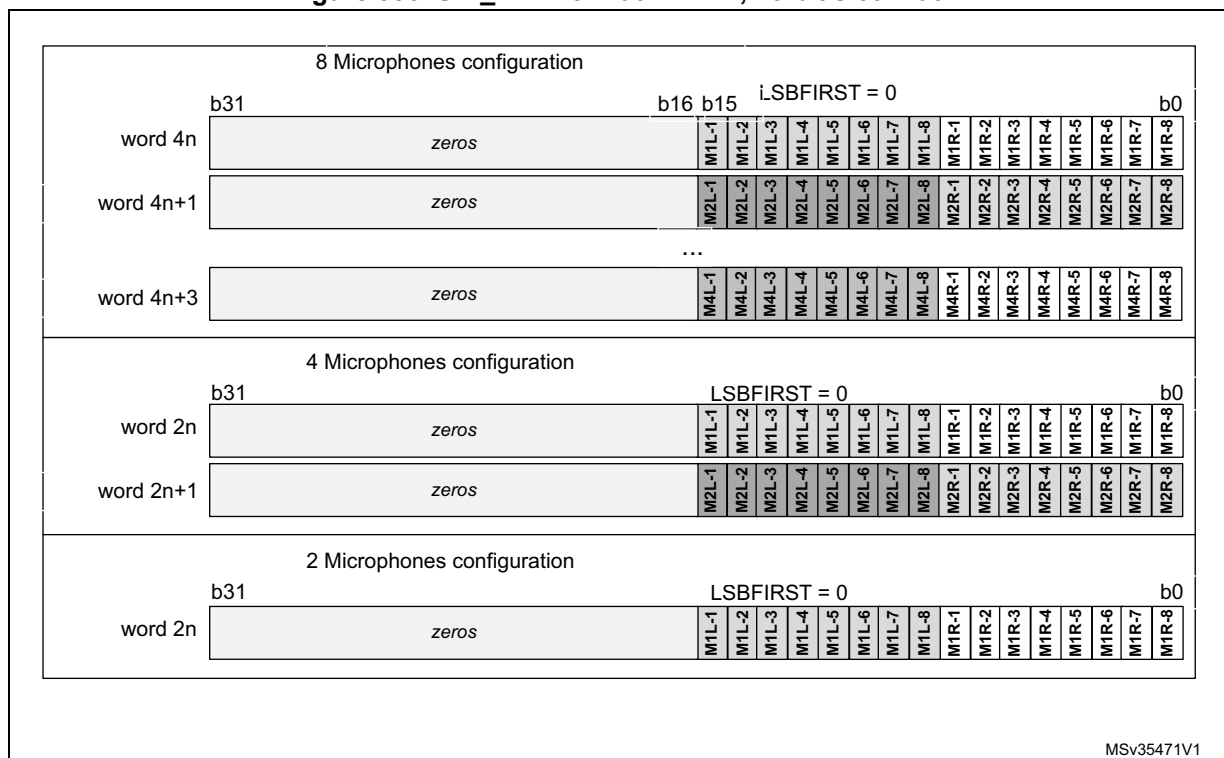
Figure 386. SAI_ADR format in TDM, 16-bit slot width
