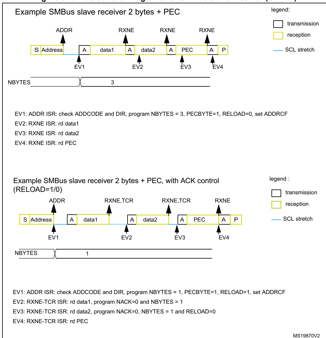
Figure 315. Bus transfer diagrams for SMBus slave receiver (SBC=1)
