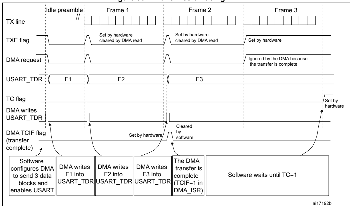
Figure 352. Transmission using DMA
