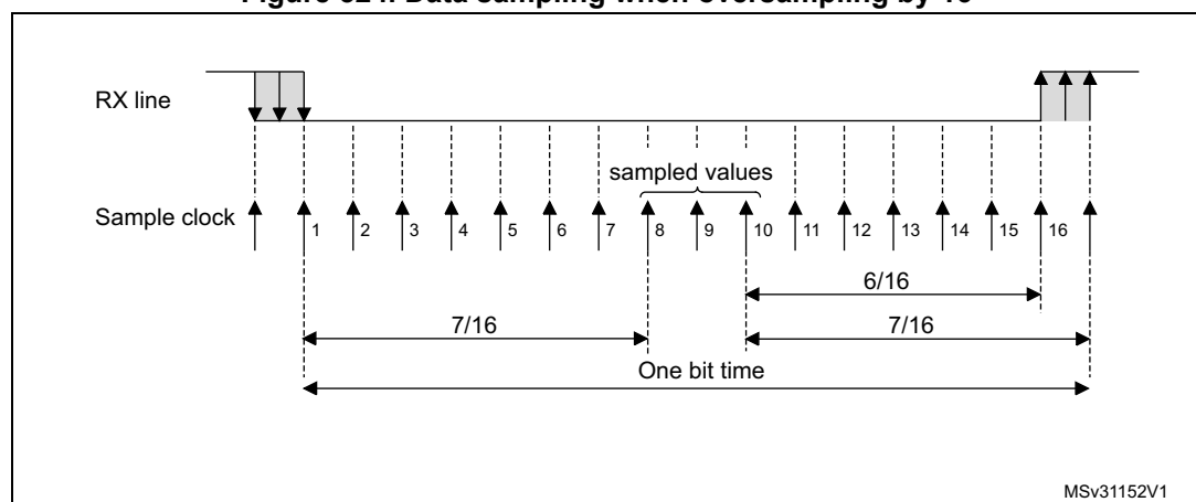
Figure 324. Data sampling when oversampling by 16
