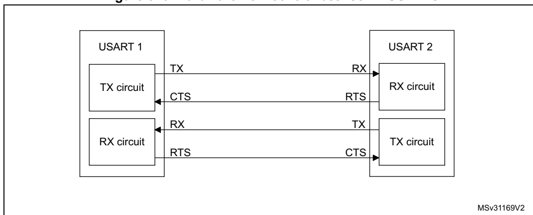
Figure 340. Hardware flow control between 2 USARTs
