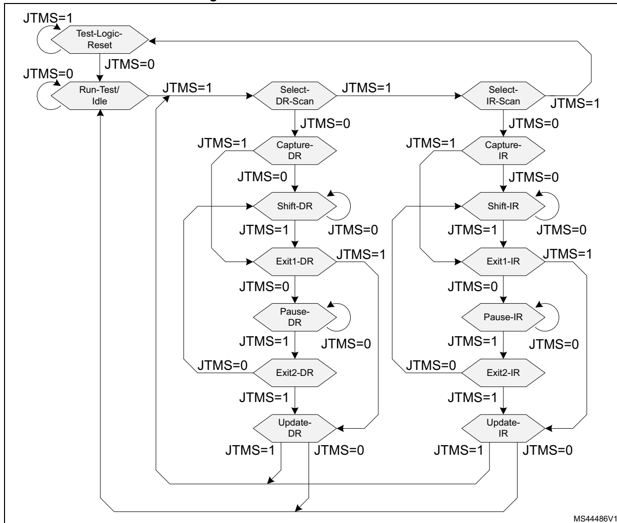
Figure 411. JTAG TAP state machine
