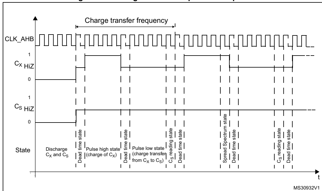
Figure 111. Charge transfer acquisition sequence
