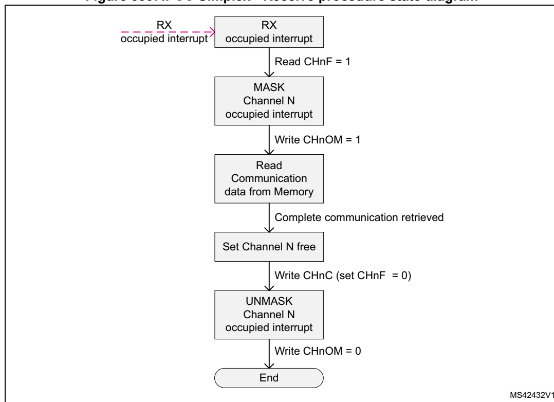
Figure 399. IPCC Simplex - Receive procedure state diagram
