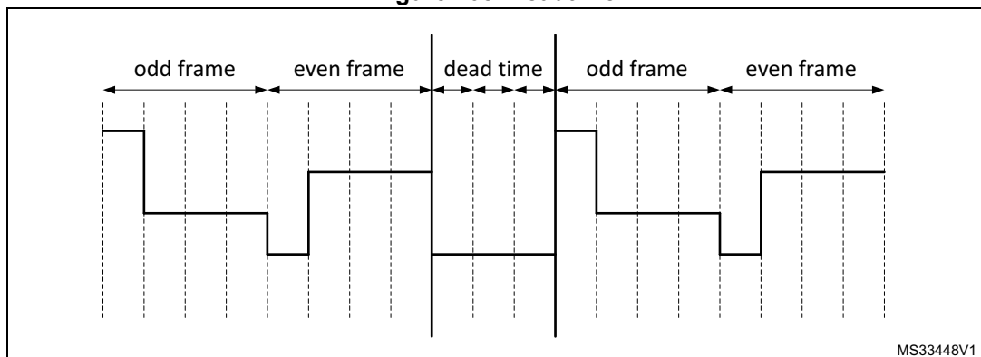
Figure 105. Deadtime
