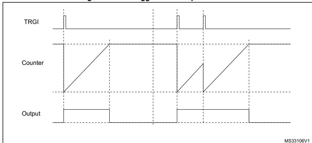
Figure 240. Retriggerable one-pulse mode.
