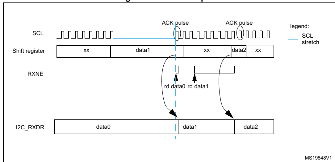
Figure 292. Data reception
