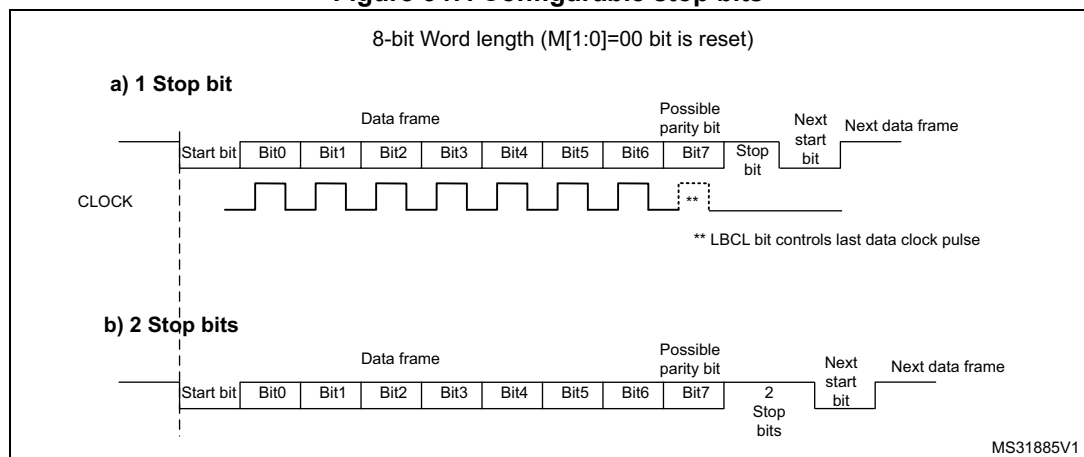
Figure 347. Configurable stop bits
