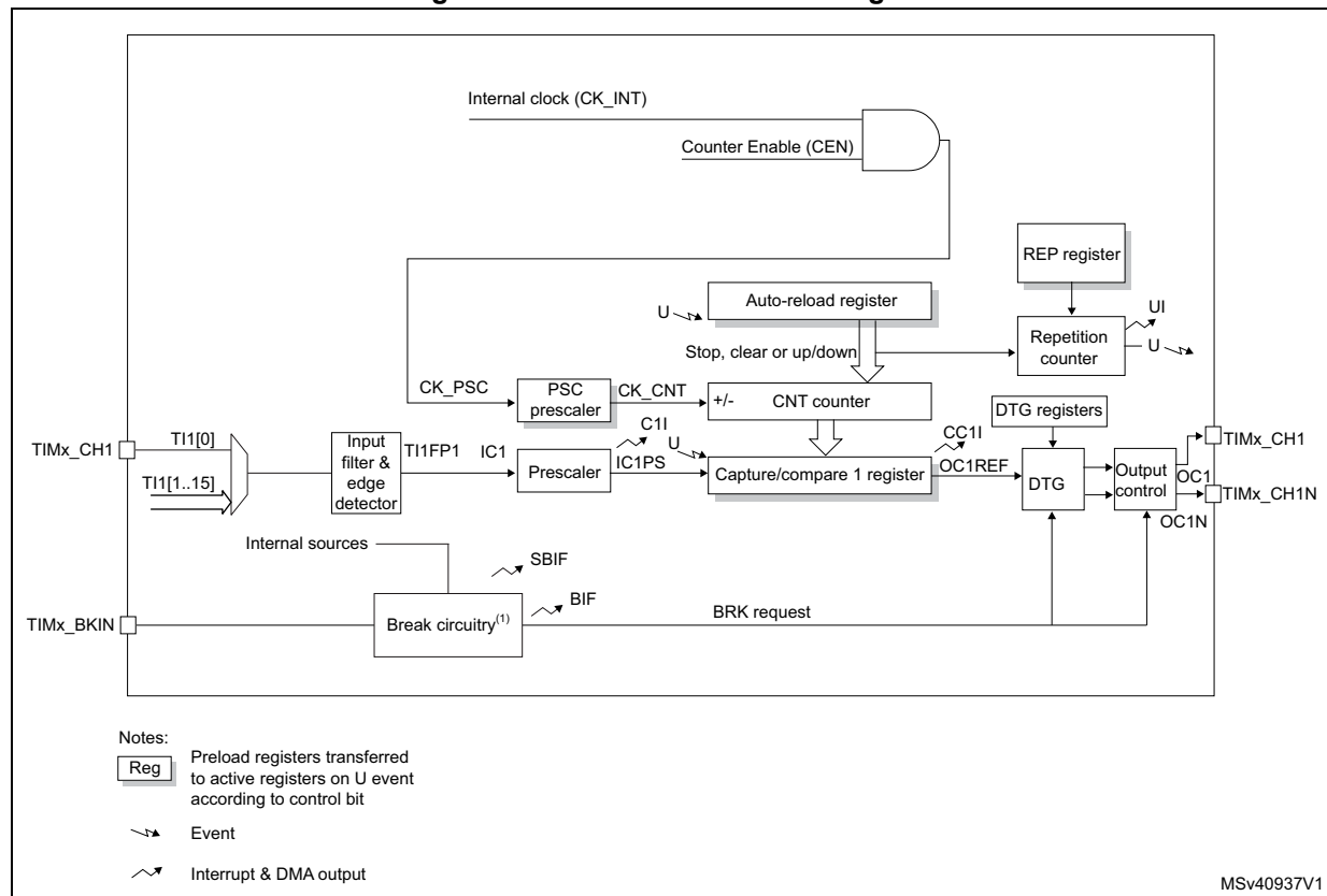
Figure 252. TIM16/TIM17 block diagram
