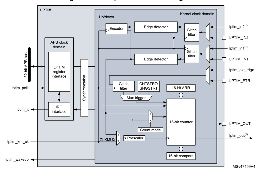
Figure 276. Low-power timer block diagram
