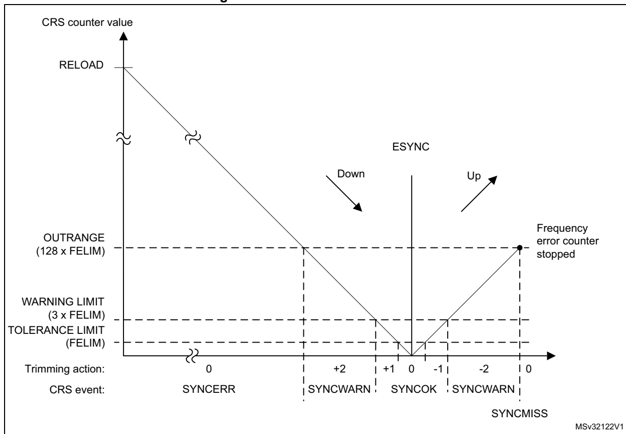
Figure 409. CRS counter behavior
