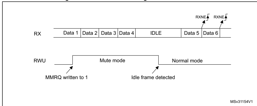
Figure 350. Mute mode using Idle line detection
