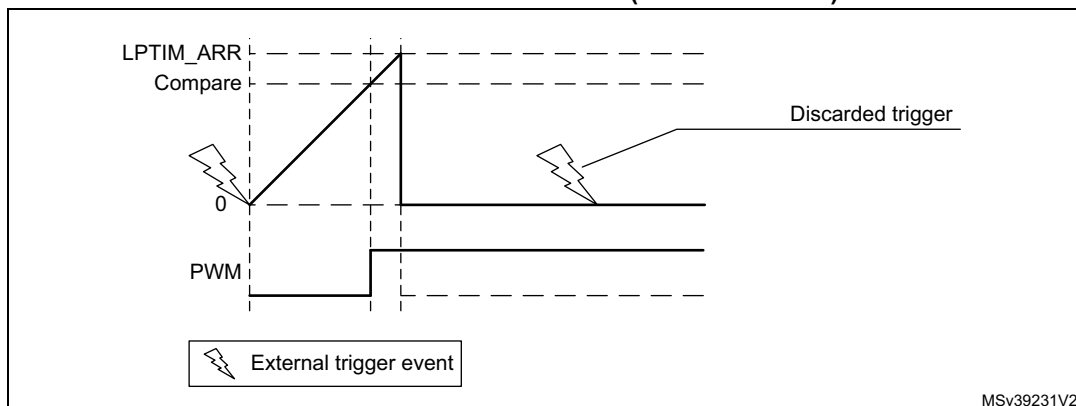
Figure 279. LPTIM output waveform, Single counting mode configuration and Set-once mode activated (WAVE bit is set)
