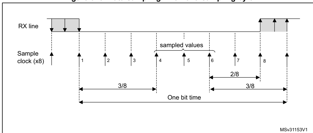
Figure 325. Data sampling when oversampling by 8
