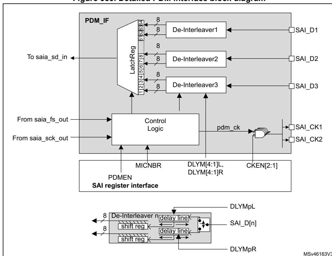
Figure 383. Detailed PDM interface block diagram
