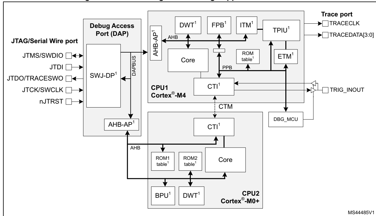
Figure 410. Block diagram of debug support infrastructure
