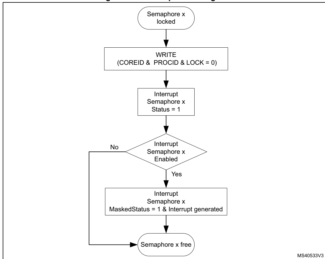
Figure 405. Interrupt state diagram
