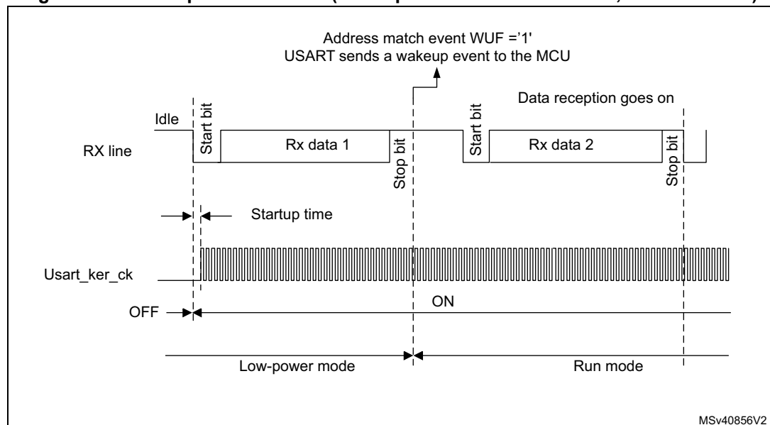
Figure 343. Wakeup event verified (wakeup event = address match, FIFO disabled)
