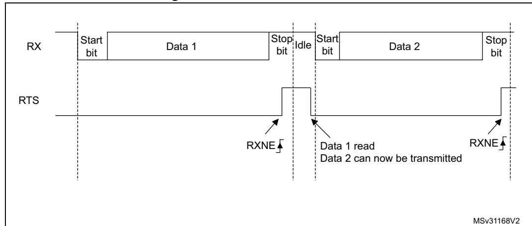
Figure 341. RS232 RTS flow control
