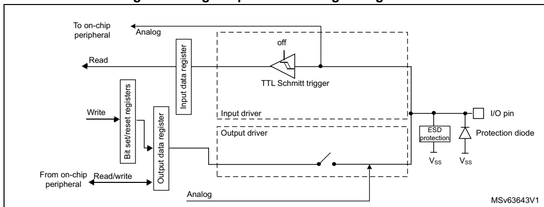
Figure 24. High impedance-analog configuration
