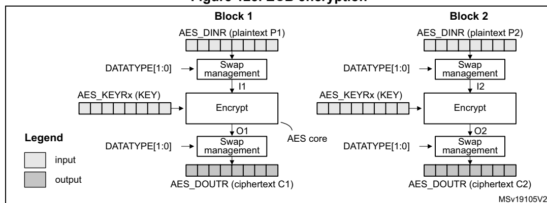
Figure 125. ECB encryption
