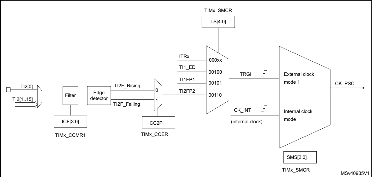
Figure 263. TI2 external clock connection example
