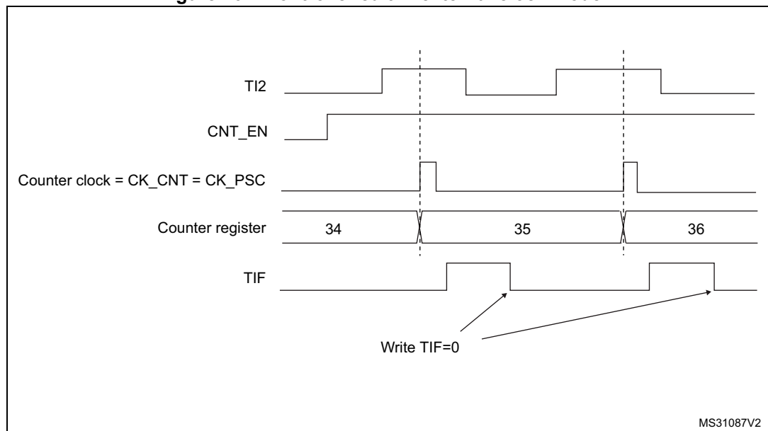
Figure 264. Control circuit in external clock mode 1
