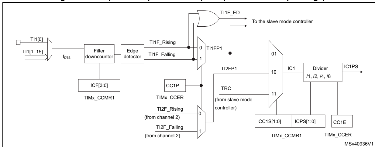
Figure 265. Capture/compare channel (example: channel 1 input stage)
