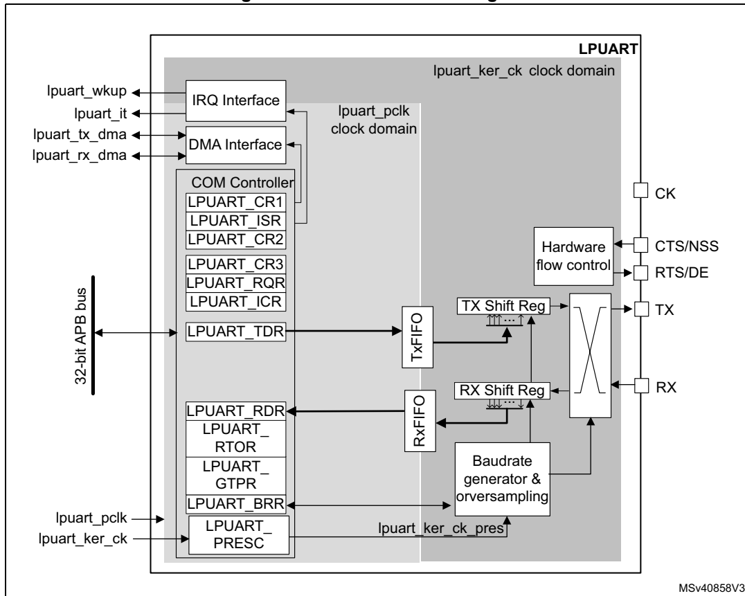
Figure 345. LPUART block diagram
