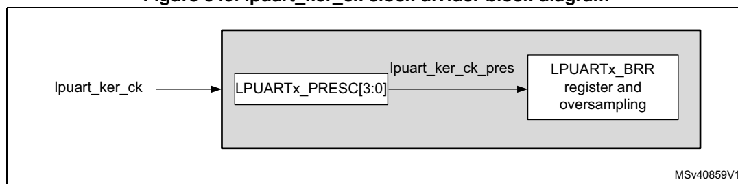
Figure 349. lpuart_ker_ck clock divider block diagram
