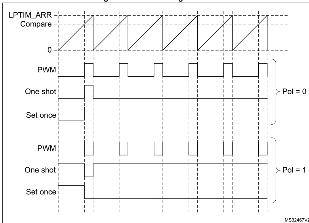
Figure 281. Waveform generation
