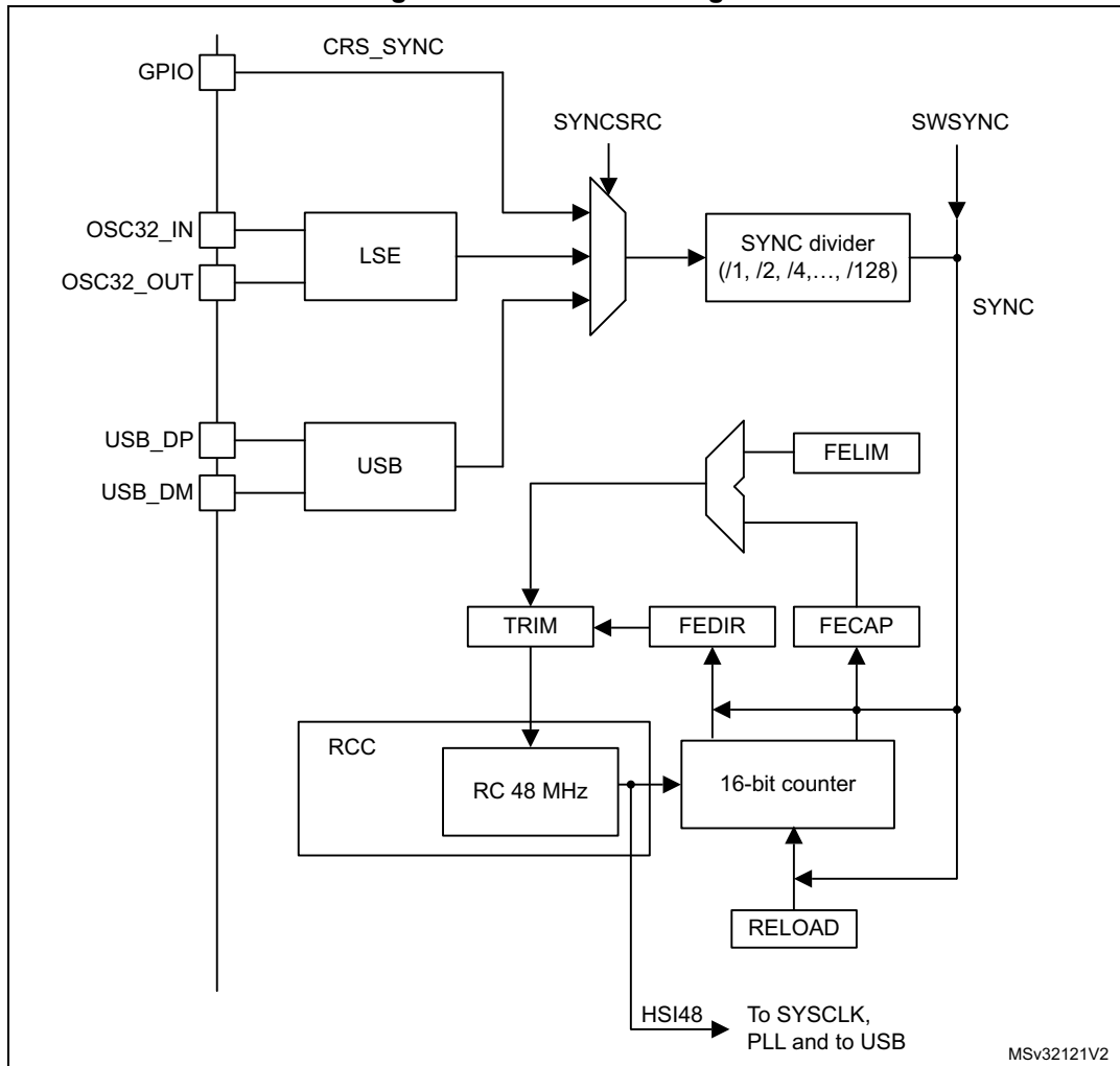
Figure 408. CRS block diagram
