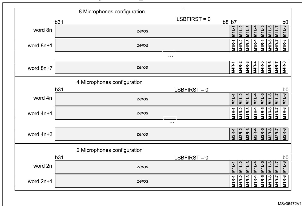
Figure 387. SAI_ADR format in TDM, 8-bit slot width
