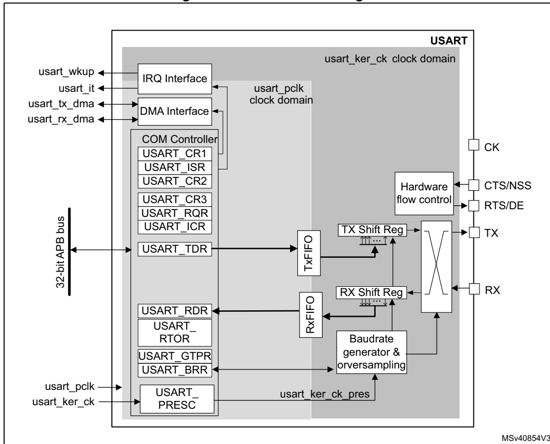
Figure 318. USART block diagram
