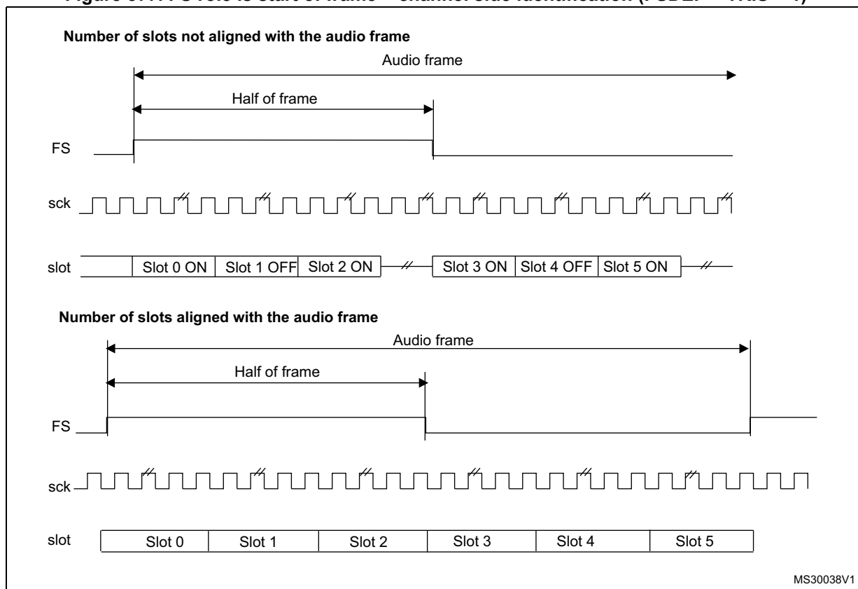
Figure 377. FS role is start of frame + channel side identification (FSDEF = TRIS = 1)
