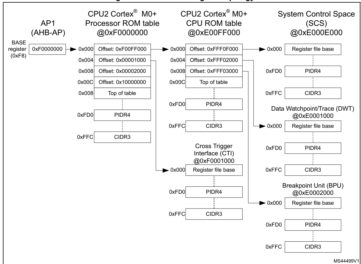
Figure 417. CPU2 CoreSight™ topology
