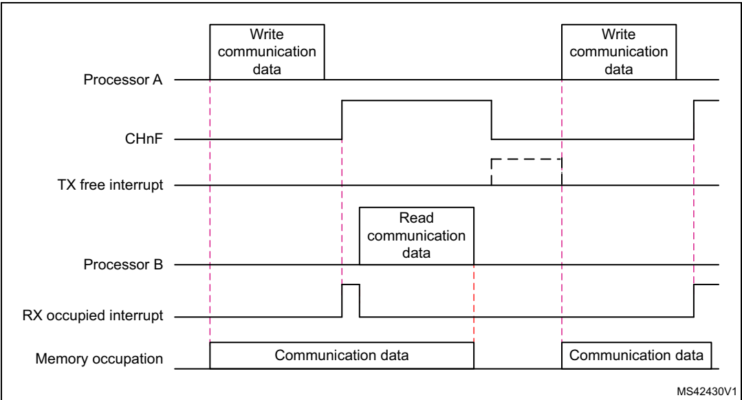
Figure 397. IPCC Simplex channel mode transfer timing
