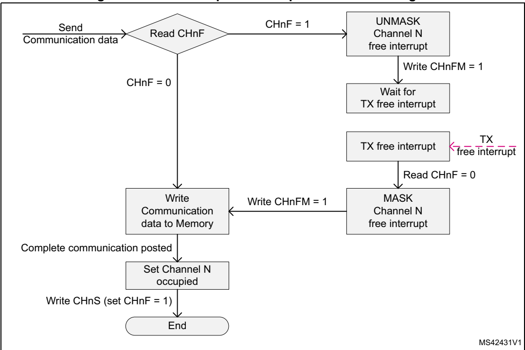
Figure 398. IPCC Simplex - Send procedure state diagram
