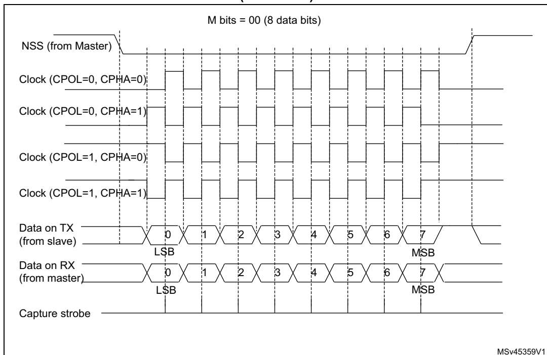
Figure 333. USART data clock timing diagram in synchronous slave mode (M bits = 00)
