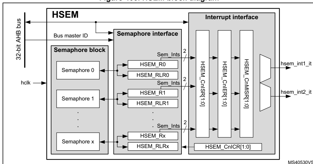
Figure 403. HSEM block diagram
