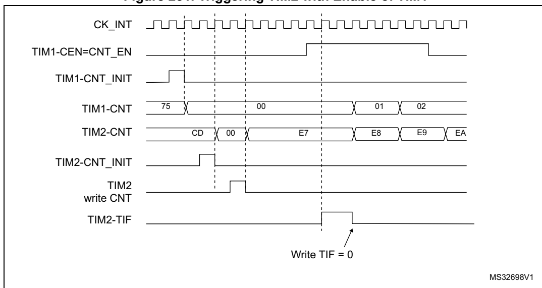
Figure 251. Triggering TIM2 with Enable of TIM1
