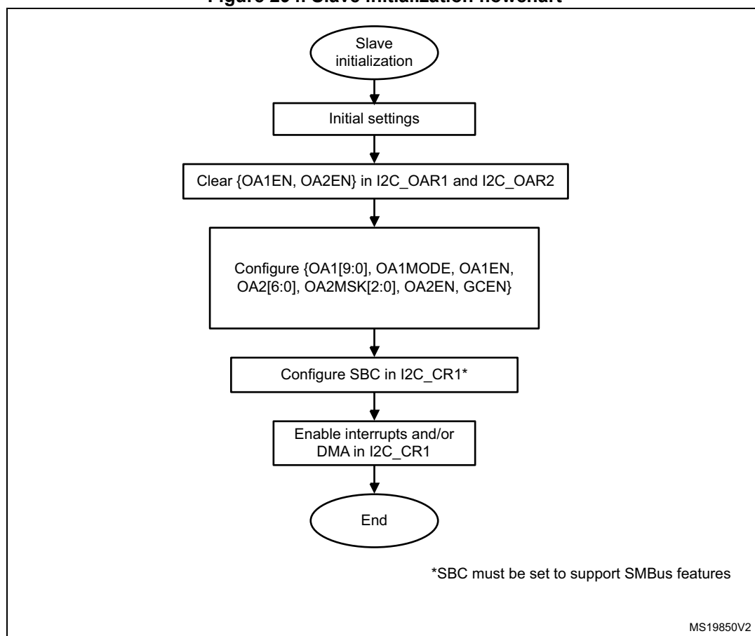
Figure 294. Slave initialization flowchart
