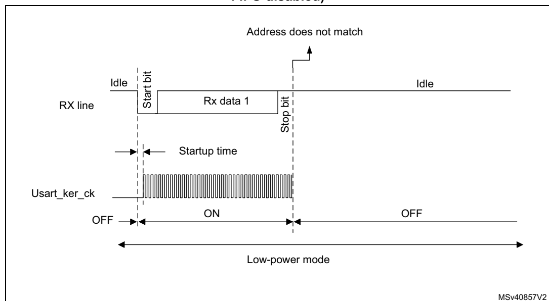
Figure 344. Wakeup event not verified (wakeup event = address match, FIFO disabled)
