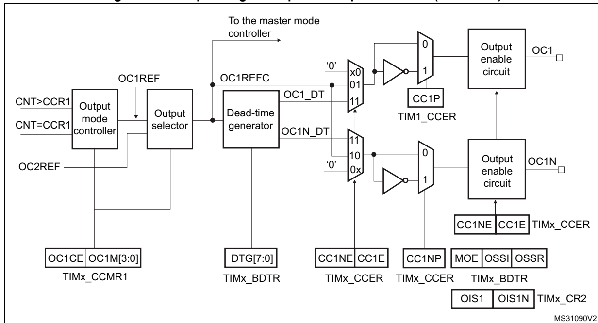
Figure 267. Output stage of capture/compare channel (channel 1)
