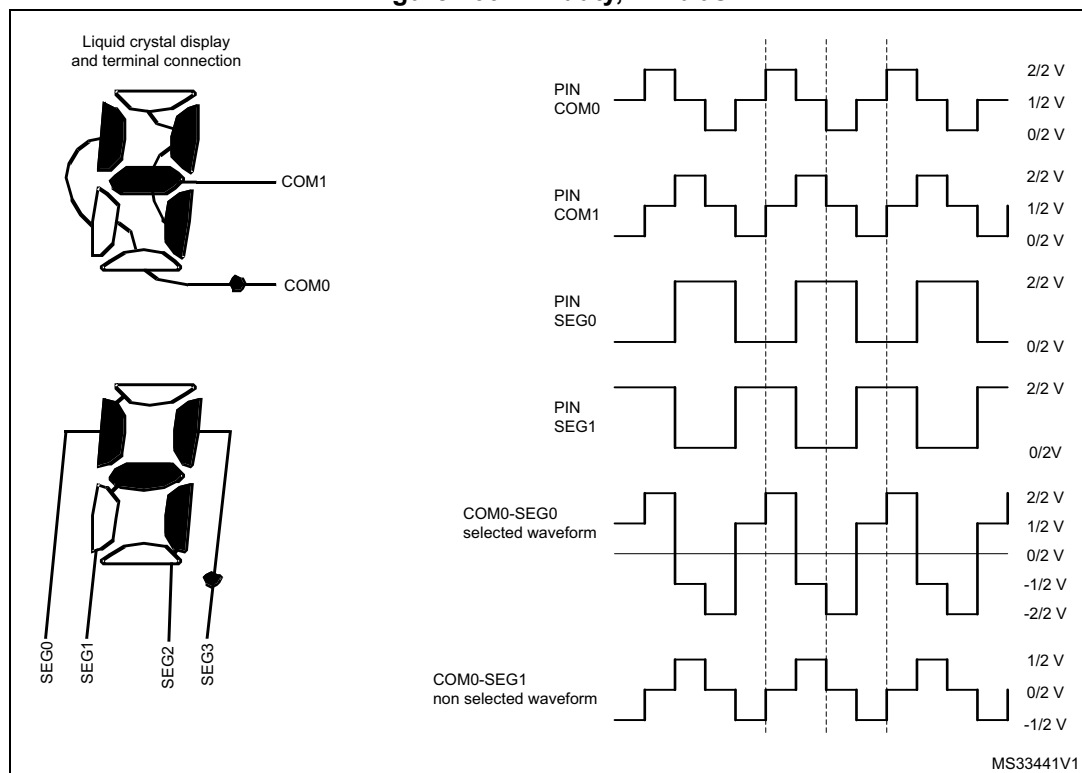
Figure 100. 1/2 duty, 1/2 bias
