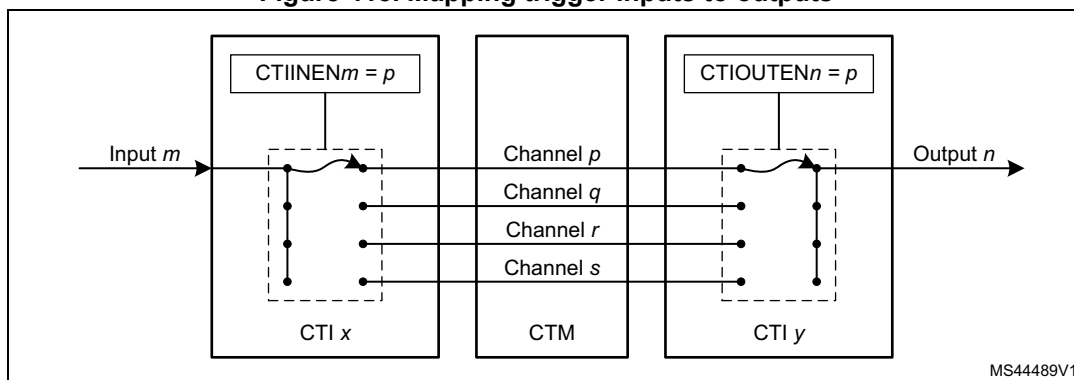
Figure 415. Mapping trigger inputs to outputs
