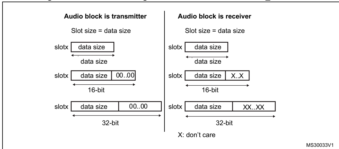
Figure 379. Slot size configuration with FBOFF = 0 in SAI_xSLOTR
