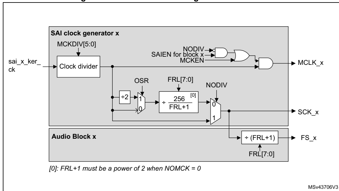
Figure 381. Audio block clock generator overview
