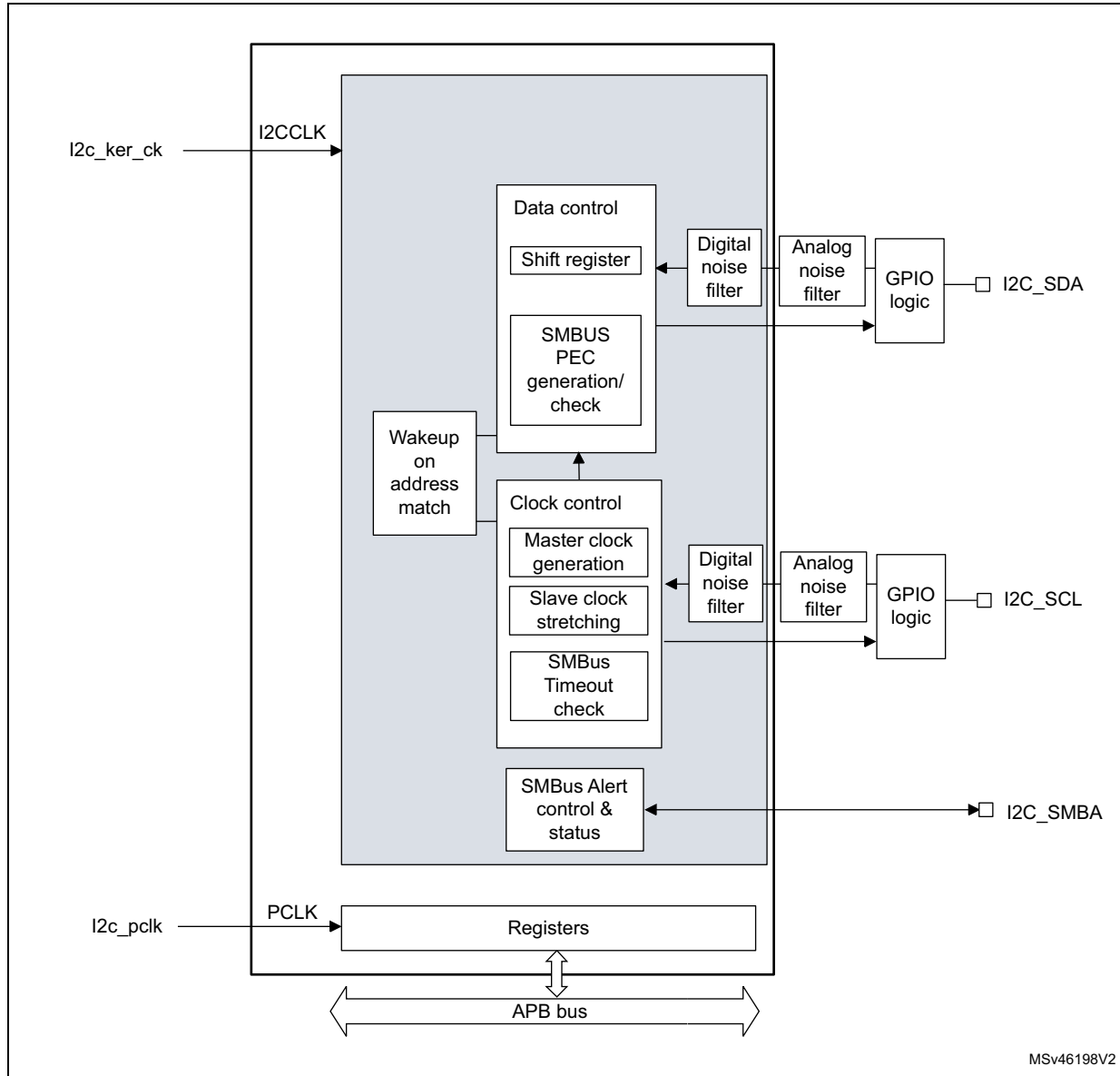
Figure 288. I2C block diagram
