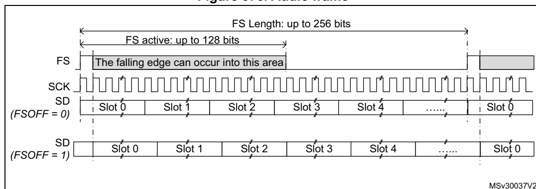
Figure 376. Audio frame
