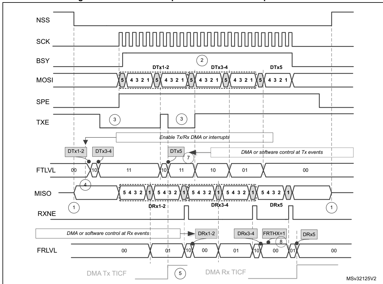
Figure 372. Master full-duplex communication in packed mode
