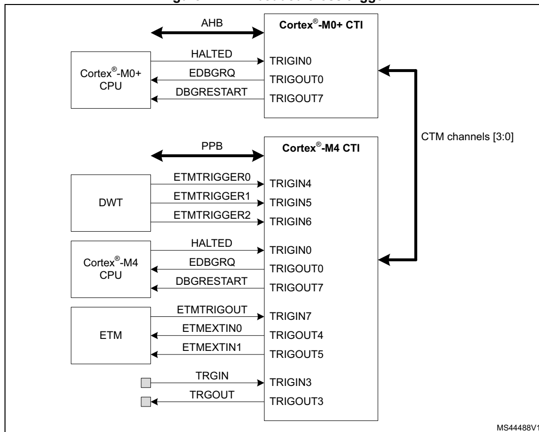
Figure 414. Embedded cross trigger
