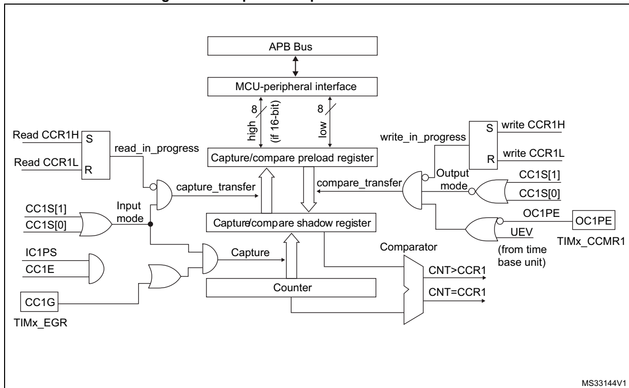
Figure 230. Capture/Compare channel 1 main circuit
