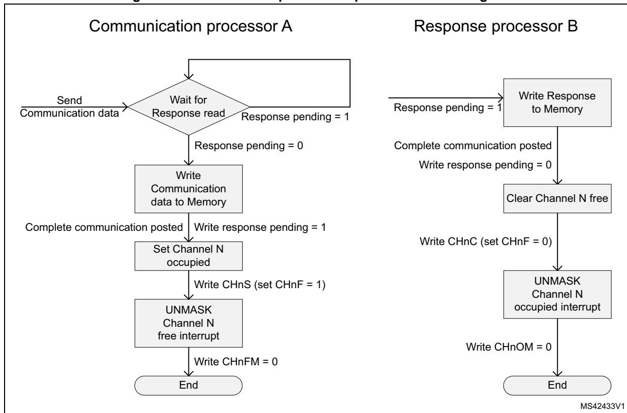
Figure 401. IPCC Half-duplex - Send procedure state diagram
