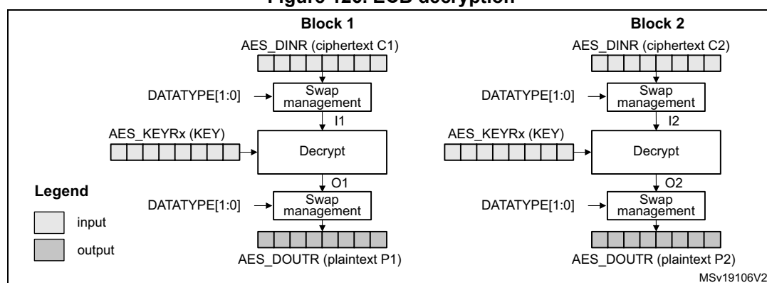
Figure 126. ECB decryption
