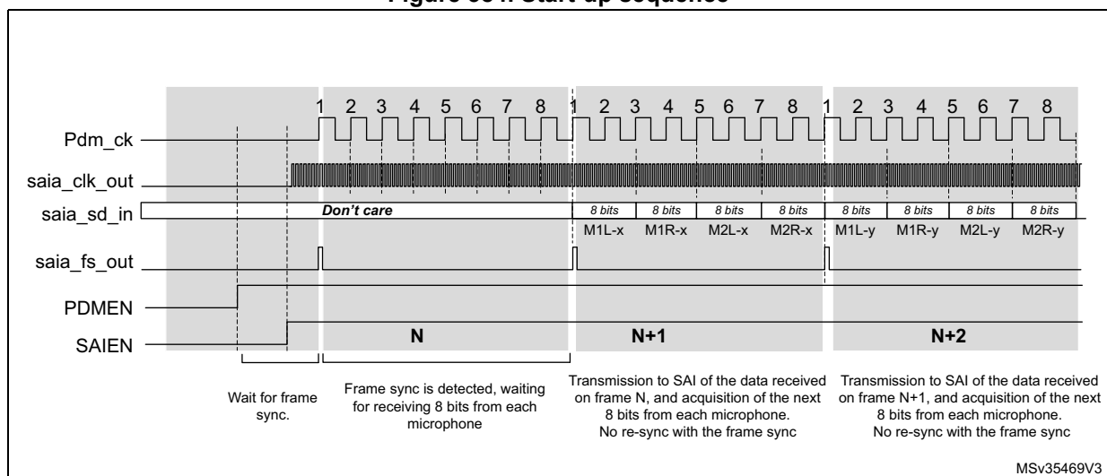
Figure 384. Start-up sequence
