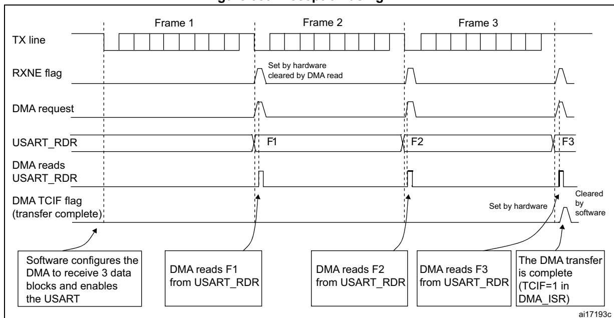
Figure 339. Reception using DMA
