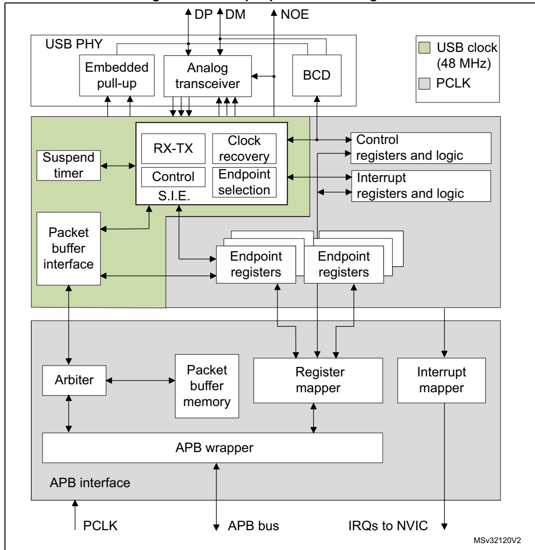
Figure 406. USB peripheral block diagram
