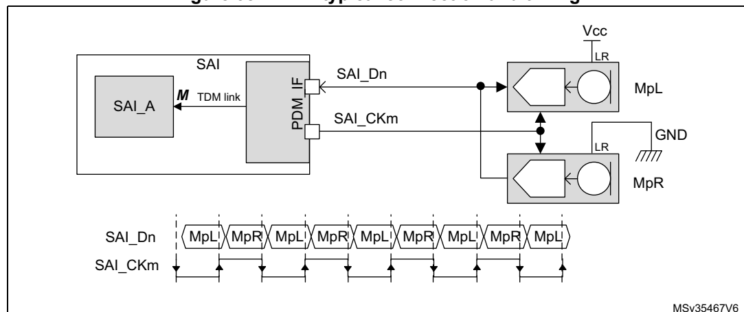
Figure 382. PDM typical connection and timing
