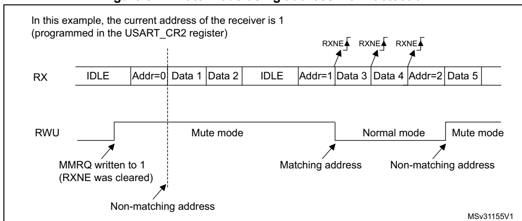
Figure 327. Mute mode using address mark detection
