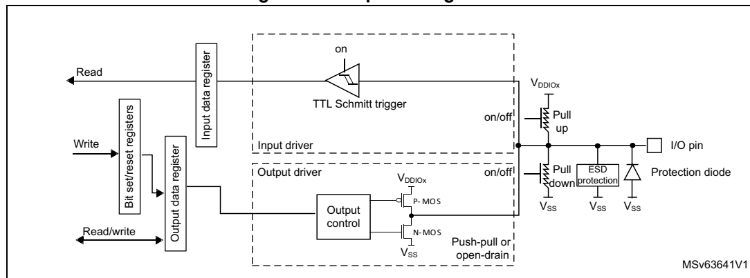
Figure 22. Output configuration
