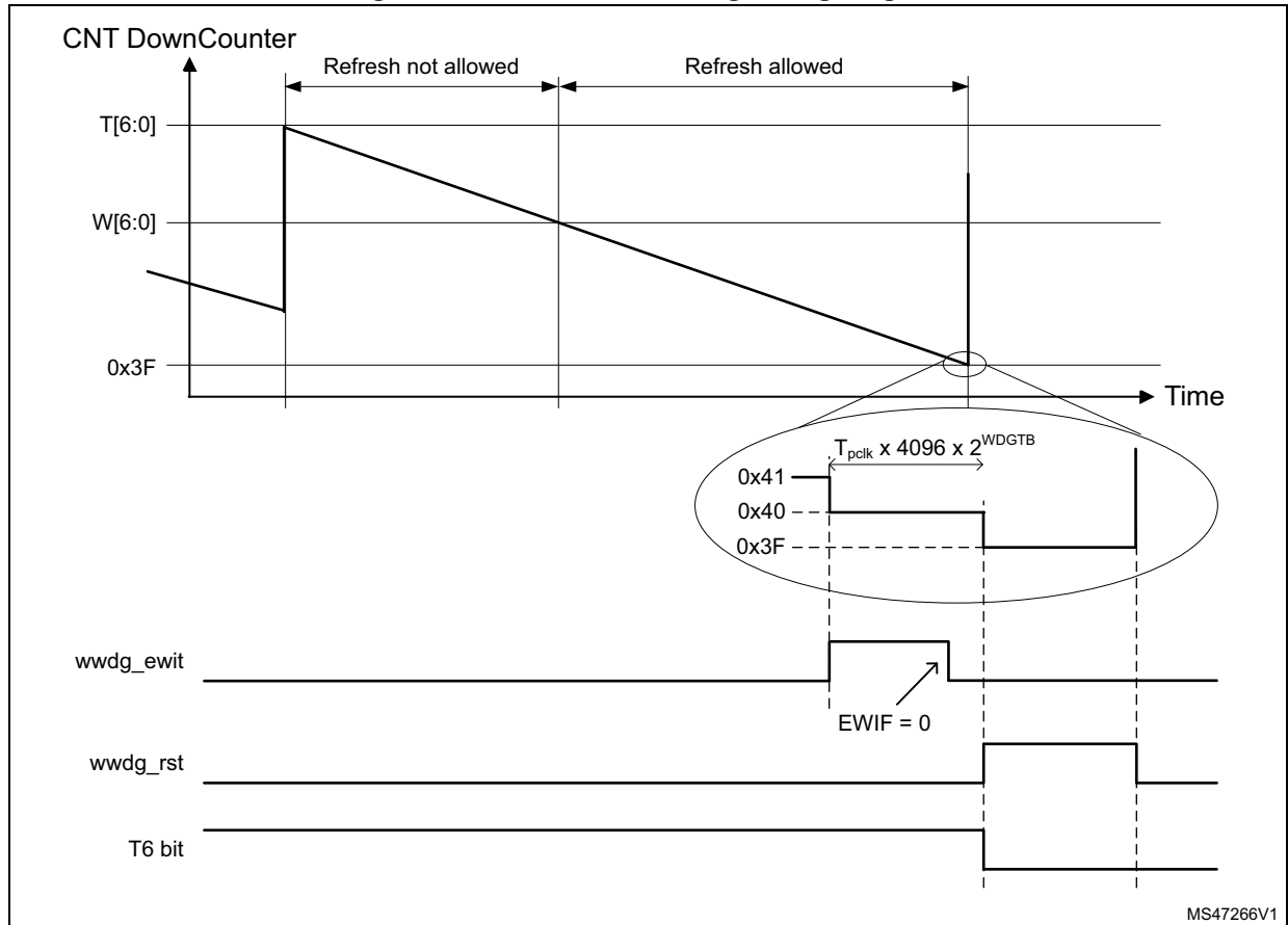
Figure 287. Window watchdog timing diagram
