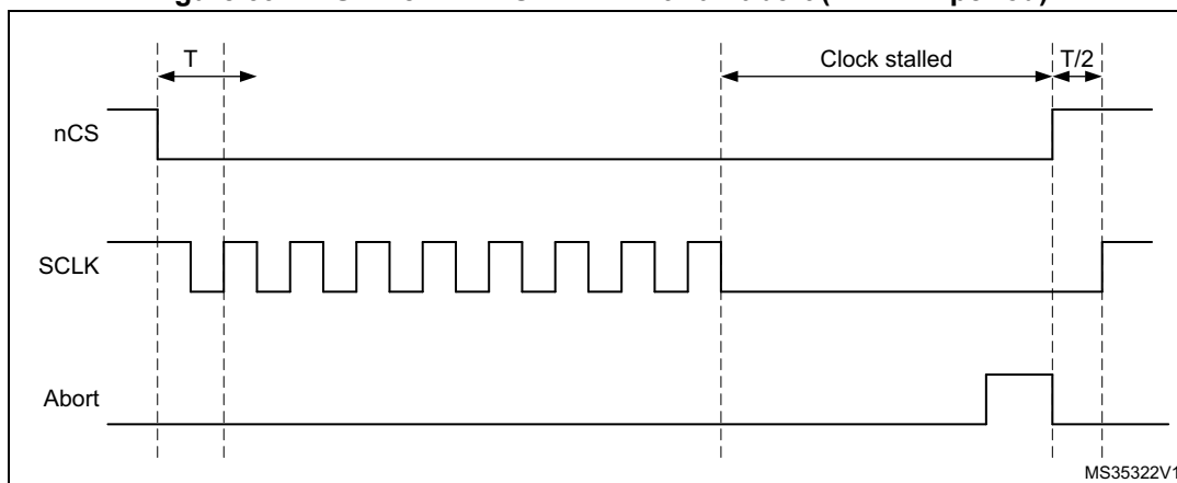
Figure 39. nCS when CKMODE = 1 with an abort ( T = \text{CLK period} )
