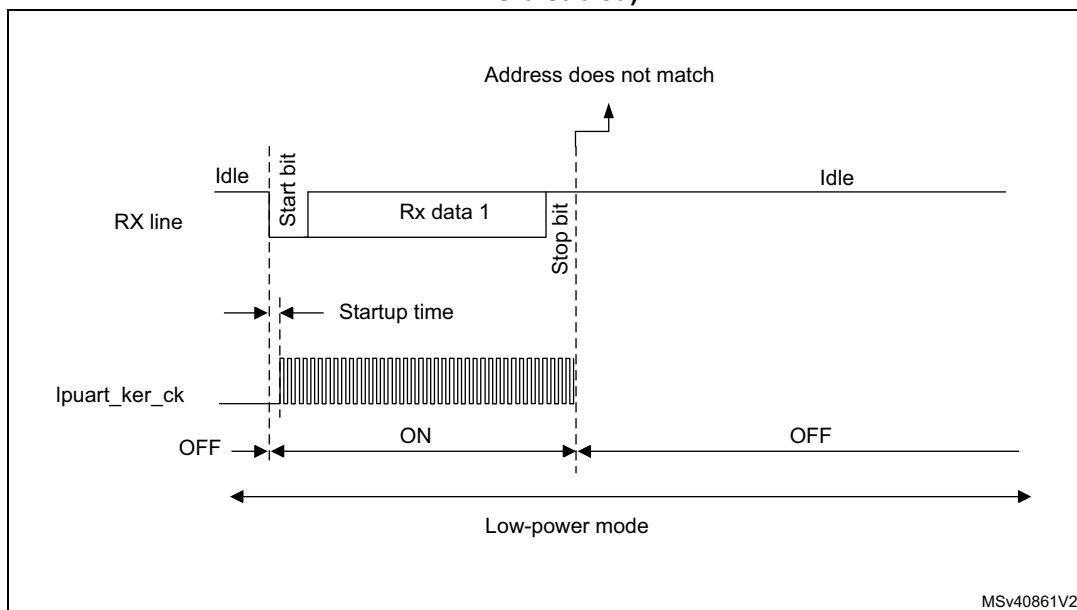
Figure 358. Wakeup event not verified (wakeup event = address match, FIFO disabled)
