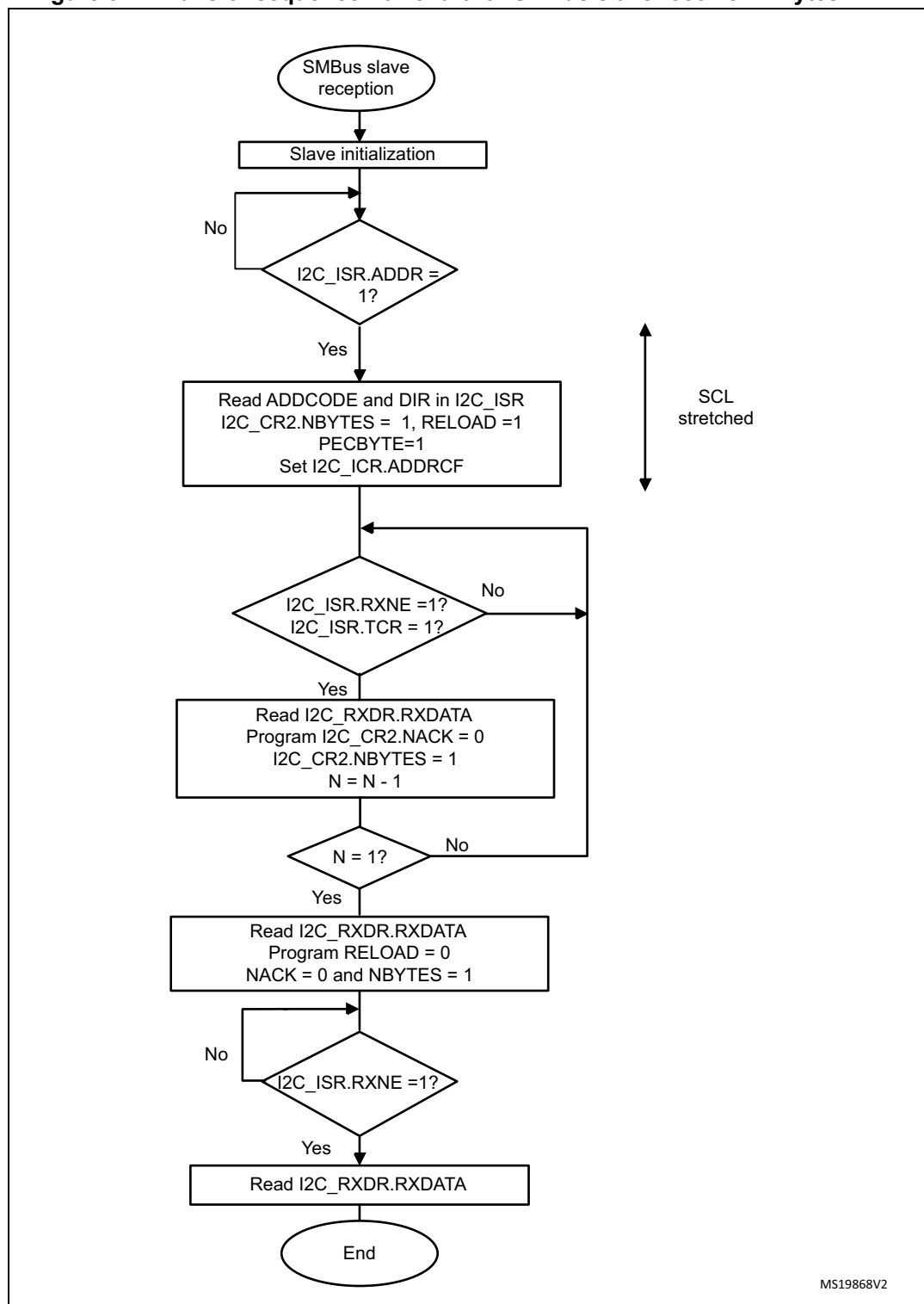
Figure 314. Transfer sequence flowchart for SMBus slave receiver N Bytes + PEC
