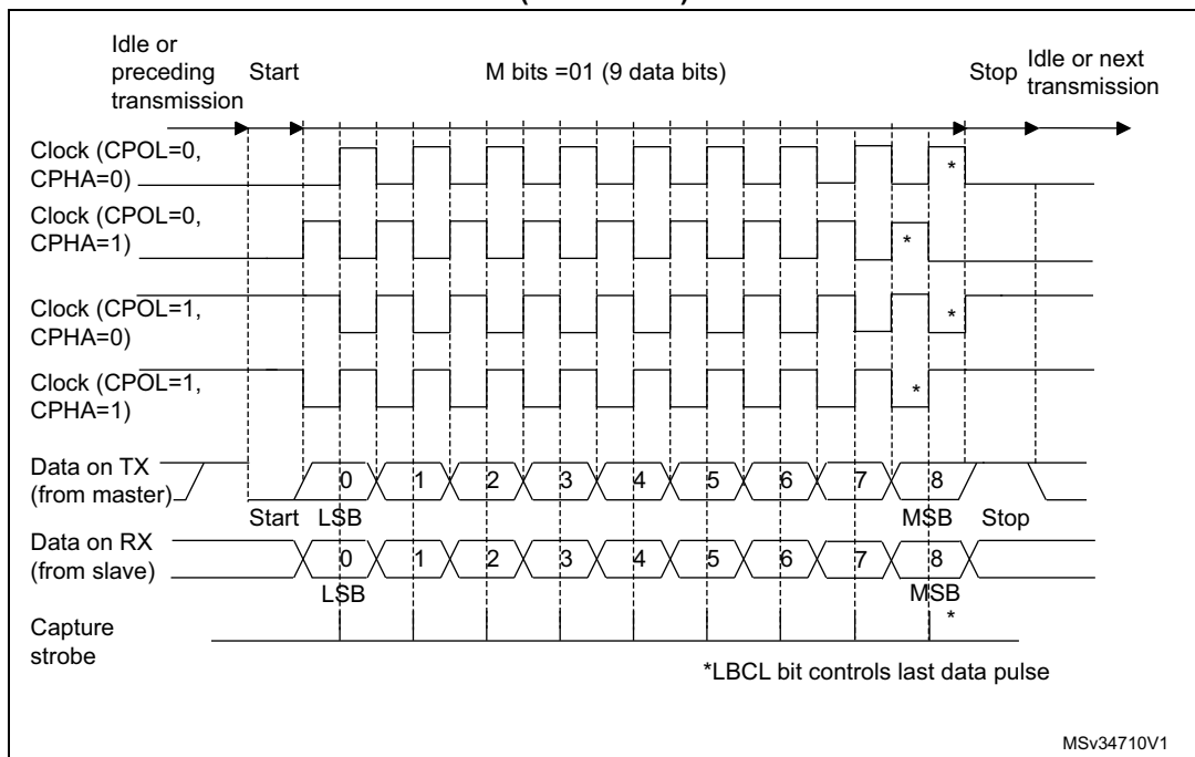
Figure 332. USART data clock timing diagram in synchronous master mode (M bits = 01)
