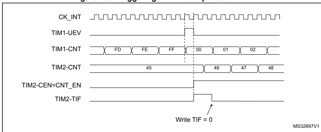
Figure 250. Triggering TIM2 with update of TIM1
