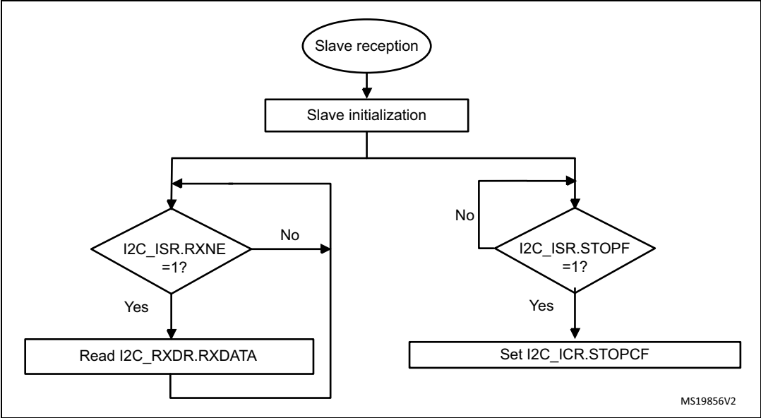
Figure 299. Transfer sequence flowchart for slave receiver with NOSTRETCH=1
