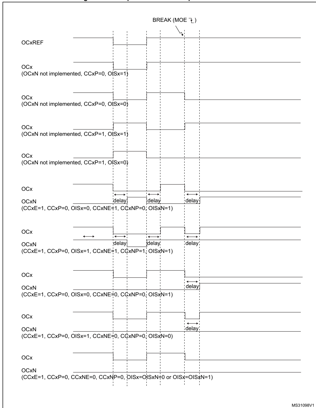
Figure 273. Output behavior in response to a break
