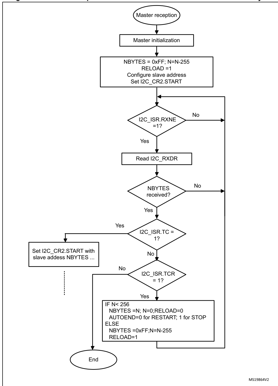
Figure 309. Transfer sequence flowchart for I2C master receiver for N &gt; 255 bytes
