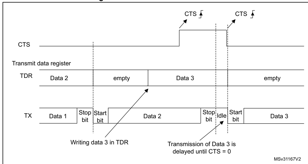
Figure 342. RS232 CTS flow control
