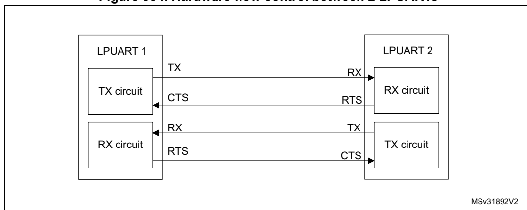
Figure 354. Hardware flow control between 2 LPUARTs
