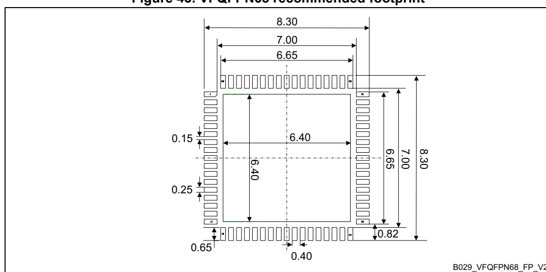
Figure 43. VFQFPN68 recommended footprint
