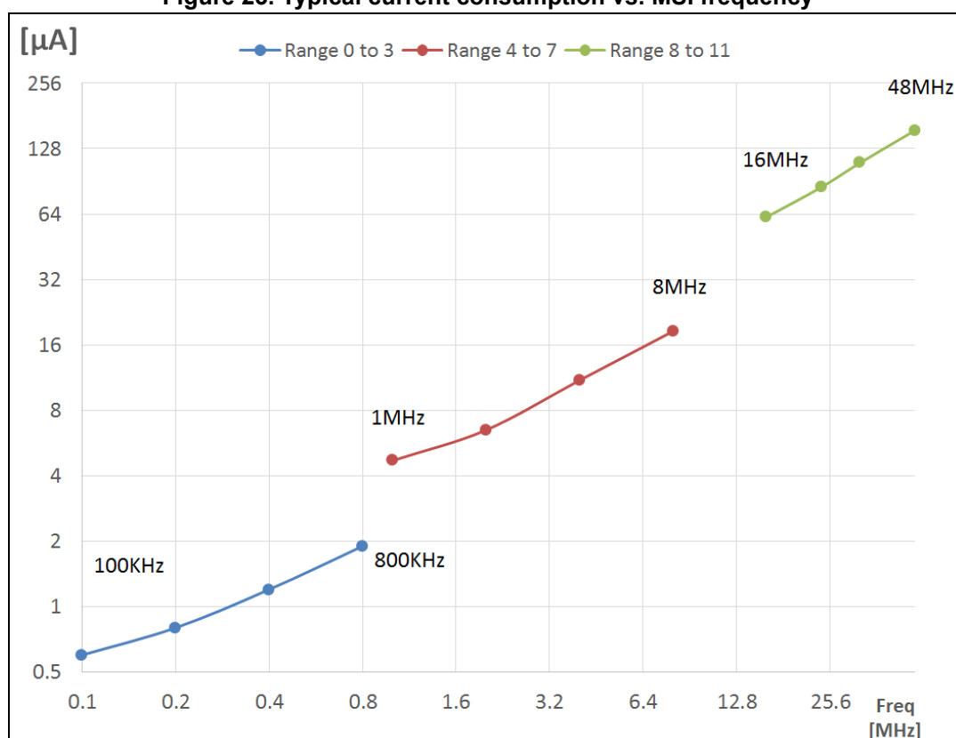
Figure 23. Typical current consumption vs. MSI frequency
