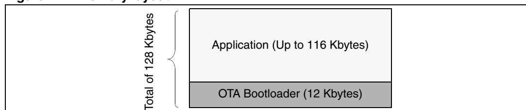
Figure 1. Memory layout
