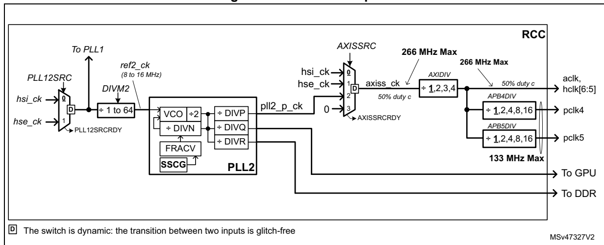
Figure 103. PLL2 clock path
