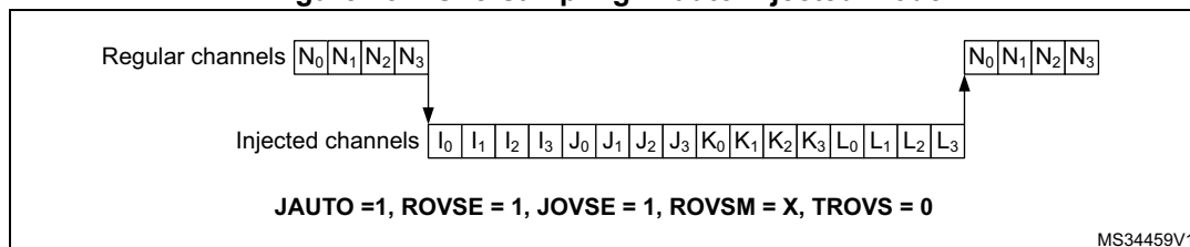
Figure 231. Oversampling in auto-injected mode
