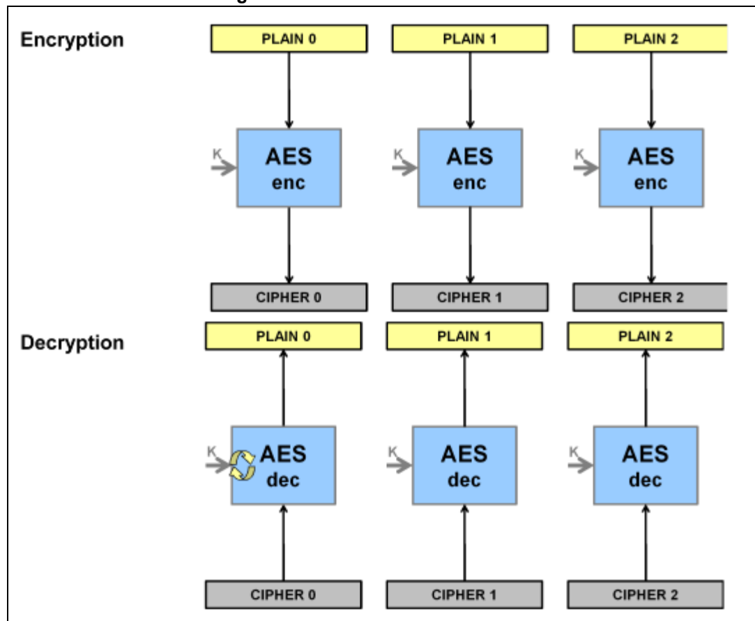
Figure 330. AES-ECB mode overview
