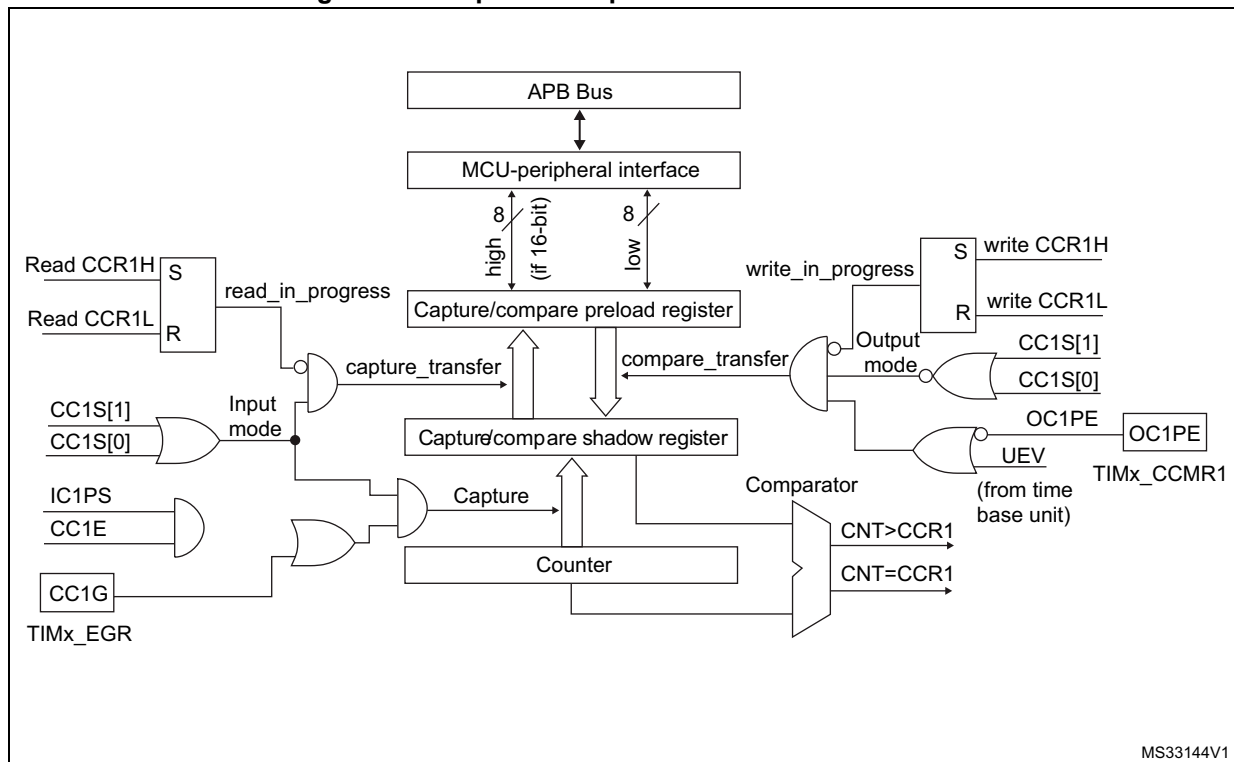
Figure 439. Capture/Compare channel 1 main circuit
