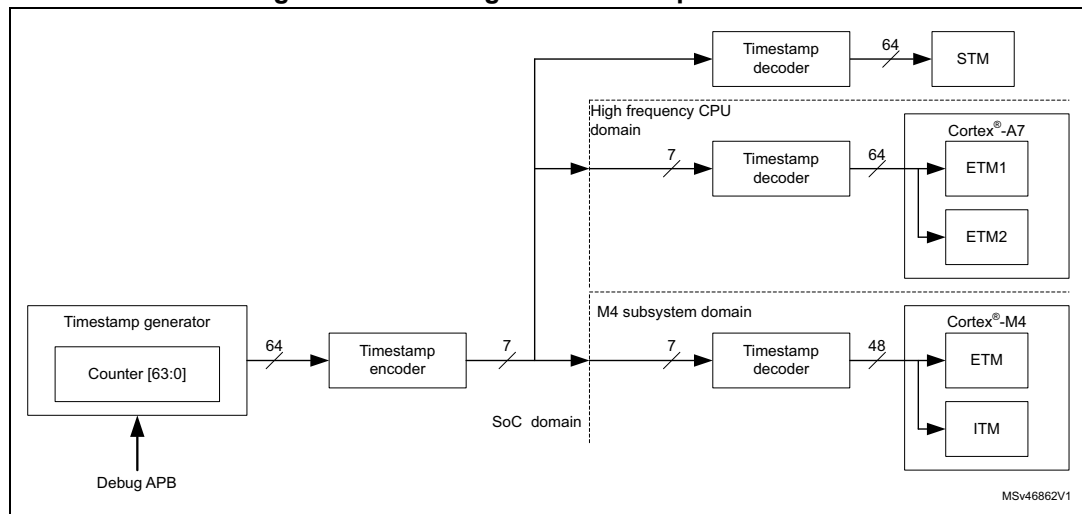
Figure 814. CoreSight™ timestamp distribution
