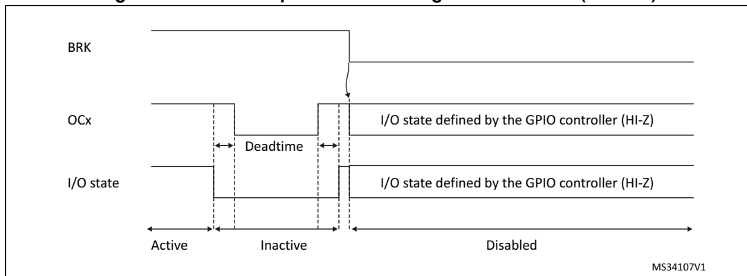
Figure 399. PWM output state following BRK assertion (OSSI=0)
