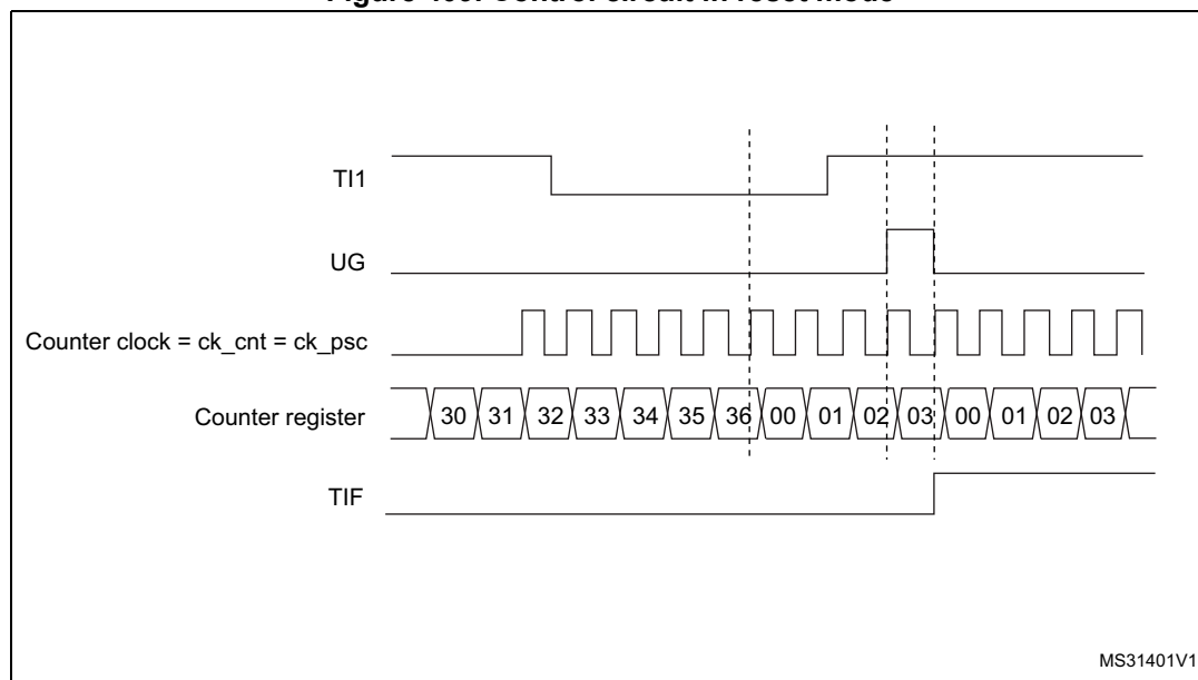
Figure 409. Control circuit in reset mode
