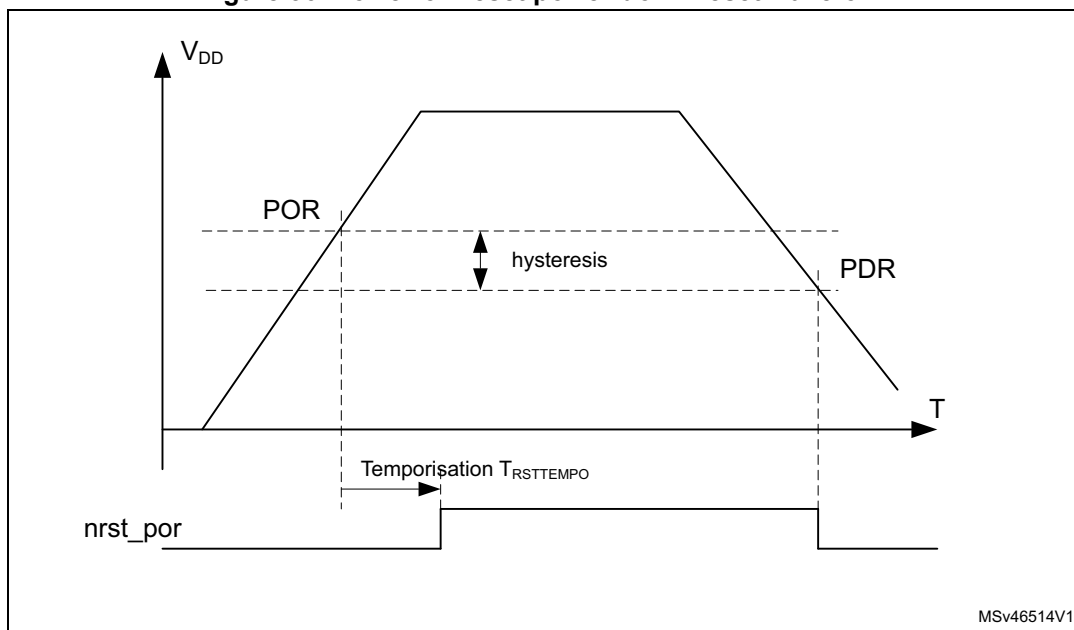
Figure 36. Power-on reset/power-down reset waveform
