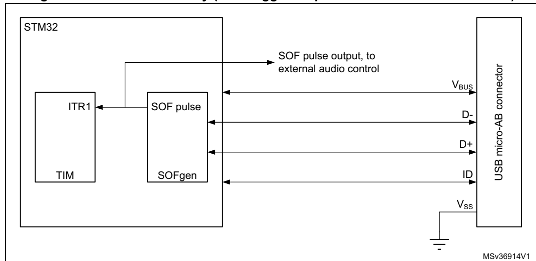
Figure 737. SOF connectivity (SOF trigger output to TIM and ITR1 connection)
