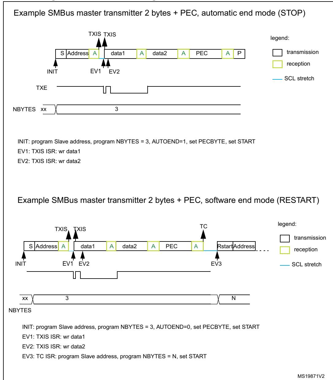
Figure 580. Bus transfer diagrams for SMBus master transmitter
