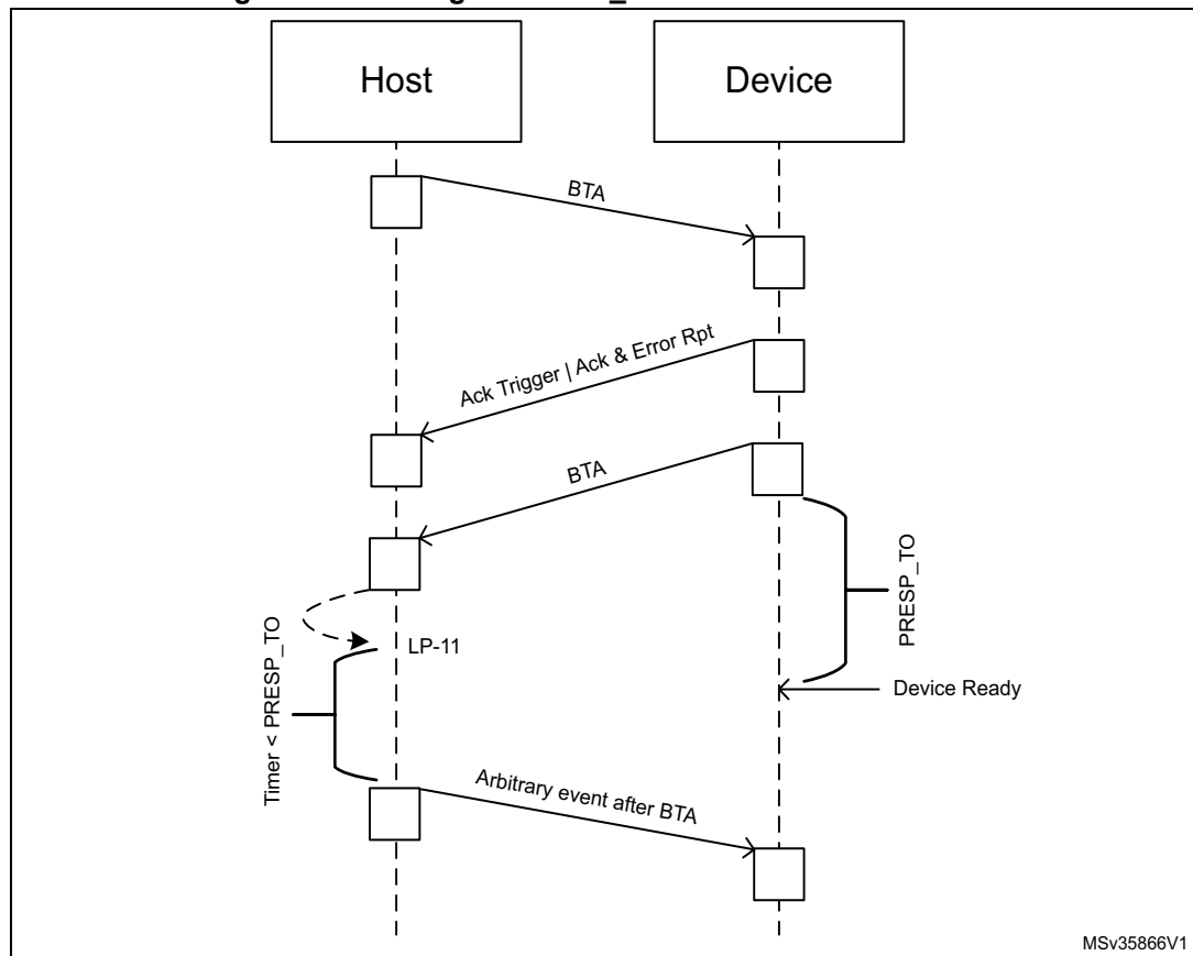
Figure 297. Timing of PRESP_TO after a bus-turn-around
