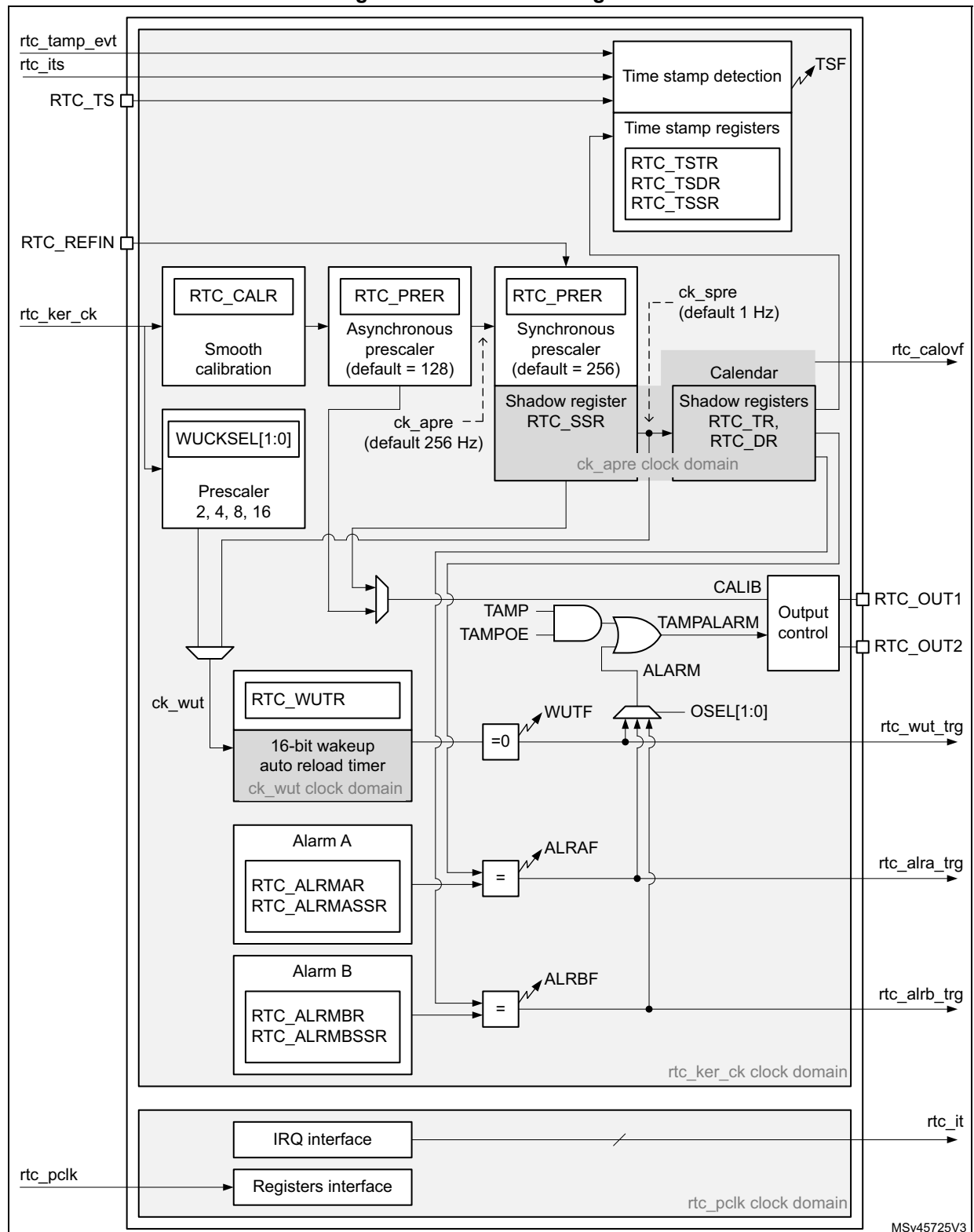
Figure 549. RTC block diagram
