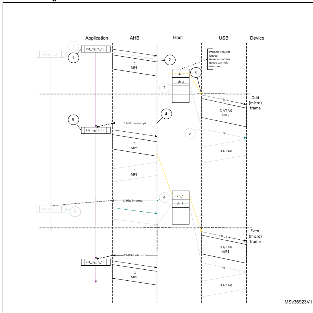
Figure 754. Normal isochronous OUT transaction - DMA mode
