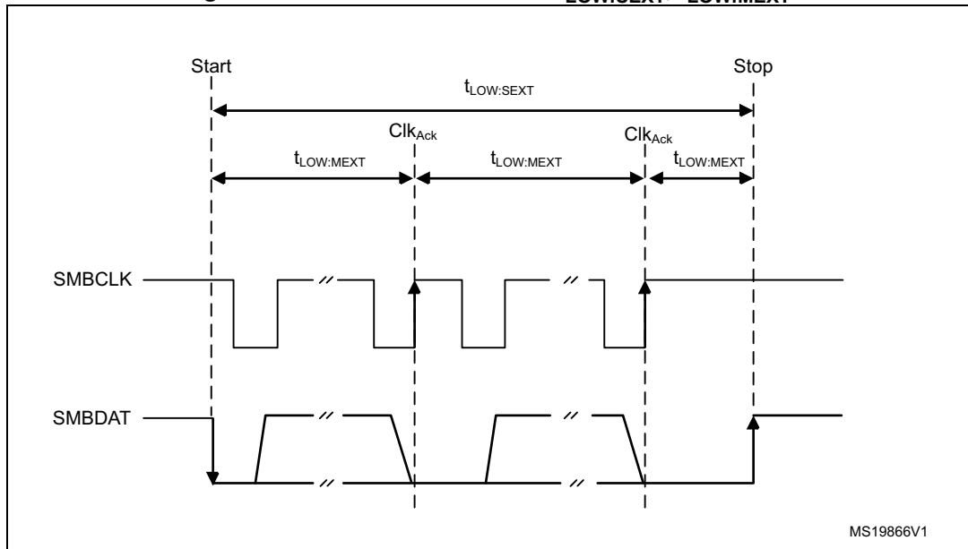
Figure 575. Timeout intervals for t_{\text{LOW:SEXT}} , t_{\text{LOW:MEXT}}
