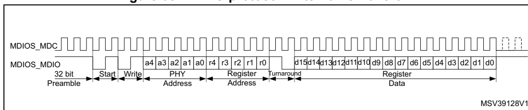
Figure 682. MDIO protocol write frame waveform
