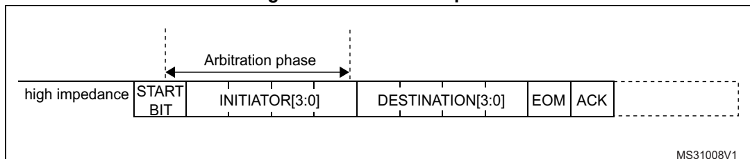
Figure 771. Arbitration phase
