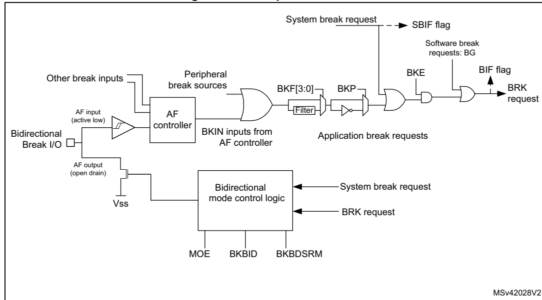
Figure 515. Output redirection
