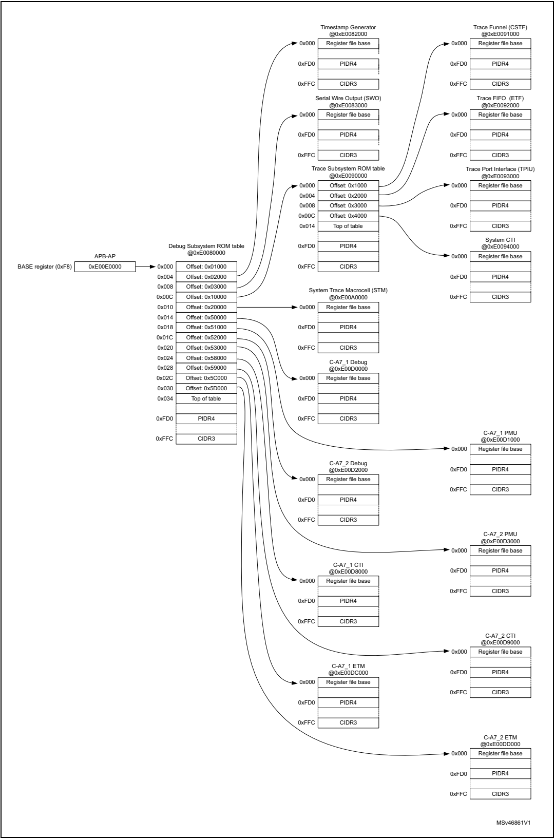
Figure 813. Debug APB CoreSight™ topology
