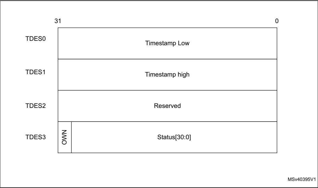
Figure 801. Transmit descriptor write-back format
