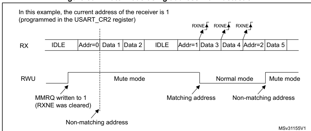
Figure 591. Mute mode using address mark detection
