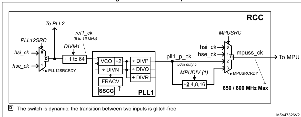
Figure 102. MPU clock path
