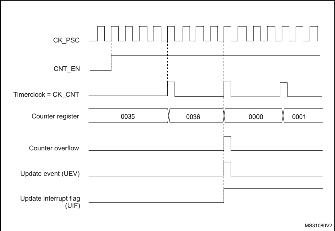
Figure 527. Counter timing diagram, internal clock divided by 4
