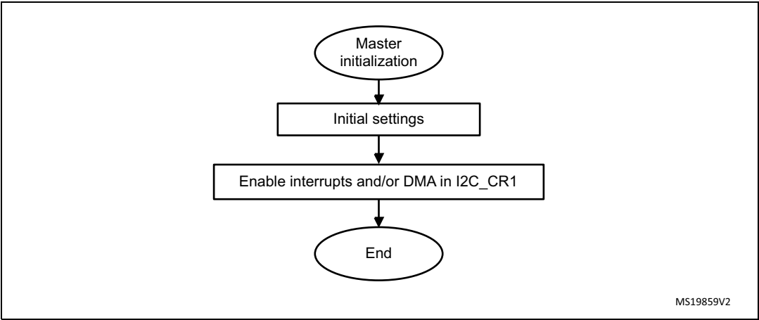
Figure 566. Master initialization flowchart
