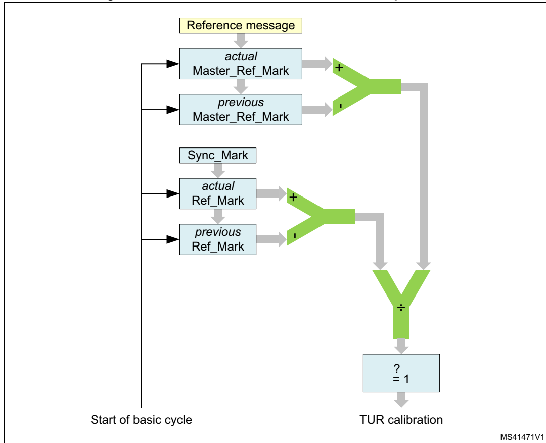
Figure 733. TTCAN level 0 and level 2 drift compensation
