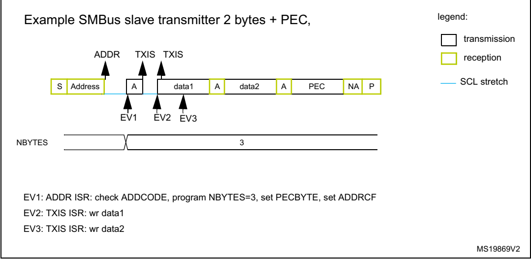
Figure 577. Transfer bus diagrams for SMBus slave transmitter (SBC=1)
