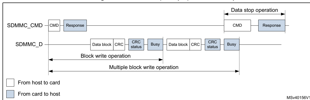
Figure 686. SDMMC (multiple) block write operation
