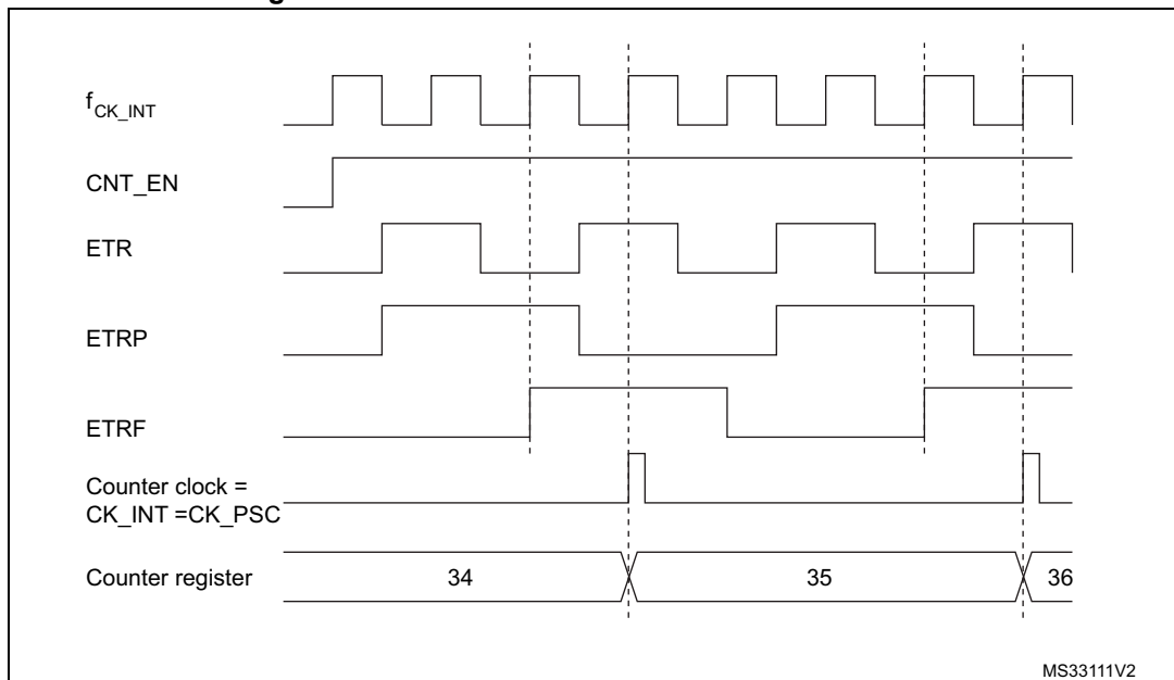
Figure 437. Control circuit in external clock mode 2
