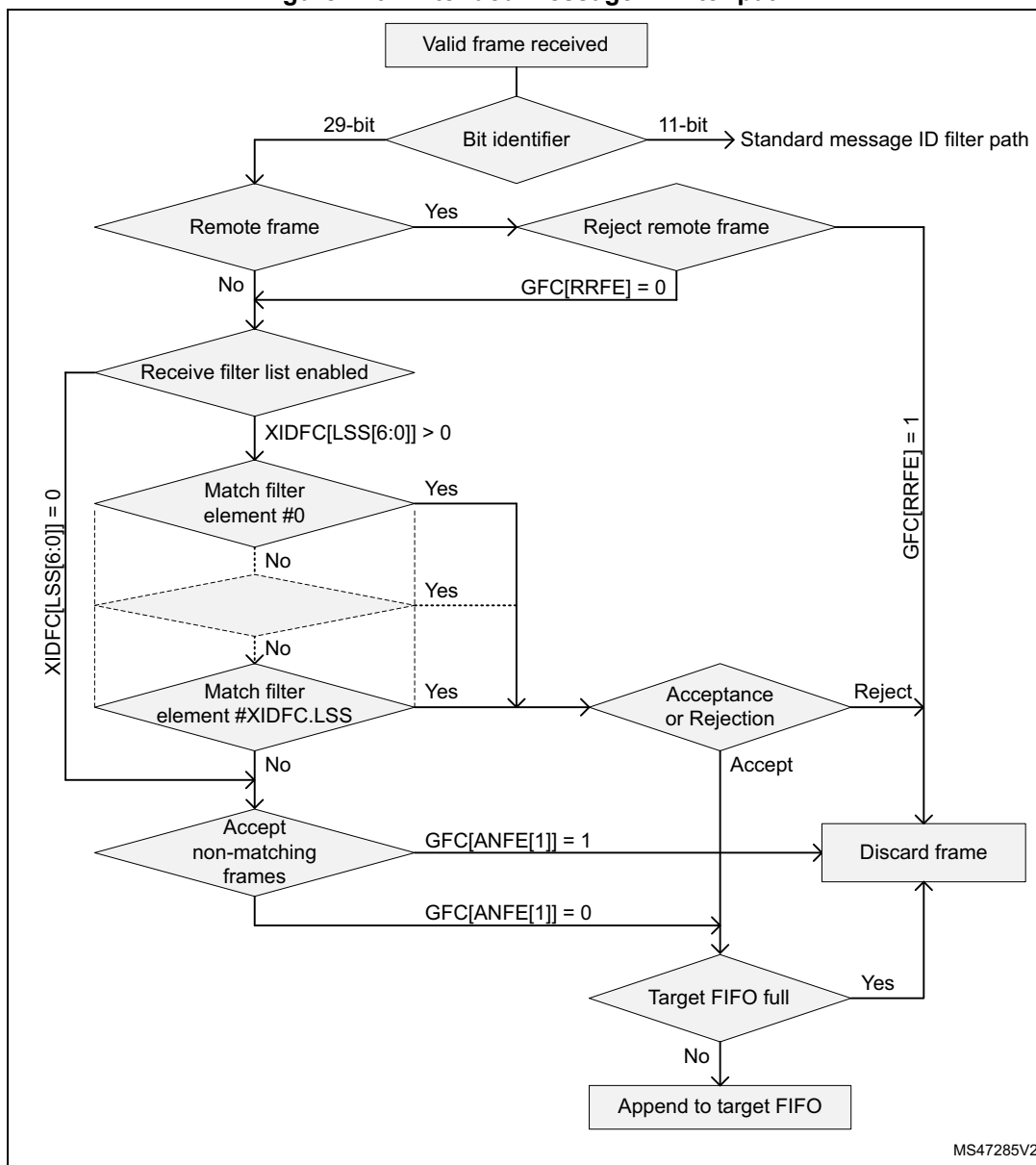
Figure 726. Extended message ID filter path
