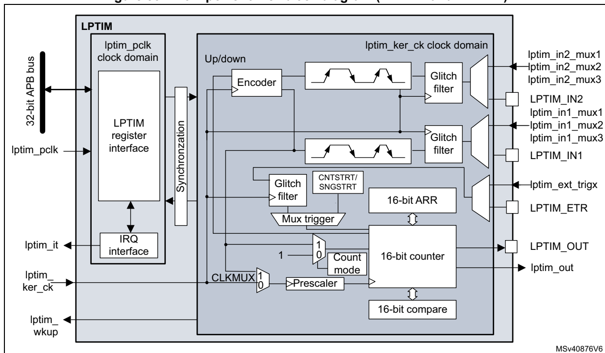
Figure 532. Low-power timer block diagram (LPTIM1 and LPTIM2)
