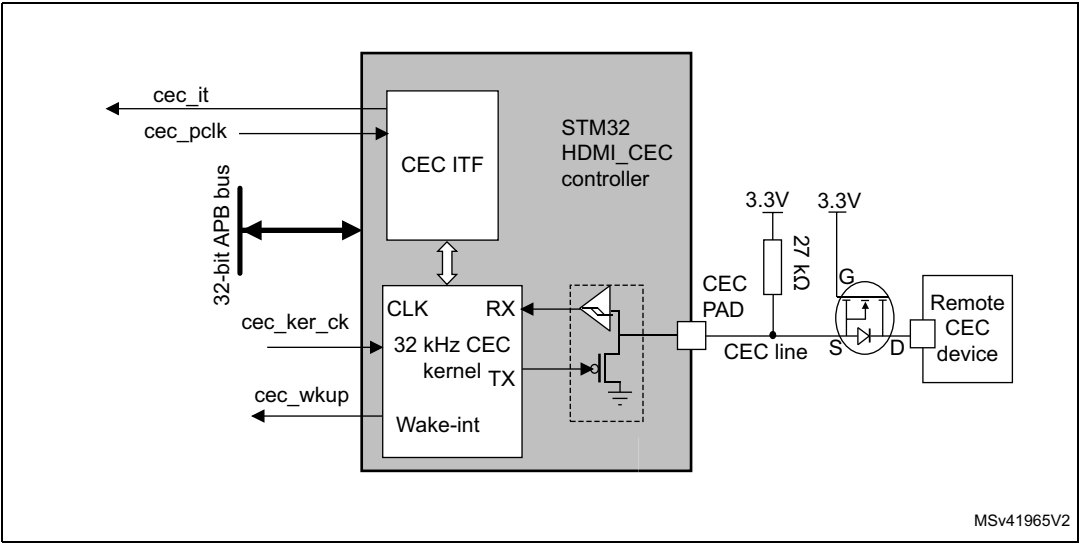
Figure 766. HDMI-CEC block diagram
