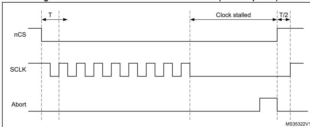
Figure 179. nCS when CKMODE = 1 with an abort ( T = \text{CLK period} )
