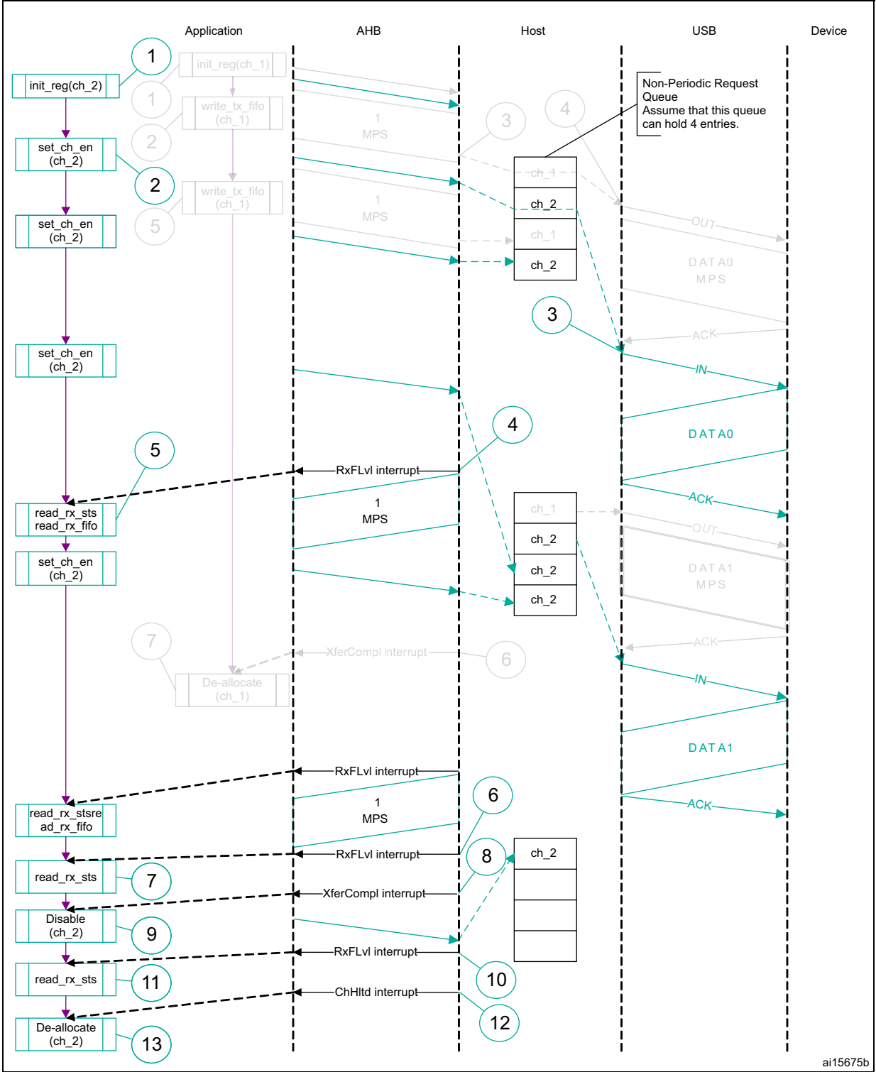
Figure 745. Bulk/control IN transactions
