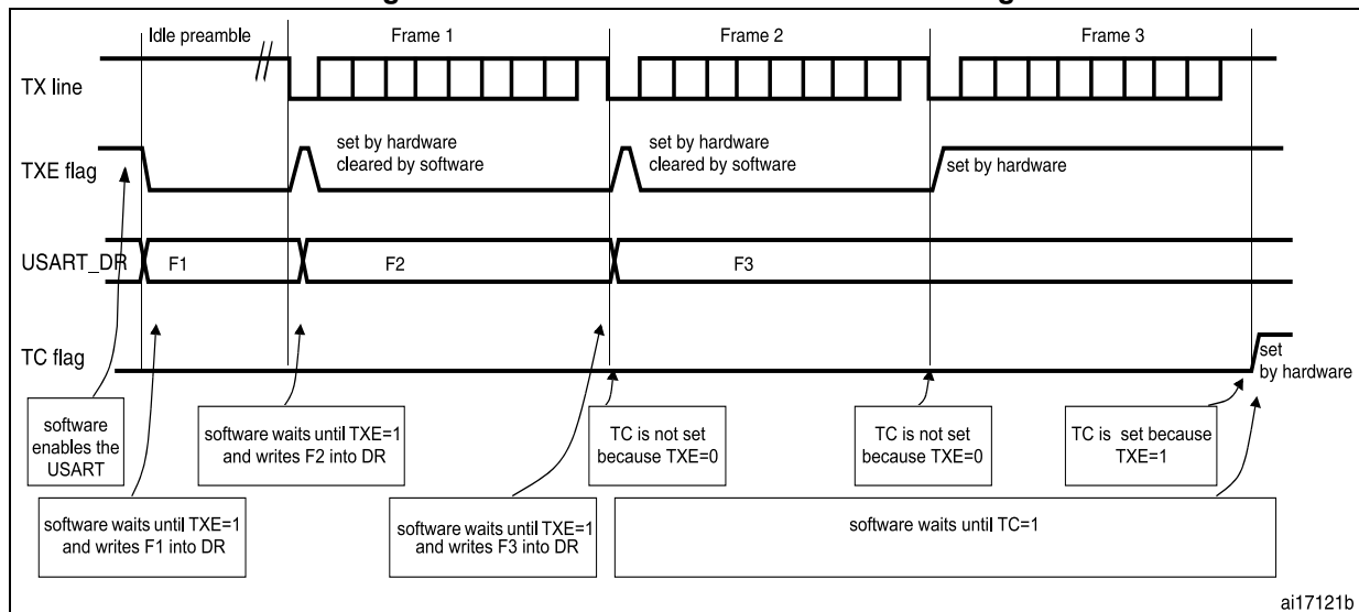
Figure 585. TC/TXE behavior when transmitting
