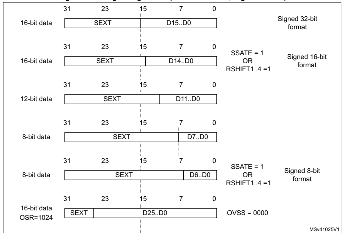
Figure 211. Right alignment (offset enabled, signed value)
