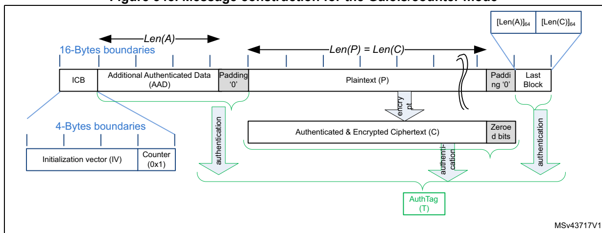
Figure 348. Message construction for the Galois/counter mode
