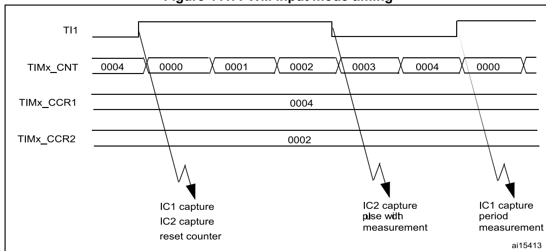
Figure 441. PWM input mode timing
