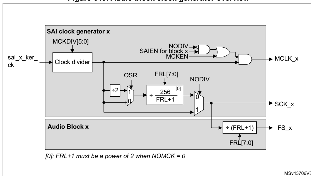
Figure 649. Audio block clock generator overview
