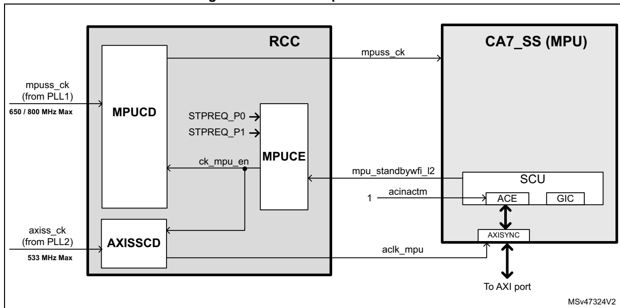
Figure 100. MPU low-power interface
