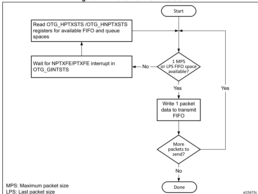
Figure 742. Transmit FIFO write task
