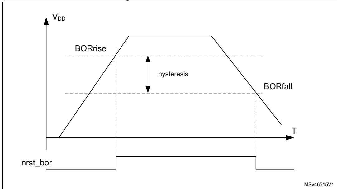
Figure 37. BOR thresholds
