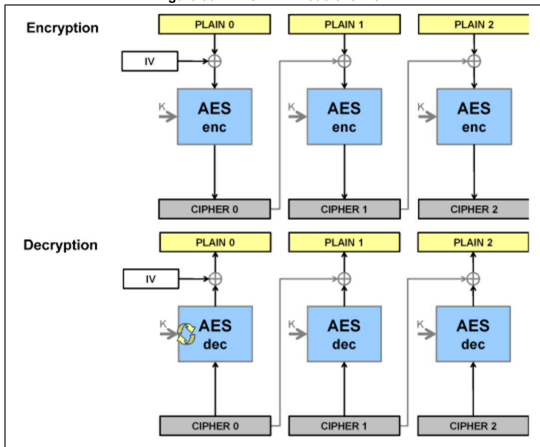
Figure 331. AES-CBC mode overview
