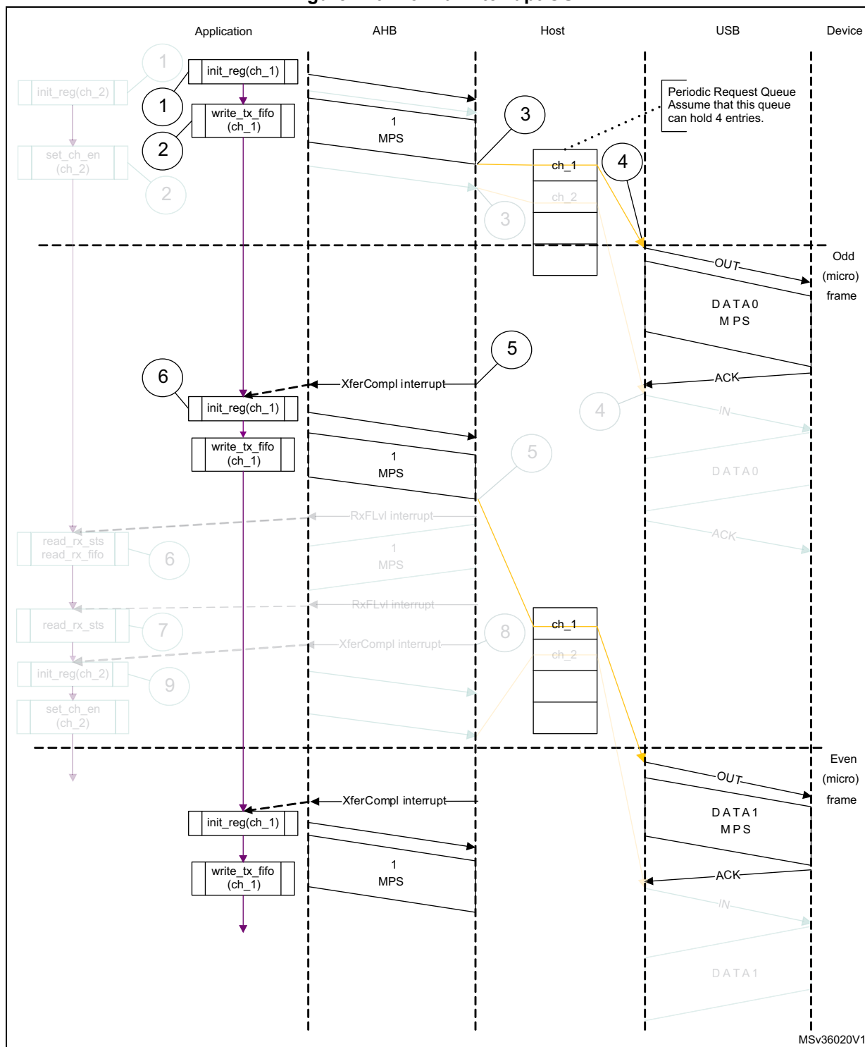
Figure 746. Normal interrupt OUT
