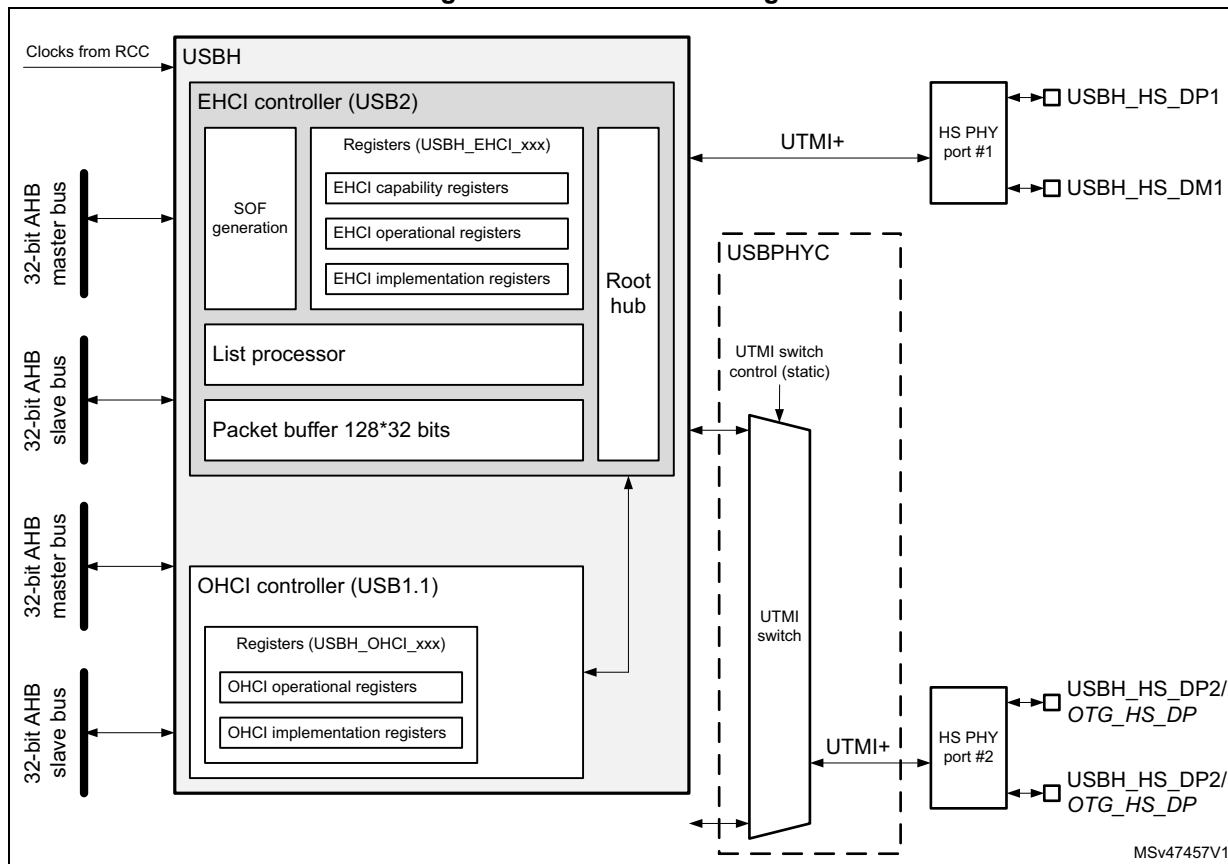
Figure 765. USBH block diagram
