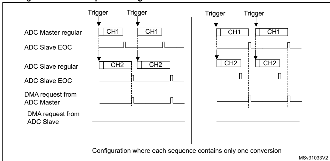
Figure 246. DMA requests in regular simultaneous mode when DAMDF=0b10
