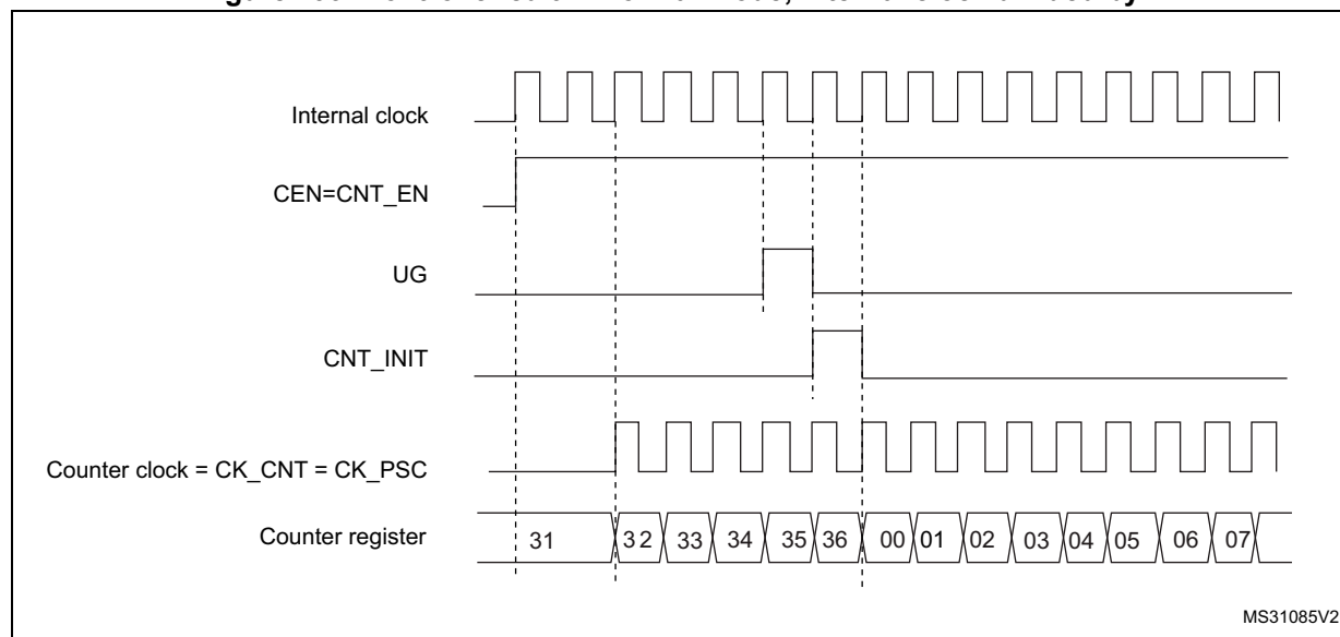
Figure 499. Control circuit in normal mode, internal clock divided by 1
