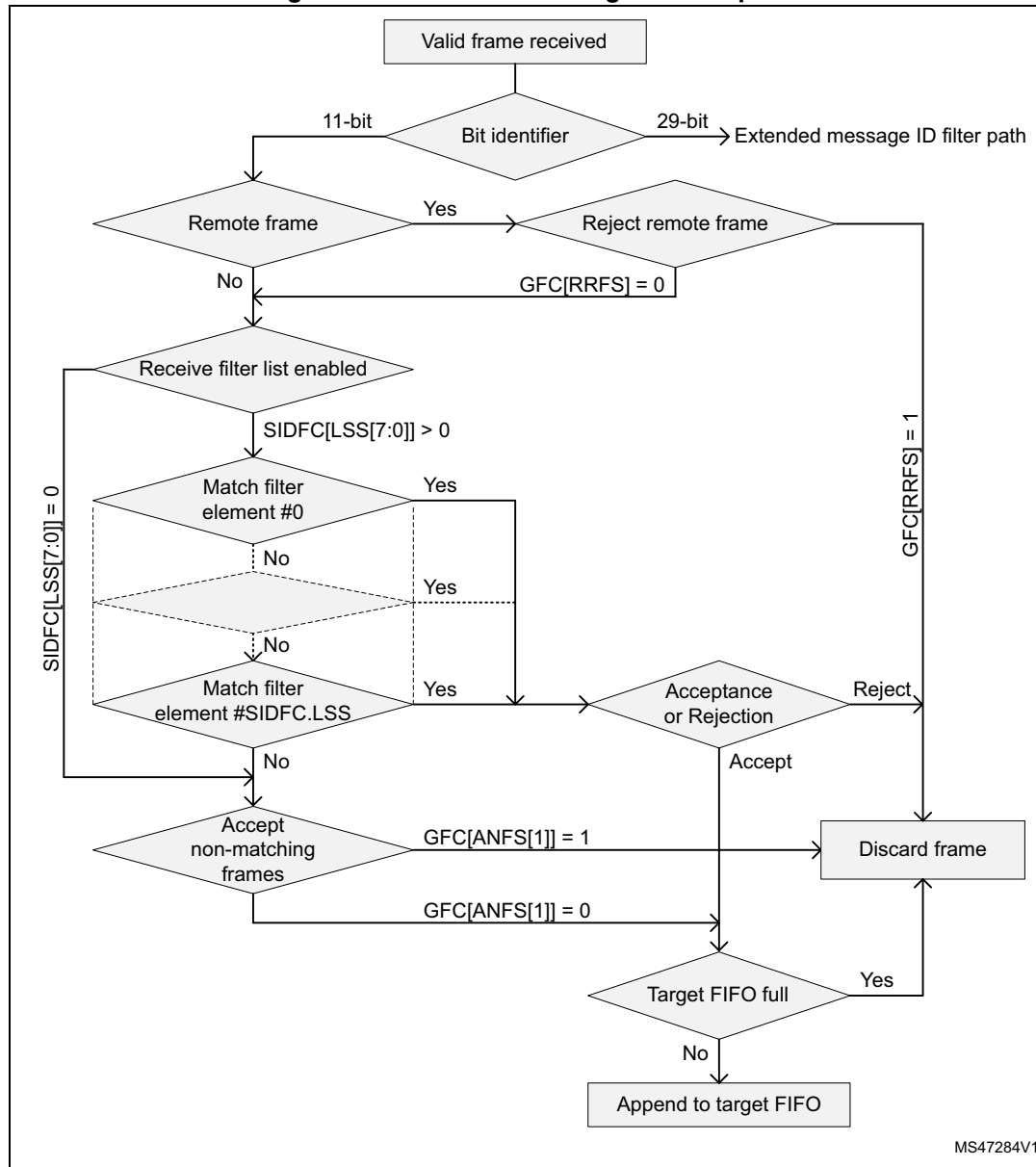
Figure 725. Standard message ID filter path
