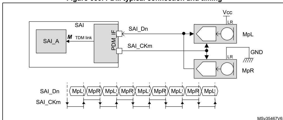
Figure 650. PDM typical connection and timing
