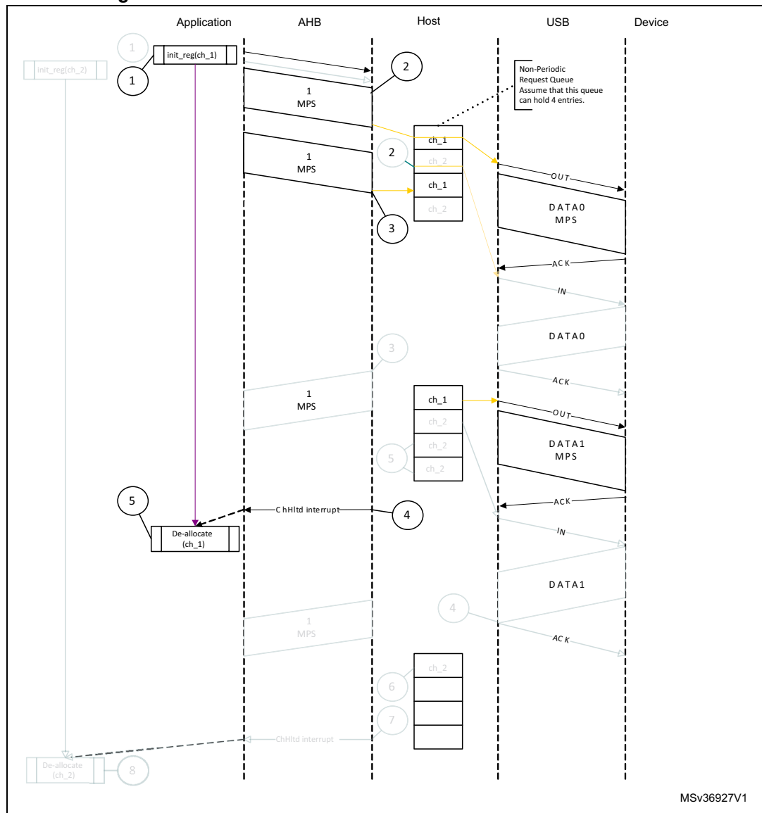
Figure 750. Normal bulk/control OUT/SETUP transactions - DMA
