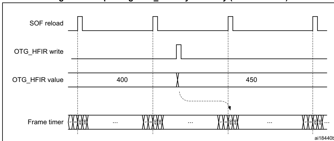
Figure 738. Updating OTG_HFIR dynamically (RLDCTRL = 1)
