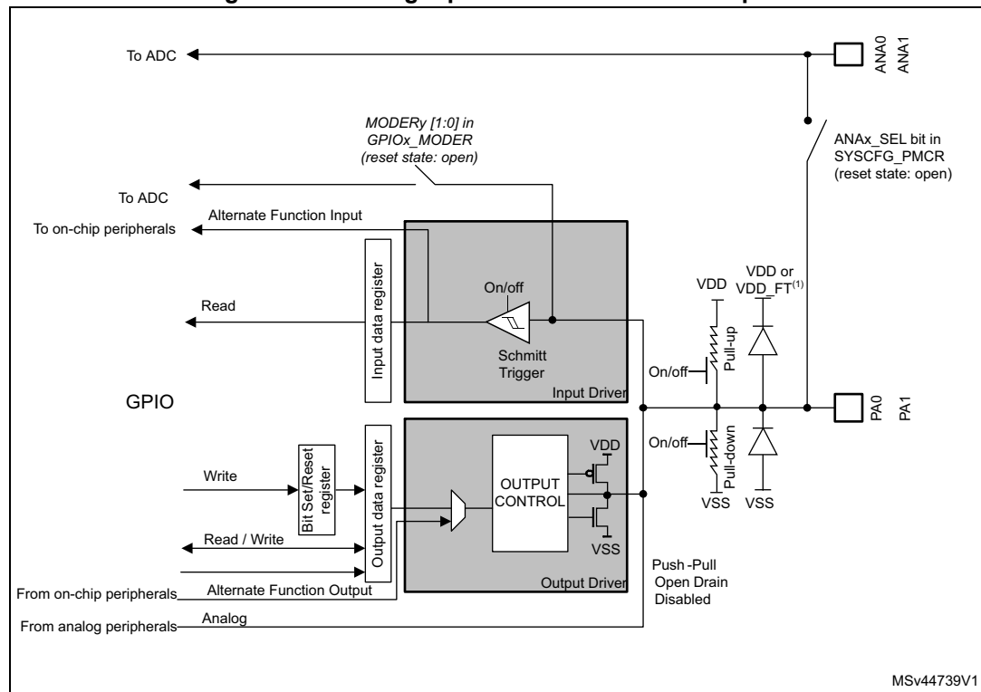
Figure 125. Analog inputs connected to ADC inputs
