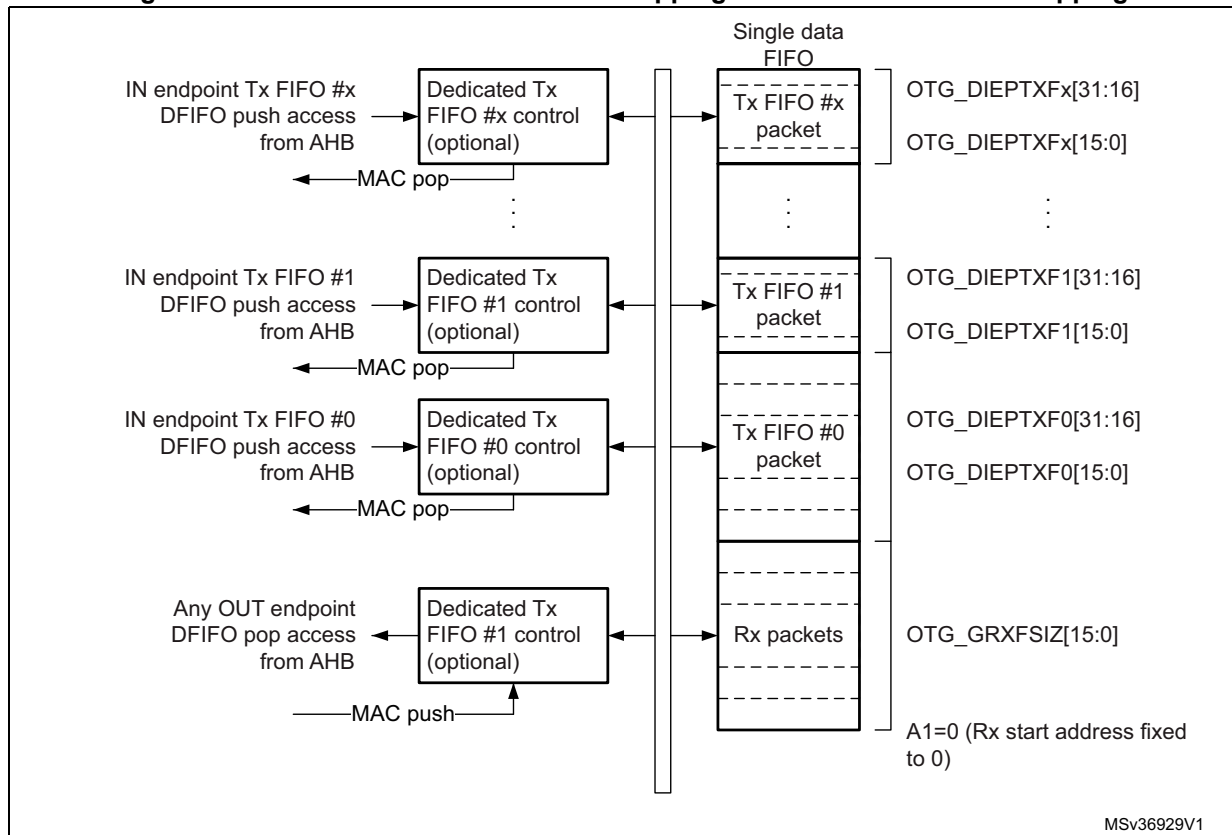
Figure 739. Device-mode FIFO address mapping and AHB FIFO access mapping
