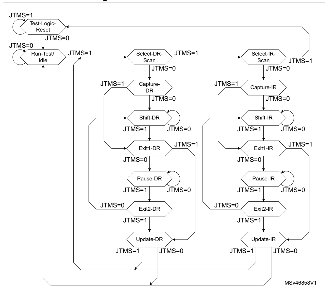
Figure 810. JTAG TAP state machine
