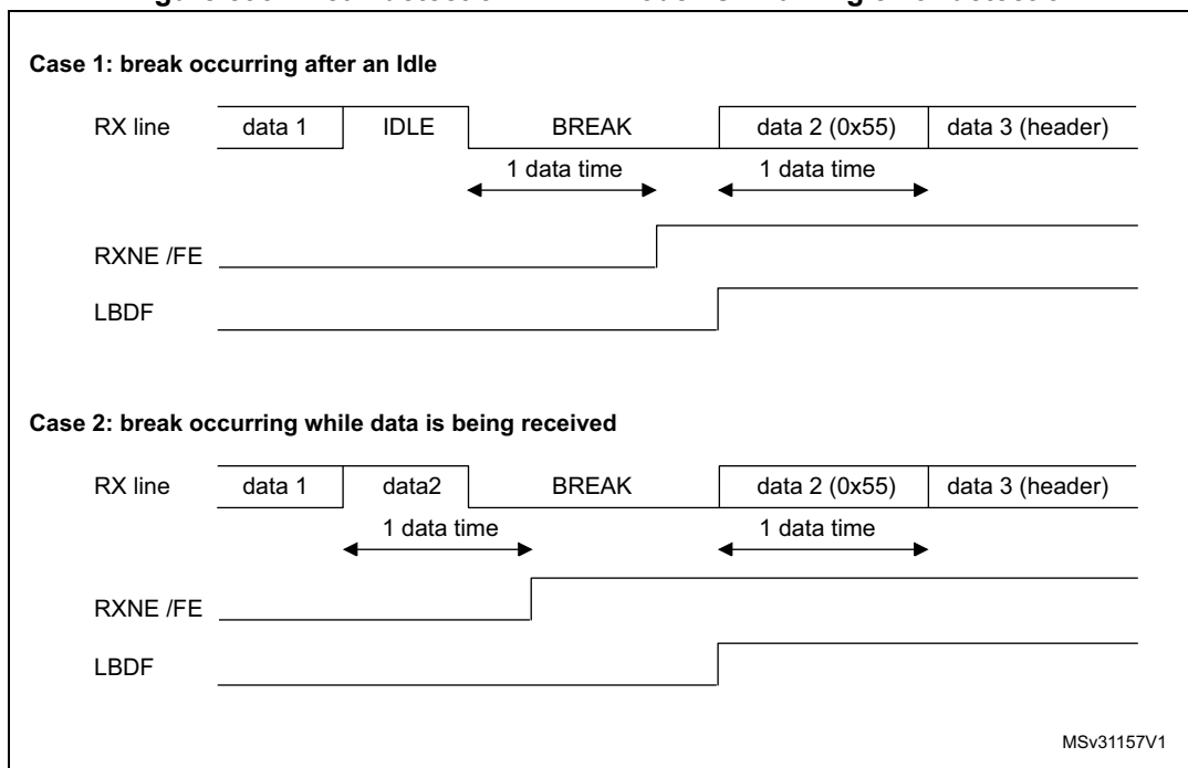
Figure 593. Break detection in LIN mode vs. Framing error detection
