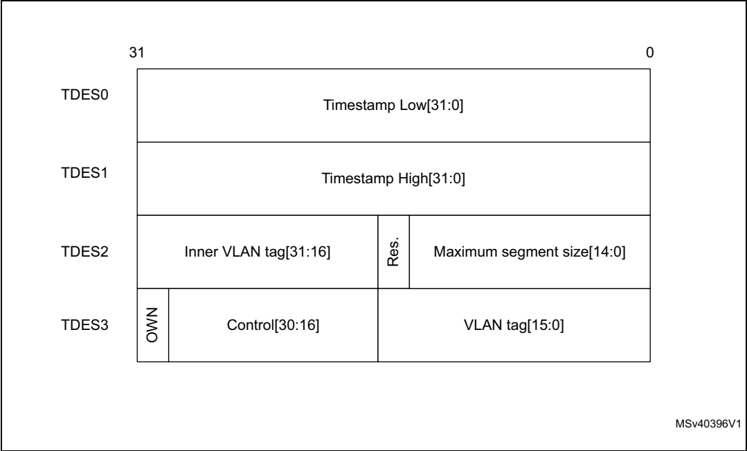
Figure 802. Transmit context descriptor format
