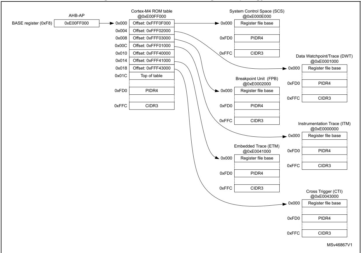
Figure 819. Cortex®-M4 CoreSight™ topology
