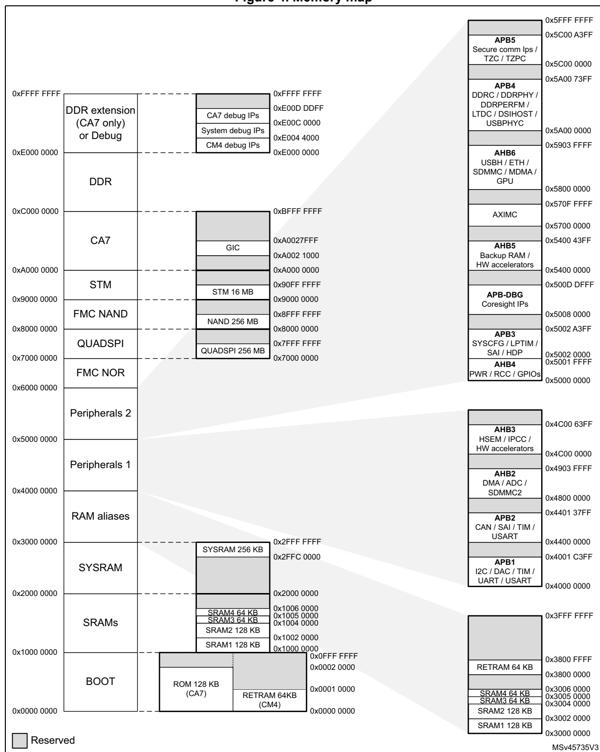
Figure 4. Memory map
