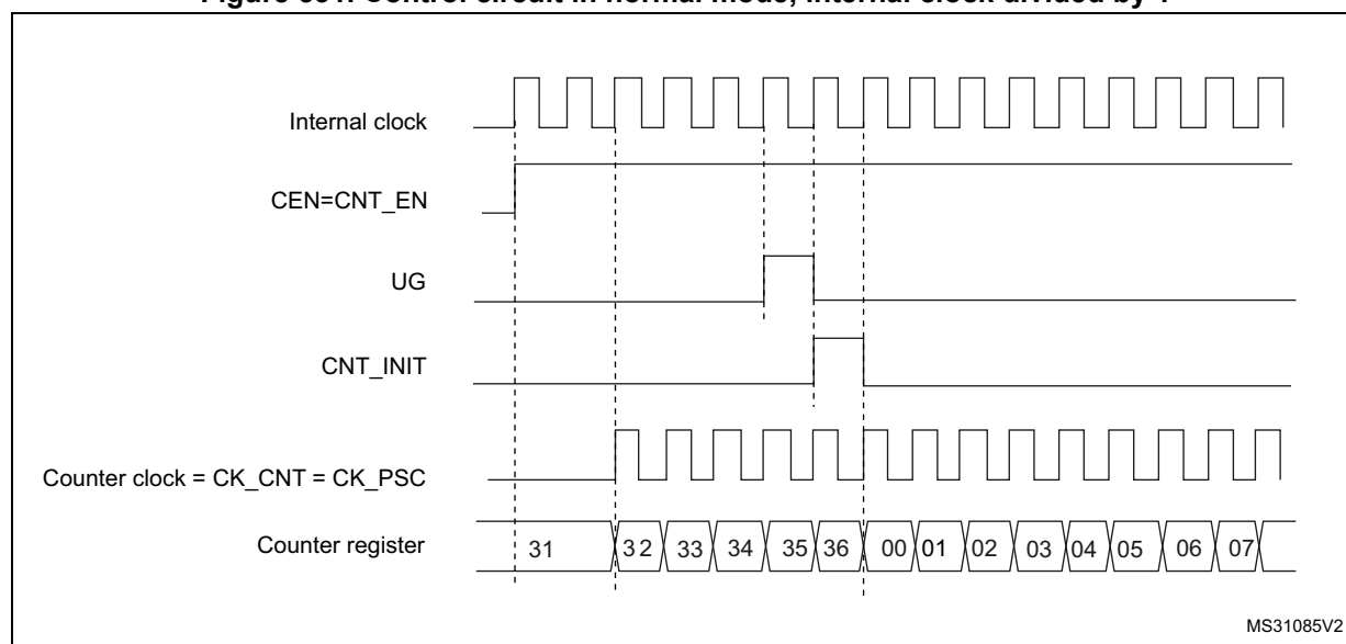
Figure 531. Control circuit in normal mode, internal clock divided by 1
