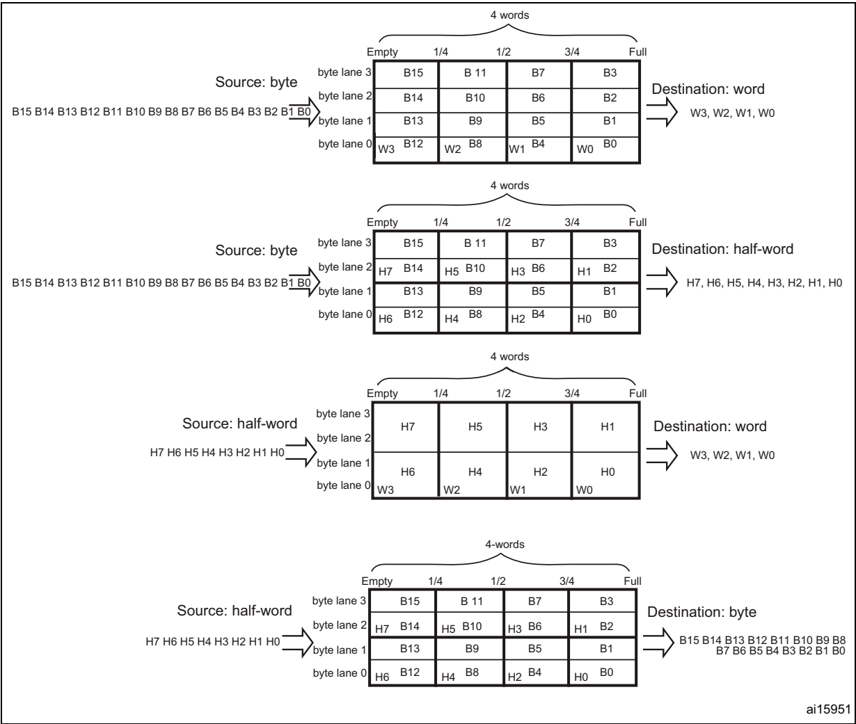
Figure 134. FIFO structure
