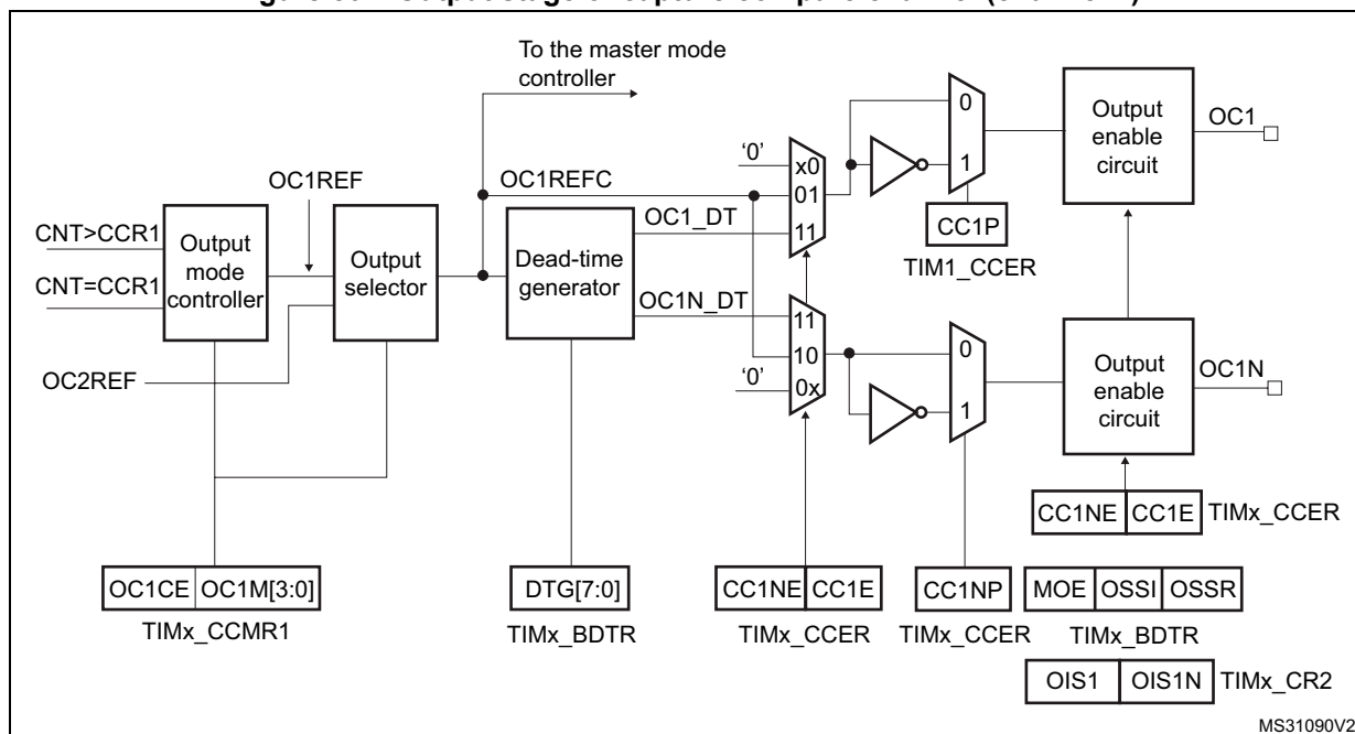
Figure 504. Output stage of capture/compare channel (channel 1)
