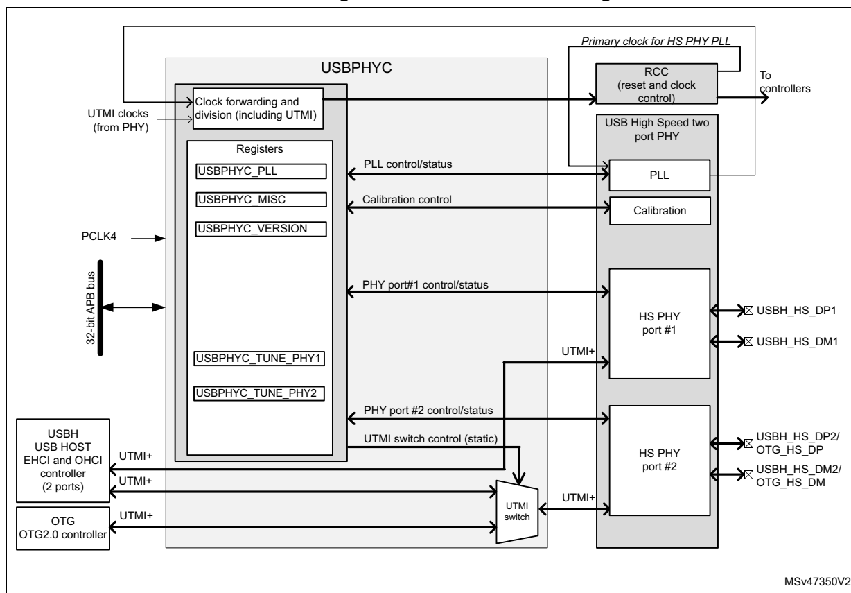
Figure 764. USBPHYC block diagram
