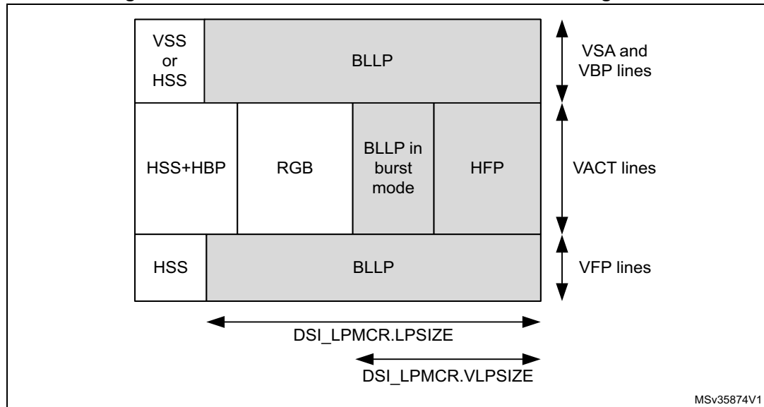
Figure 308. Location of LPSIZE and VLPSIZE in the image area
