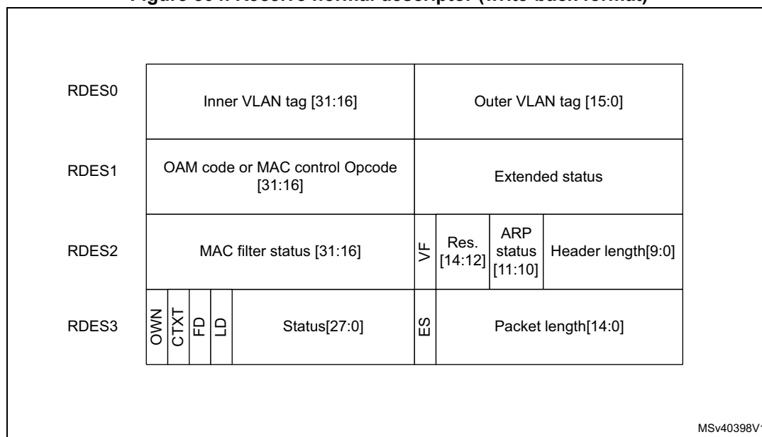
Figure 804. Receive normal descriptor (write-back format)
