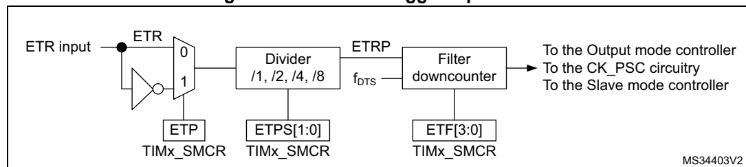
Figure 374. External trigger input block
