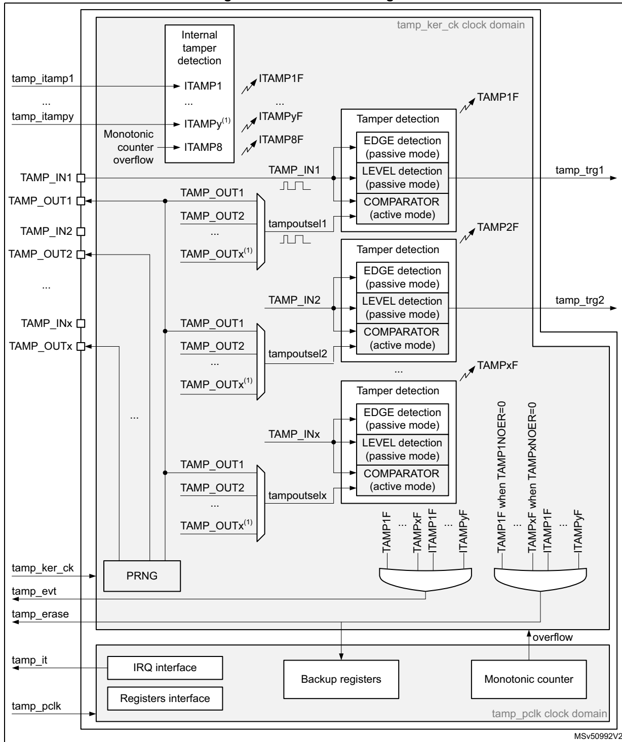
Figure 550. TAMP block diagram
