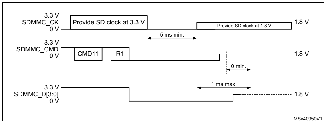
Figure 717. CMD11 signal voltage switch sequence
