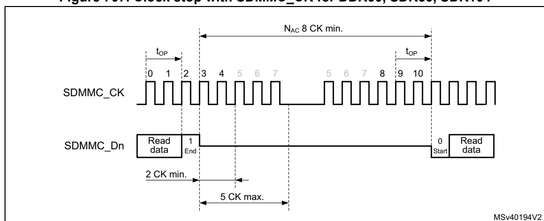
Figure 707. Clock stop with SDMMC_CK for DDR50, SDR50, SDR104
