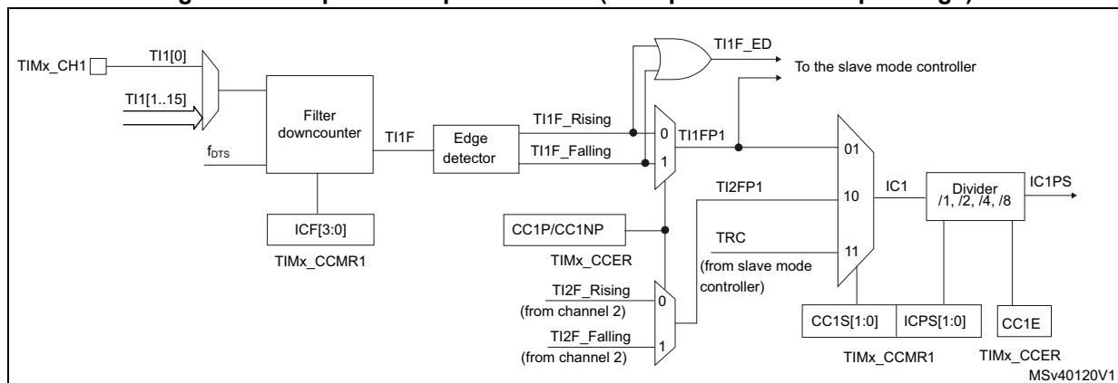
Figure 438. Capture/Compare channel (example: channel 1 input stage)
