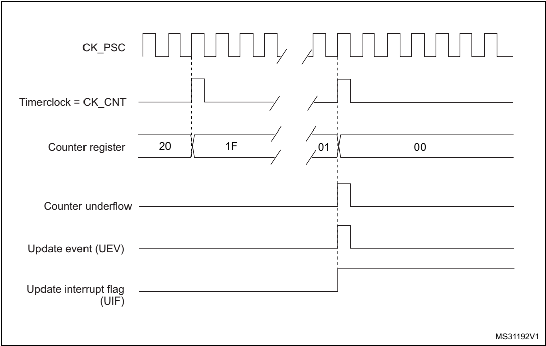
Figure 430. Counter timing diagram, internal clock divided by N
