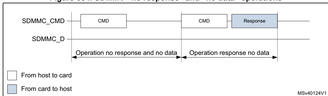
Figure 684. SDMMC “no response” and “no data” operations
