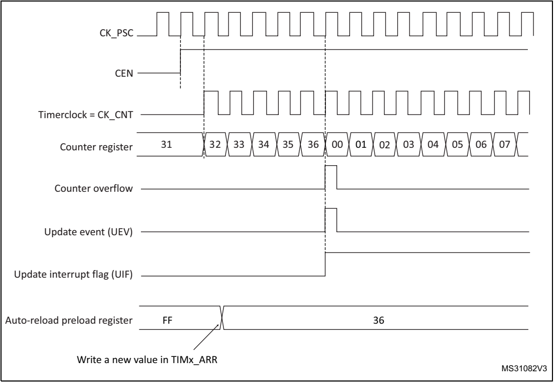
Figure 360. Counter timing diagram, update event when ARPE=0 (TIMx_ARR not preloaded)
