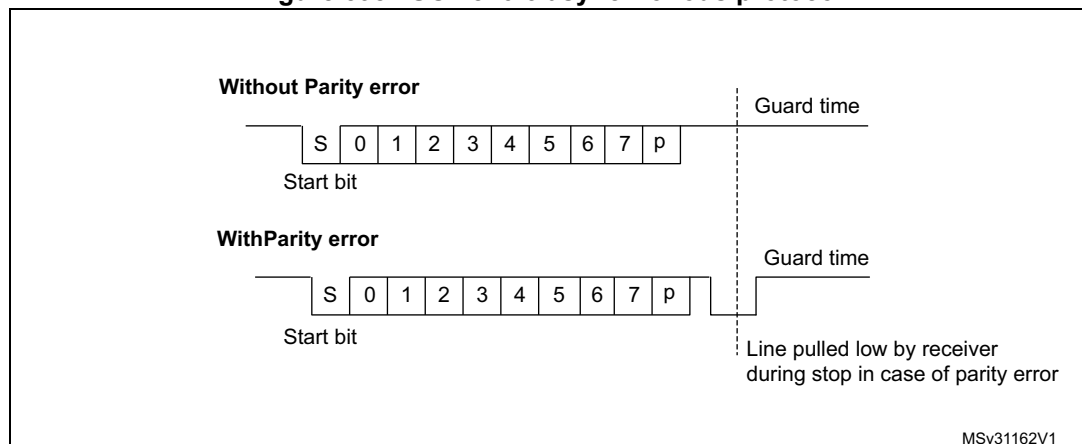
Figure 598. ISO 7816-3 asynchronous protocol
