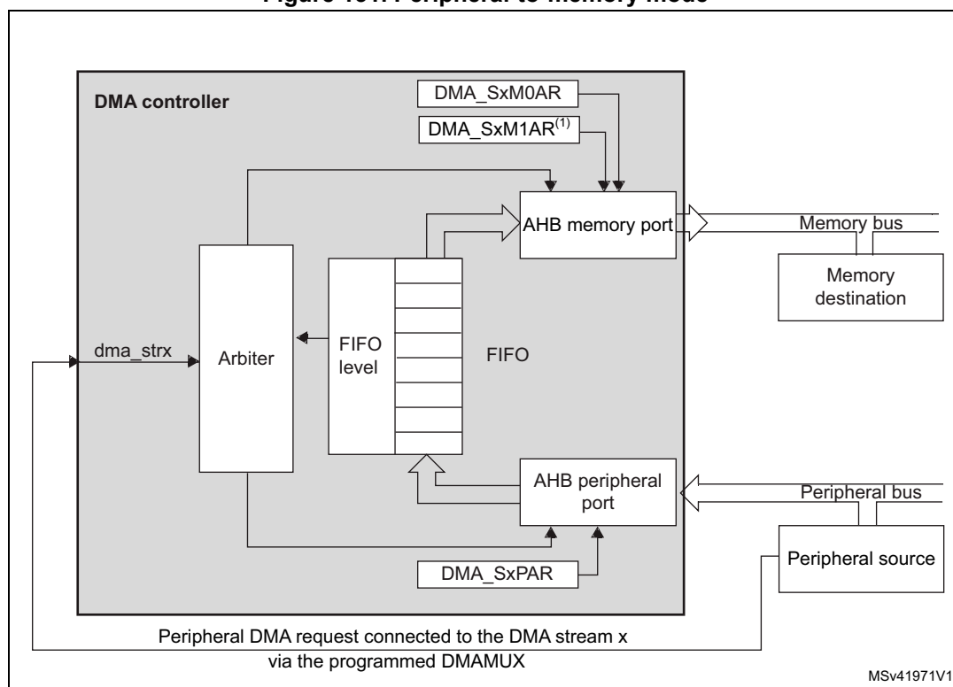
Figure 131. Peripheral-to-memory mode
