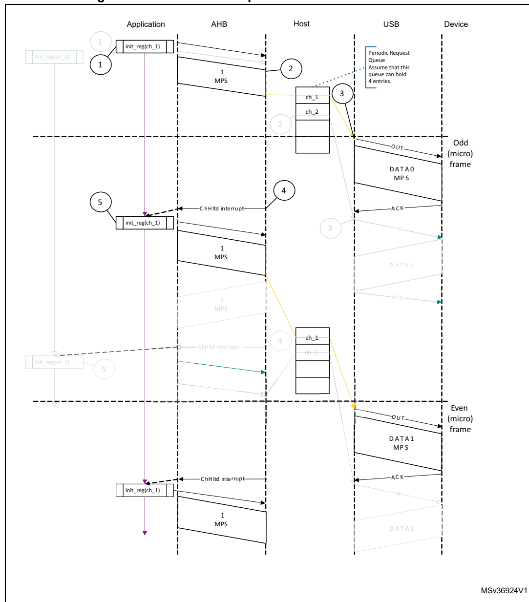
Figure 752. Normal interrupt OUT transactions - DMA mode
