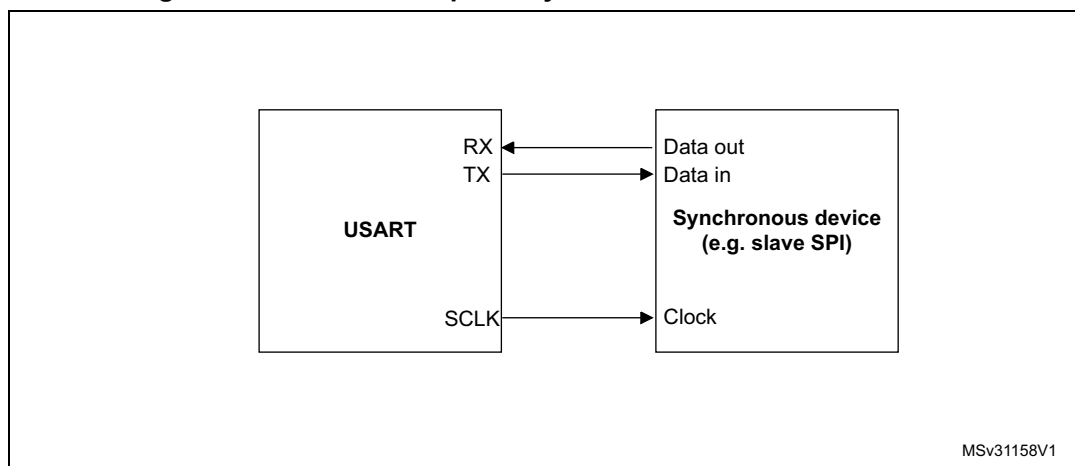
Figure 594. USART example of synchronous master transmission
