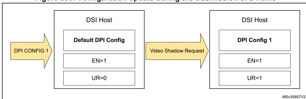
Figure 290. Configuration update during the transmission of a frame
