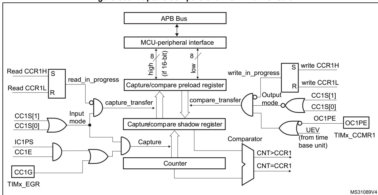
Figure 503. Capture/compare channel 1 main circuit
