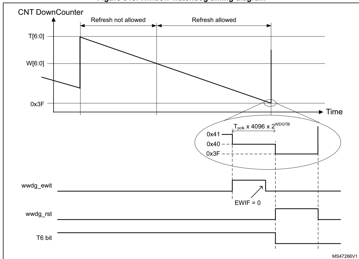
Figure 548. Window watchdog timing diagram
