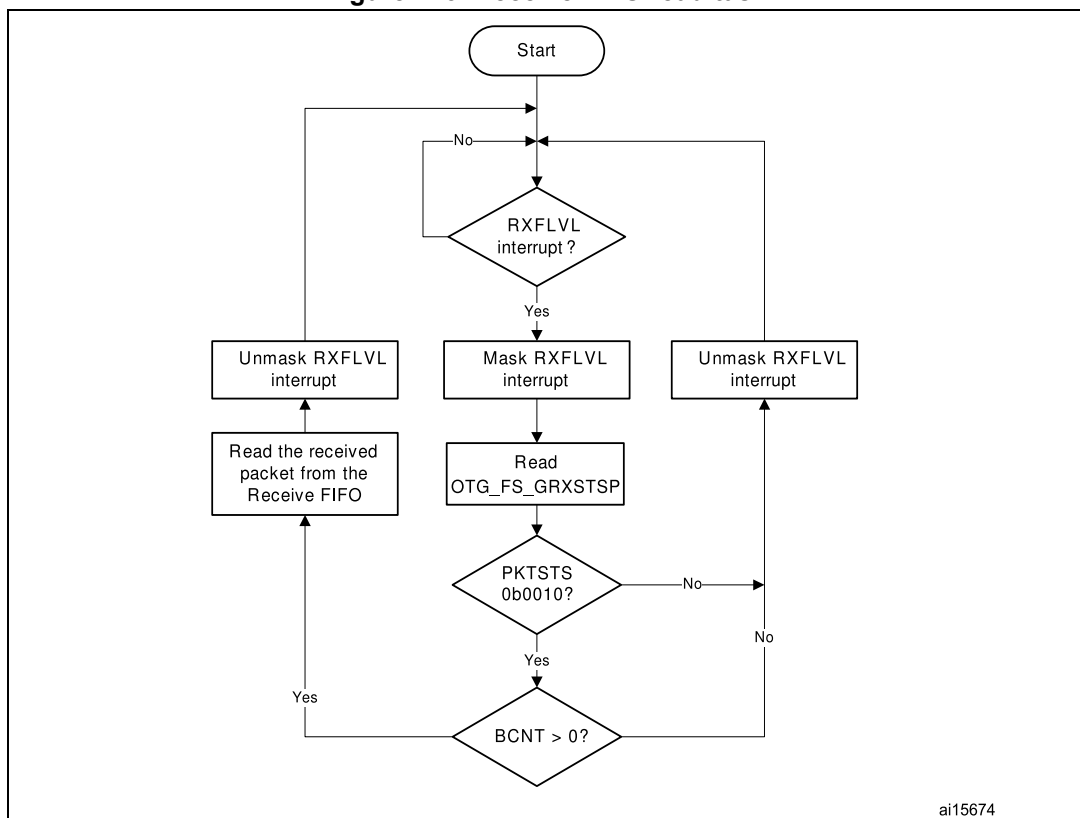
Figure 743. Receive FIFO read task
