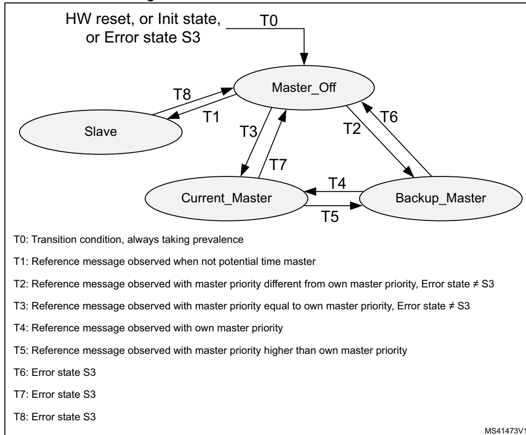
Figure 735. Level 0 master to slave relation
