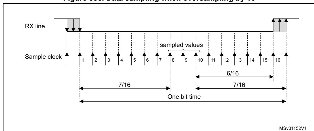
Figure 588. Data sampling when oversampling by 16
