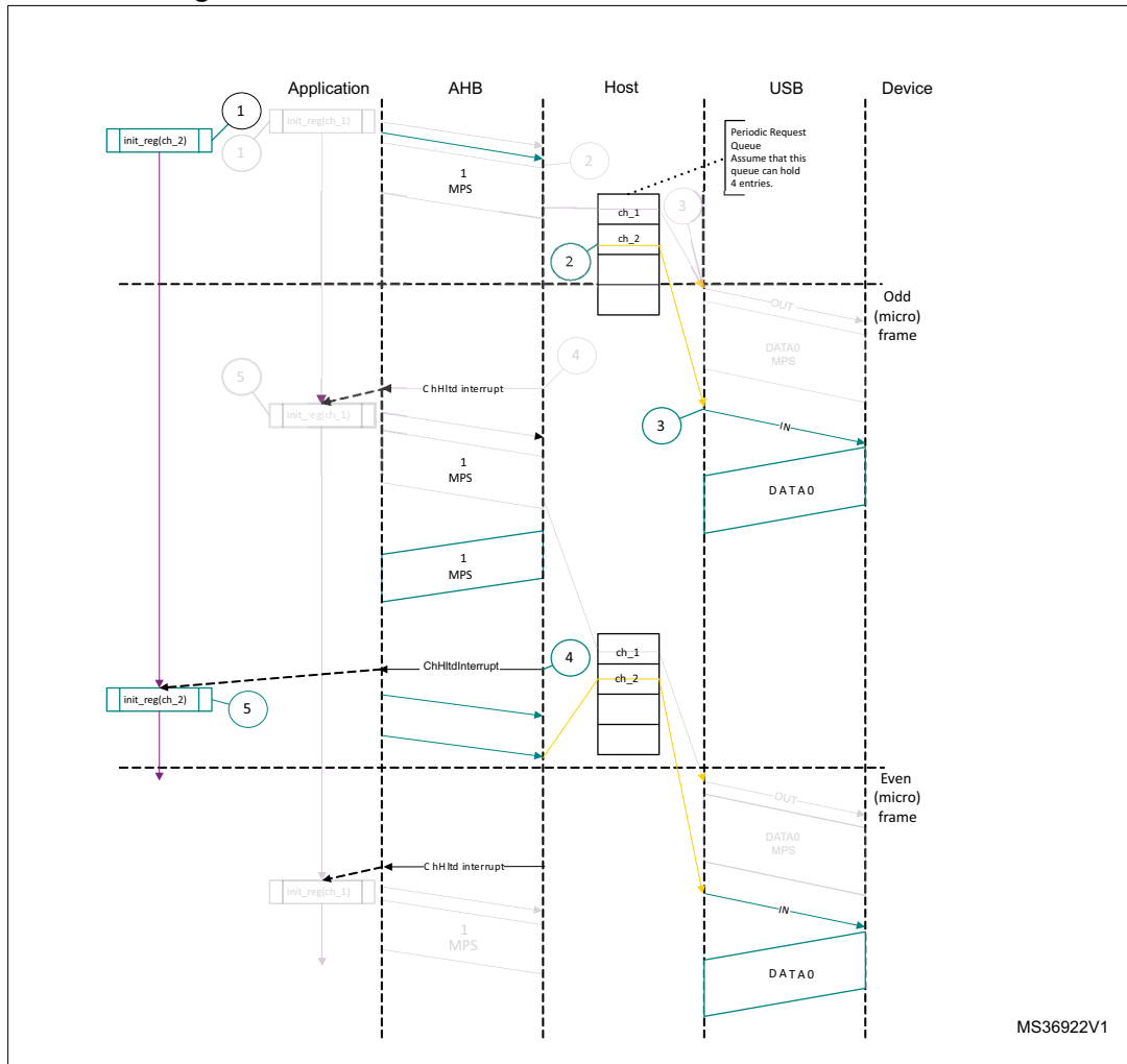
Figure 755. Normal isochronous IN transactions - DMA mode
