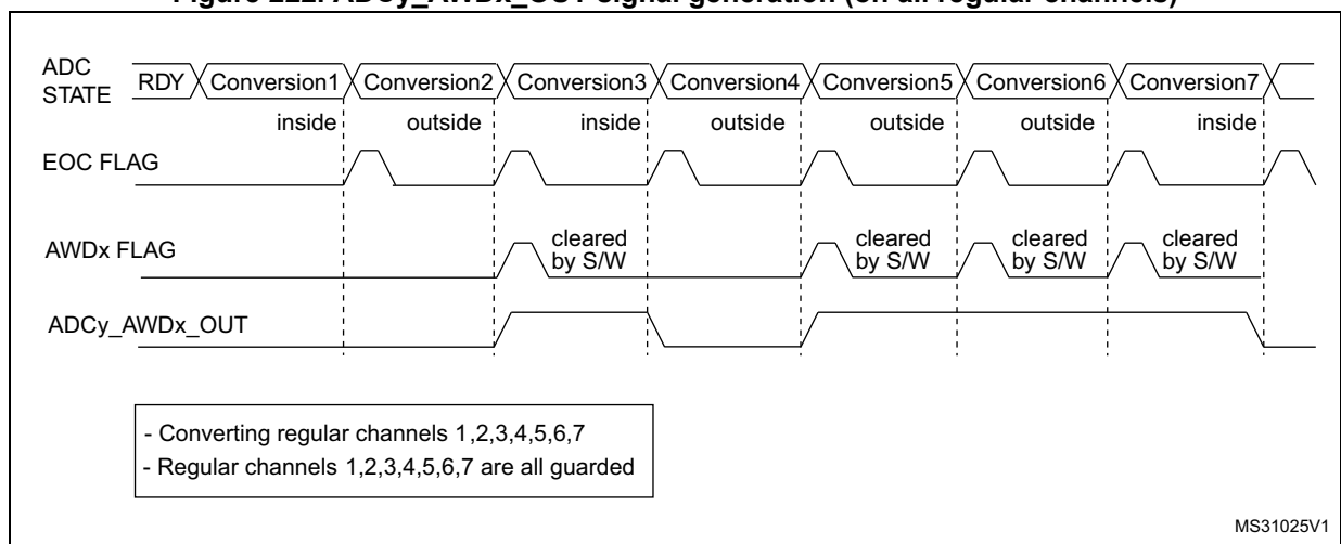
Figure 222. ADCy_AWDx_OUT signal generation (on all regular channels)
