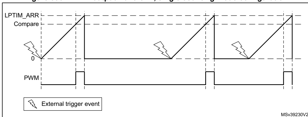
Figure 536. LPTIM output waveform, single counting mode configuration
