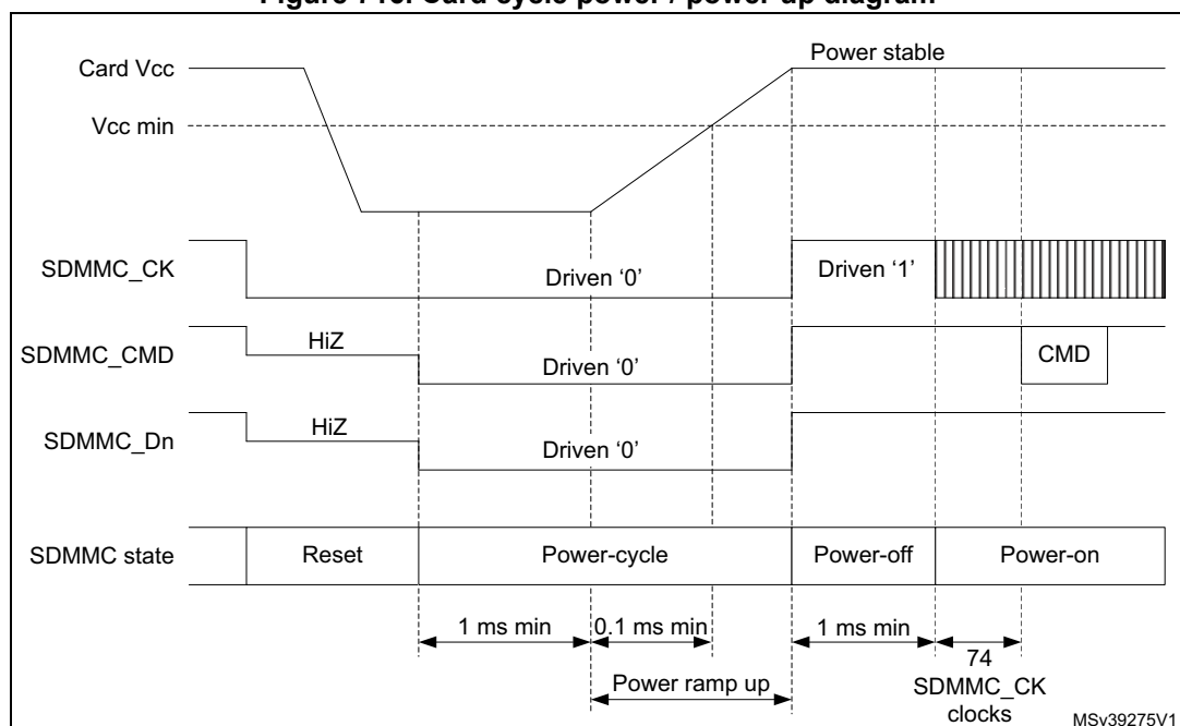
Figure 716. Card cycle power / power up diagram
