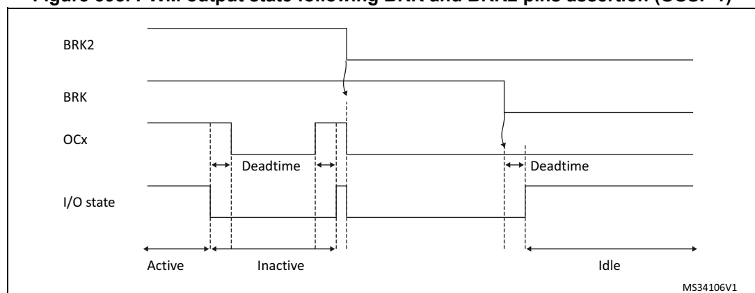
Figure 398. PWM output state following BRK and BRK2 pins assertion (OSSl=1)
