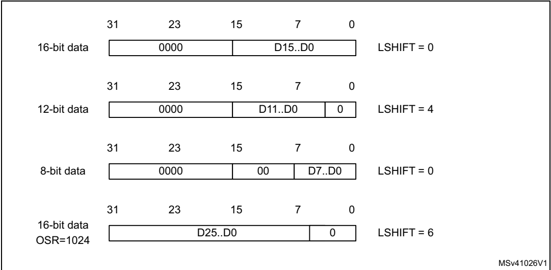
Figure 212. Left alignment (offset disabled, unsigned value)
