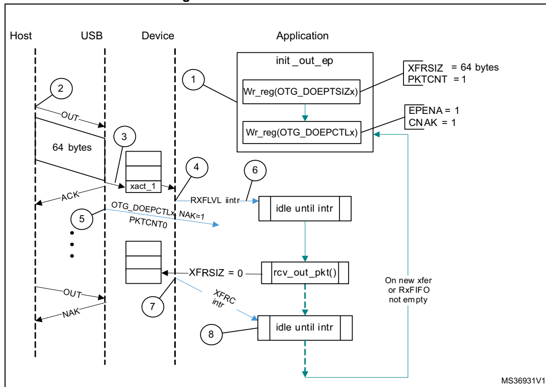
Figure 758. Bulk OUT transaction
