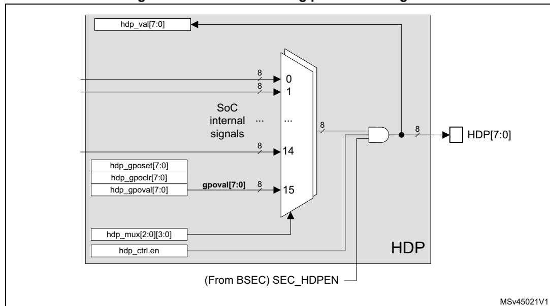
Figure 807. Hardware debug port block diagram
