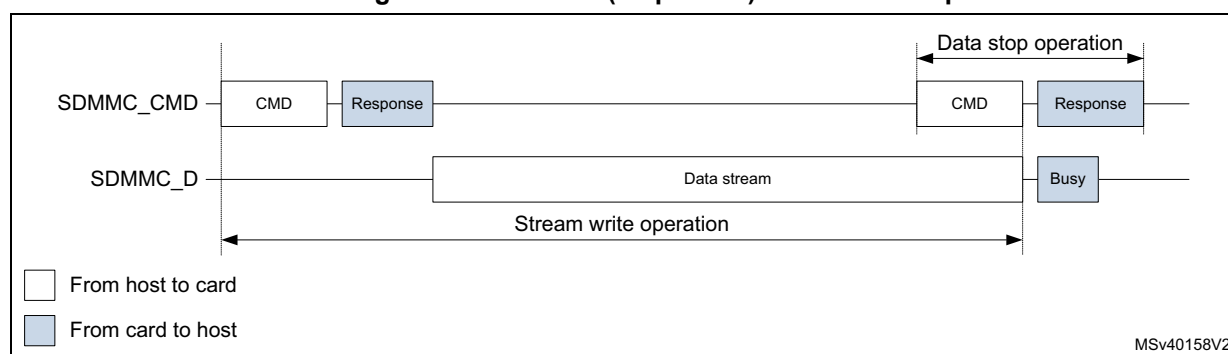
Figure 688. SDMMC (sequential) stream write operation
