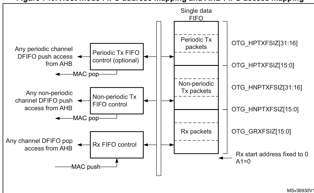
Figure 740. Host-mode FIFO address mapping and AHB FIFO access mapping
