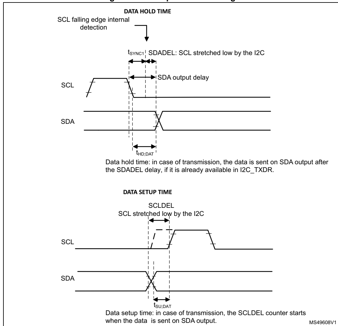
Figure 554. Setup and hold timings
