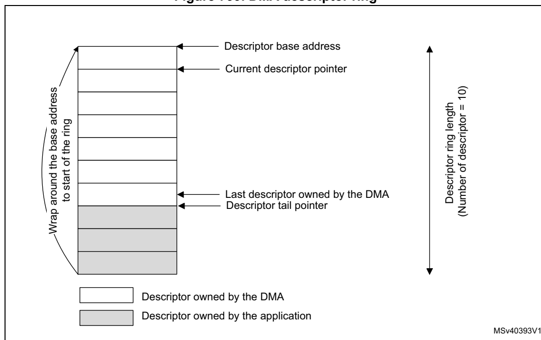
Figure 799. DMA descriptor ring
