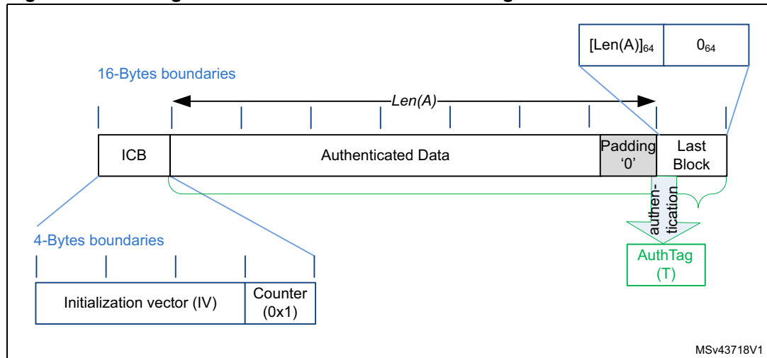
Figure 349. Message construction for the Galois Message Authentication Code mode
