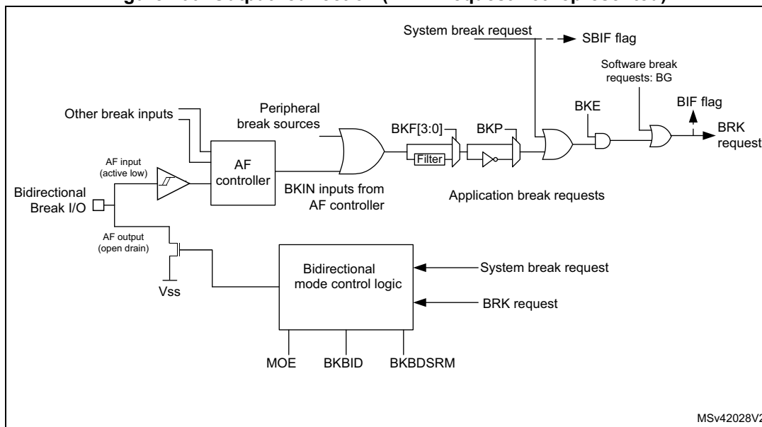
Figure 400. Output redirection (BRK2 request not represented)
