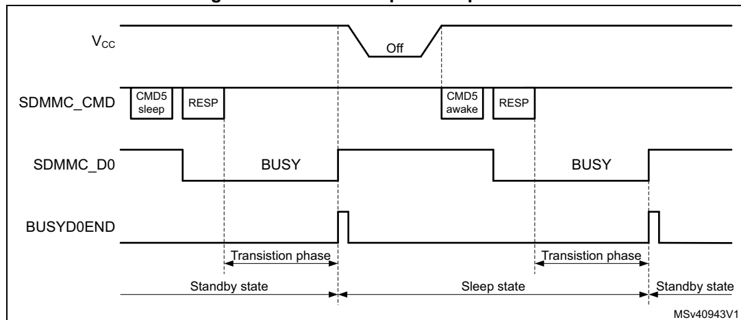
Figure 711. CMD5 Sleep Awake procedure
