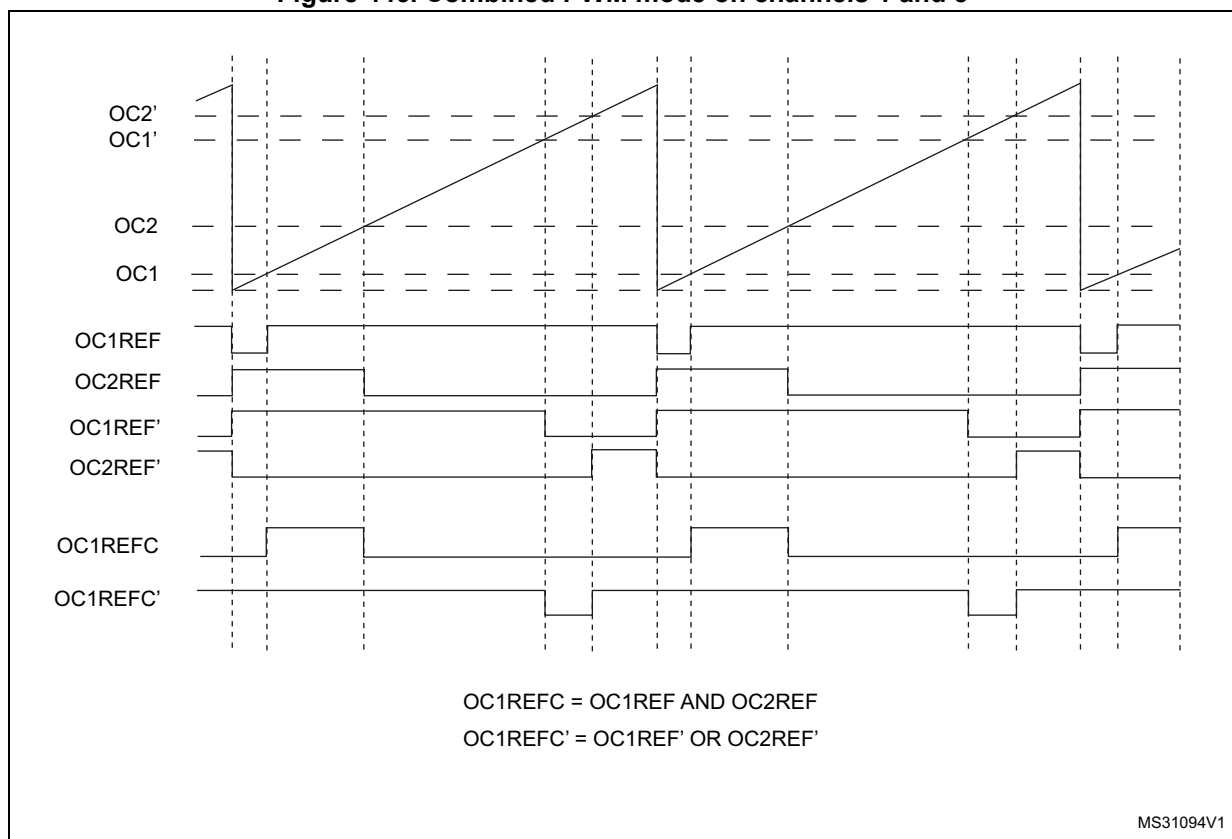
Figure 446. Combined PWM mode on channels 1 and 3
