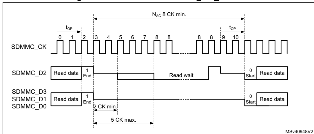
Figure 709. ReadWait with SDMMC_CK \geq 50 MHz
