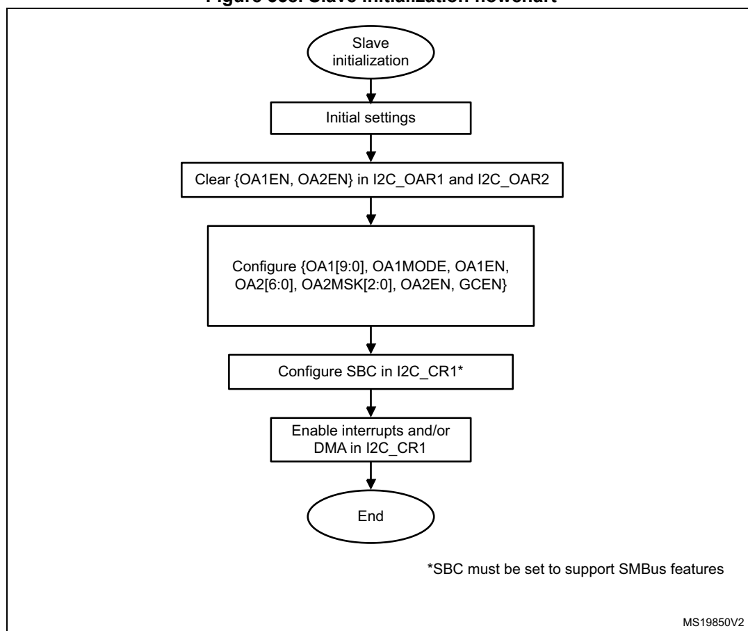
Figure 558. Slave initialization flowchart
