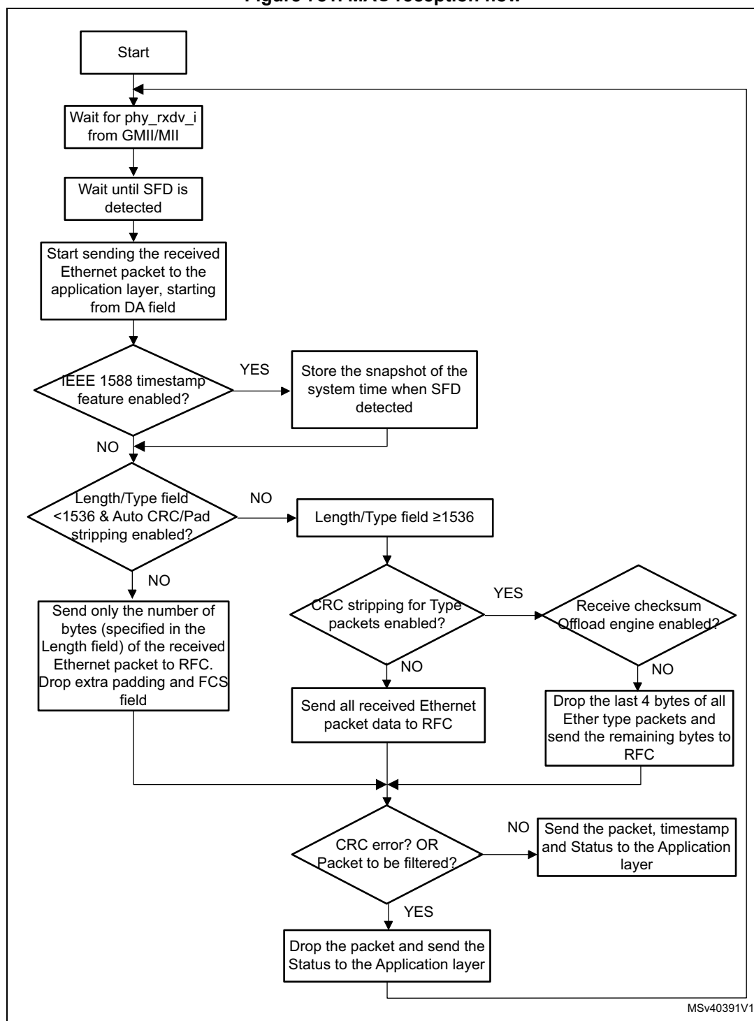
Figure 781. MAC reception flow
