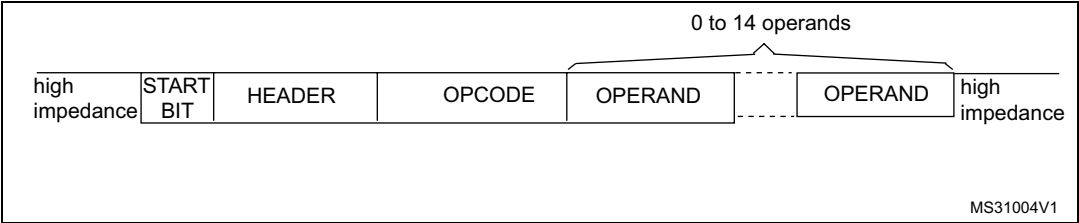
Figure 767. Message structure
