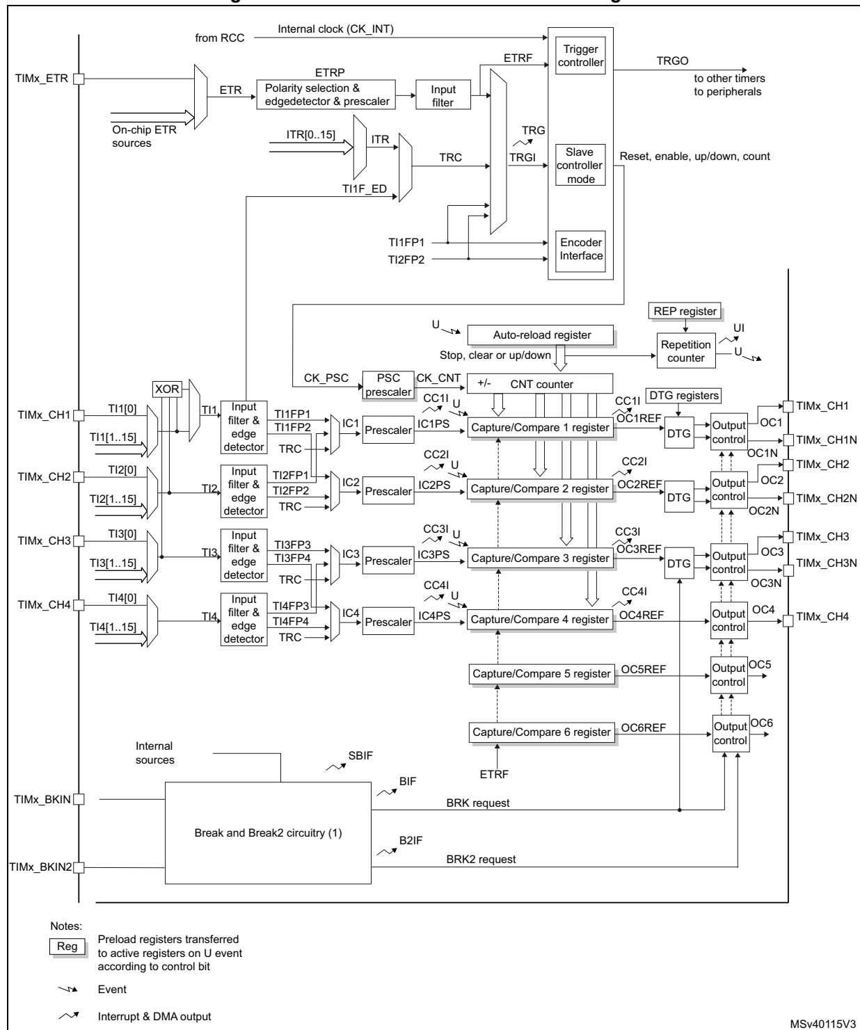
Figure 353. Advanced-control timer block diagram
