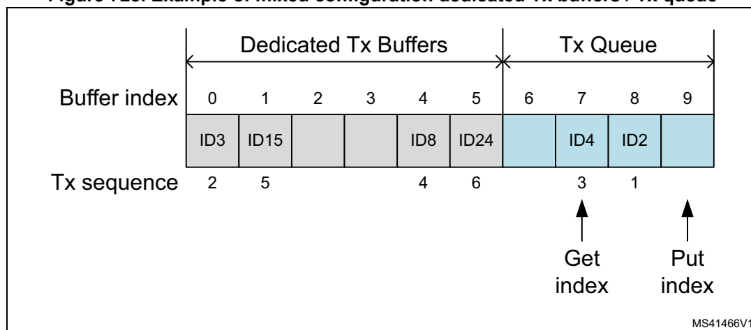
Figure 728. Example of mixed configuration dedicated Tx buffers / Tx queue
