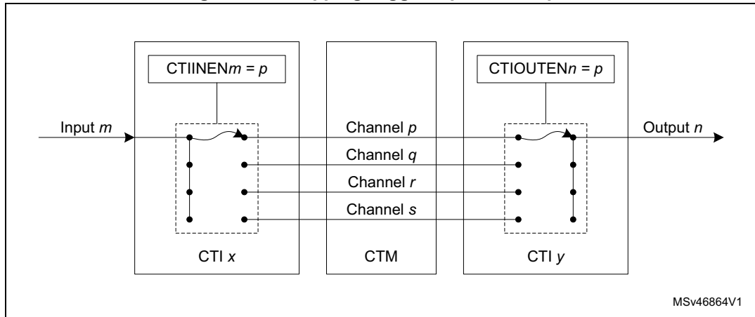
Figure 816. Mapping trigger inputs to outputs
