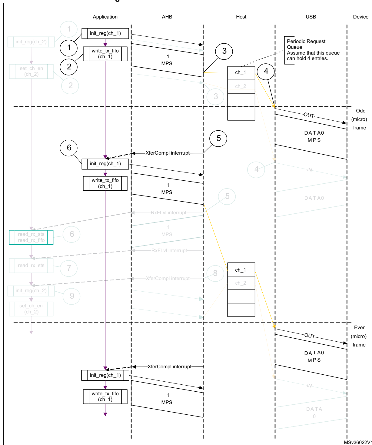
Figure 748. Isochronous OUT transactions
