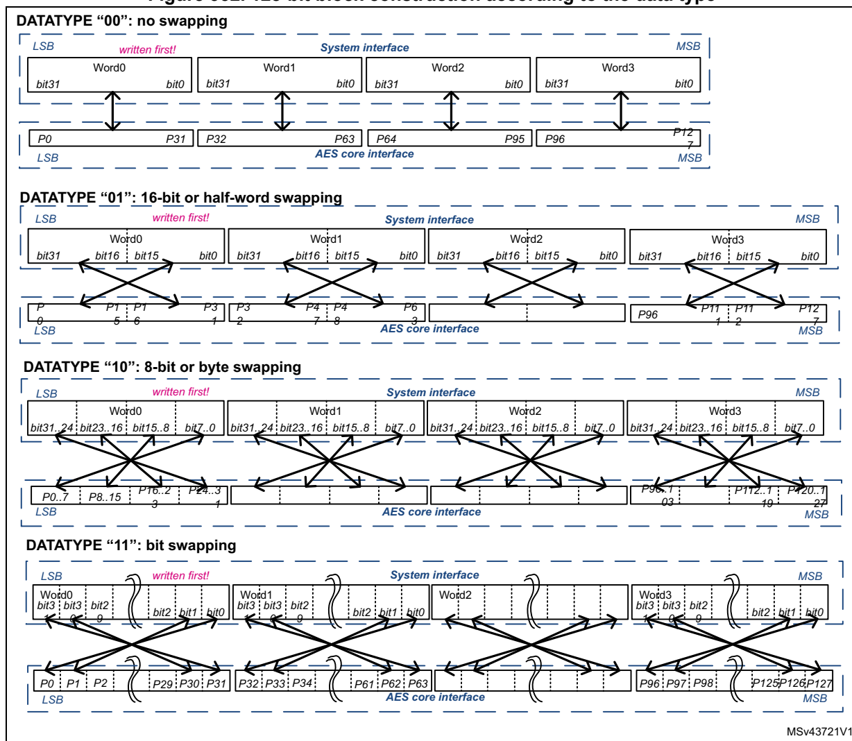
Figure 352. 128-bit block construction according to the data type
