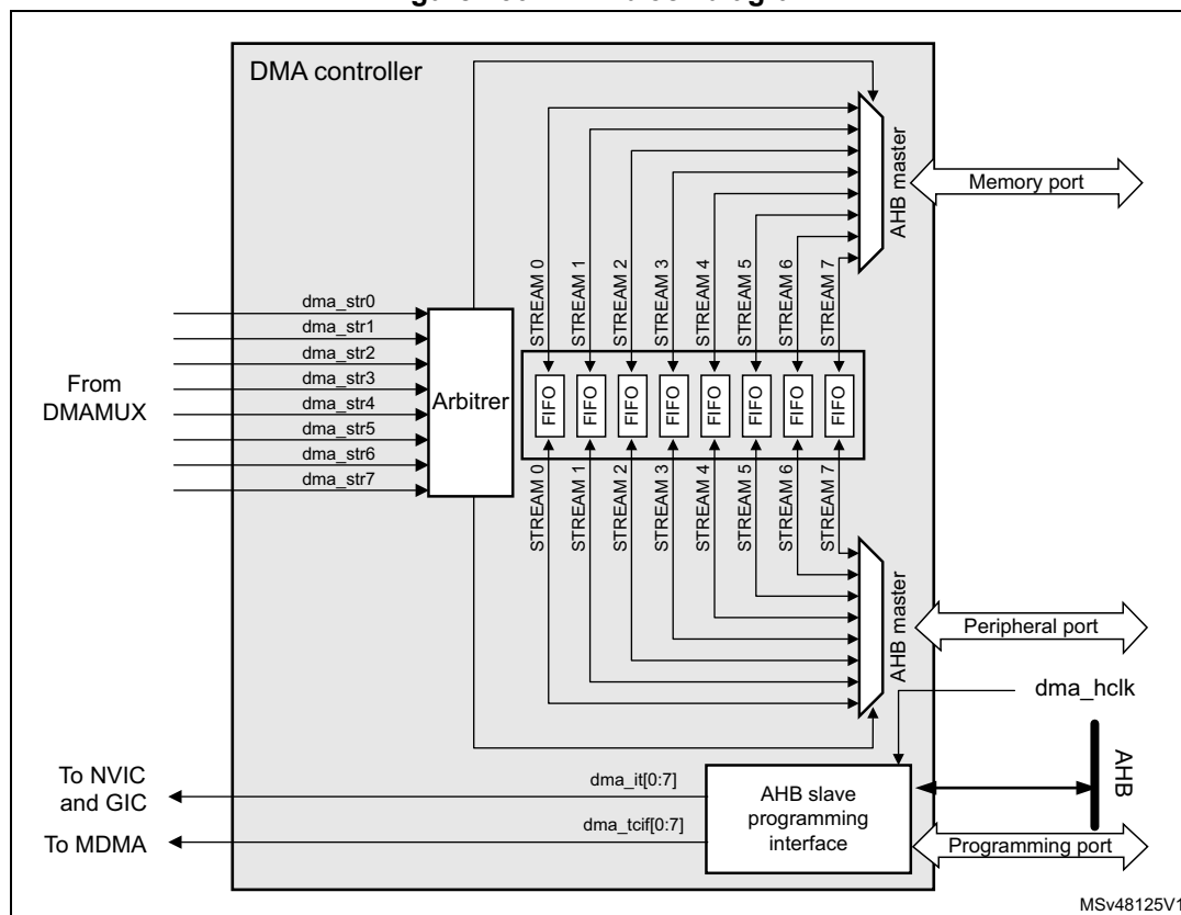
Figure 130. DMA block diagram
