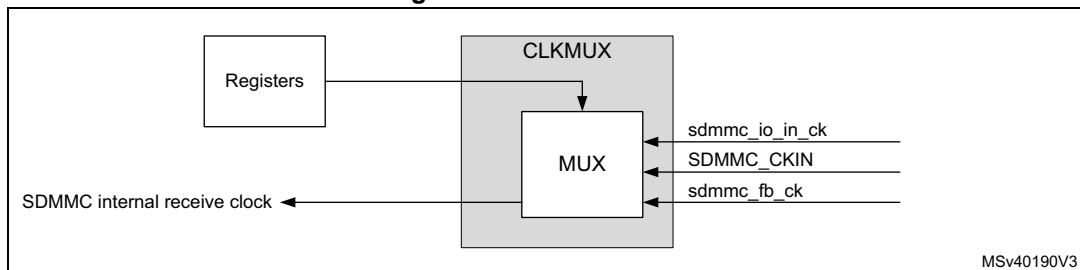
Figure 698. CLKMUX unit
