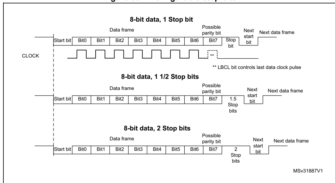
Figure 584. Configurable stop bits
