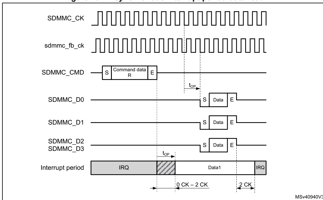
Figure 704. Asynchronous interrupt period data read
