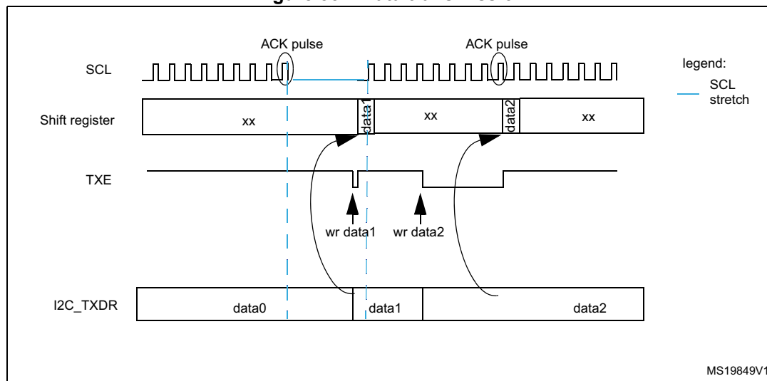
Figure 557. Data transmission
