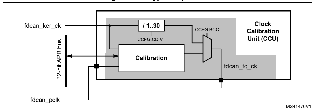
Figure 730. Bypass operation
