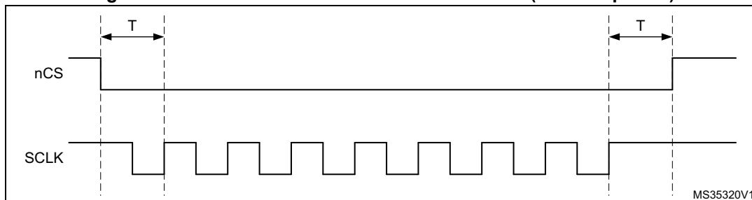
Figure 177. nCS when CKMODE = 1 in SDR mode ( T = \text{CLK period} )
