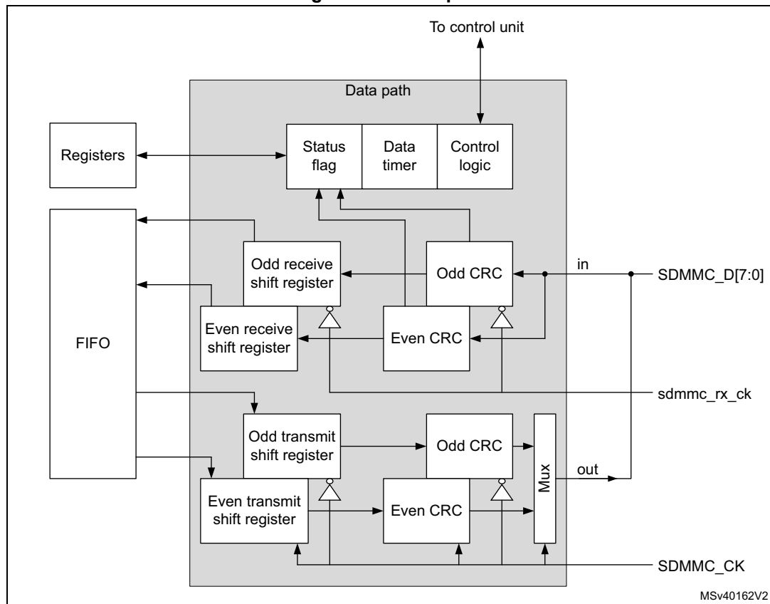
Figure 694. Data path
