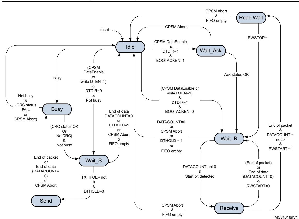
Figure 697. Data path state machine (DPSM)
