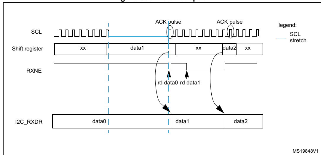
Figure 556. Data reception
