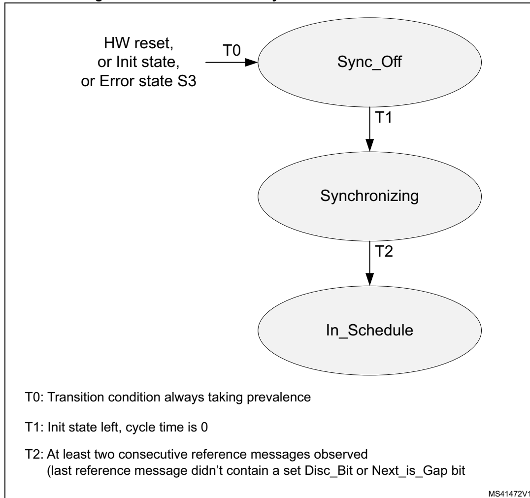
Figure 734. Level 0 schedule synchronization state machine
