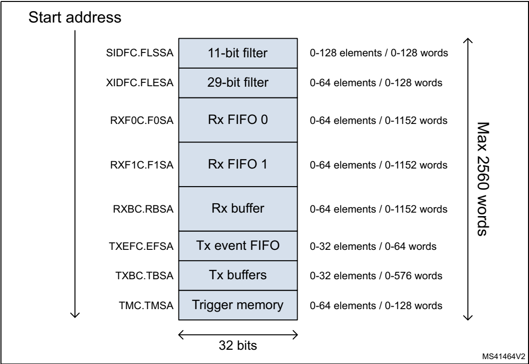
Figure 724. Message RAM configuration
