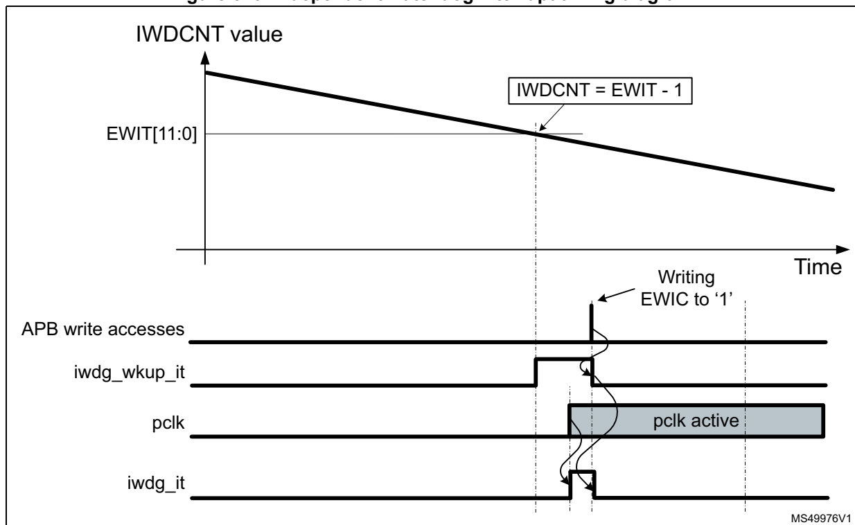
Figure 546. Independent watchdog interrupt timing diagram
