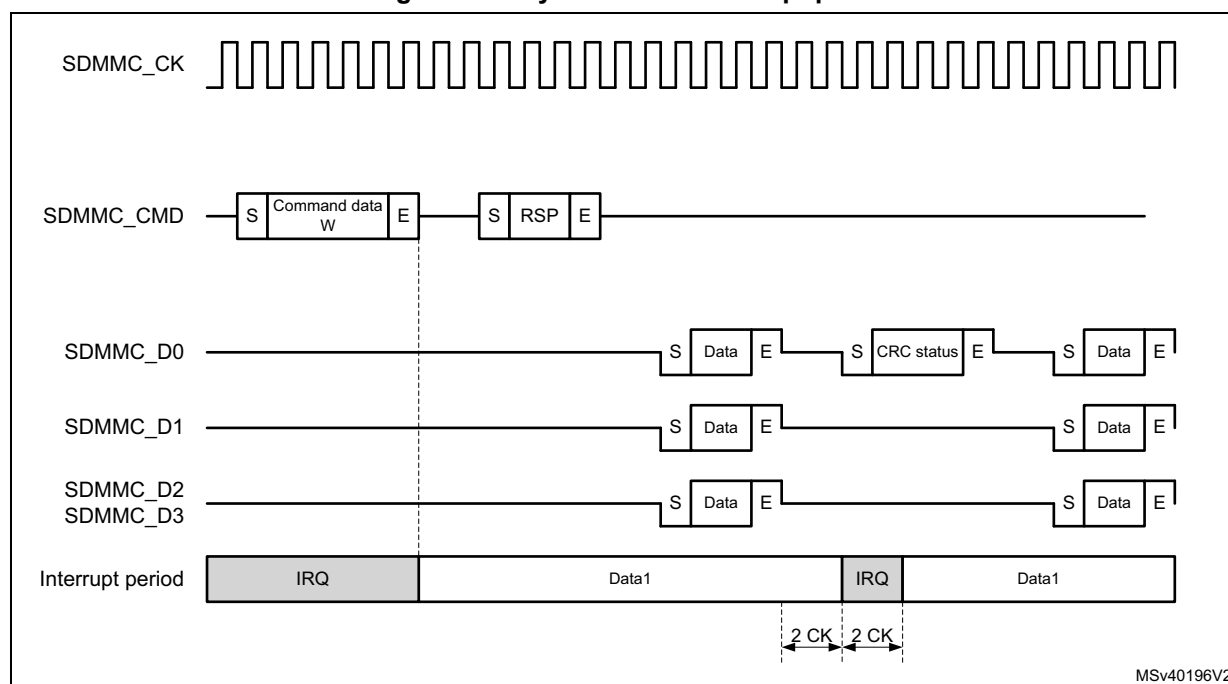
Figure 703. Synchronous interrupt period data write
