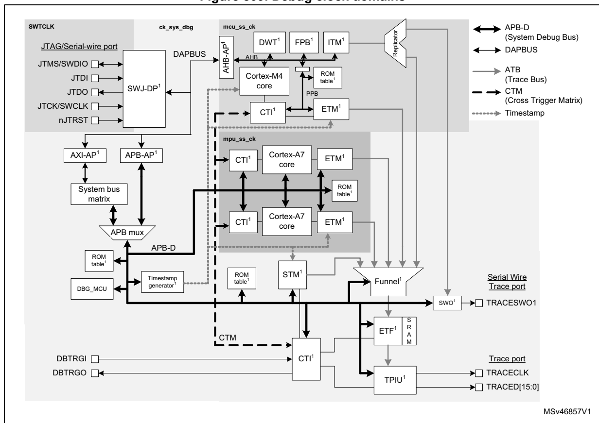
Figure 809. Debug clock domains
