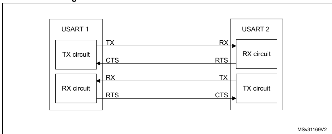
Figure 604. Hardware flow control between 2 USARTs
