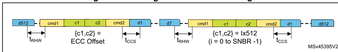
Figure 170. Change read command timings
