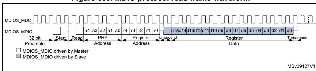
Figure 683. MDIO protocol read frame waveform
