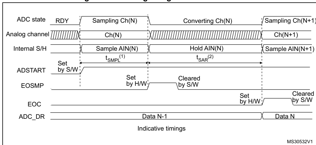
Figure 189. Analog to digital conversion time
