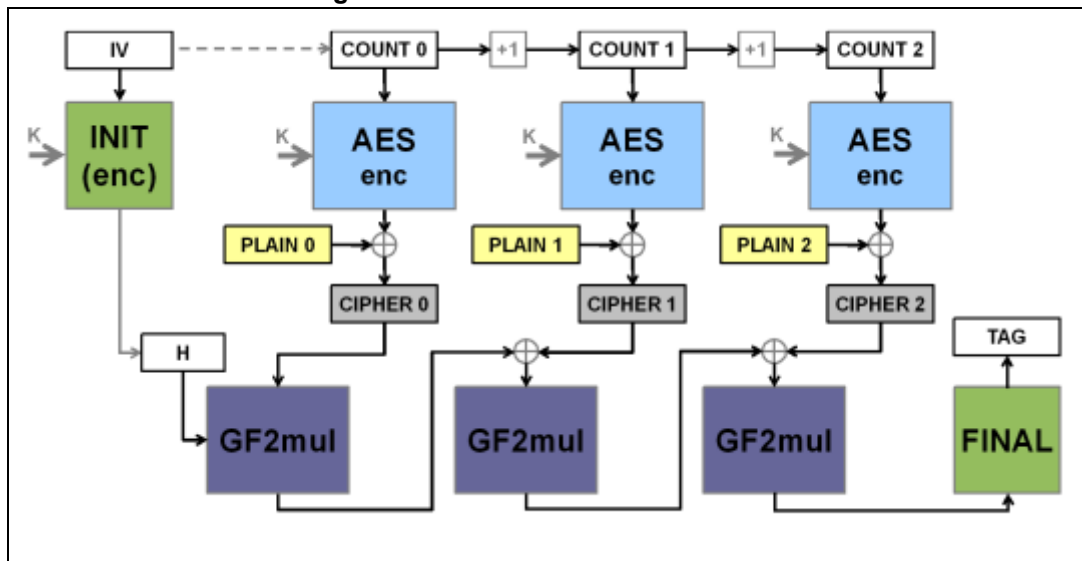
Figure 333. AES-GCM mode overview
