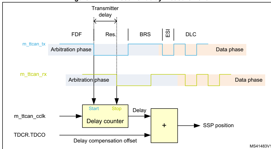
Figure 721. Transceiver delay measurement
