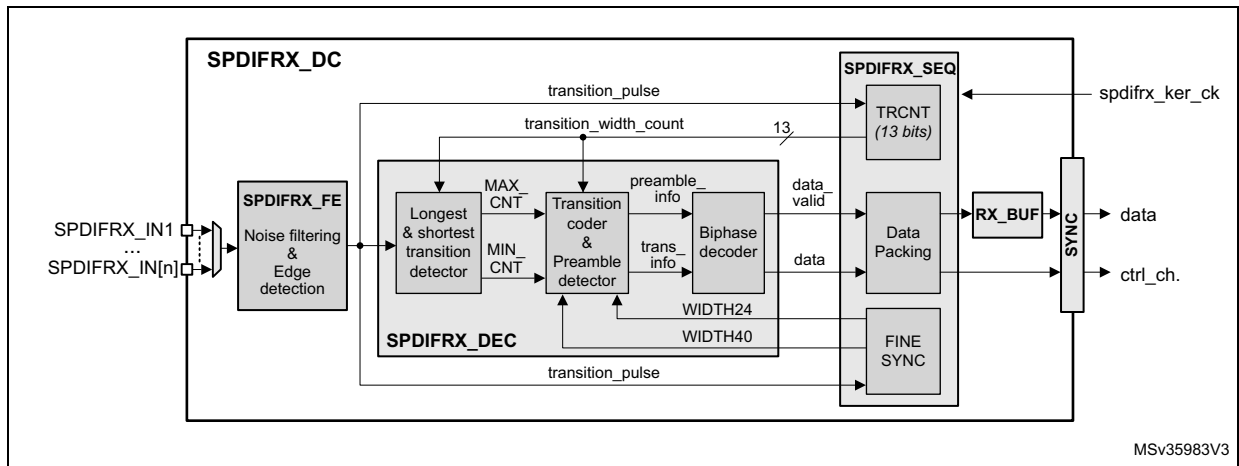
Figure 670. SPDIFRX decoder
