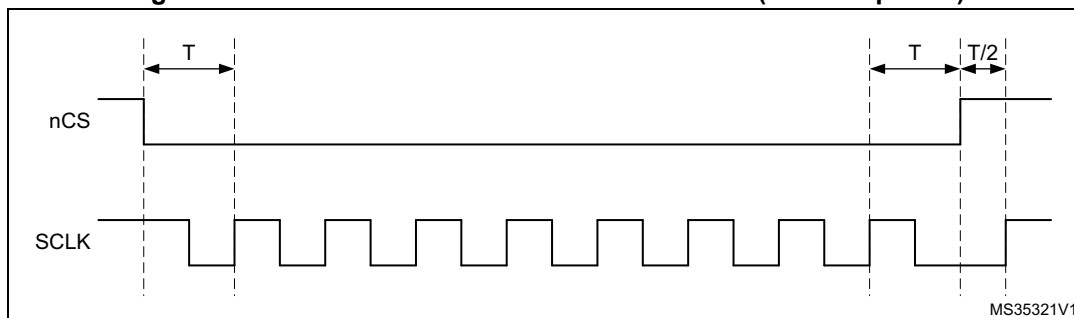
Figure 178. nCS when CKMODE = 1 in DDR mode ( T = \text{CLK period} )
