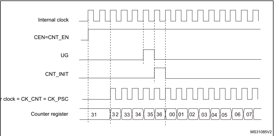
Figure 472. Control circuit in normal mode, internal clock divided by 1
