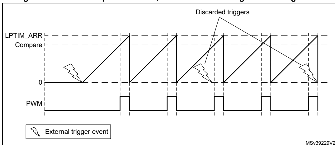
Figure 538. LPTIM output waveform, Continuous counting mode configuration
