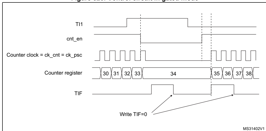
Figure 520. Control circuit in gated mode
