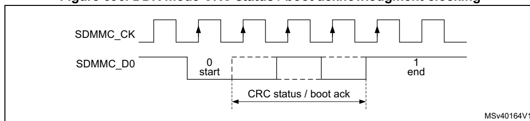
Figure 696. DDR mode CRC status / boot acknowledgment clocking
