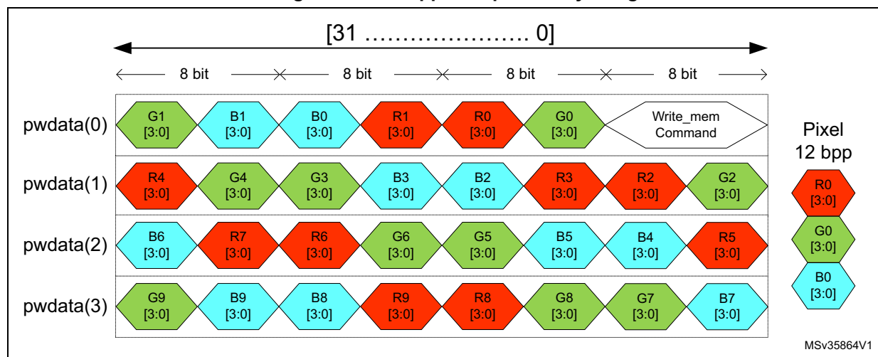
Figure 295. 12 bpp APB pixel to byte organization
