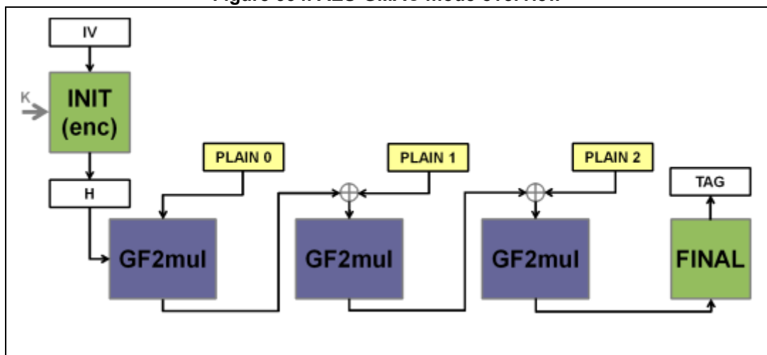
Figure 334. AES-GMAC mode overview
