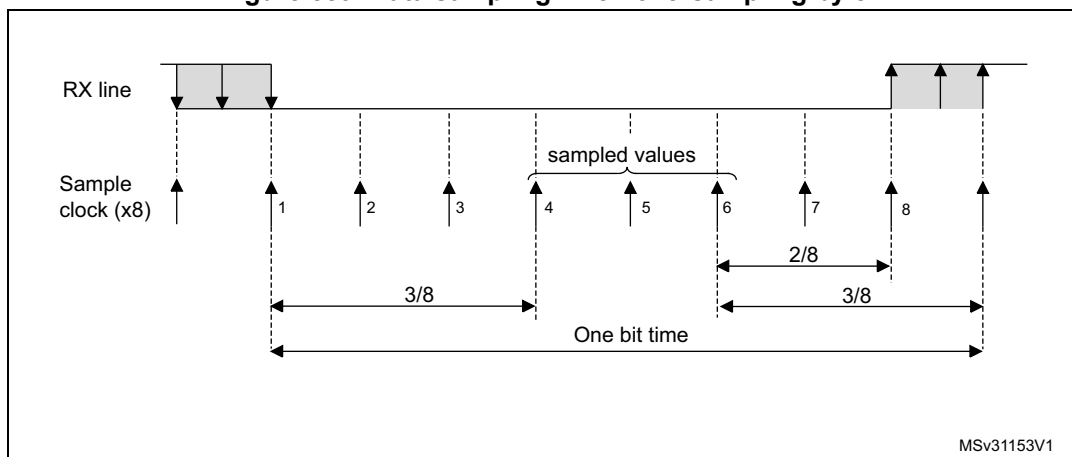
Figure 589. Data sampling when oversampling by 8
