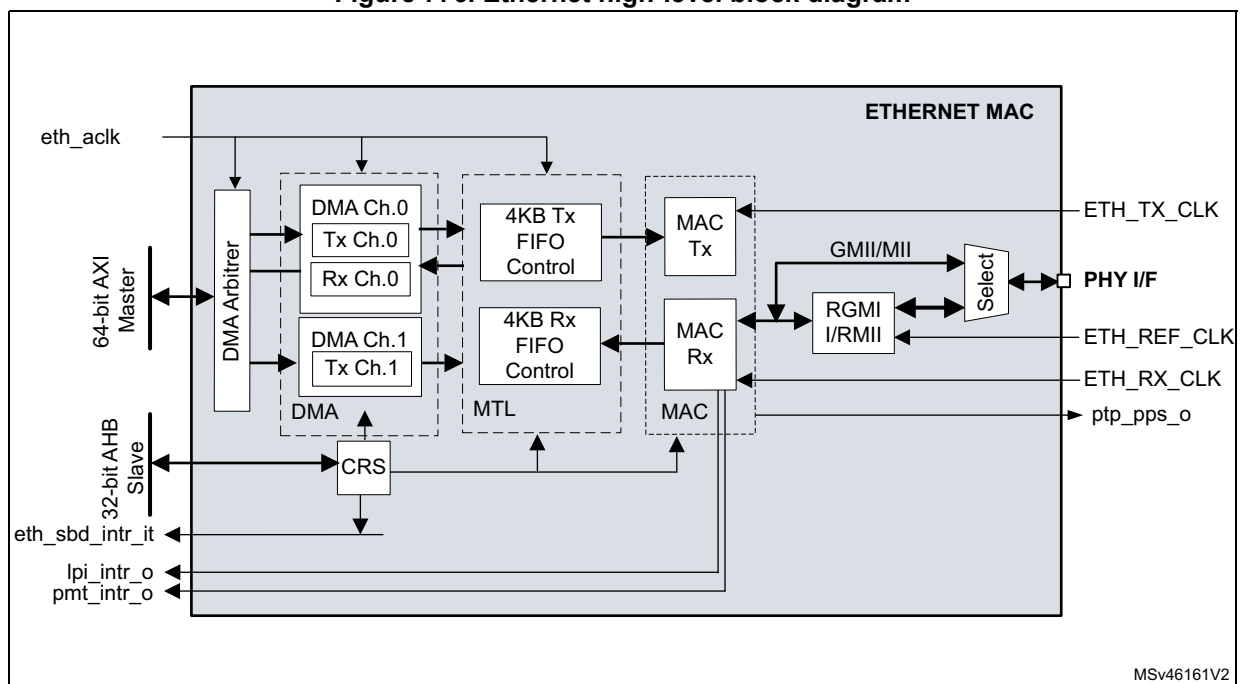
Figure 776. Ethernet high-level block diagram
