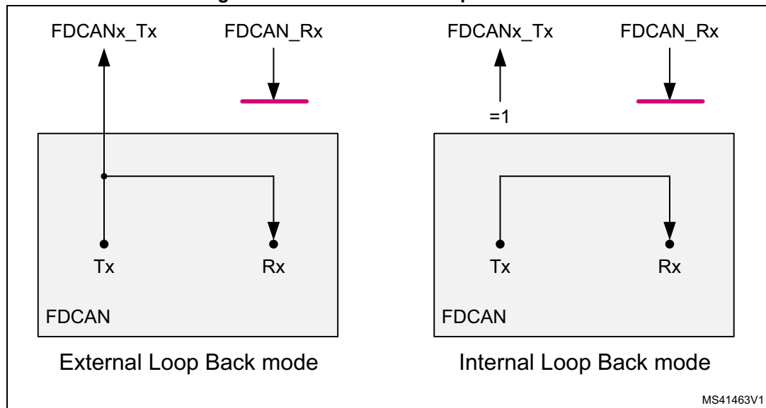
Figure 723. Pin control in loop back mode
