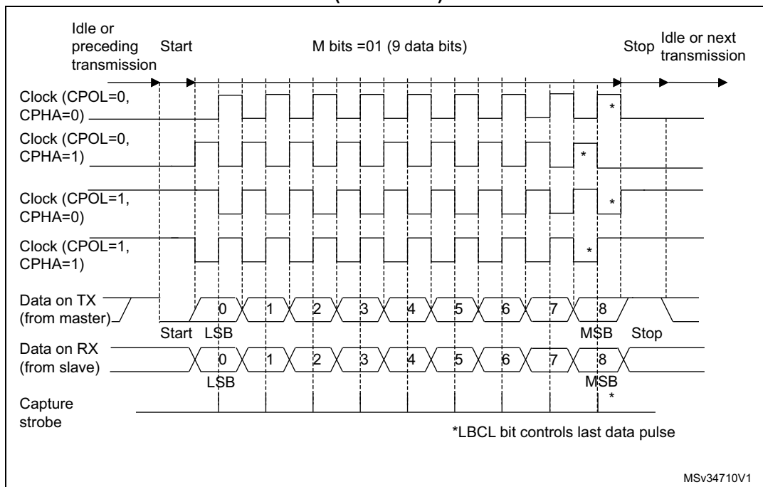
Figure 596. USART data clock timing diagram in synchronous master mode (M bits = 01)
