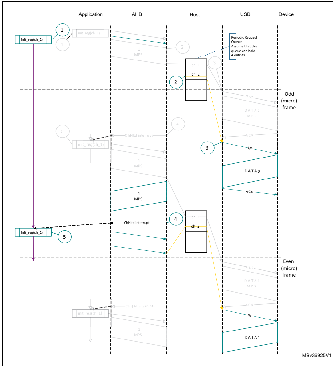
Figure 753. Normal interrupt IN transactions - DMA mode
