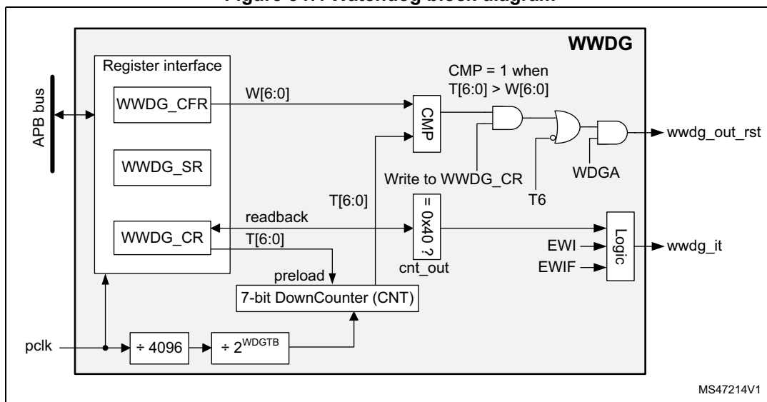
Figure 547. Watchdog block diagram
