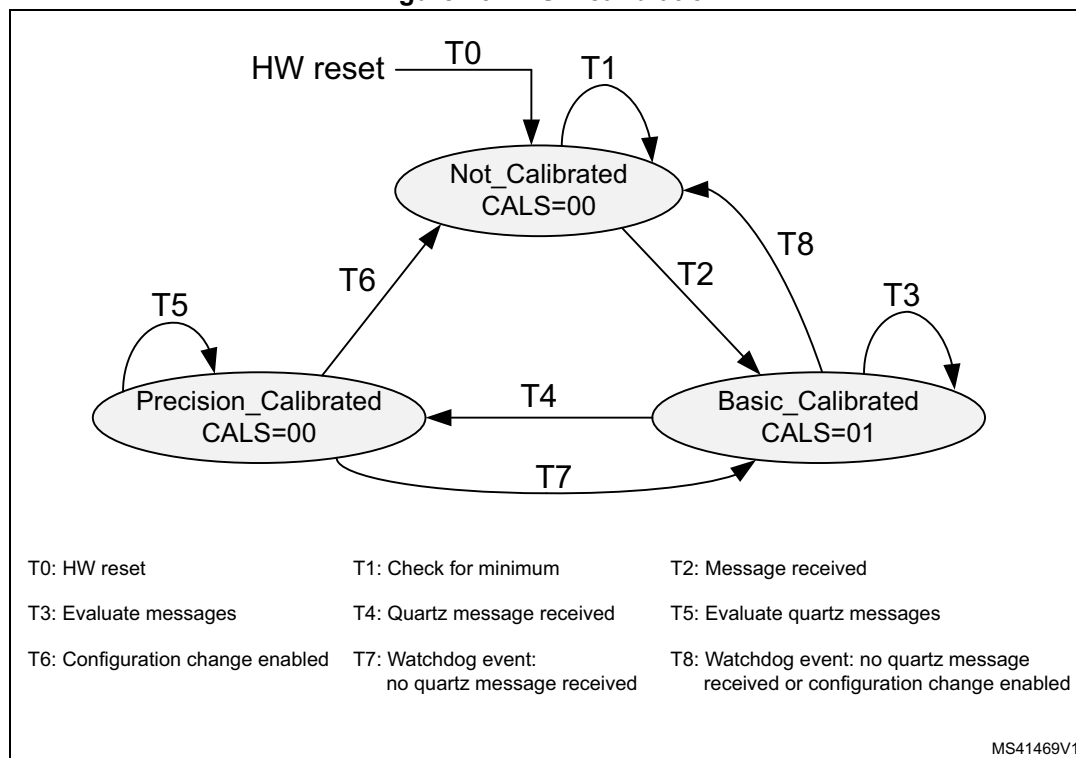
Figure 731. FSM calibration
