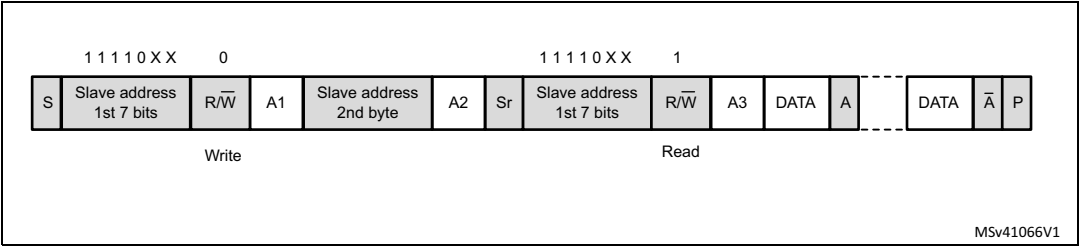
Figure 567. 10-bit address read access with HEAD10R=0
