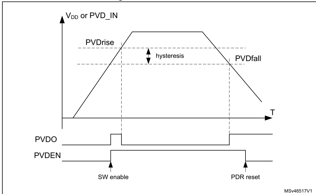
Figure 39. PVD thresholds
