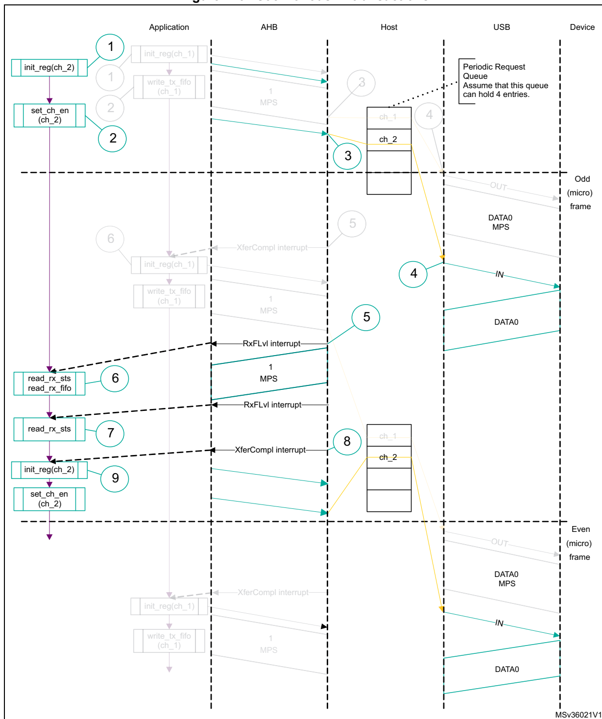
Figure 749. Isochronous IN transactions
