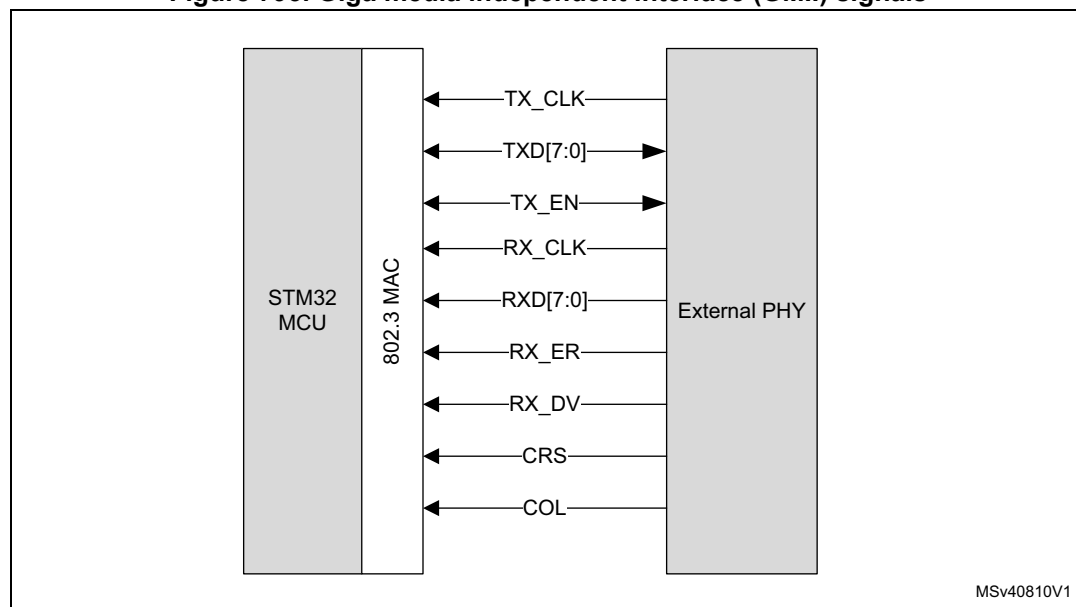
Figure 793. Giga media independent interface (GMII) signals
