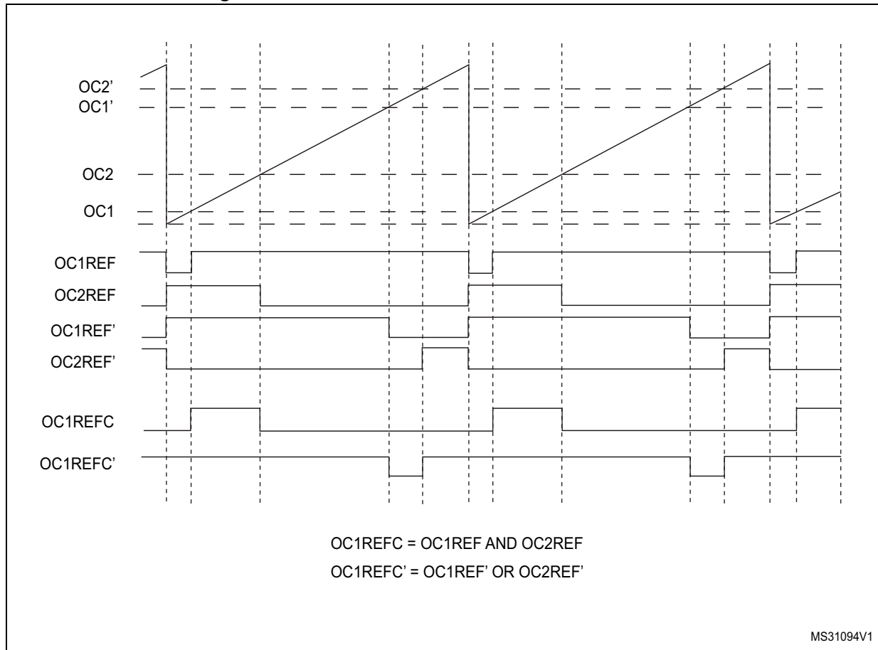
Figure 481. Combined PWM mode on channel 1 and 2
