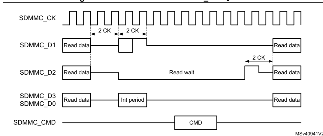
Figure 708. ReadWait with SDMMC_CLK < 50 MHz
