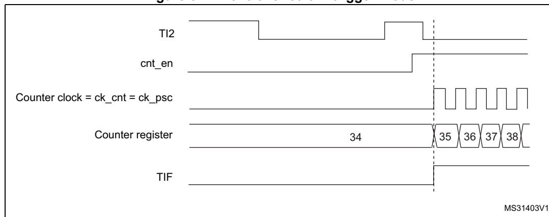
Figure 521. Control circuit in trigger mode
