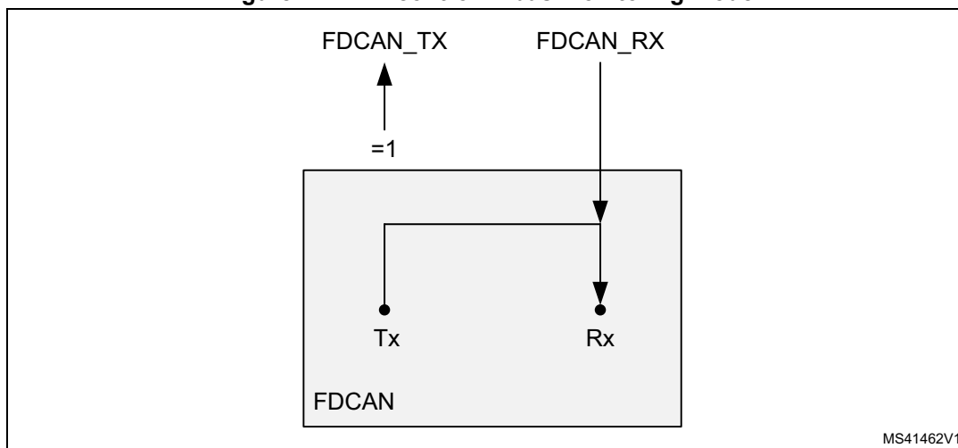
Figure 722. Pin control in bus monitoring mode
