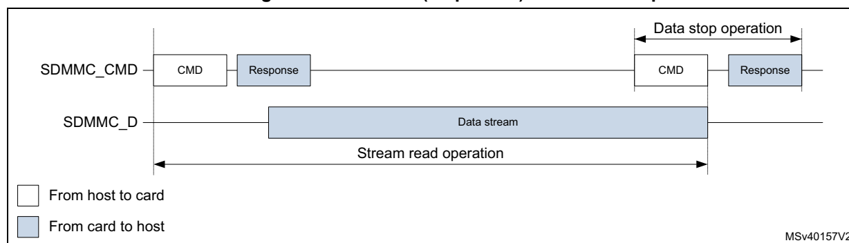
Figure 687. SDMMC (sequential) stream read operation
