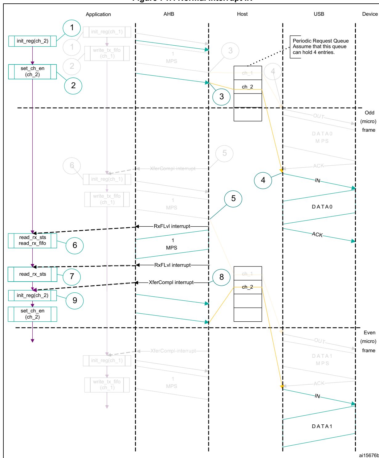
Figure 747. Normal interrupt IN
