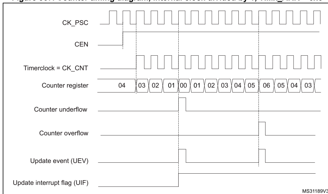
Figure 367. Counter timing diagram, internal clock divided by 1, TIMx_ARR = 0x6
