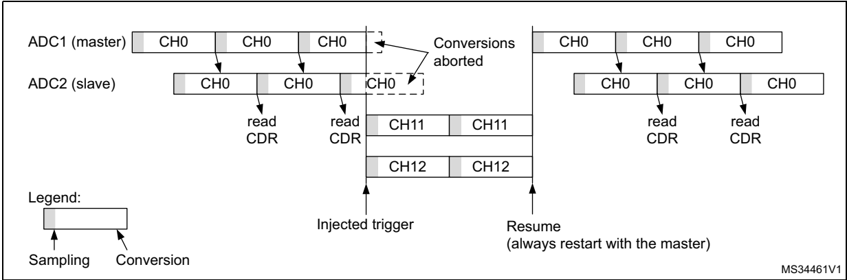
Figure 242. Interleaved single channel CH0 with injected sequence CH11, CH12
