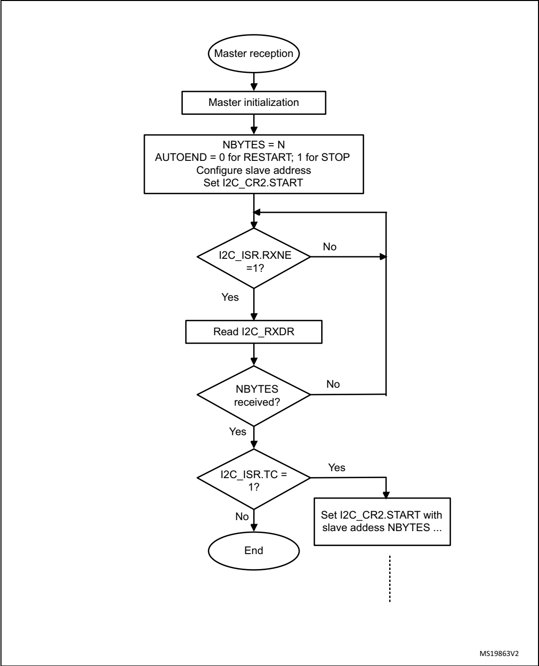
Figure 572. Transfer sequence flowchart for I2C master receiver for N \leq 255 bytes
