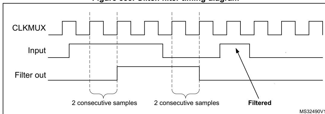
Figure 535. Glitch filter timing diagram
