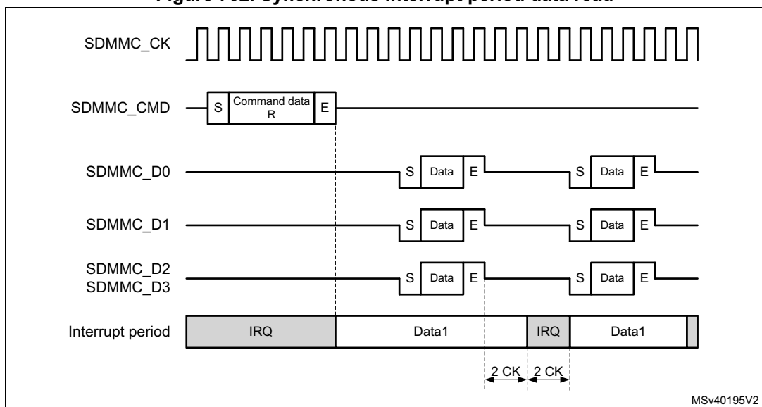
Figure 702. Synchronous interrupt period data read
