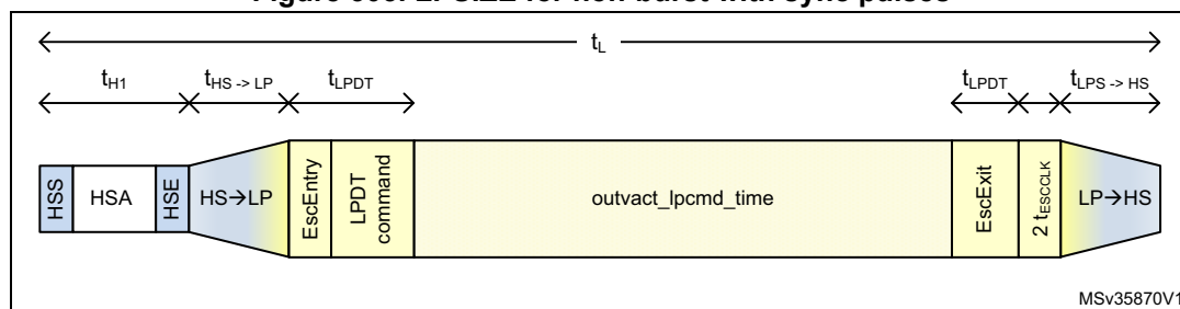
Figure 303. LPSIZE for non-burst with sync pulses
