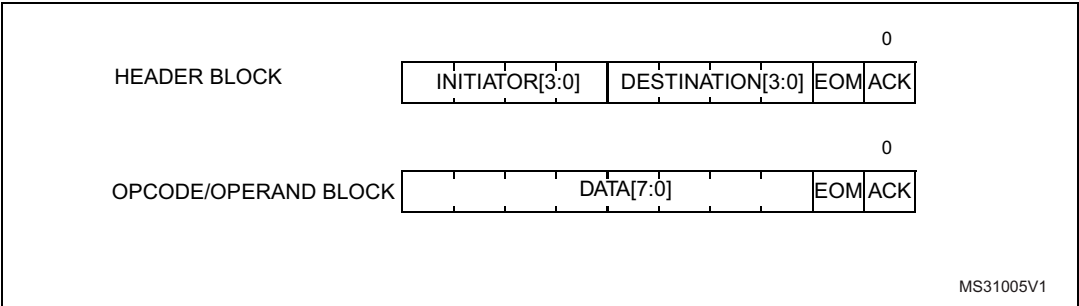
Figure 768. Blocks
