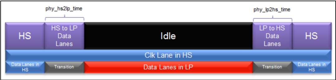
Figure 310. Clock lane in HS and data lanes in LP
