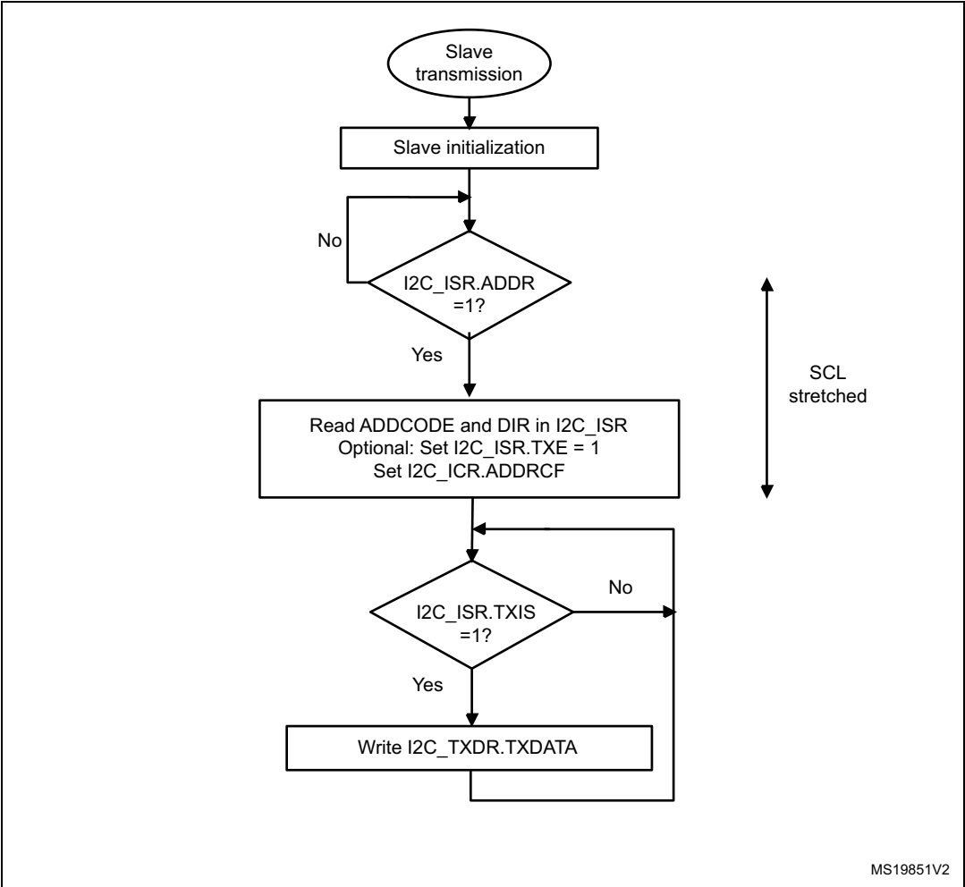
Figure 559. Transfer sequence flowchart for I2C slave transmitter, NOSTRETCH= 0
