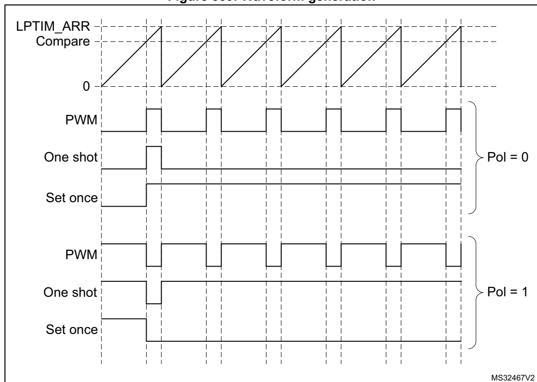
Figure 539. Waveform generation
