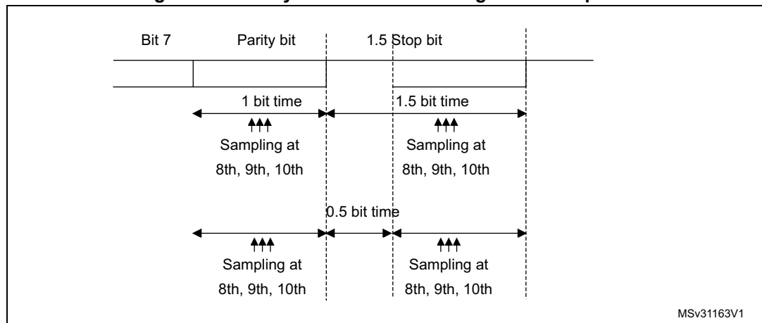
Figure 599. Parity error detection using the 1.5 stop bits
