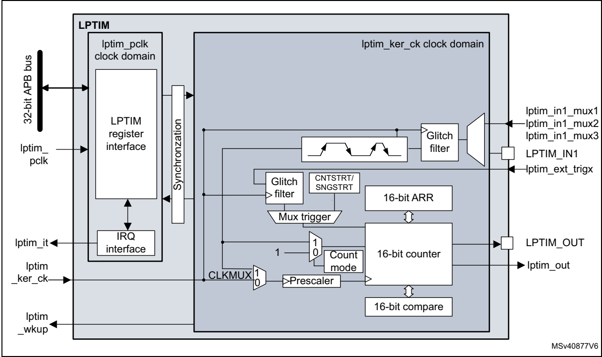
Figure 533. Low-power timer block diagram (LPTIM3)
