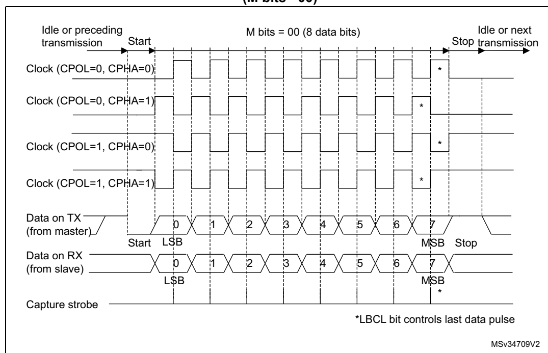
Figure 595. USART data clock timing diagram in synchronous master mode (M bits = 00)
