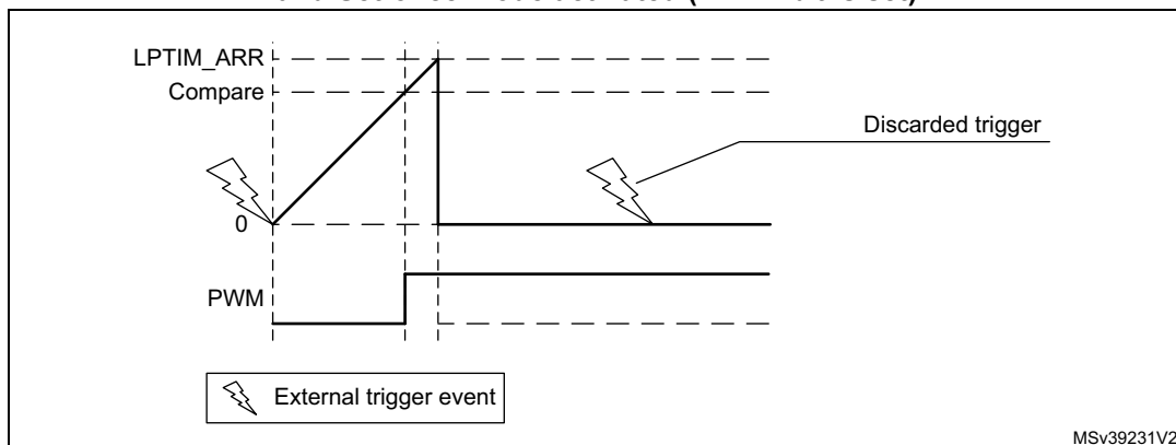
Figure 537. LPTIM output waveform, Single counting mode configuration and Set-once mode activated (WAVE bit is set)
