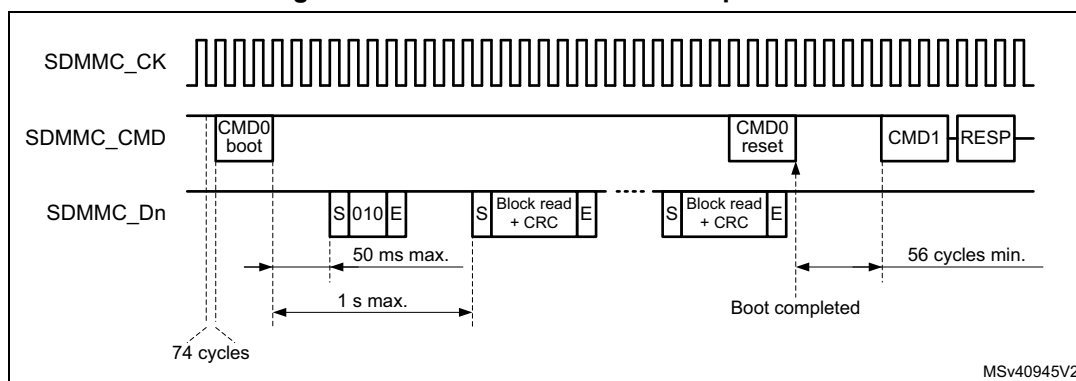
Figure 713. Alternative boot mode operation
