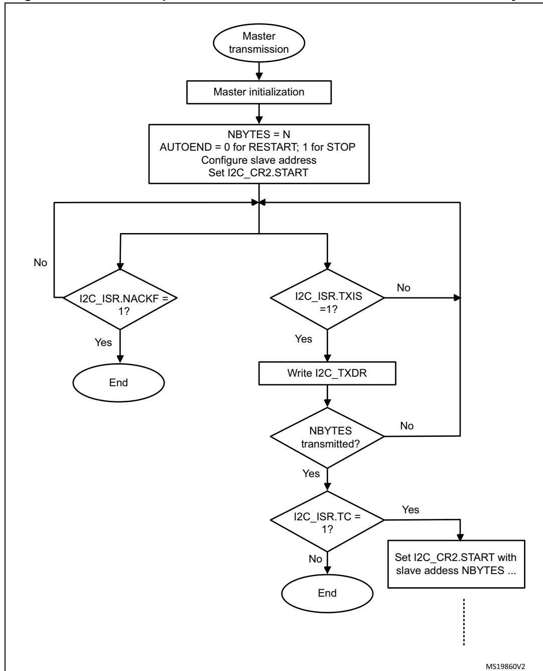
Figure 569. Transfer sequence flowchart for I2C master transmitter for N \leq 255 bytes
