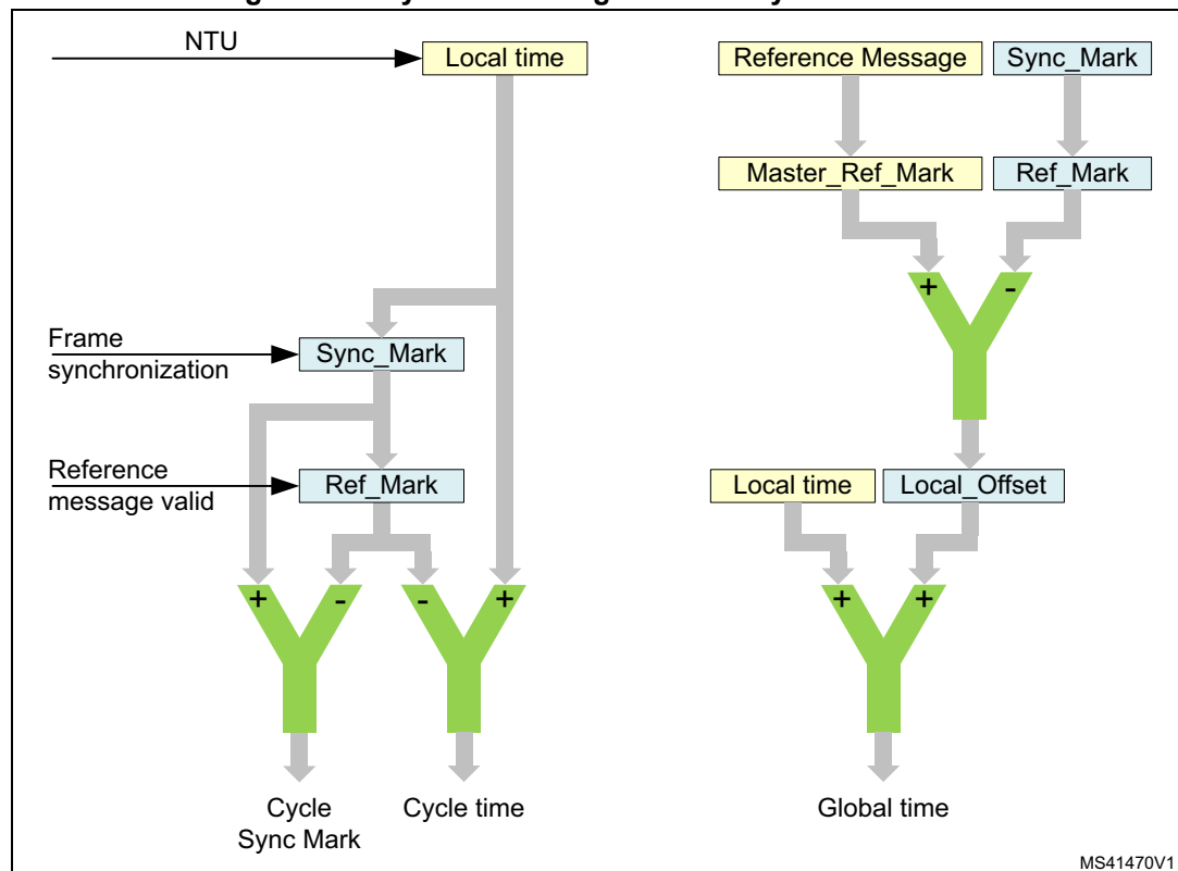
Figure 732. Cycle time and global time synchronization
