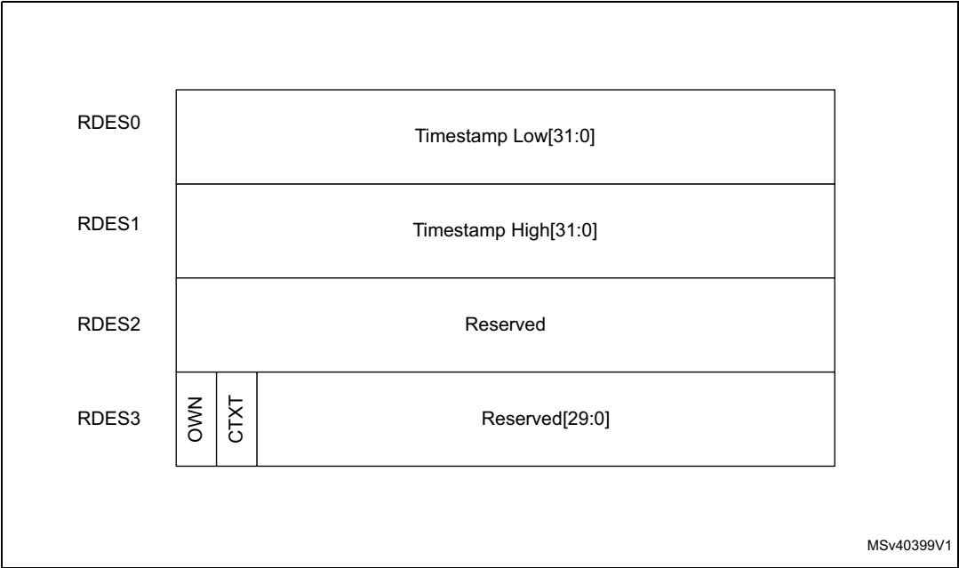
Figure 805. Receive context descriptor
