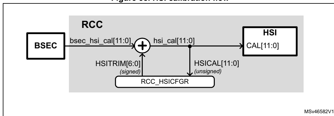
Figure 58. HSI calibration flow
