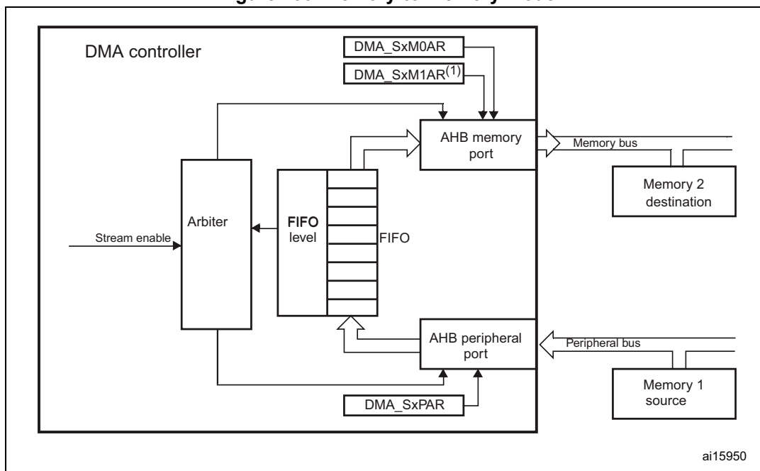
Figure 133. Memory-to-memory mode
