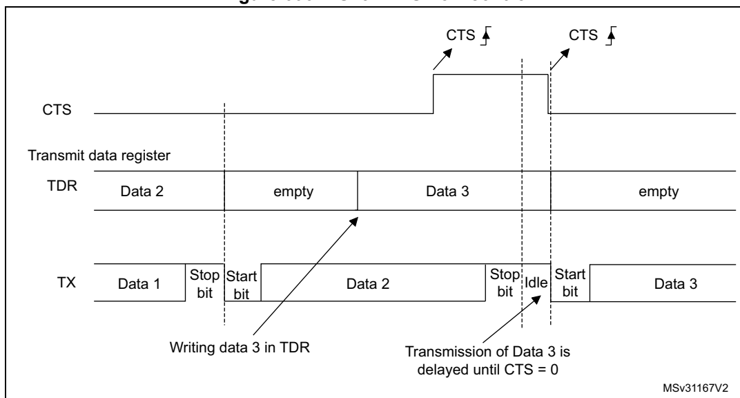
Figure 606. RS232 CTS flow control
