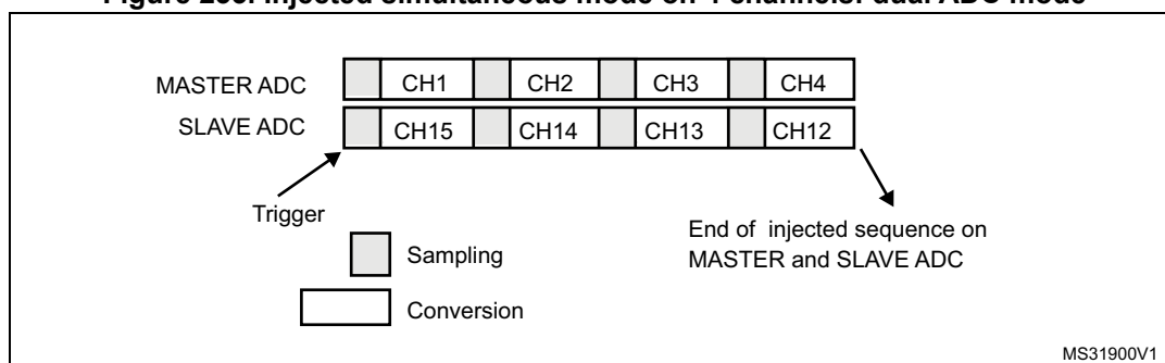
Figure 233. Injected simultaneous mode on 4 channels: dual ADC mode
