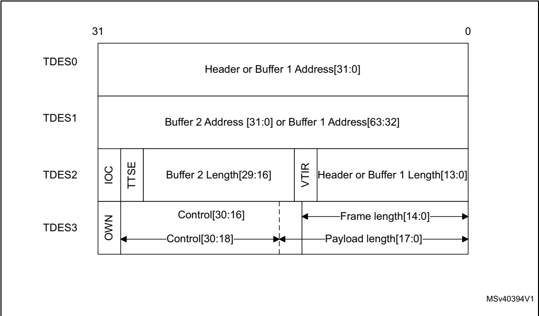
Figure 800. Transmit descriptor (read format)
