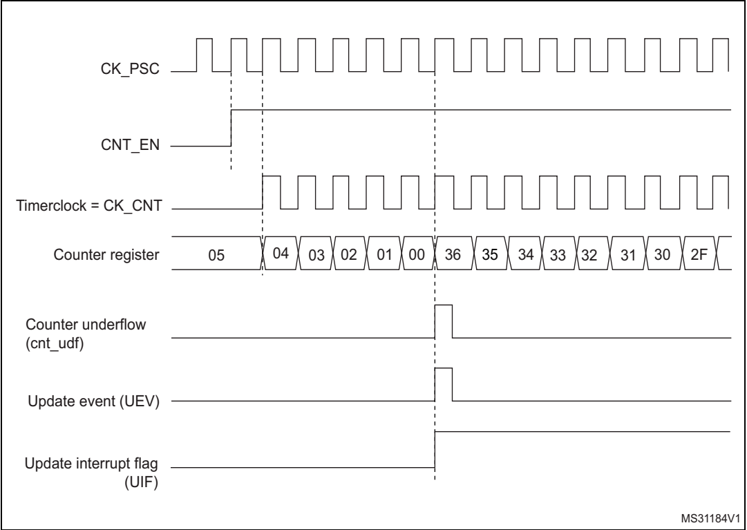
Figure 362. Counter timing diagram, internal clock divided by 1
