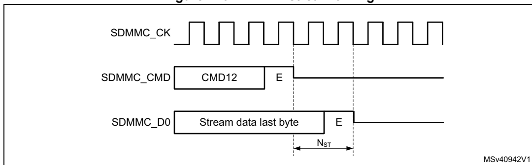
Figure 710. CMD12 stream timing
