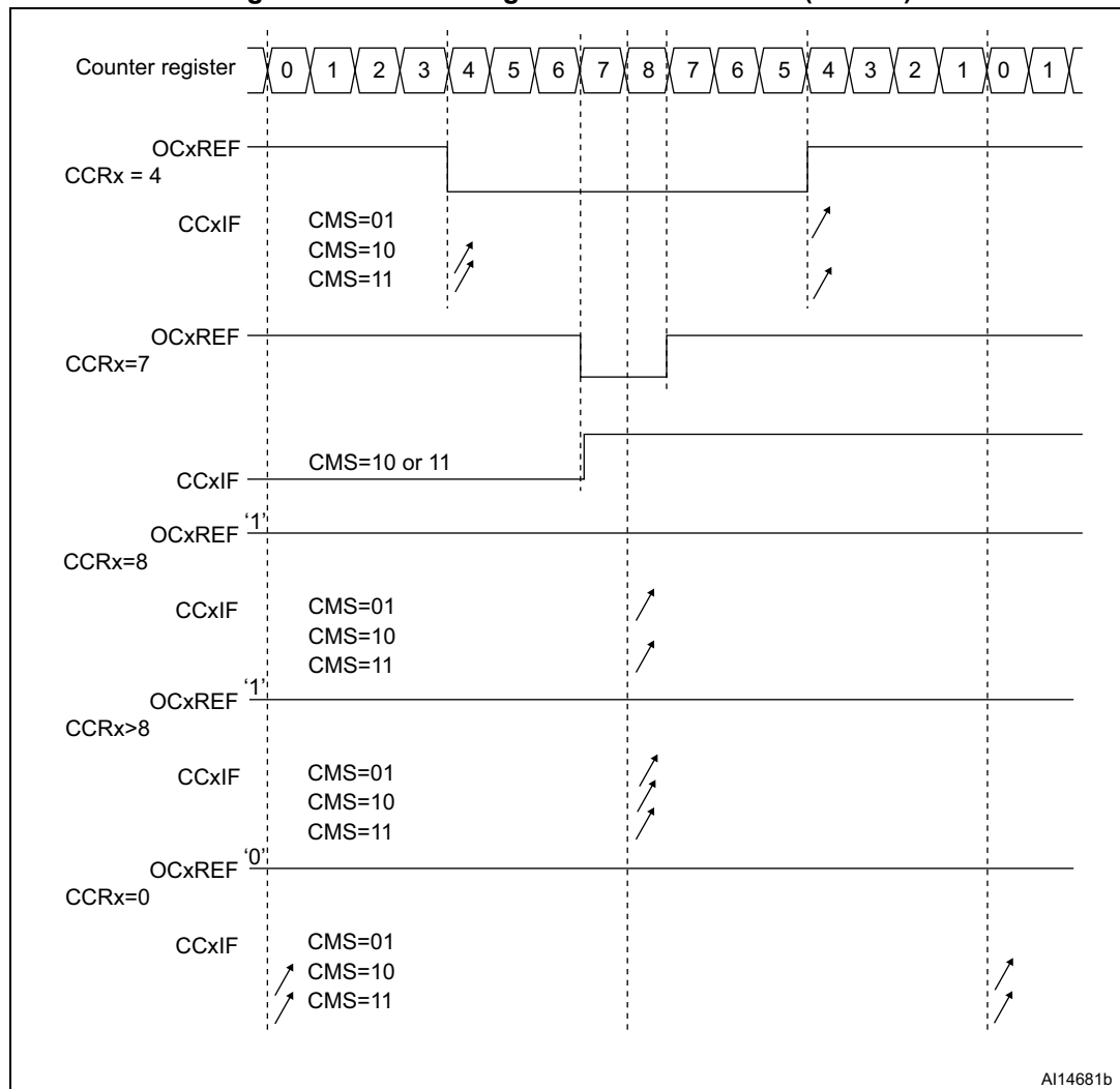
Figure 444. Center-aligned PWM waveforms (ARR=8)
