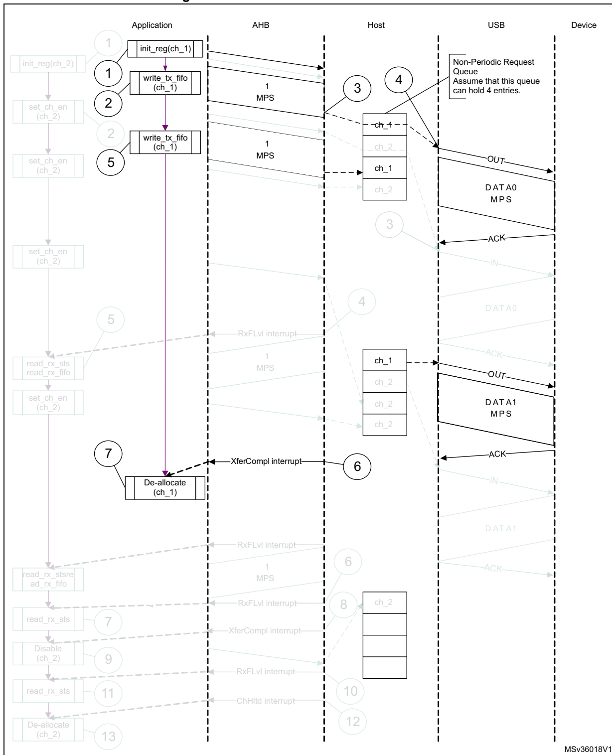
Figure 744. Normal bulk/control OUT/SETUP
