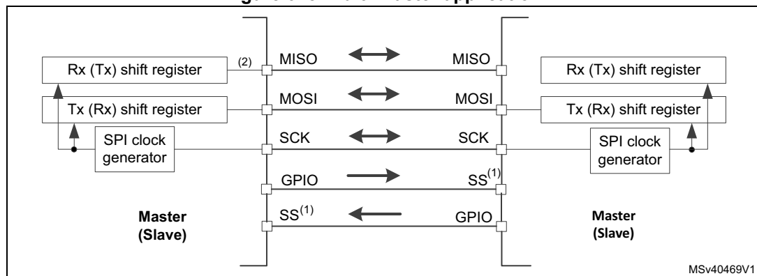
Figure 615. Multi-master application
