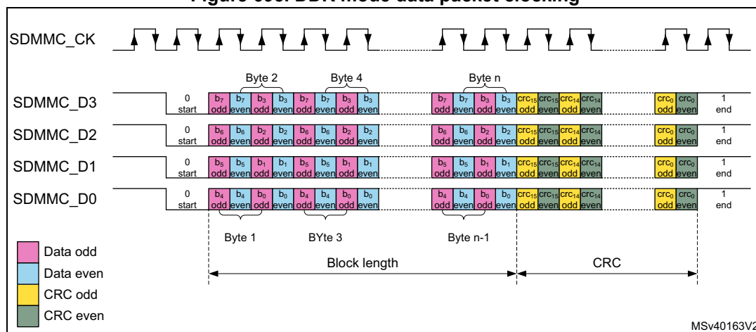
Figure 695. DDR mode data packet clocking
