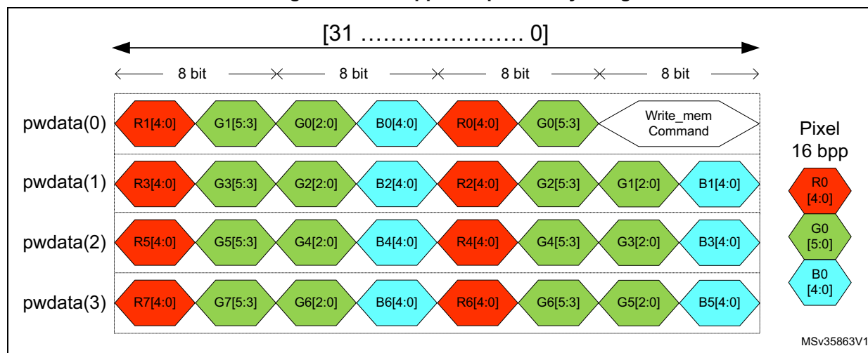
Figure 294. 16 bpp APB pixel to byte organization
