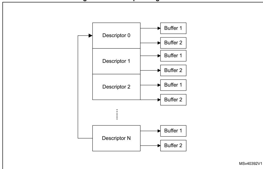
Figure 798. Descriptor ring structure
