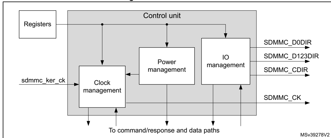
Figure 691. Control unit
