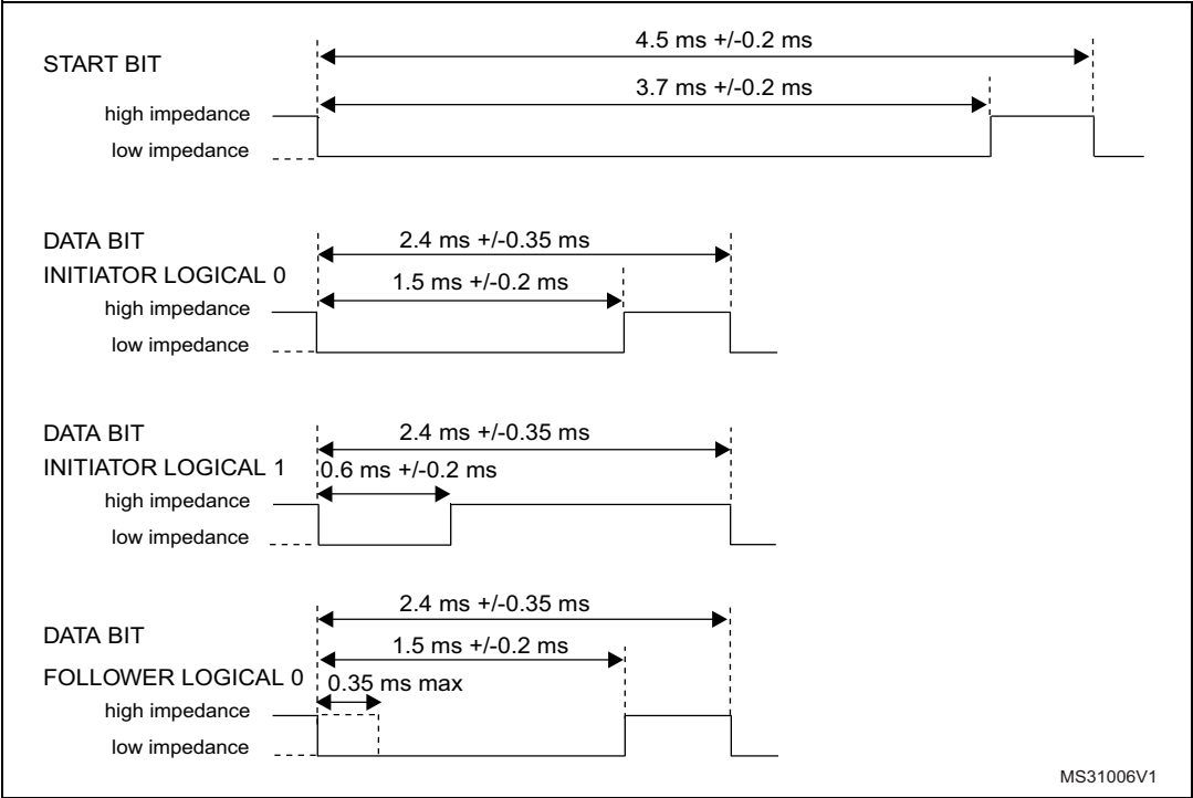
Figure 769. Bit timings
