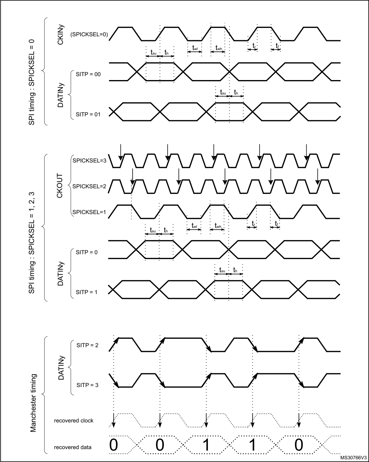
Figure 267. Channel transceiver timing diagrams
