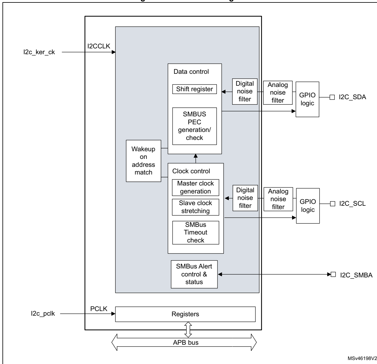
Figure 552. I2C block diagram
