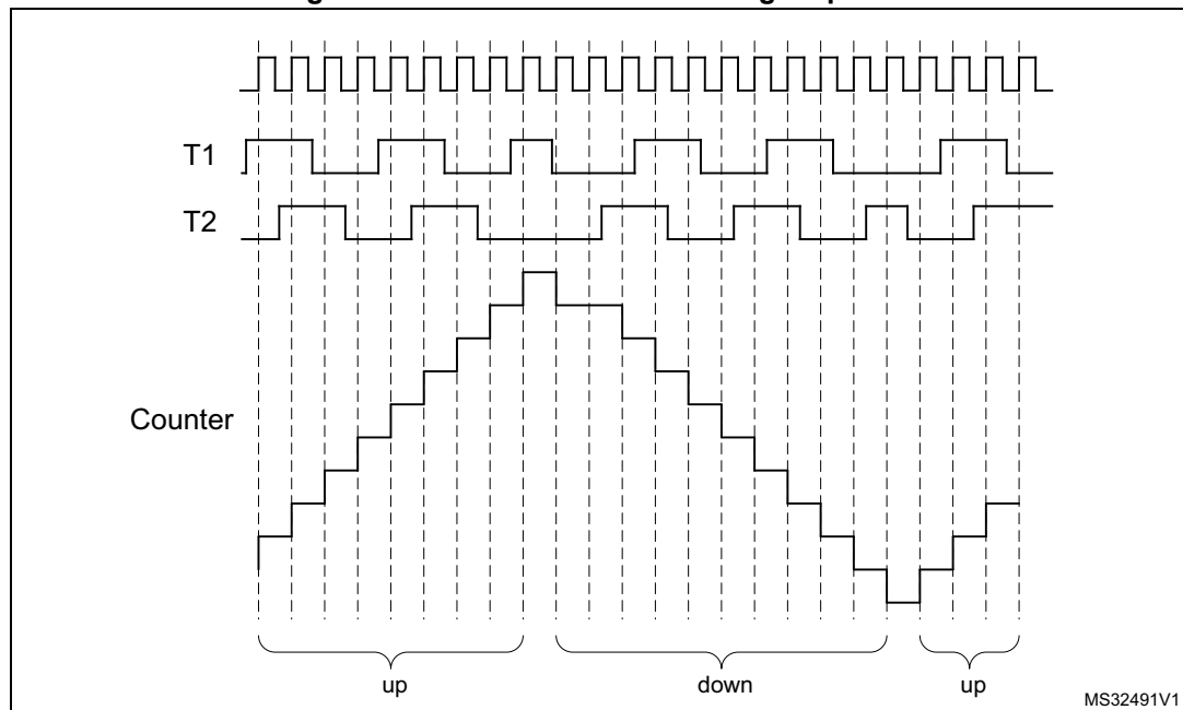
Figure 540. Encoder mode counting sequence
