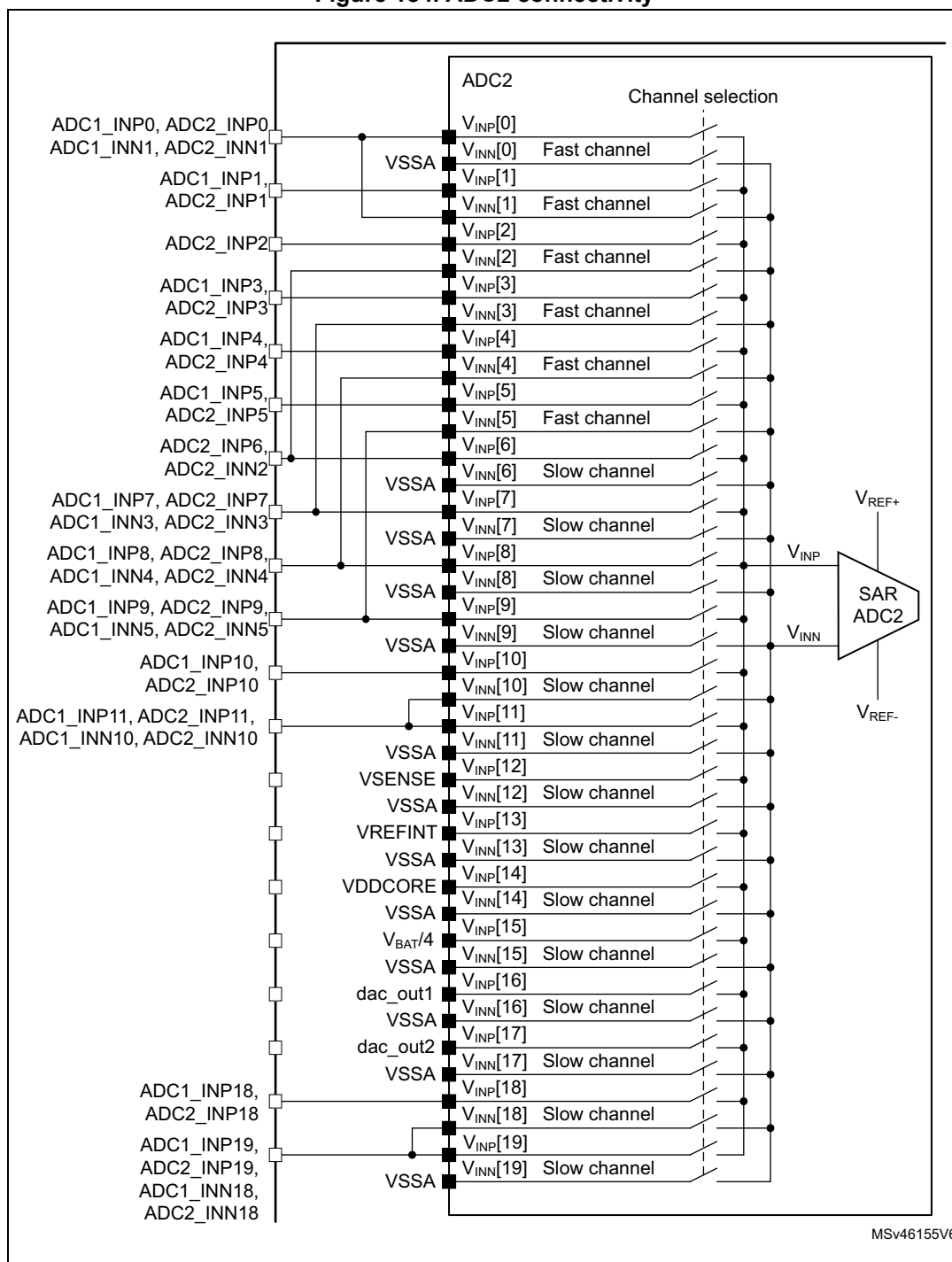
Figure 184. ADC2 connectivity
