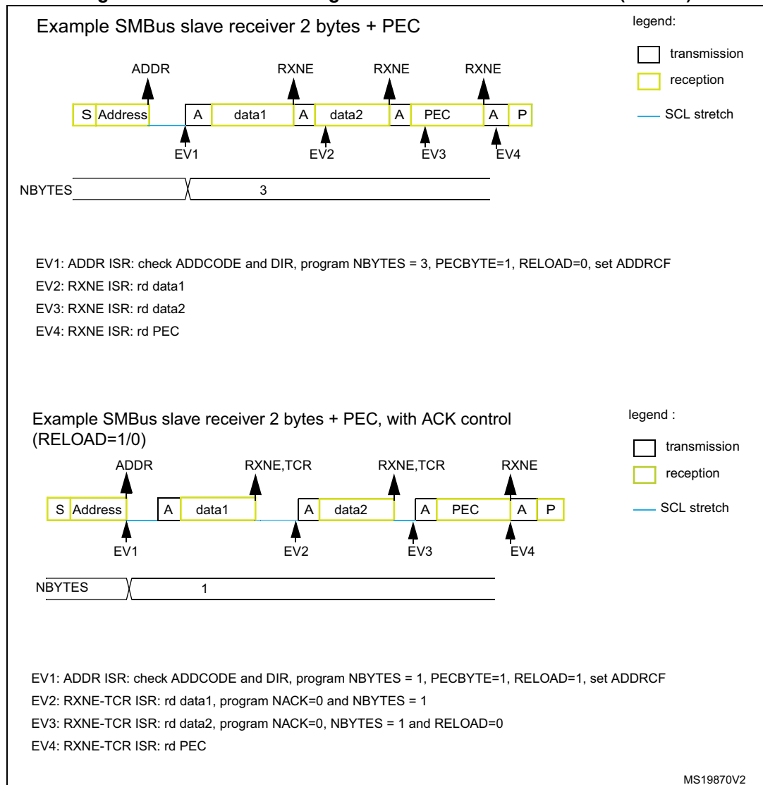
Figure 579. Bus transfer diagrams for SMBus slave receiver (SBC=1)
