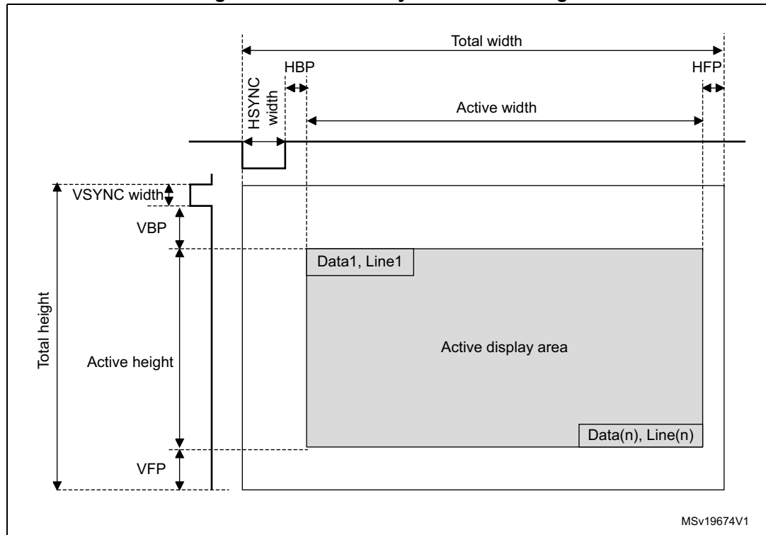
Figure 282. LCD-TFT synchronous timings
