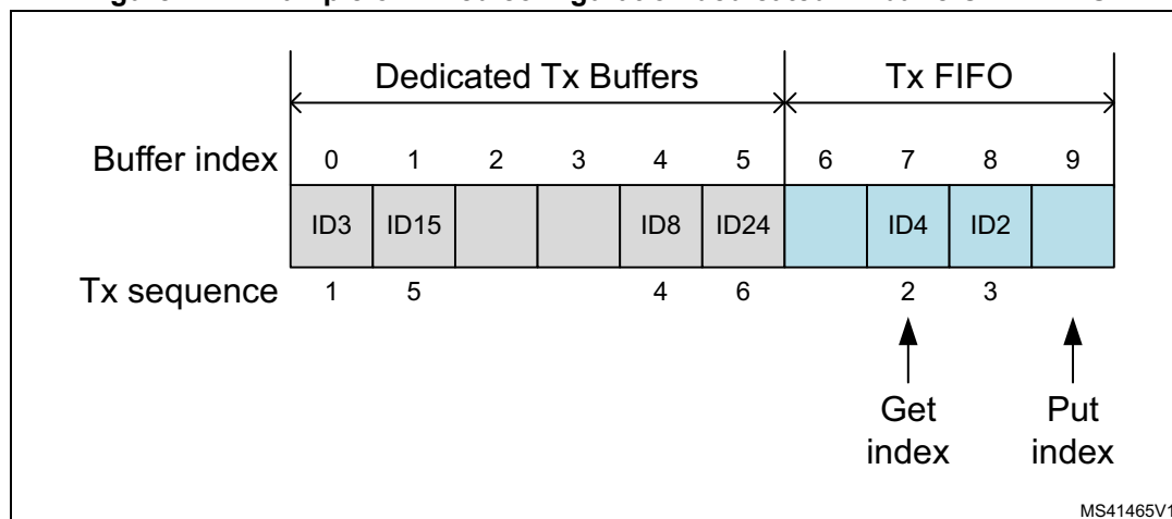
Figure 727. Example of mixed configuration dedicated Tx buffers / Tx FIFO
