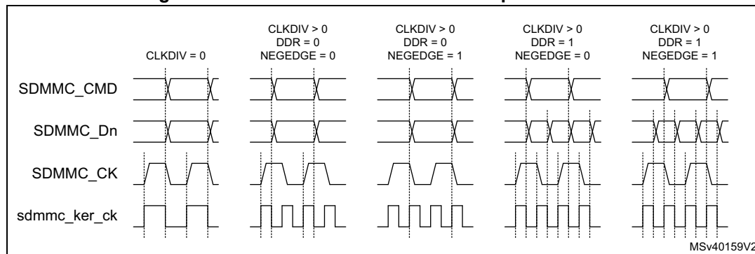
Figure 690. SDMMC Command and data phase relation
