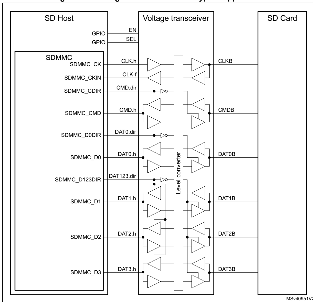
Figure 718. Voltage switch transceiver typical application
