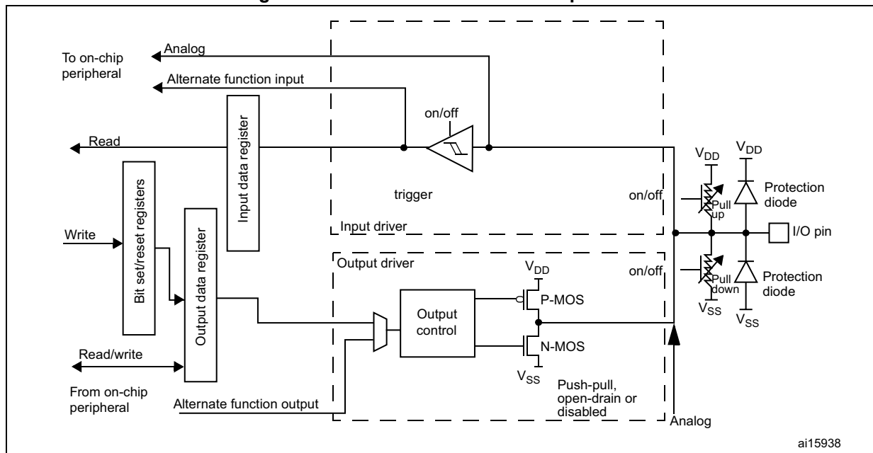
Figure 119. Basic structure of an I/O port bitt
