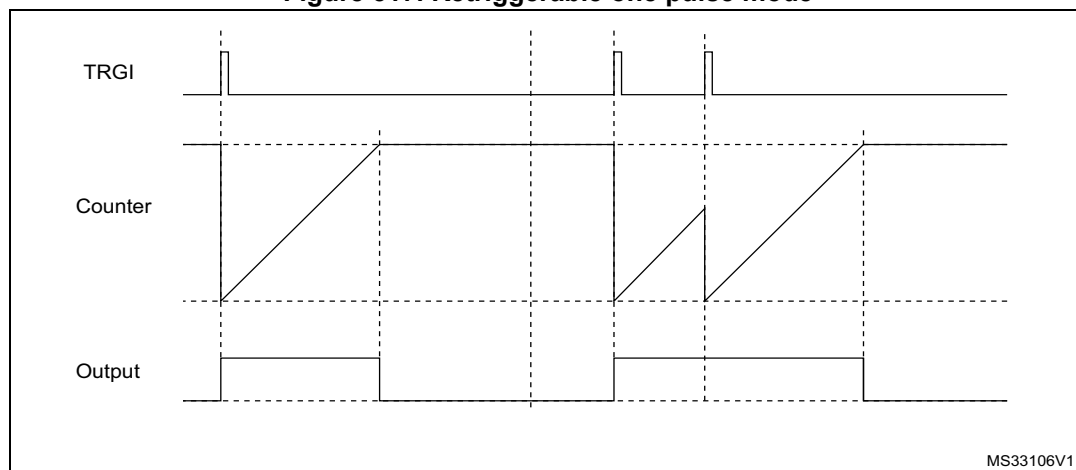
Figure 517. Retriggerable one pulse mode
