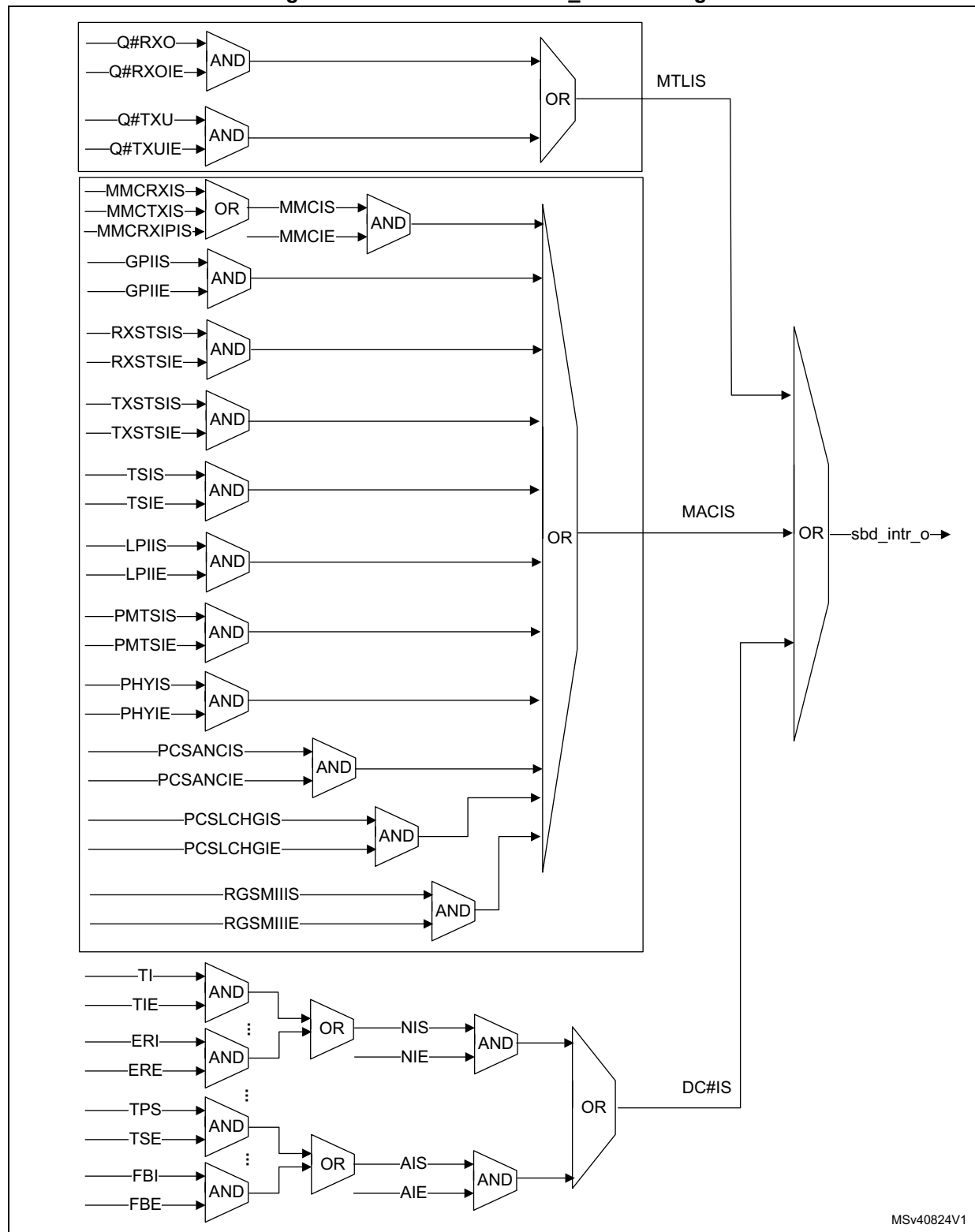
Figure 806. Generation of ETH_DMAISR flags
