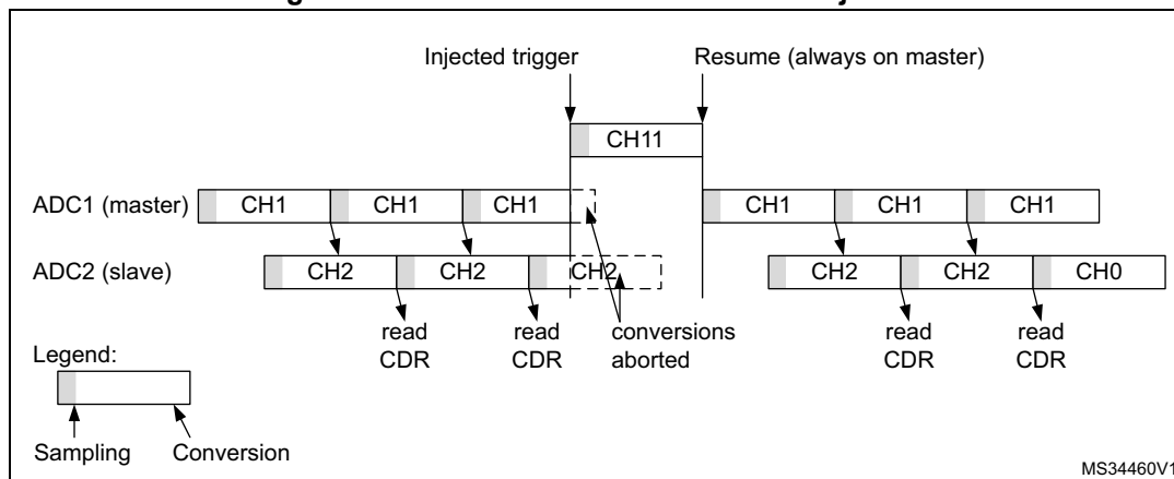
Figure 237. Interleaved conversion with injection
