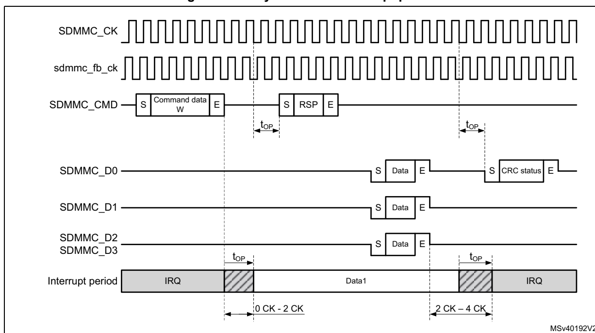
Figure 705. Asynchronous interrupt period data write
