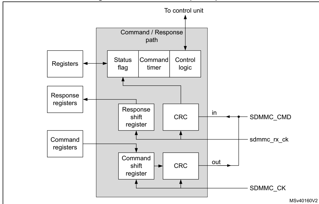
Figure 692. Command/Response path
