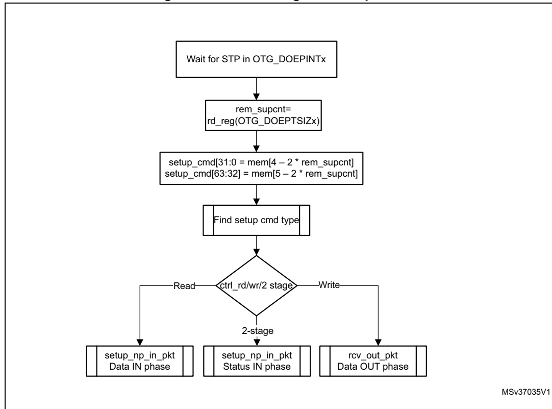
Figure 757. Processing a SETUP packet
