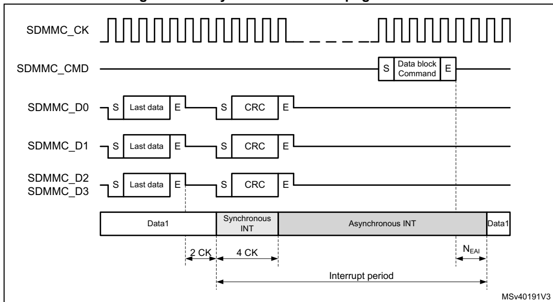
Figure 701. Asynchronous interrupt generation
