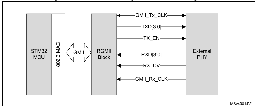
Figure 797. RGMII block diagram and interface signals
