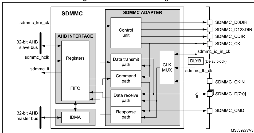
Figure 689. SDMMC block diagram
