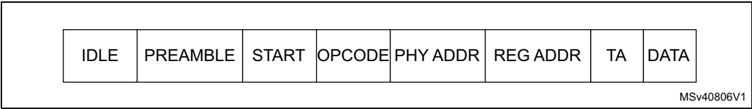
Figure 790. MDIO packet structure
