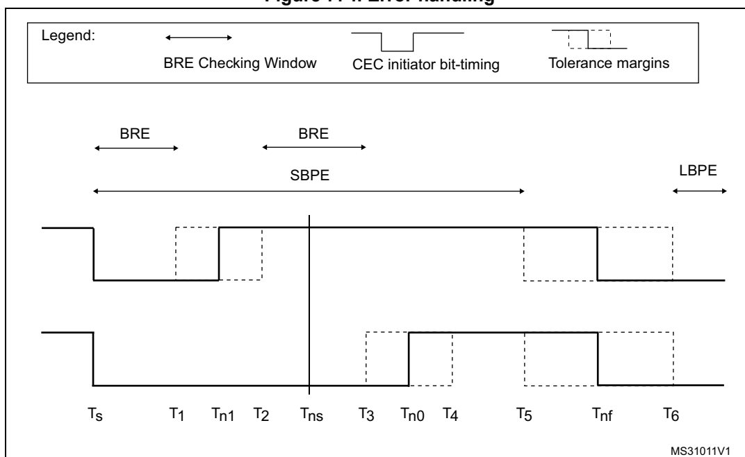
Figure 774. Error handling
