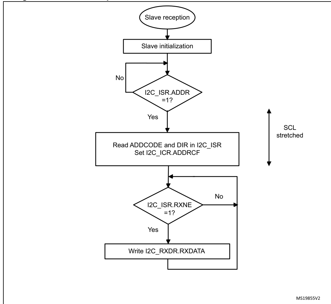
Figure 562. Transfer sequence flowchart for slave receiver with NOSTRETCH=0
