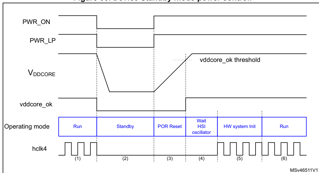
Figure 33. Device Standby mode power control.
