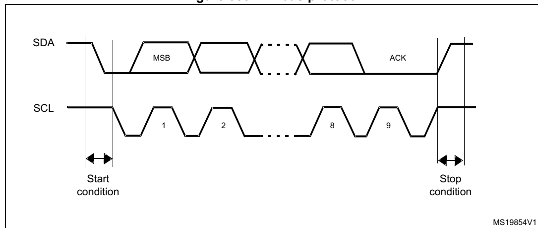
Figure 553. I 2 C bus protocol
