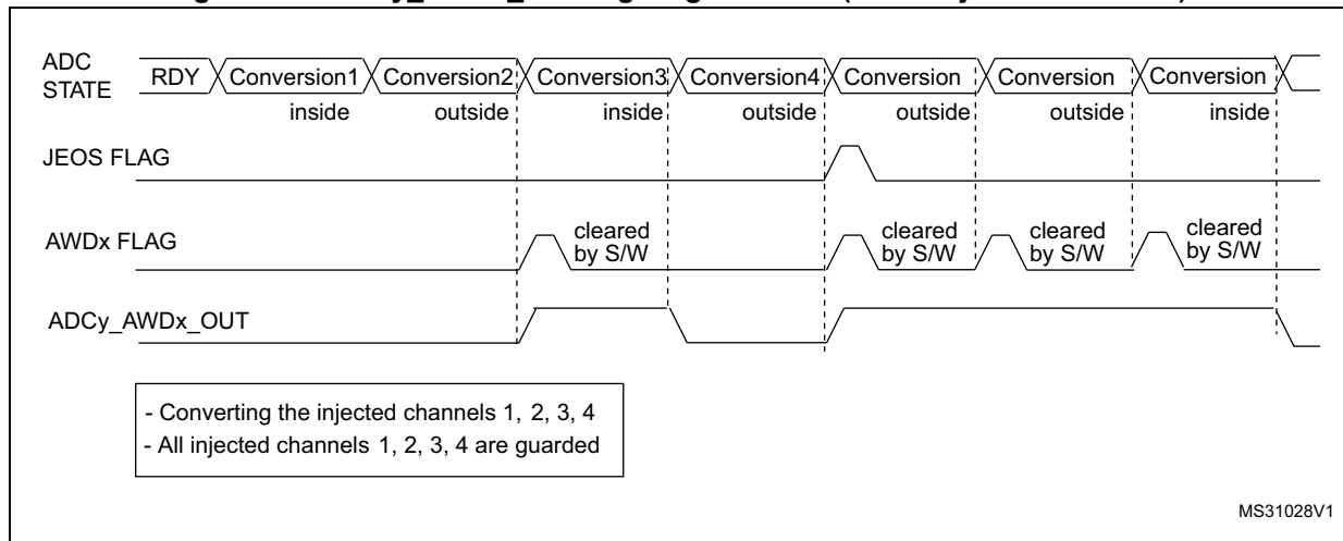
Figure 225. ADCy_AWDx_OUT signal generation (on all injected channels)
