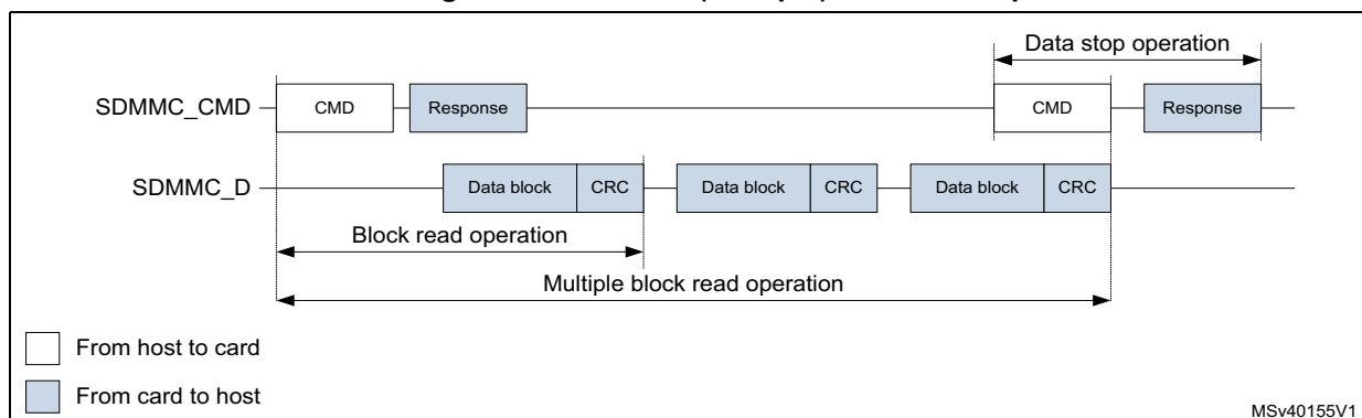
Figure 685. SDMMC (multiple) block read operation
