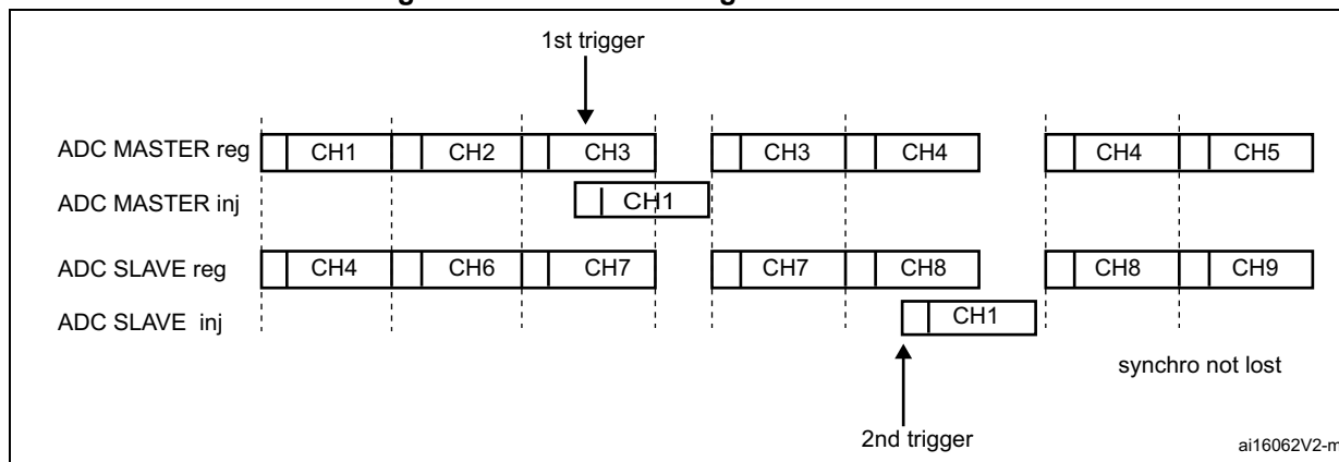
Figure 240. Alternate + regular simultaneous
