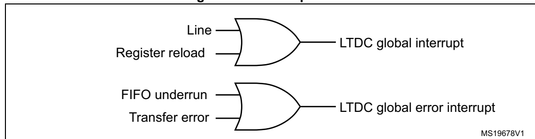
Figure 285. Interrupt events
