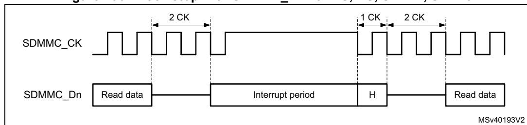
Figure 706. Clock stop with SDMMC_CK for DS, HS, SDR12, SDR25
