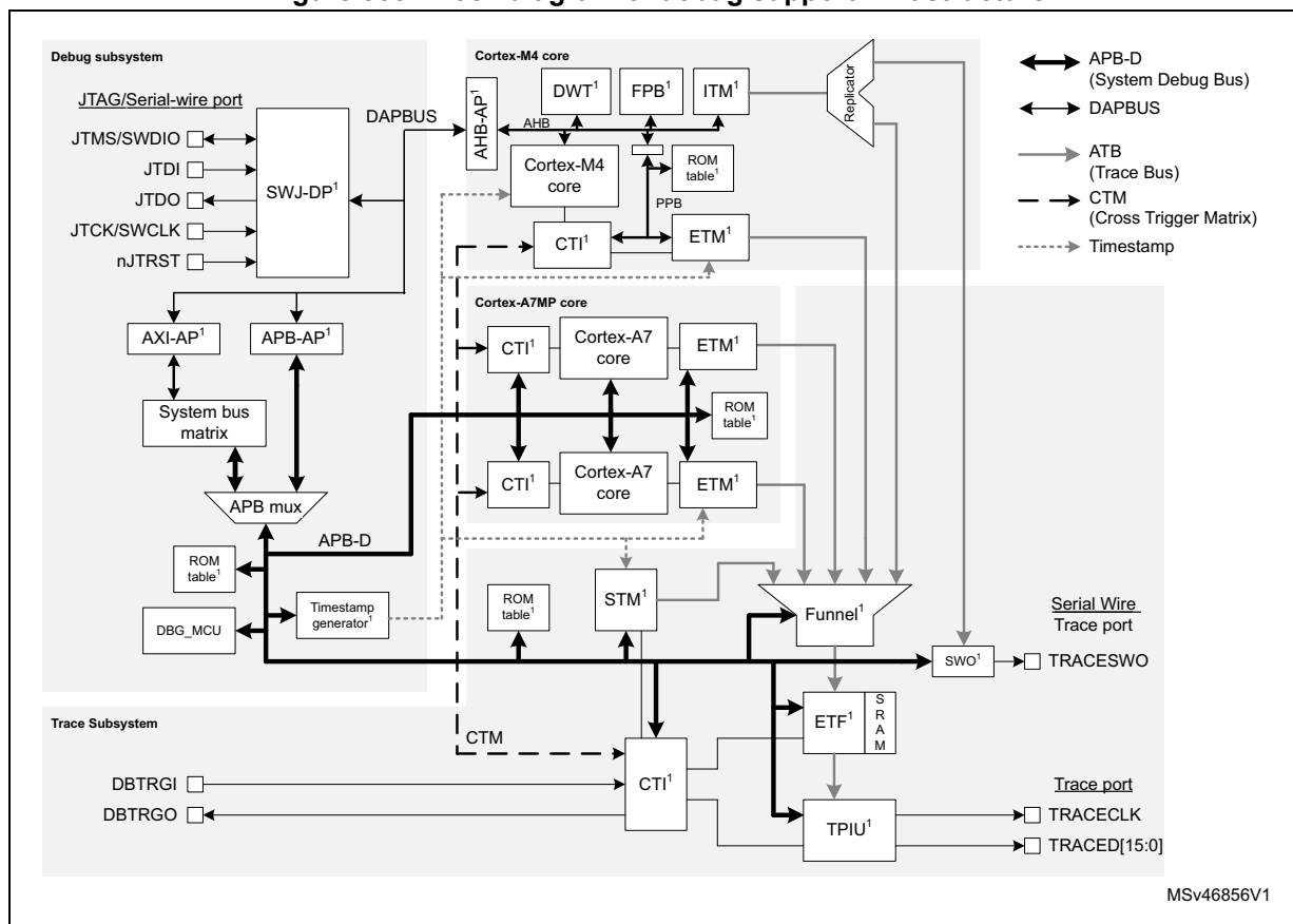
Figure 808. Block diagram of debug support infrastructure
