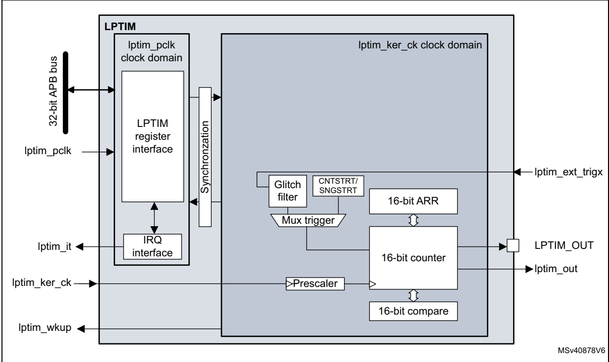
Figure 534. Low-power timer block diagram (LPTIM4 and LPTIM5)
