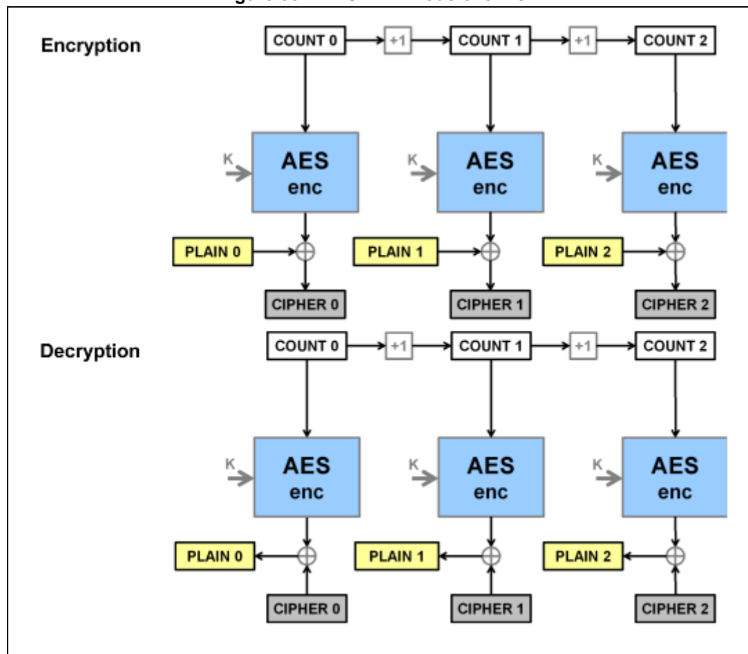
Figure 332. AES-CTR mode overview
