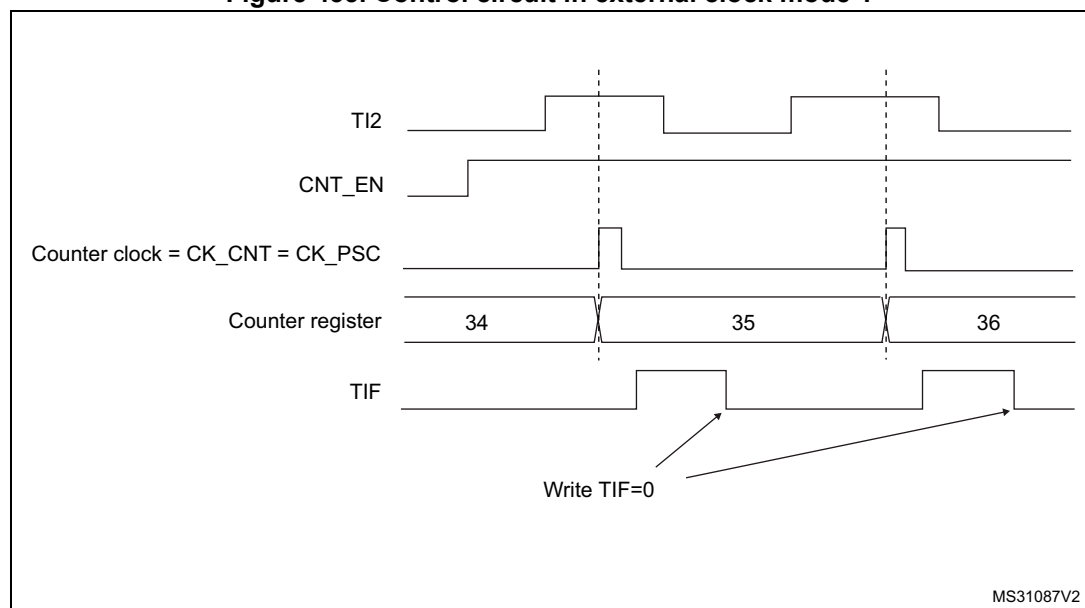
Figure 435. Control circuit in external clock mode 1
