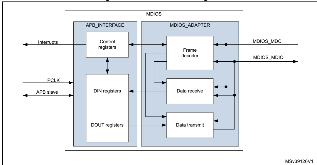
Figure 681. MDIOS block diagram
