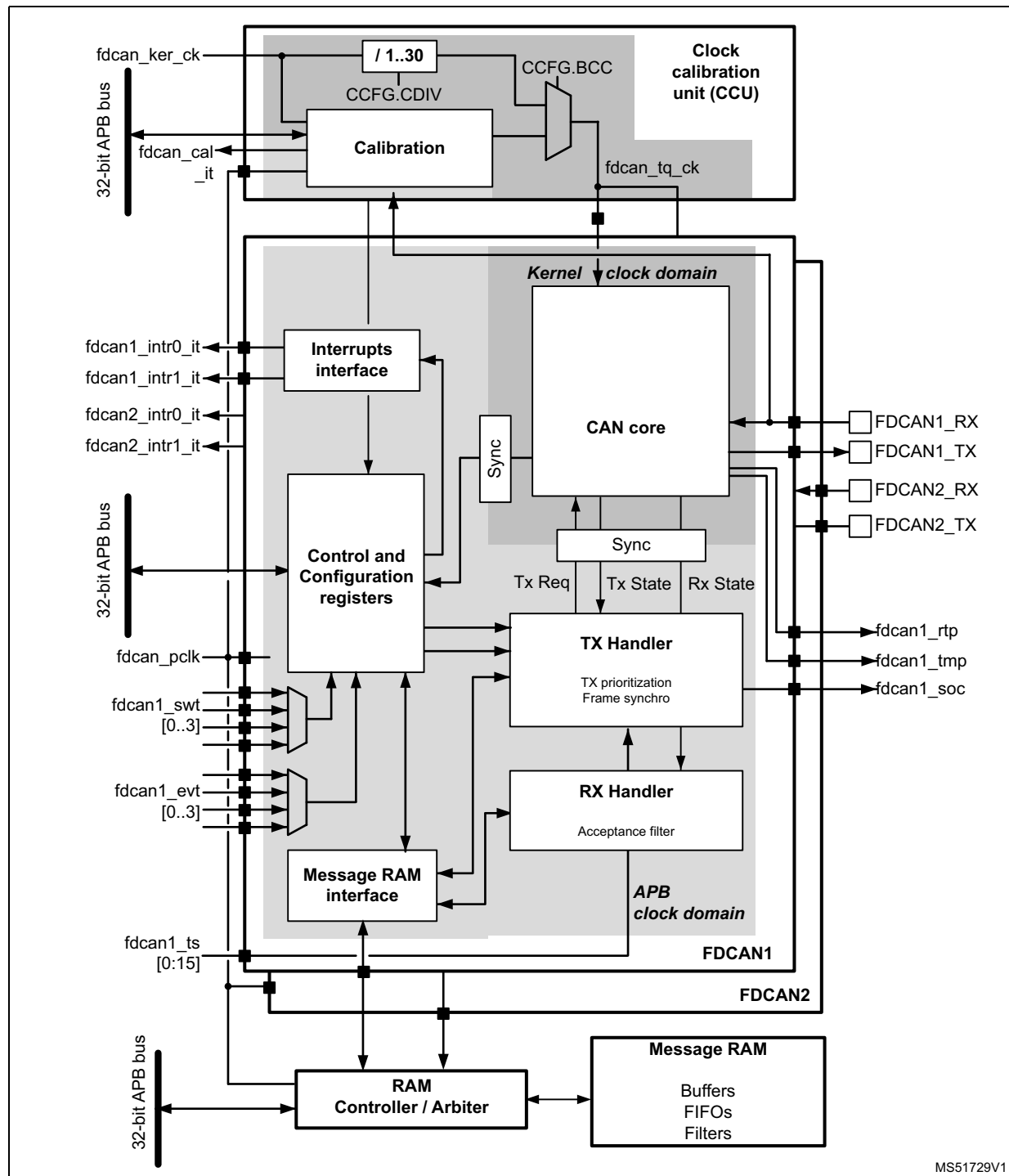
Figure 719. CAN subsystem
