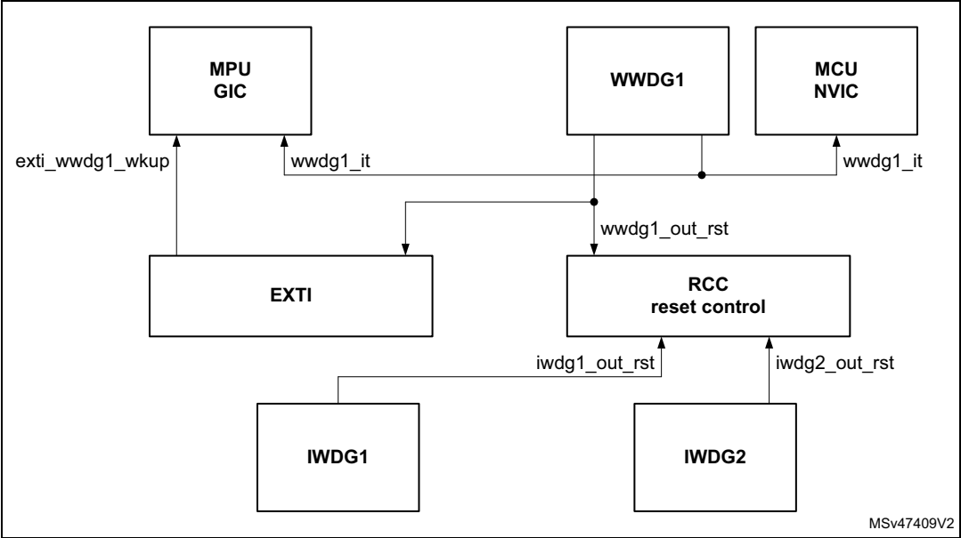
Figure 542. Watchdogs top view
