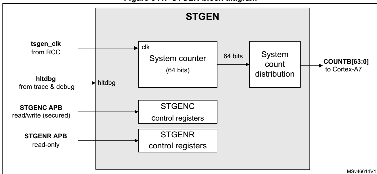
Figure 541. STGEN block diagram
