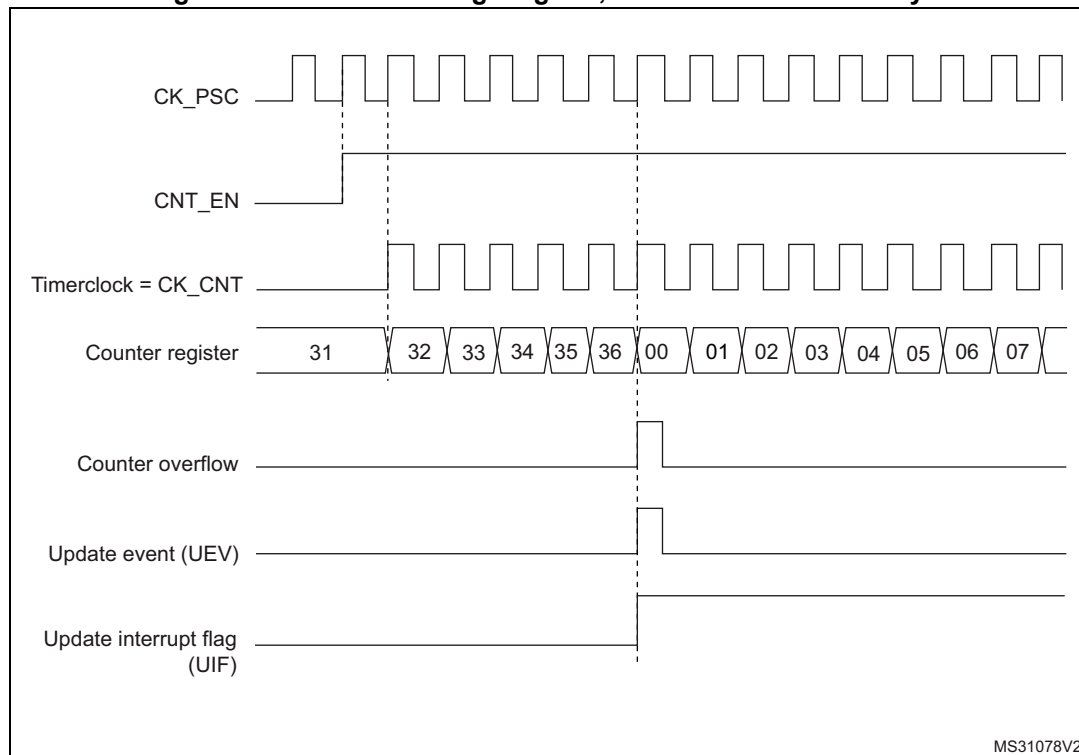
Figure 525. Counter timing diagram, internal clock divided by 1
