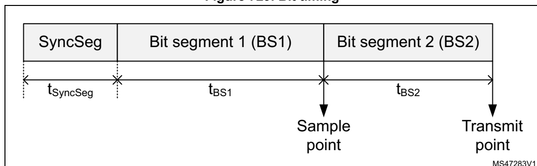
Figure 729. Bit timing
