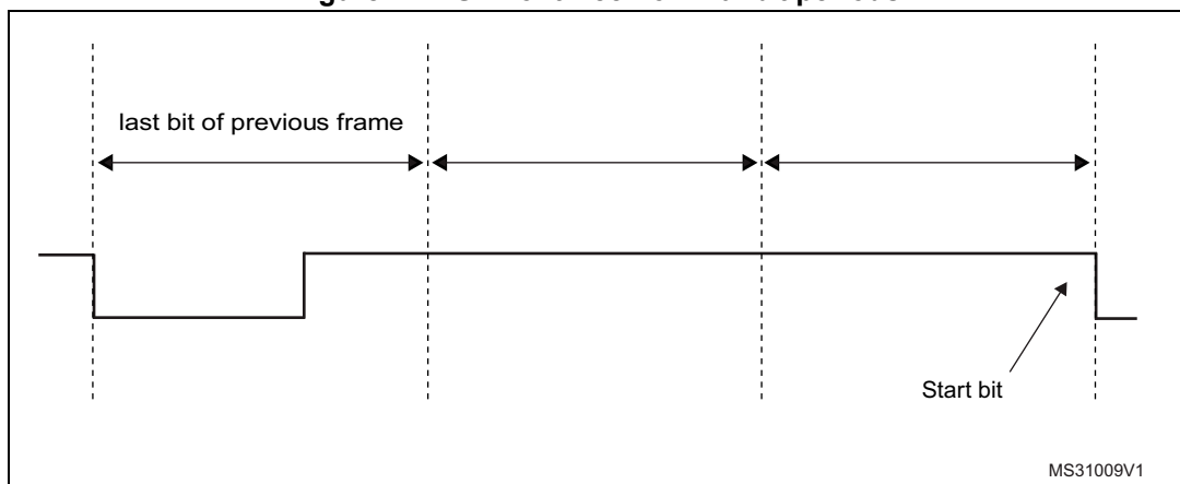
Figure 772. SFT of three nominal bit periods
