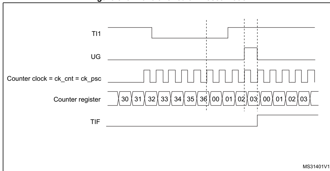
Figure 519. Control circuit in reset mode
