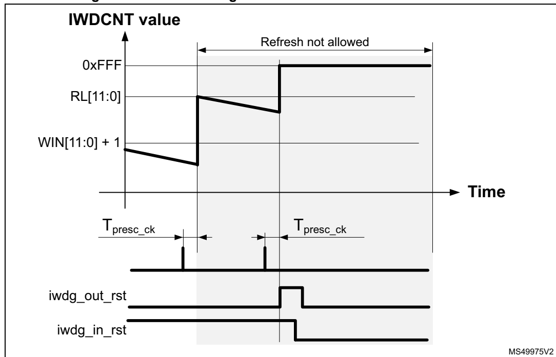
Figure 545. Reset timing due to refresh in the not allowed area
