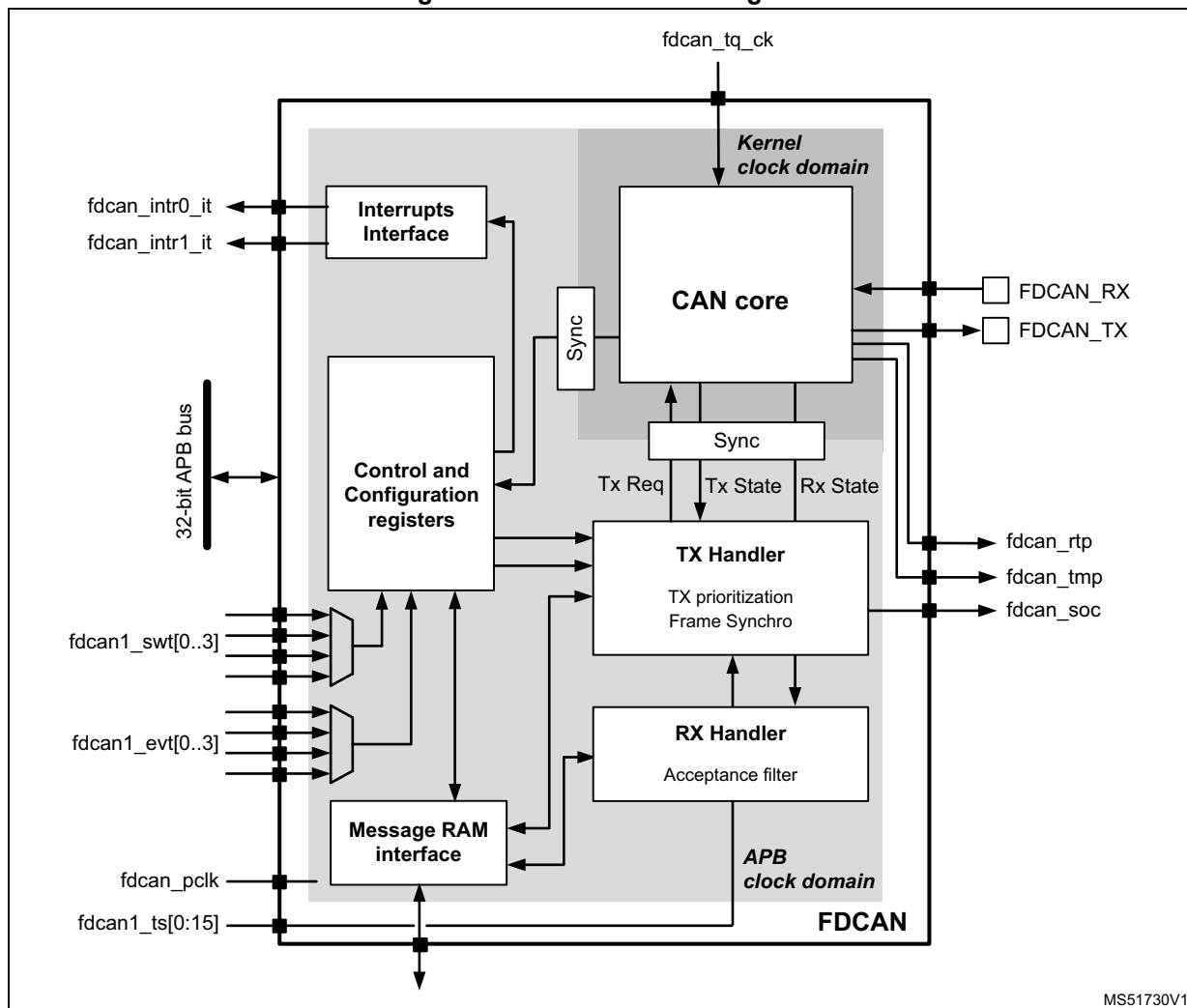
Figure 720. FDCAN block diagram
