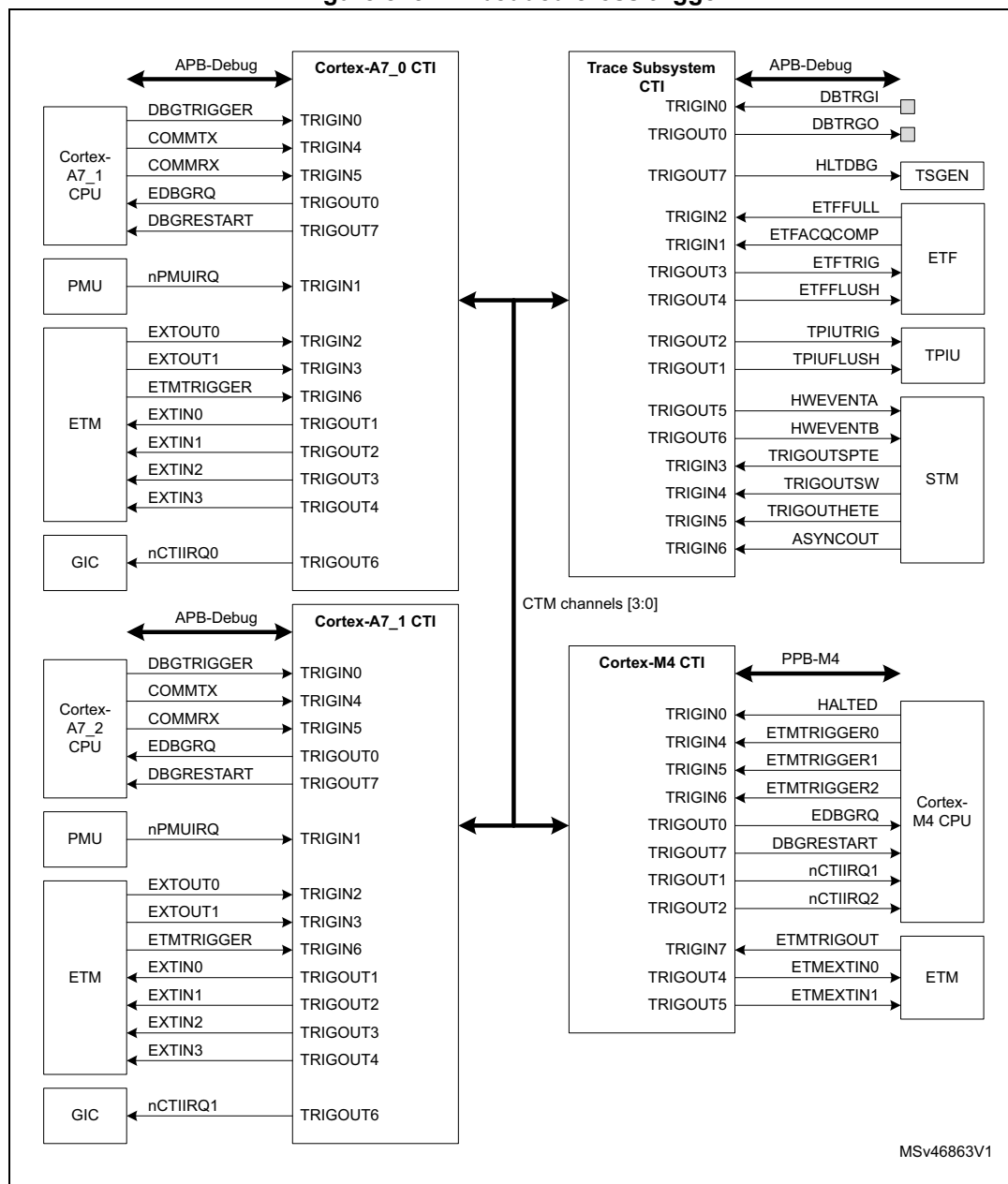
Figure 815. Embedded cross trigger
