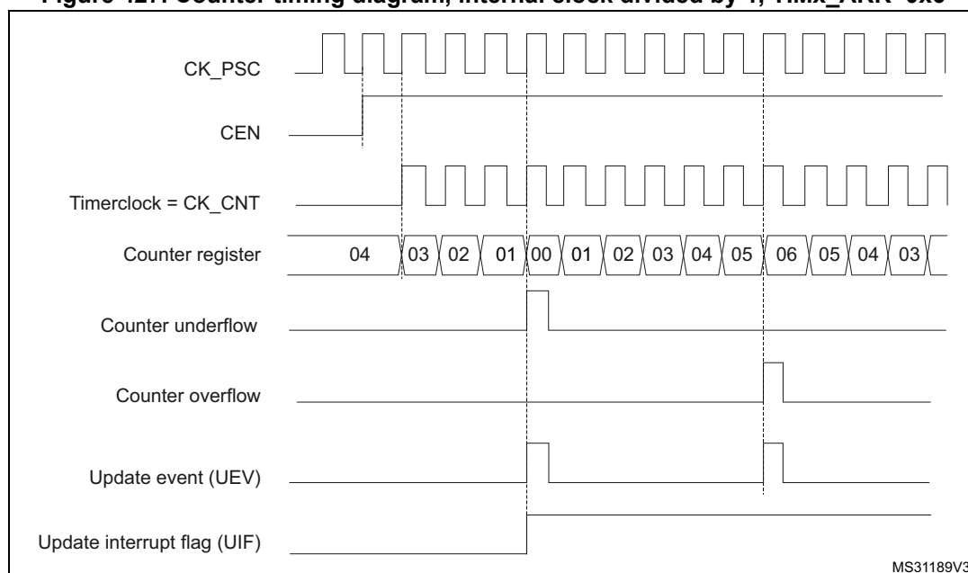
Figure 427. Counter timing diagram, internal clock divided by 1, TIMx_ARR=0x6
