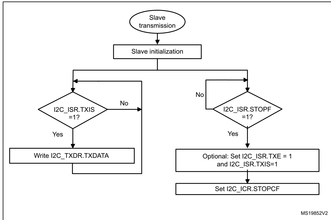
Figure 560. Transfer sequence flowchart for I2C slave transmitter, NOSTRETCH= 1
