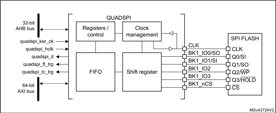
Figure 172. QUADSPI block diagram
