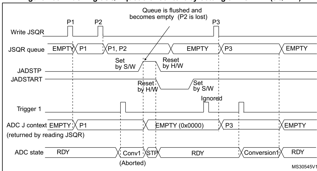
Figure 203. Flushing JSQR queue of context by setting JADSTP=1 (JQM=1)
