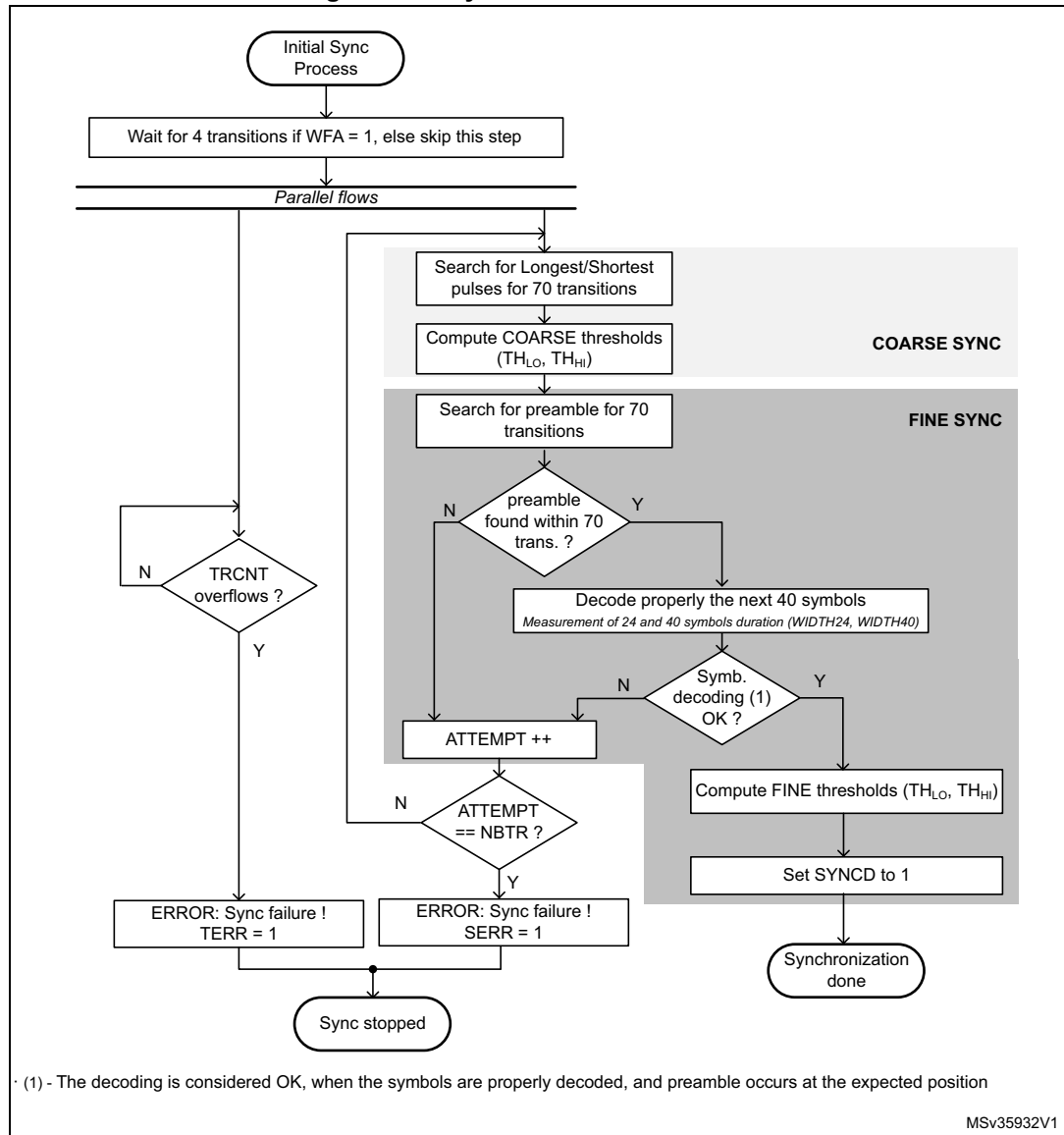
Figure 673. Synchronization flowchart
