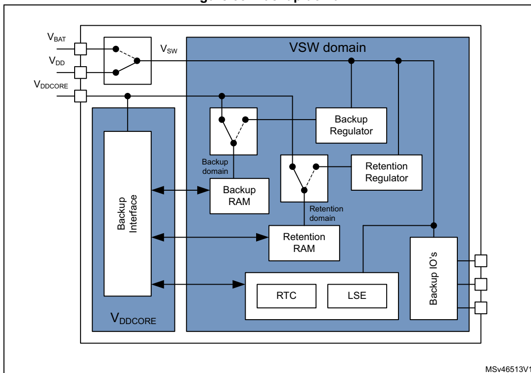
Figure 35. Backup domain
