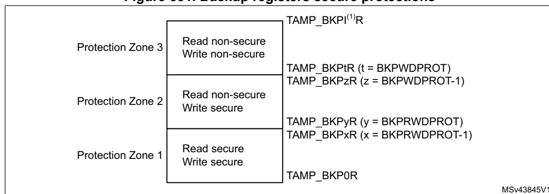
Figure 551. Backup registers secure protections
