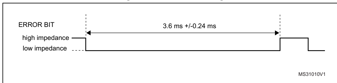
Figure 773. Error bit timing
