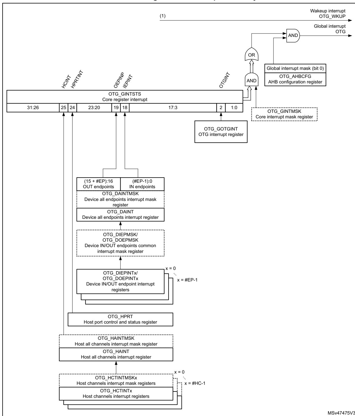
Figure 741. Interrupt hierarchy
