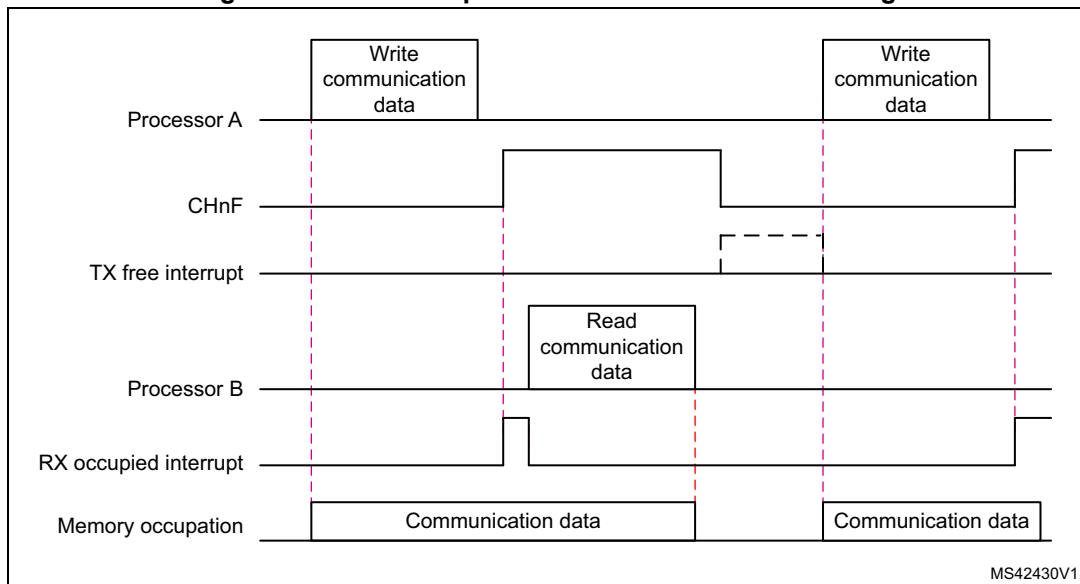
Figure 113. IPCC Simplex channel mode transfer timing
