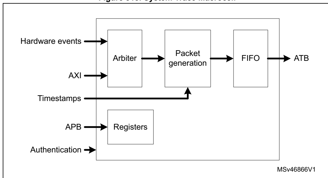
Figure 818. System Trace Macrocell
