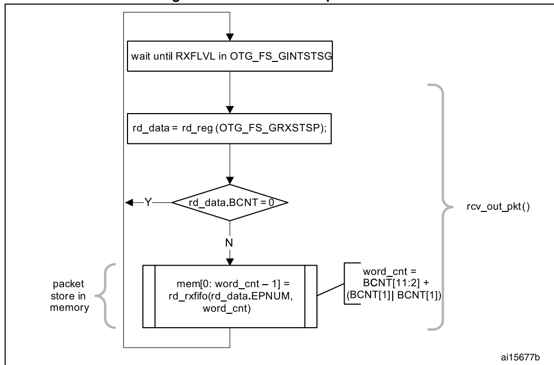
Figure 756. Receive FIFO packet read
