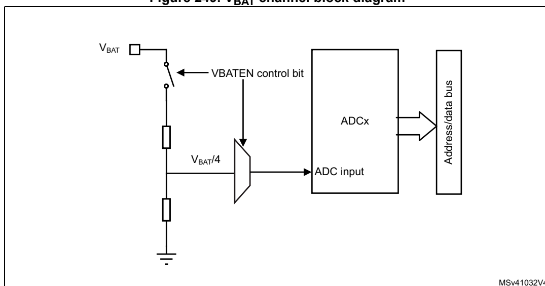
Figure 249. V_{BAT} channel block diagram
