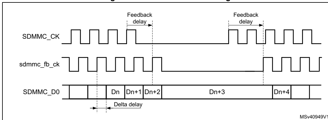
Figure 700. Hardware flow timing
