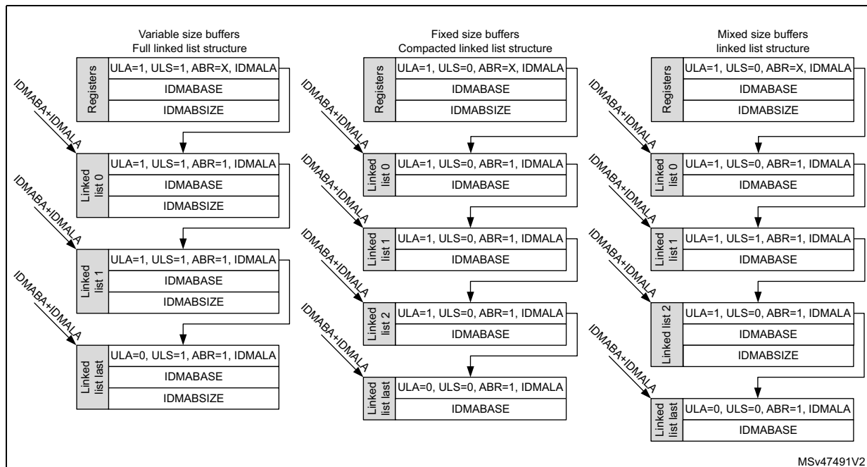
Figure 699. Linked list structures
