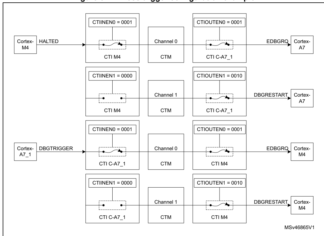
Figure 817. Cross trigger configuration example
