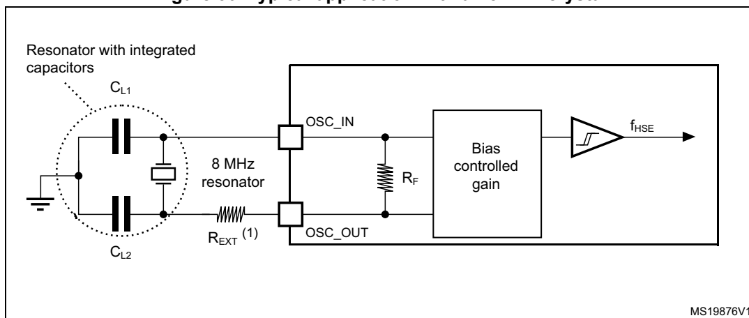
Figure 30. Typical application with an 8 MHz crystal
