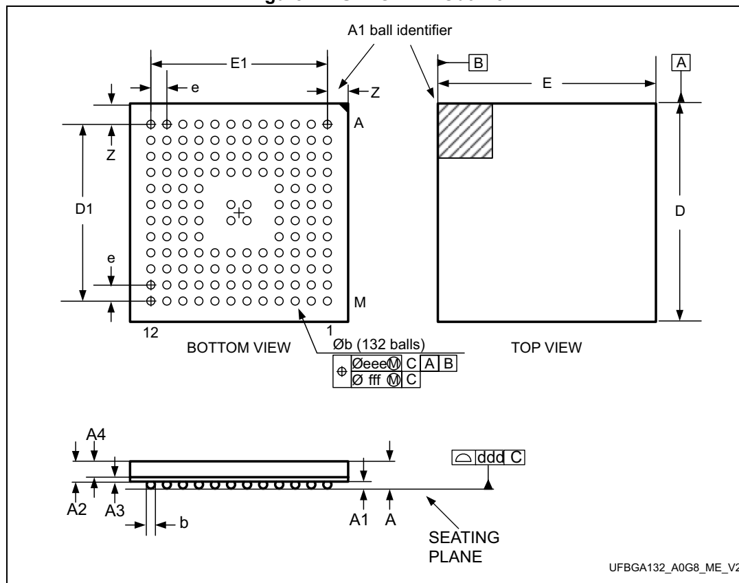
Figure 71. UFBGA12 - Outline
