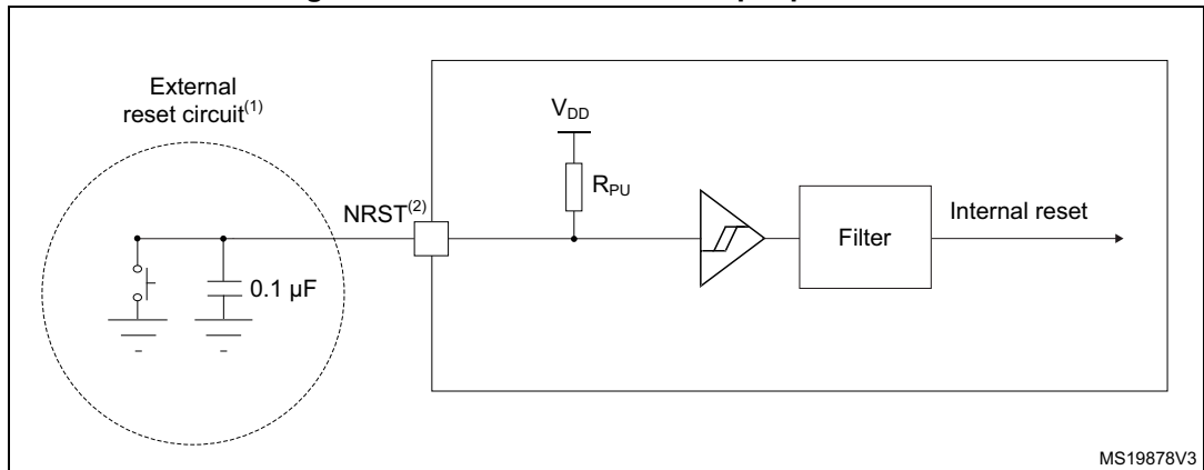
Figure 34. Recommended NRST pin protection
