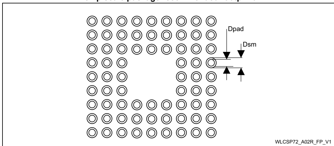
Figure 64. WLCSP72 - 72-ball, 4.4084 x 3.7594 mm, 0.4 mm pitch wafer level chip scale package recommended footprint
