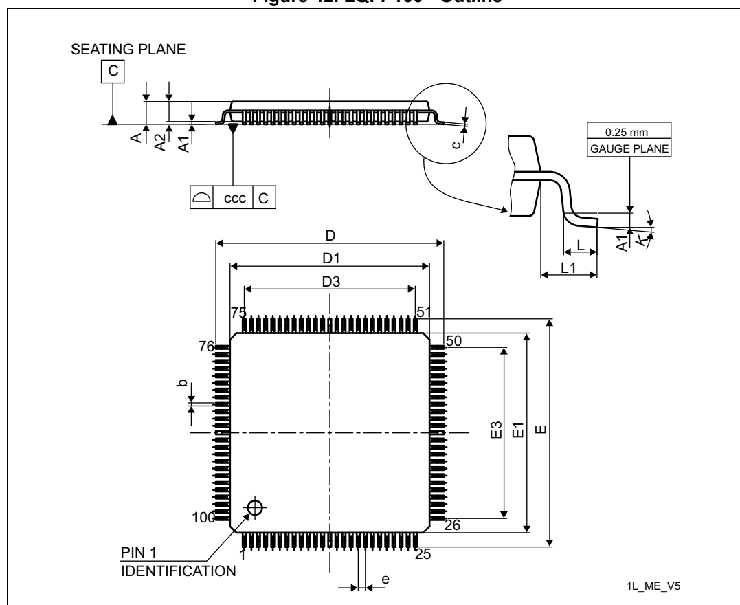
Figure 42. LQFP100 - Outline
