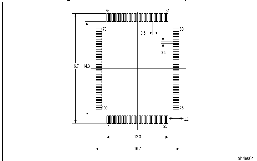
Figure 43. LQFP100 - Recommended footprint
