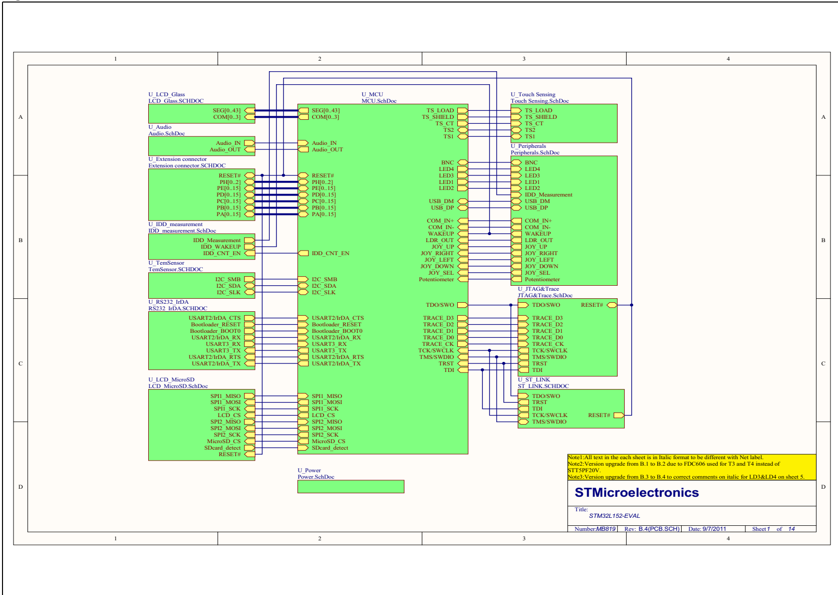
Figure 13. STM32L152-EVAL
