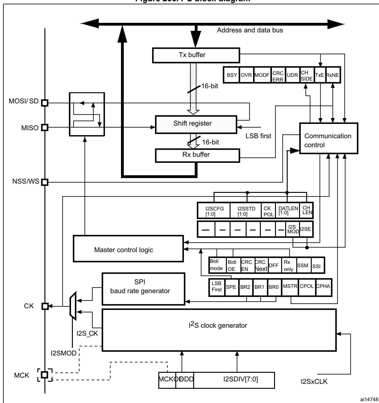
Figure 256. I 2 S block diagram
