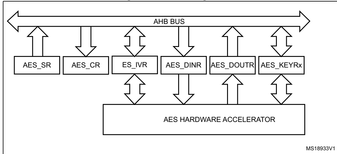
Figure 169. Block diagram
