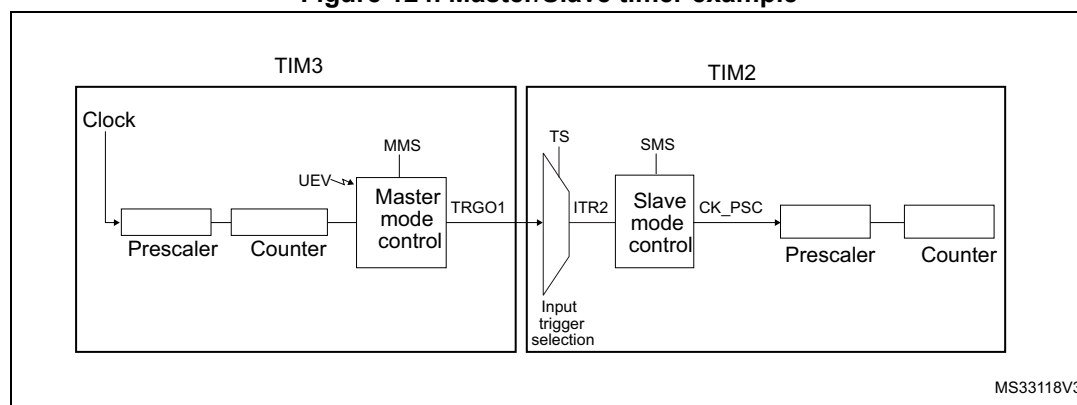
Figure 124. Master/Slave timer example
