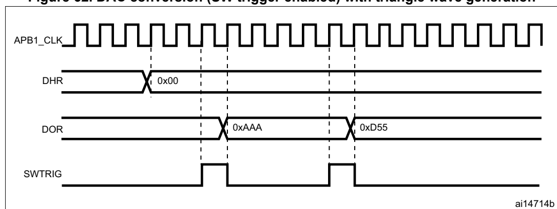
Figure 62. DAC conversion (SW trigger enabled) with triangle wave generation
