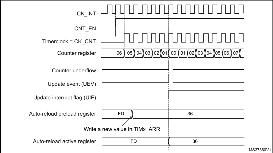
Figure 102. Counter timing diagram, Update event with ARPE=1 (counter underflow)
