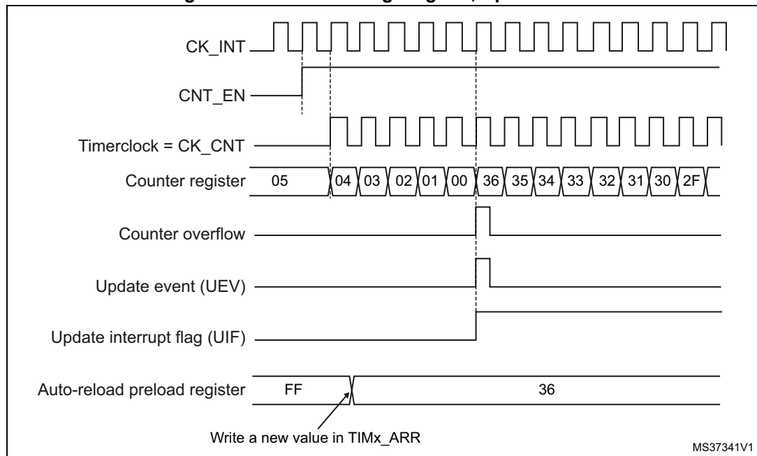
Figure 97. Counter timing diagram, Update event
