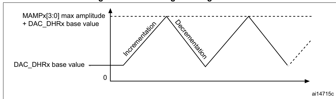
Figure 61. DAC triangle wave generation
