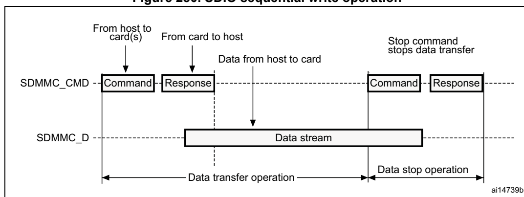
Figure 280. SDIO sequential write operation
