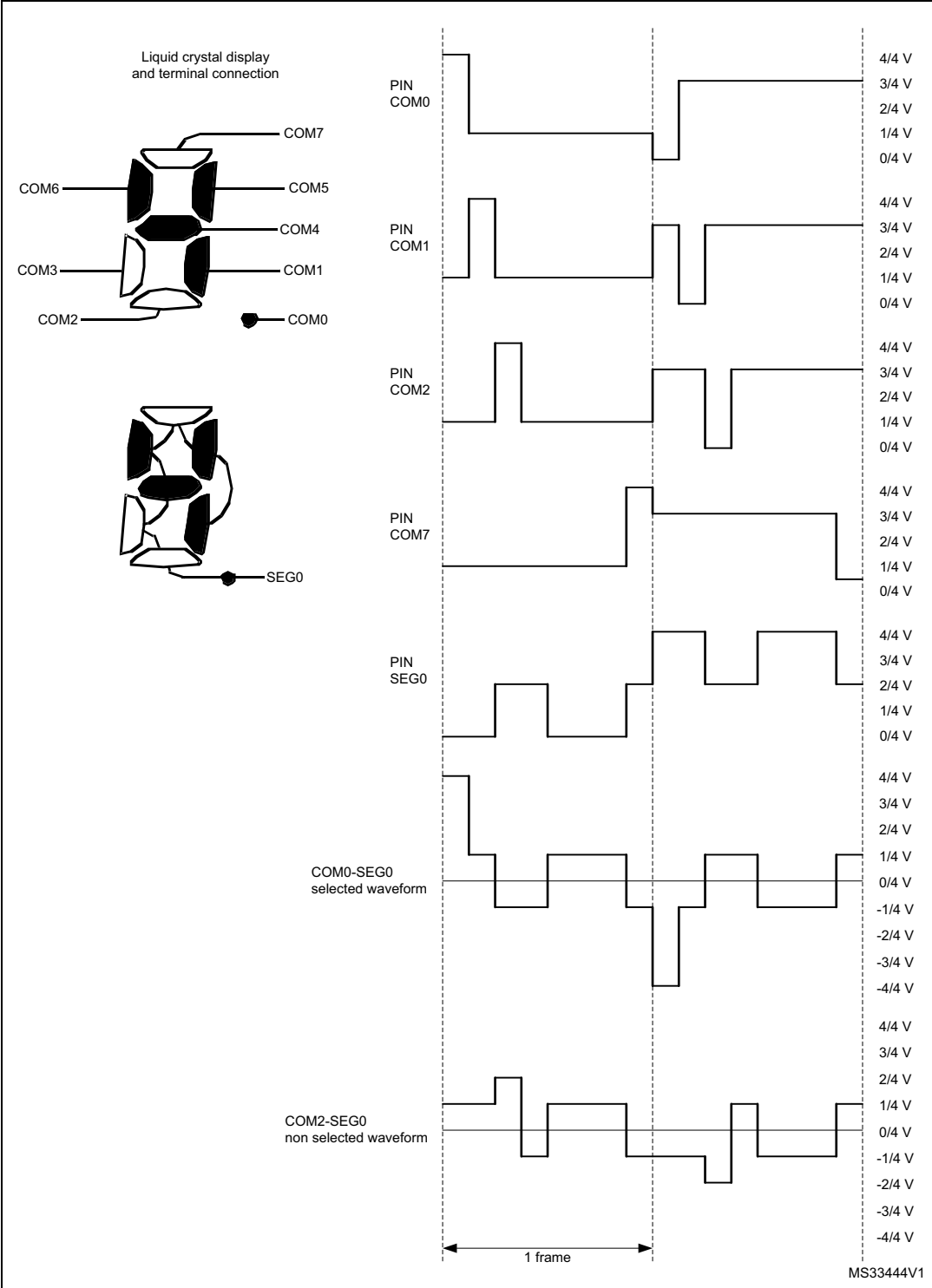
Figure 79. 1/8 duty, 1/4 bias
