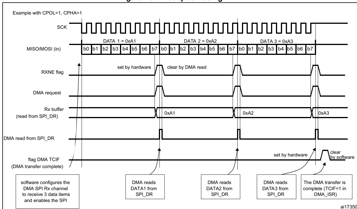
Figure 254. Reception using DMA
