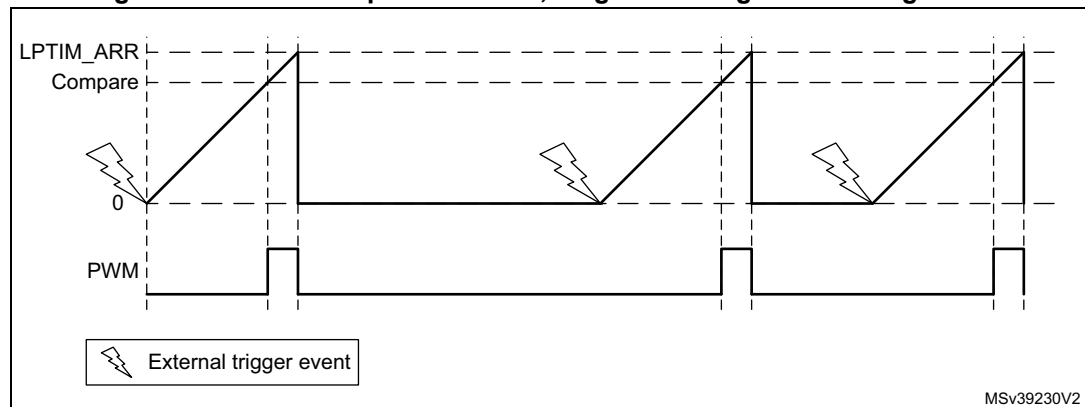
Figure 197. LPTIM output waveform, single counting mode configuration
