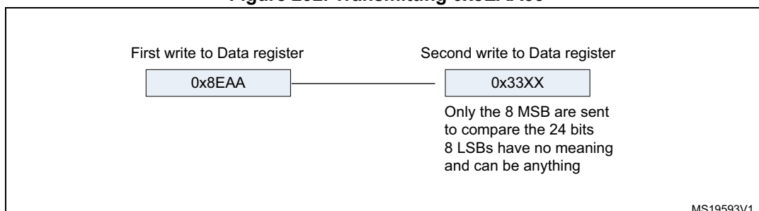
Figure 292. Transmitting 0x8EAA33
