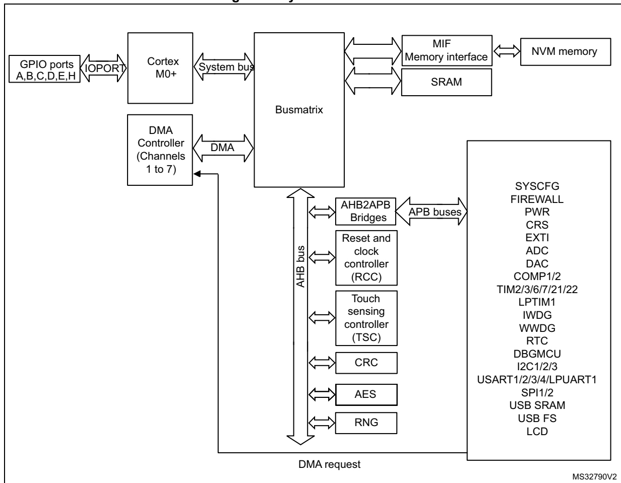
Figure 1. System architecture
