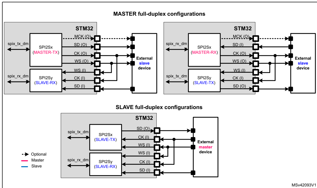
Figure 289. Full-duplex communication
