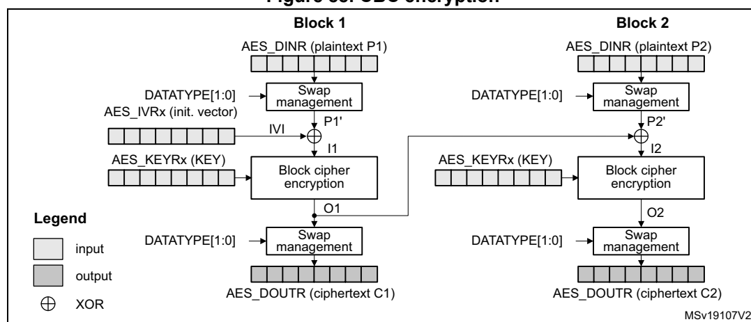
Figure 88. CBC encryption
