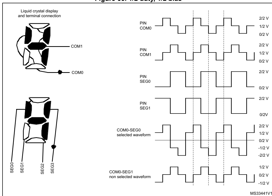
Figure 66. 1/2 duty, 1/2 bias
