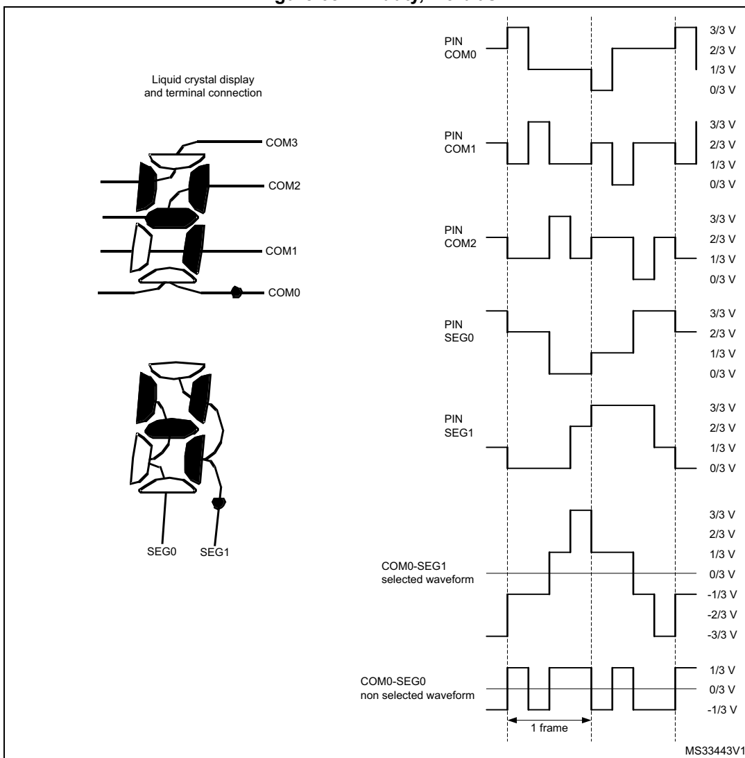
Figure 68. 1/4 duty, 1/3 bias
