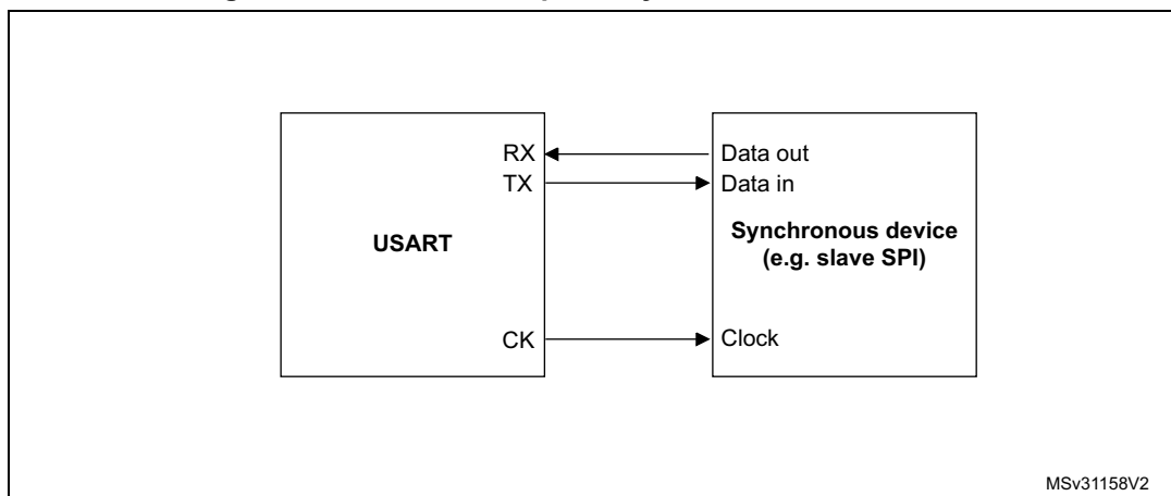
Figure 249. USART example of synchronous transmission
