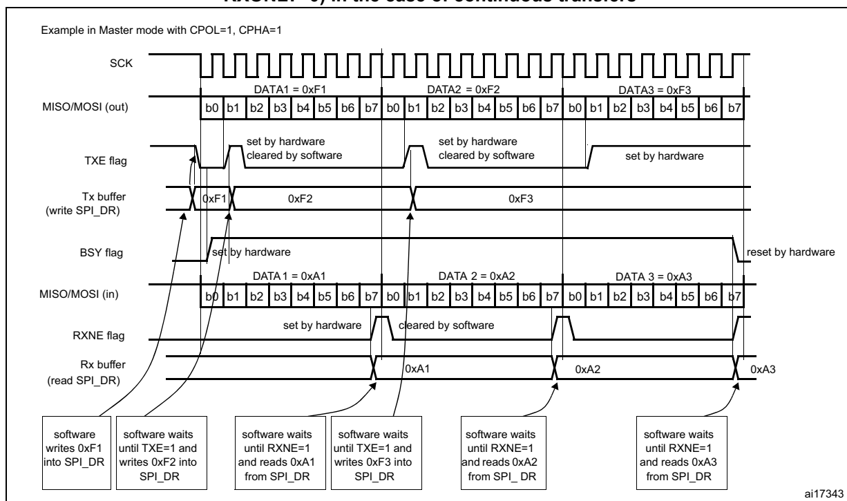
Figure 283. TXE/RXNE/BSY behavior in master / full-duplex mode (BIDIMODE=0, RXONLY=0) in the case of continuous transfers
