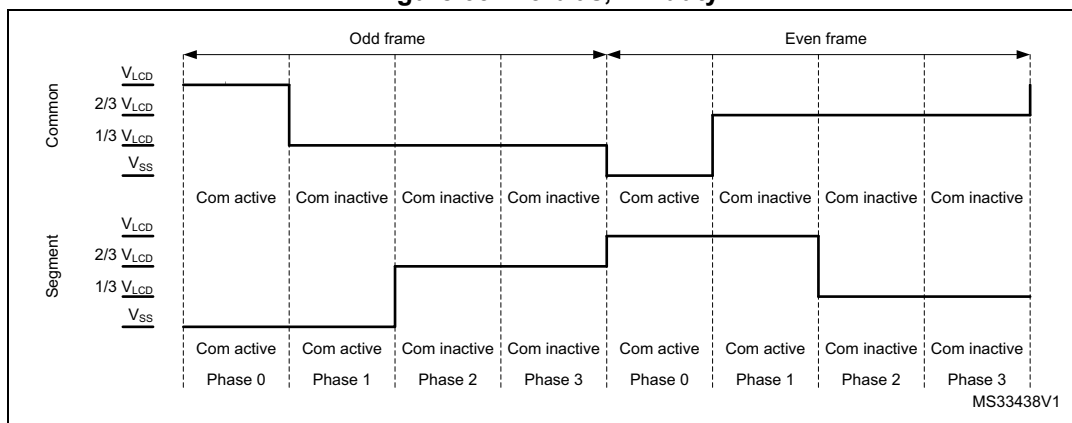
Figure 63. 1/3 bias, 1/4 duty
