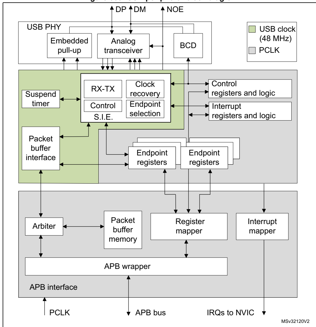
Figure 309. USB peripheral block diagram
