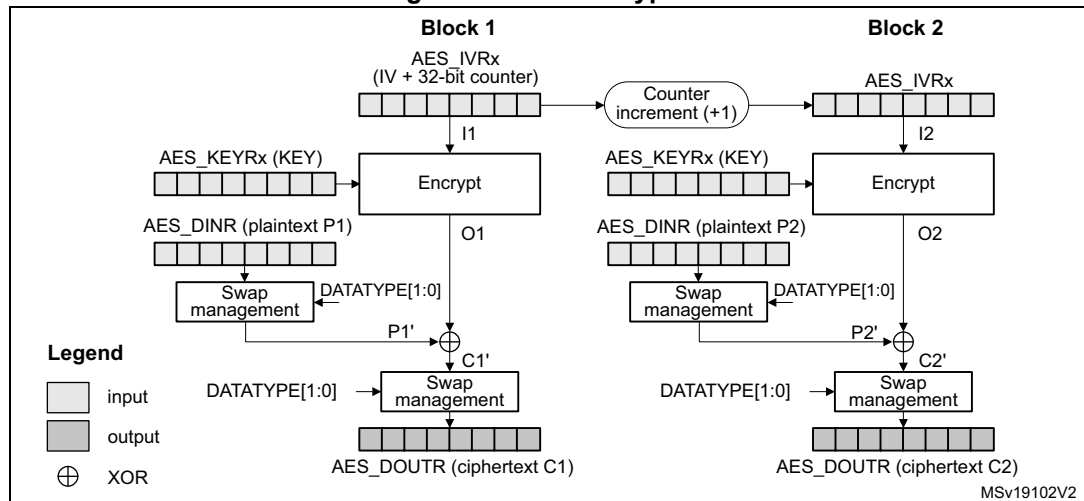
Figure 93. CTR encryption
