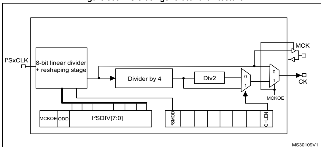
Figure 308. I 2 S clock generator architecture
