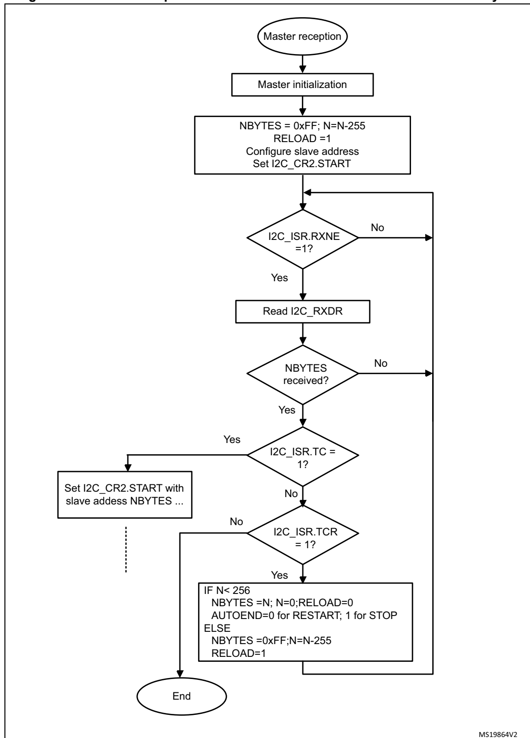
Figure 228. Transfer sequence flowchart for I2C master receiver for N &gt; 255 bytes
