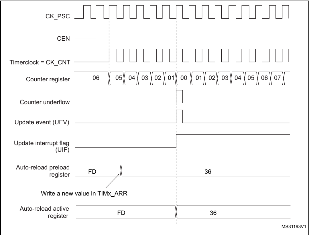
Figure 119. Counter timing diagram, Update event with ARPE=1 (counter underflow)
