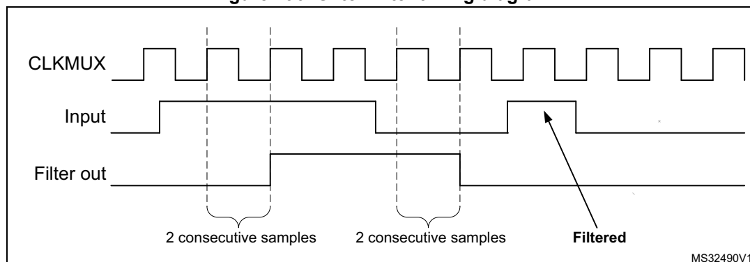
Figure 196. Glitch filter timing diagram
