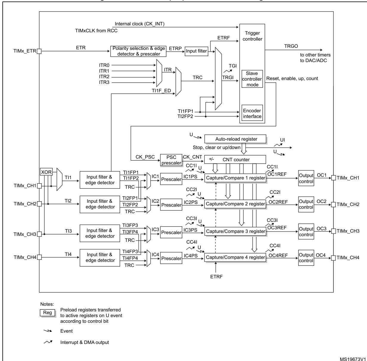
Figure 101. General-purpose timer block diagram
