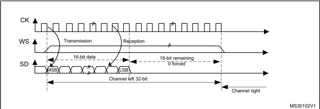
Figure 298. MSB justified 16-bit extended to 32-bit packet frame with CPOL = 0
