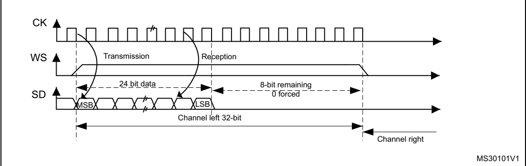
Figure 297. MSB justified 24-bit frame length with CPOL = 0
