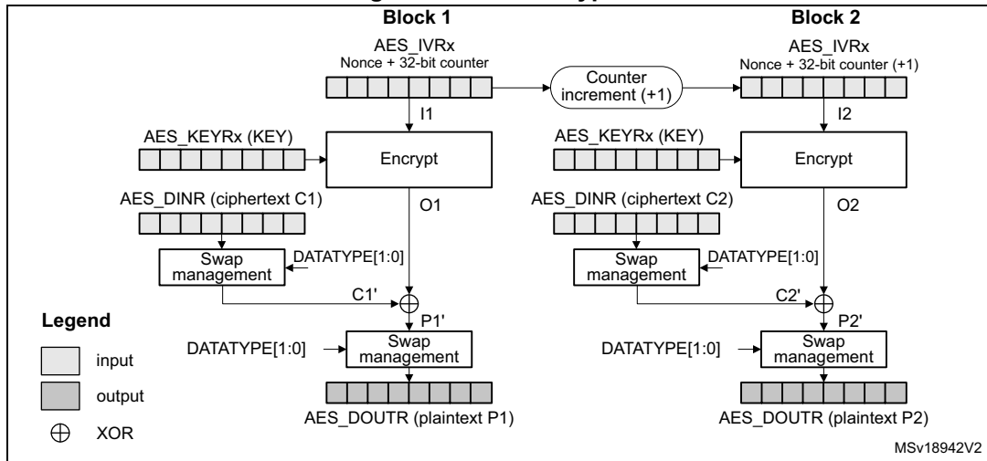
Figure 94. CTR decryption
