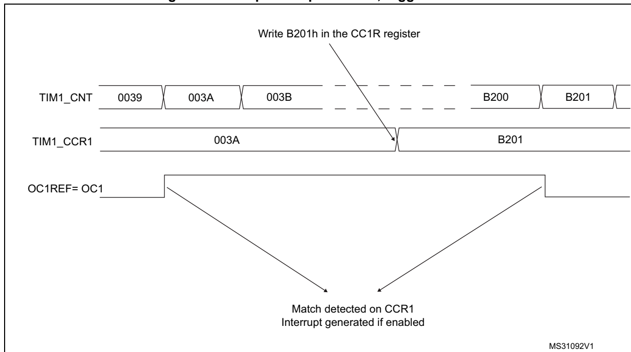
Figure 130. Output compare mode, toggle on OC1.
