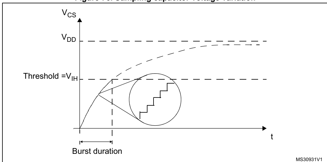
Figure 76. Sampling capacitor voltage variation
