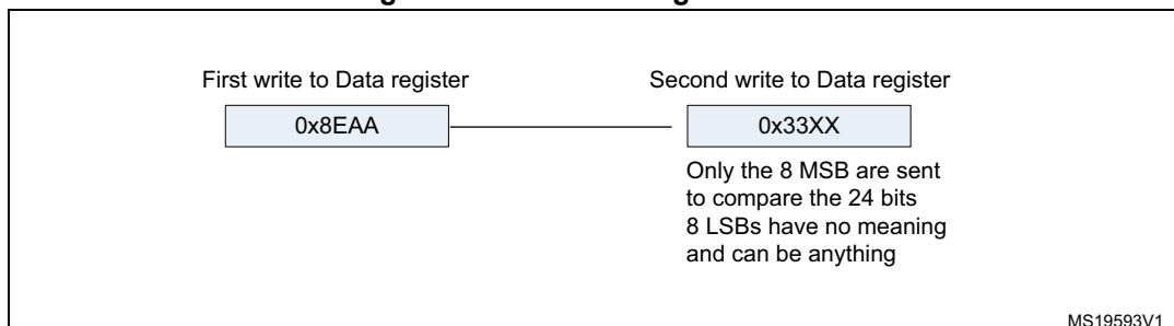
Figure 292. Transmitting 0x8EAA33
