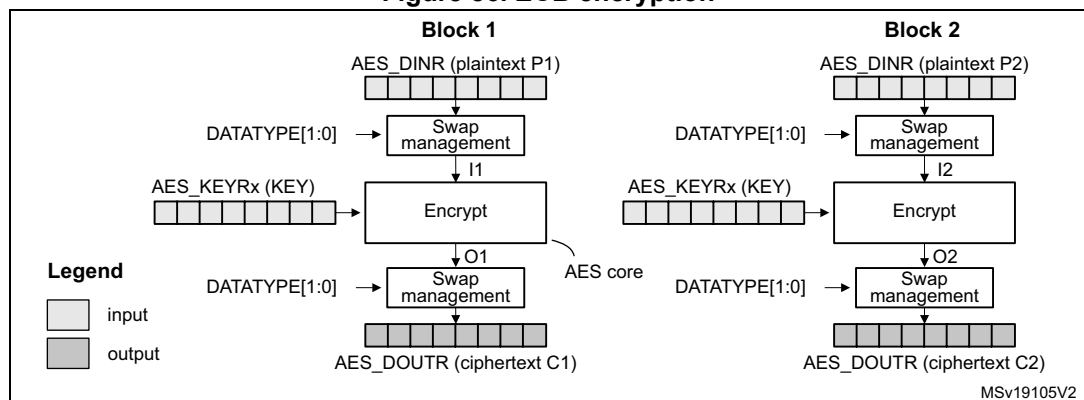
Figure 86. ECB encryption
