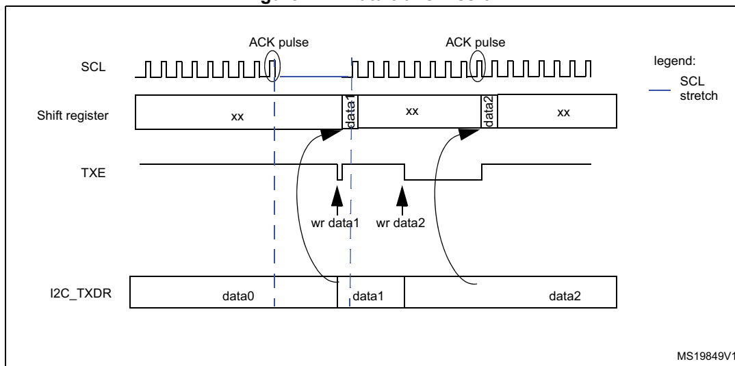
Figure 212. Data transmission
