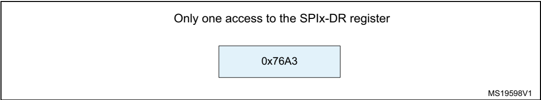
Figure 304. Example of 16-bit data frame extended to 32-bit channel frame
