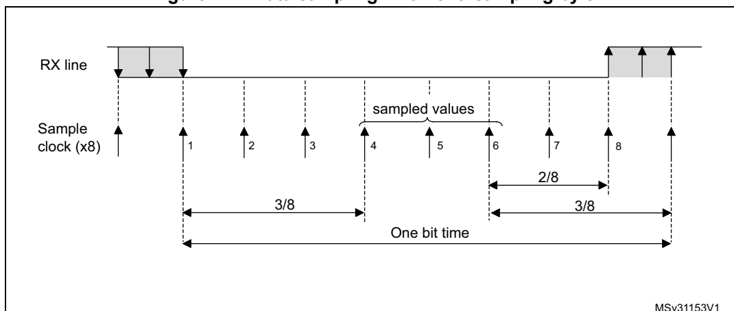
Figure 244. Data sampling when oversampling by 8
