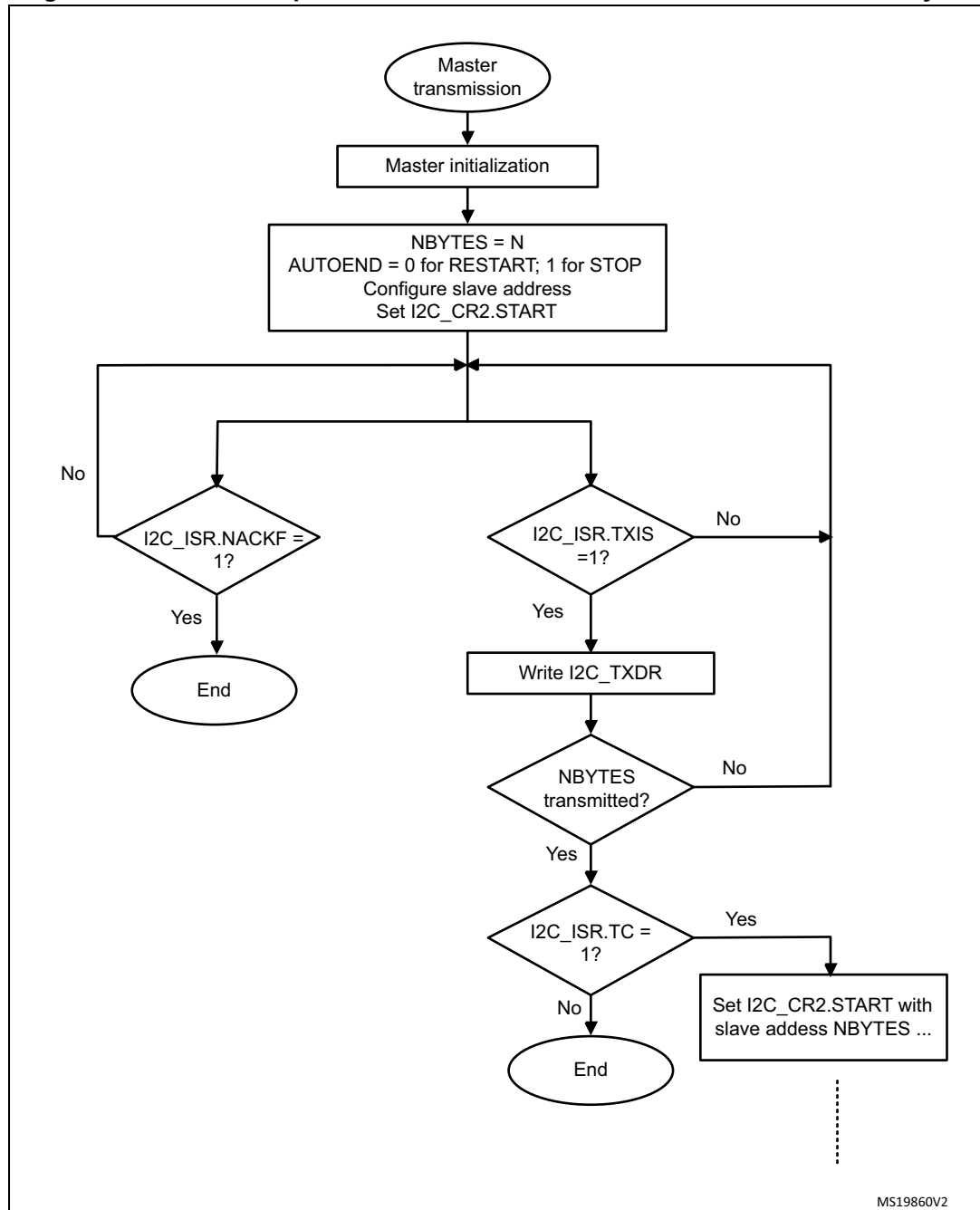
Figure 224. Transfer sequence flowchart for I2C master transmitter for N \leq 255 bytes
