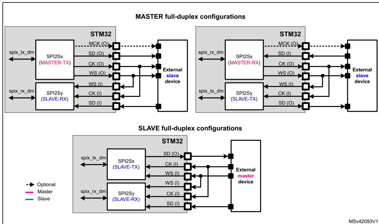
Figure 289. Full-duplex communication
