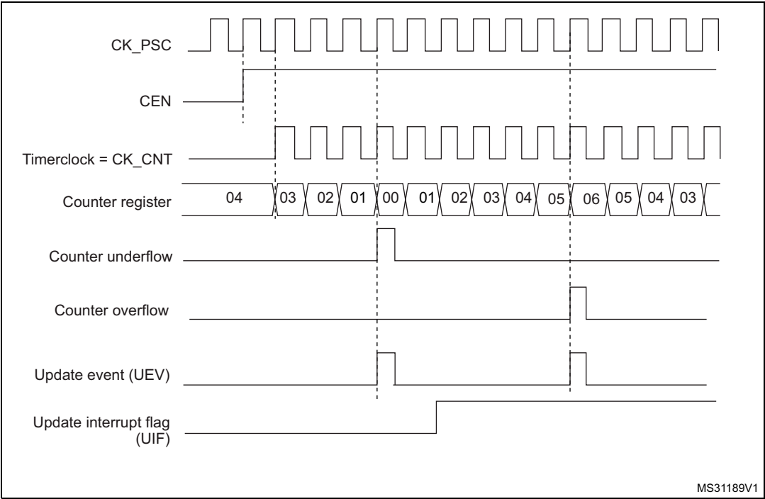
Figure 160. Counter timing diagram, internal clock divided by 1, TIMx_ARR=0x6
