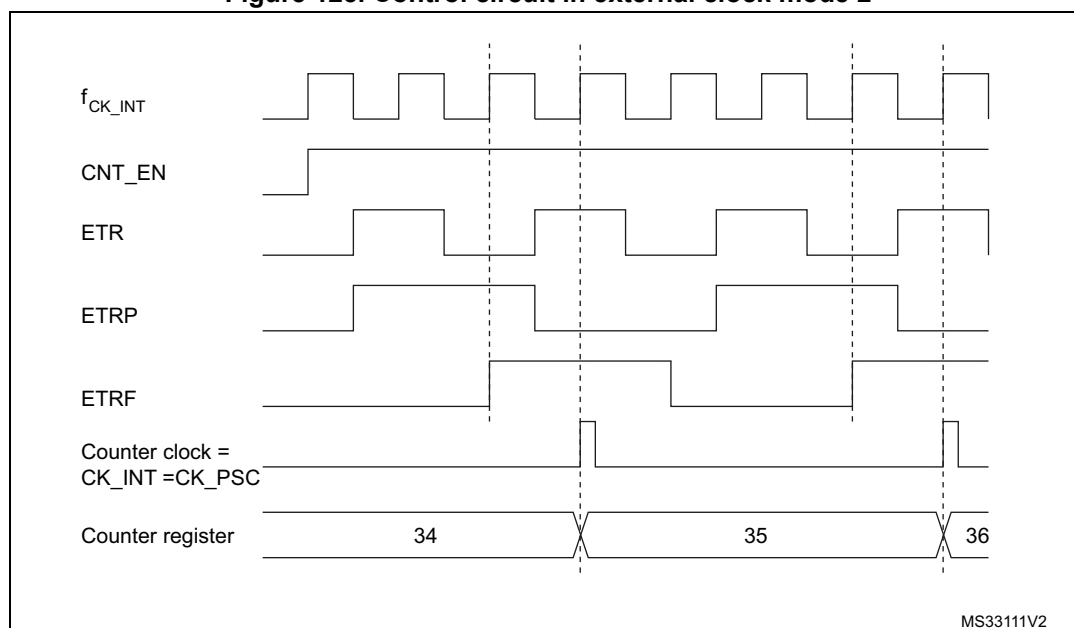
Figure 125. Control circuit in external clock mode 2
