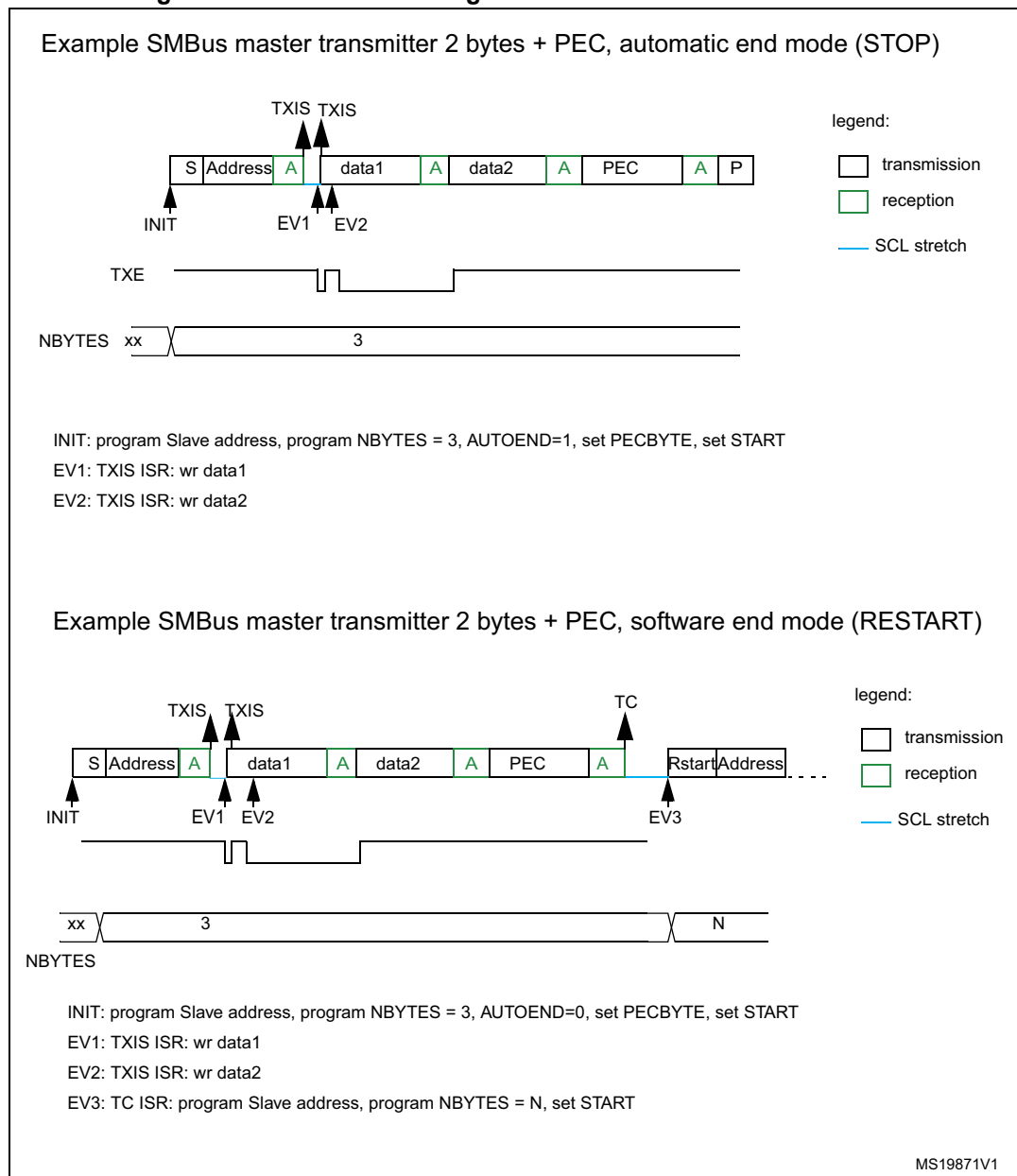
Figure 235. Bus transfer diagrams for SMBus master transmitter
