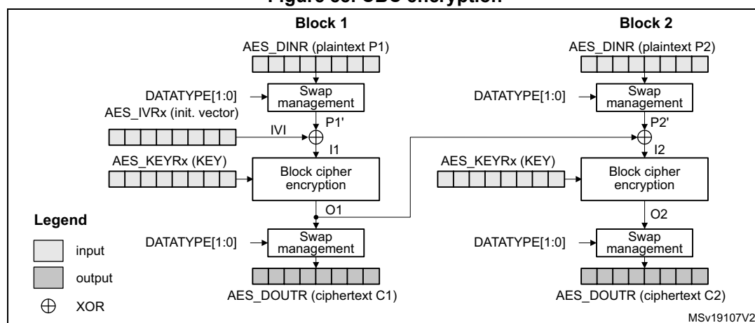
Figure 88. CBC encryption
