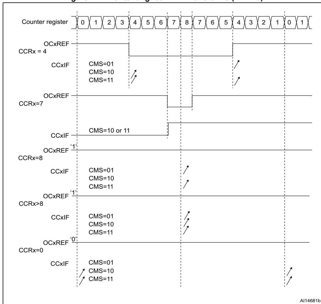
Figure 177. Center-aligned PWM waveforms (ARR=8)
