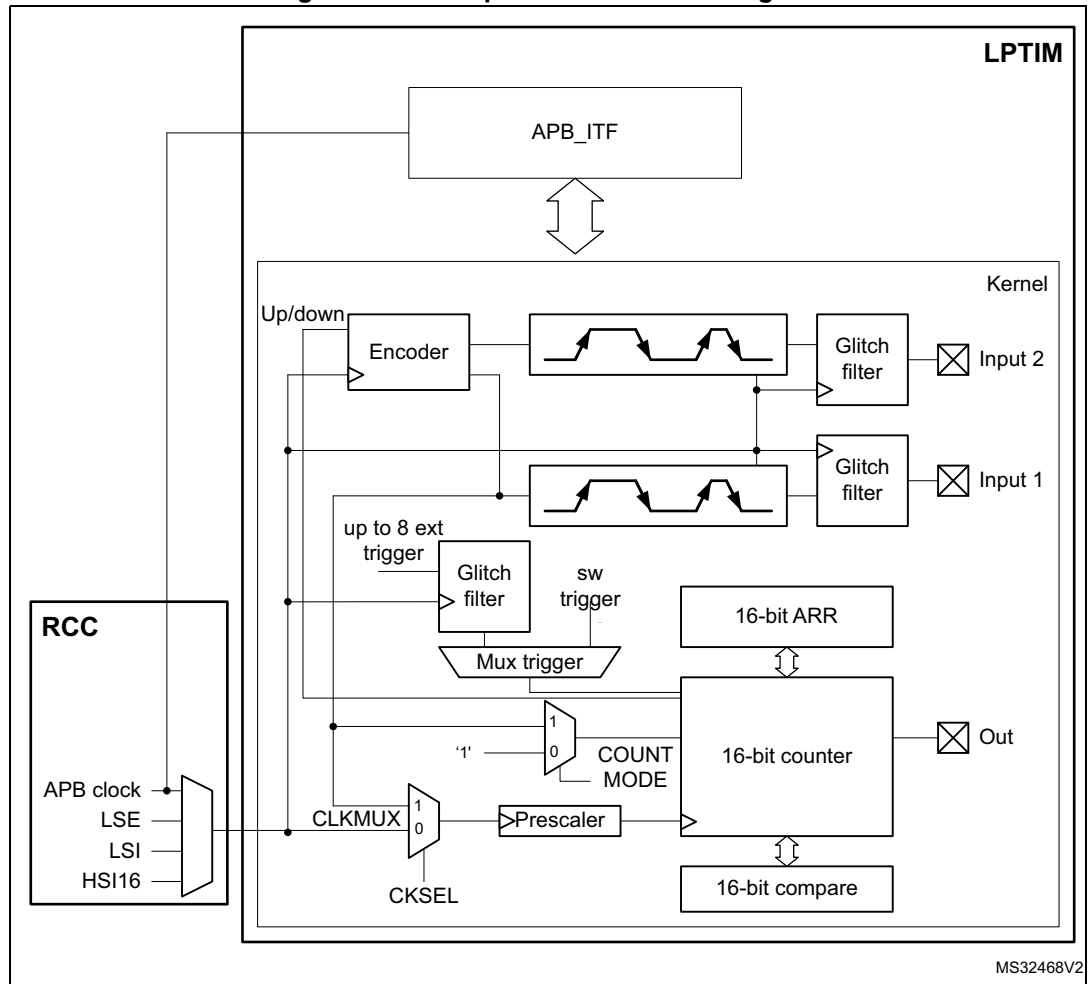
Figure 195. Low-power timer block diagram
