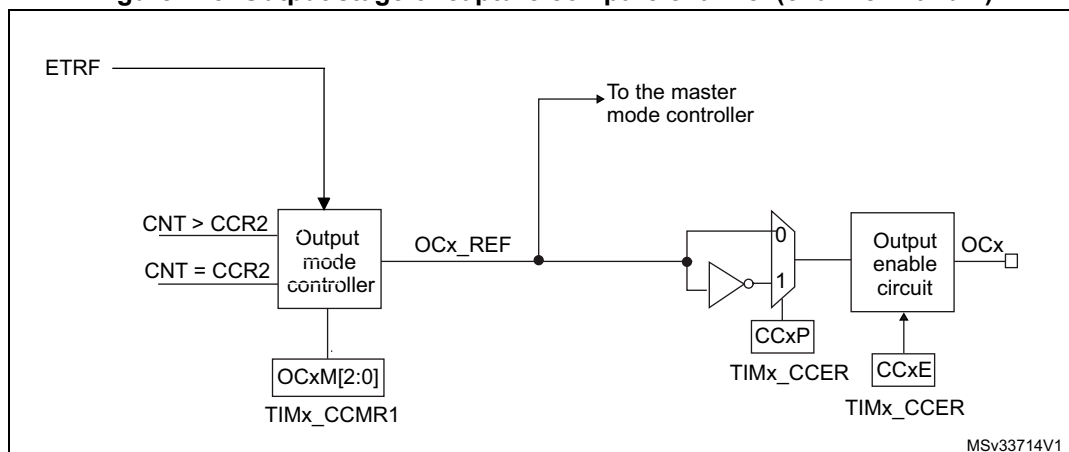
Figure 173. Output stage of capture/compare channel (channel 1 and 2)
