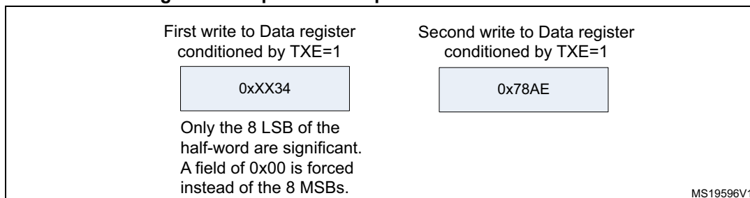
Figure 301. Operations required to transmit 0x3478AE
