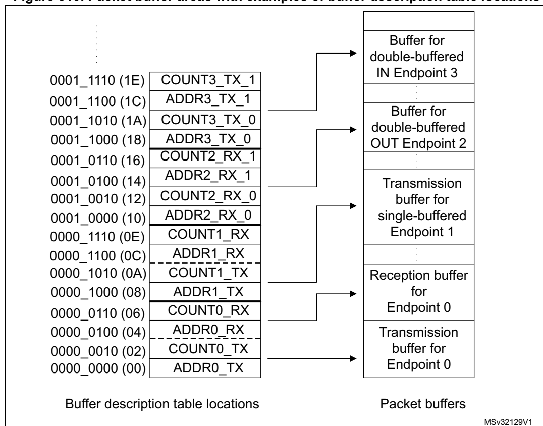
Figure 310. Packet buffer areas with examples of buffer description table locations
