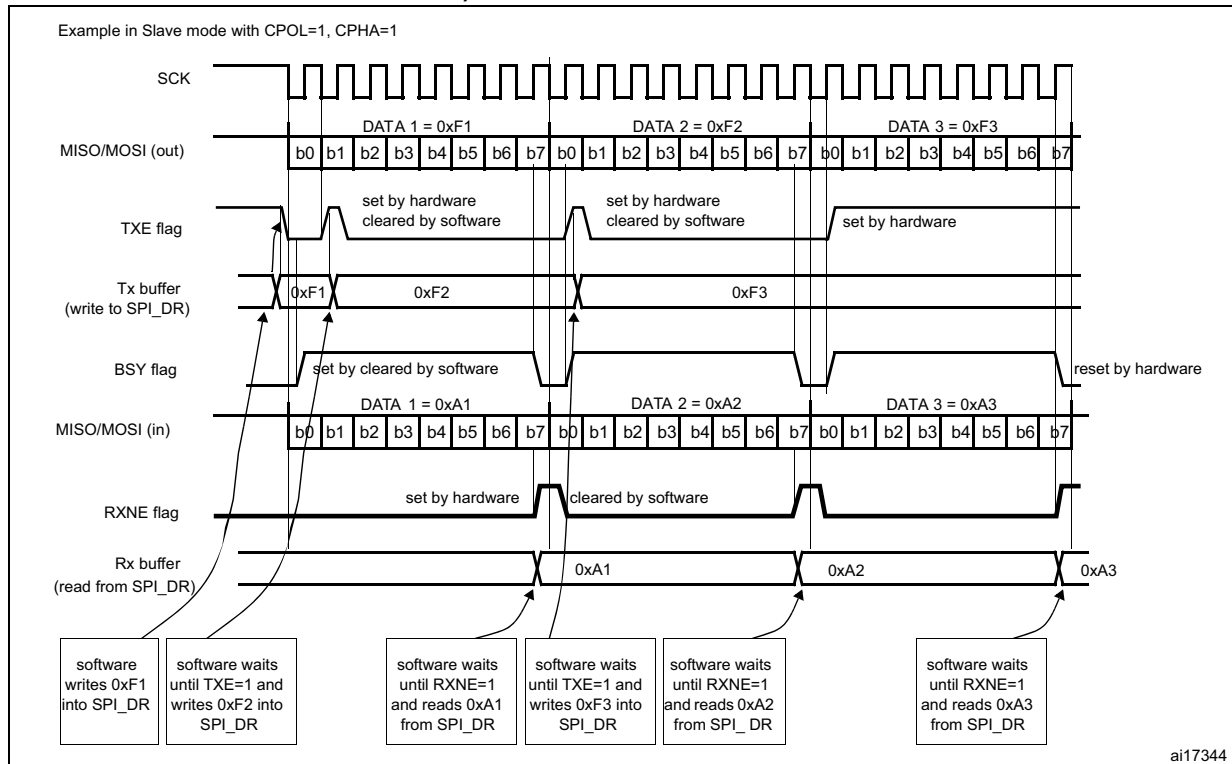
Figure 284. TXE/RXNE/BSY behavior in slave / full-duplex mode (BIDIMODE=0, RXONLY=0) in the case of continuous transfers
