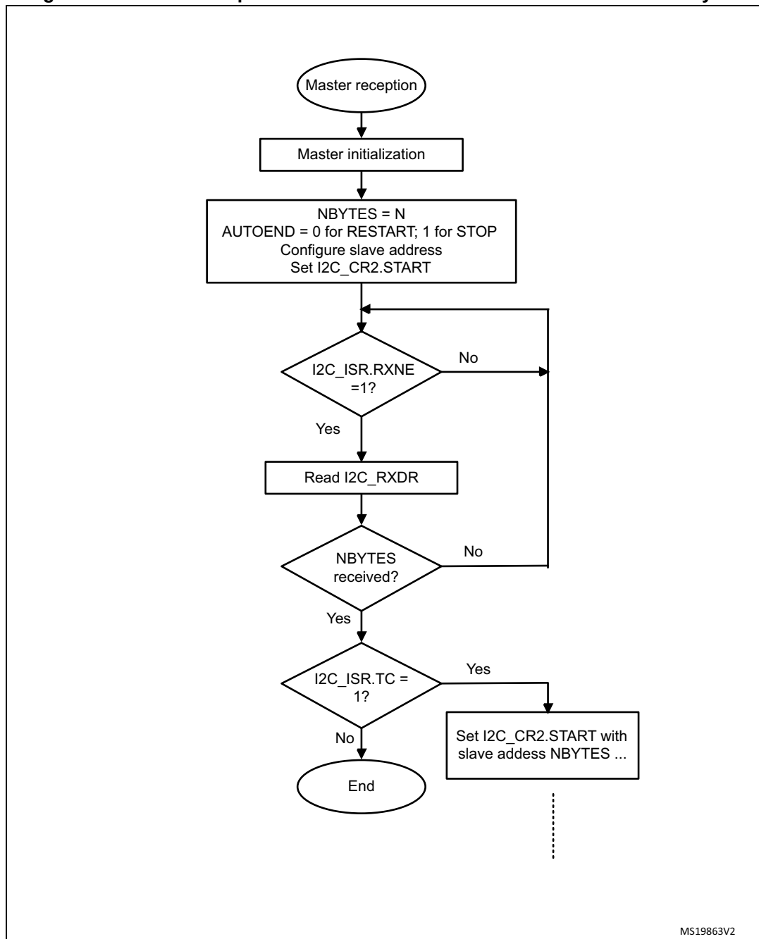
Figure 227. Transfer sequence flowchart for I2C master receiver for N \leq 255 bytes
