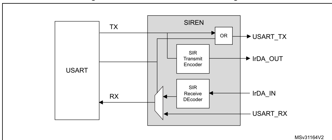
Figure 255. IrDA SIR ENDEC- block diagram
