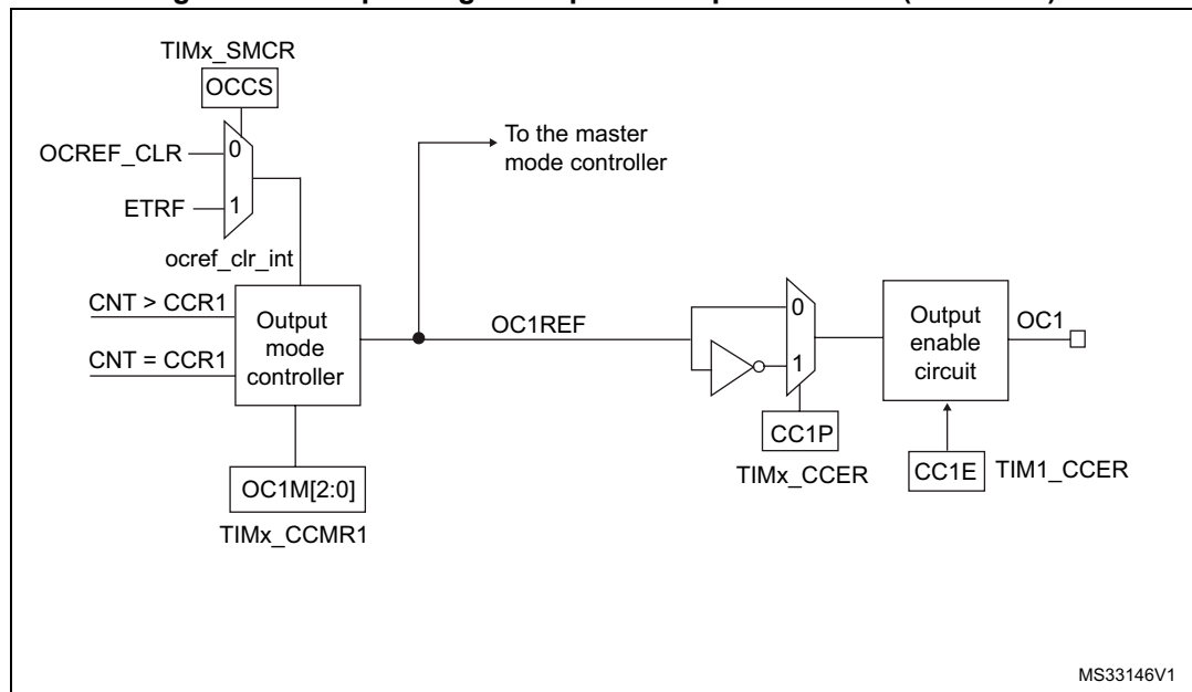
Figure 128. Output stage of capture/compare channel (channel 1)
