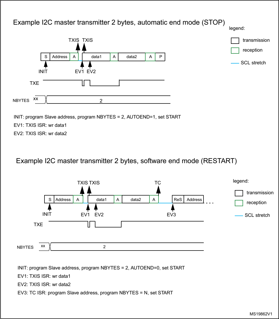
Figure 226. Transfer bus diagrams for I2C master transmitter
