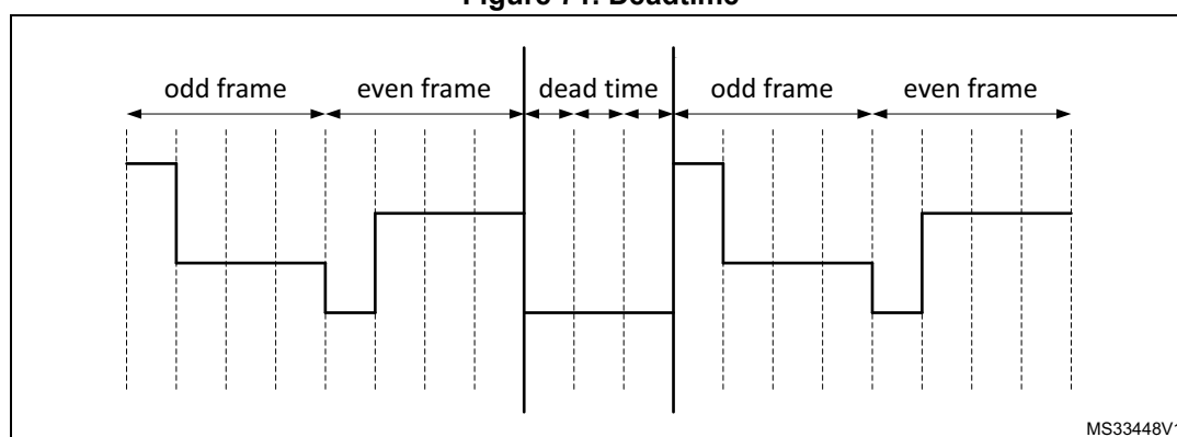
Figure 71. Deadtime
