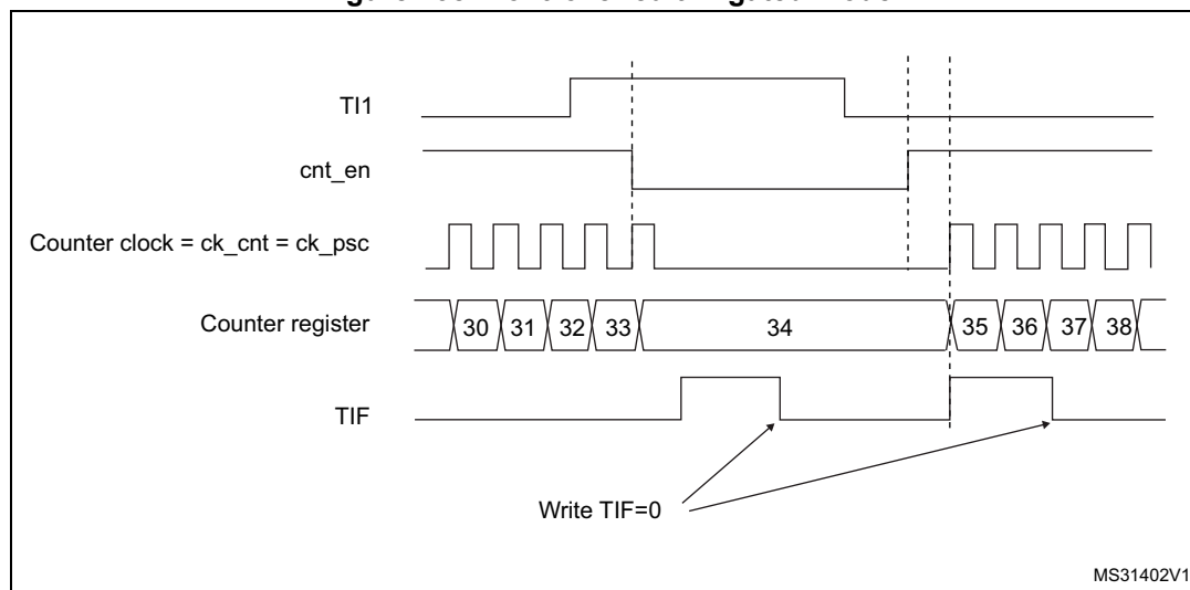
Figure 138. Control circuit in gated mode
