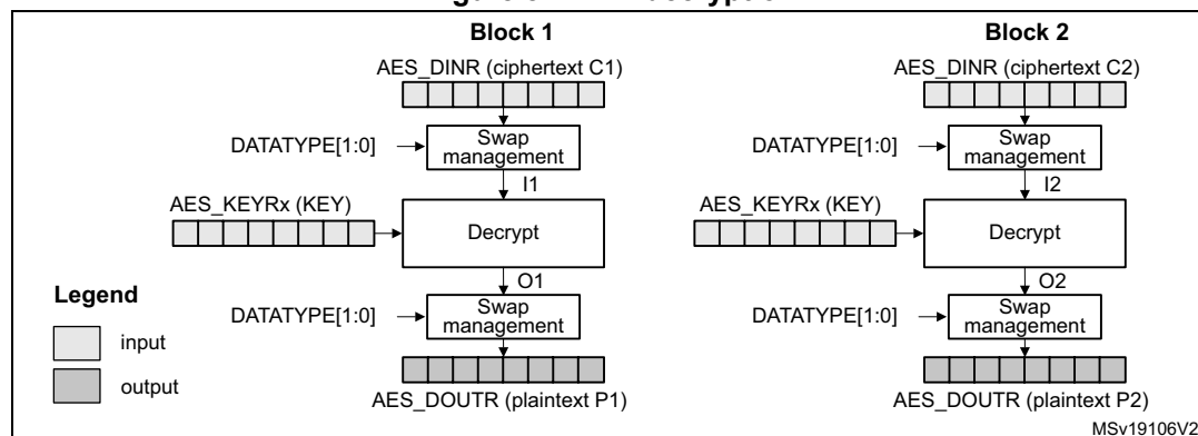
Figure 87. ECB decryption
