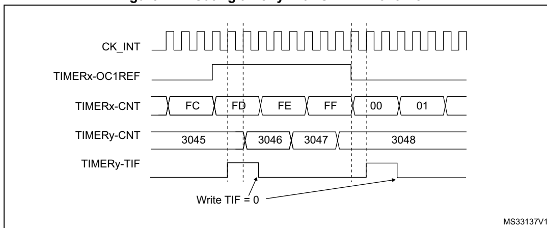
Figure 142. Gating timer y with OC1REF of timer x
