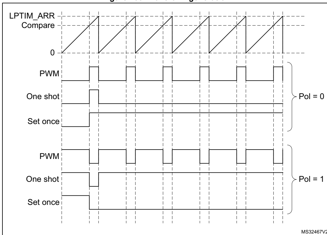
Figure 200. Waveform generation
