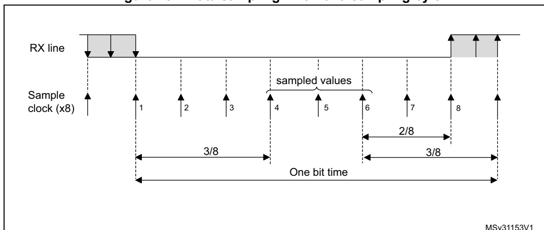
Figure 232. Data sampling when oversampling by 8
