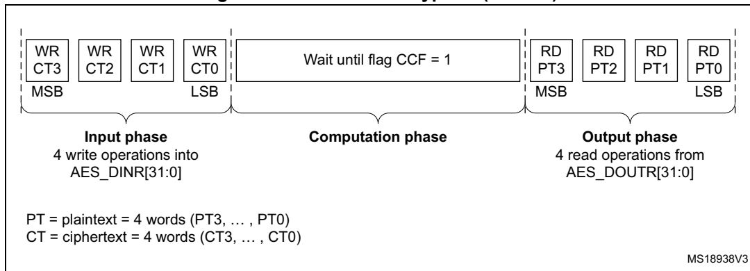
Figure 79. ECB/CBC decryption (Mode 3)
