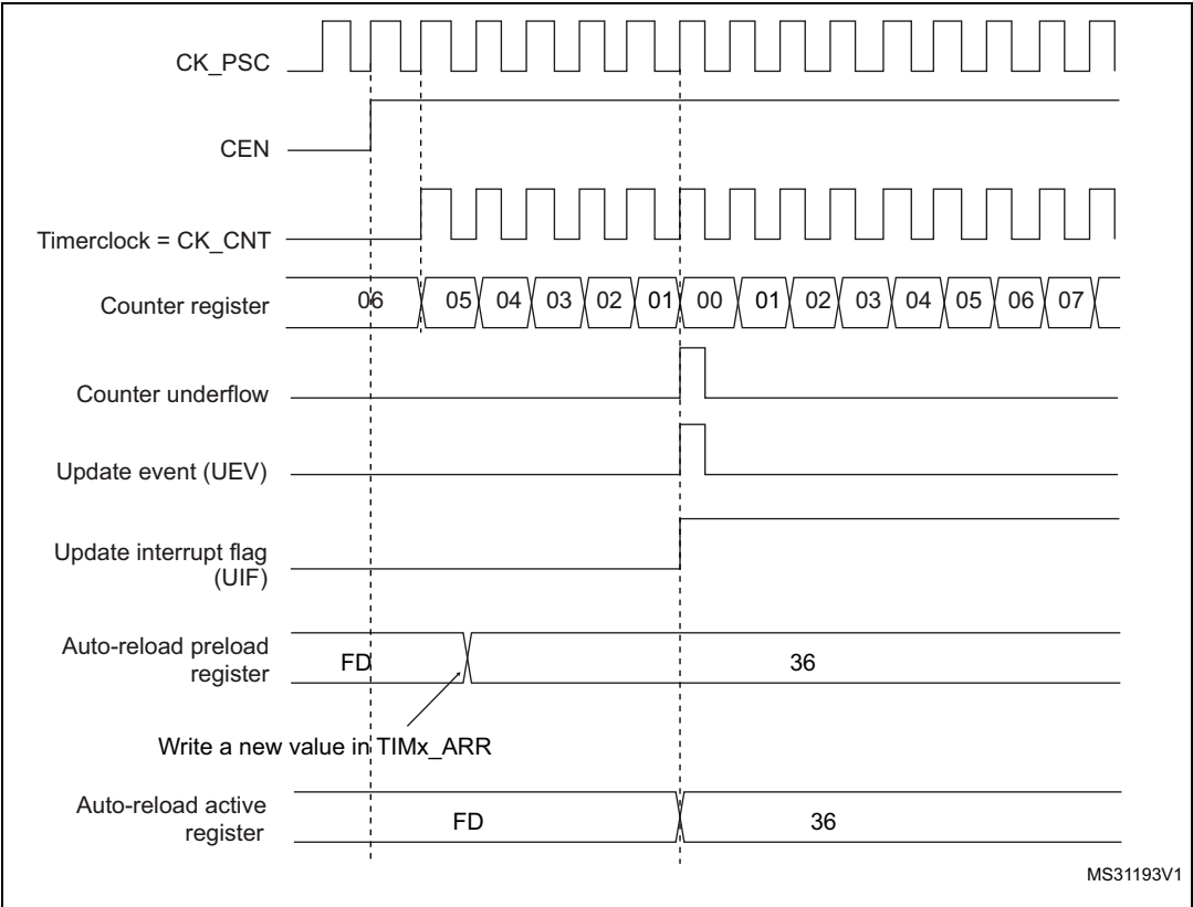
Figure 107. Counter timing diagram, Update event with ARPE=1 (counter underflow)
