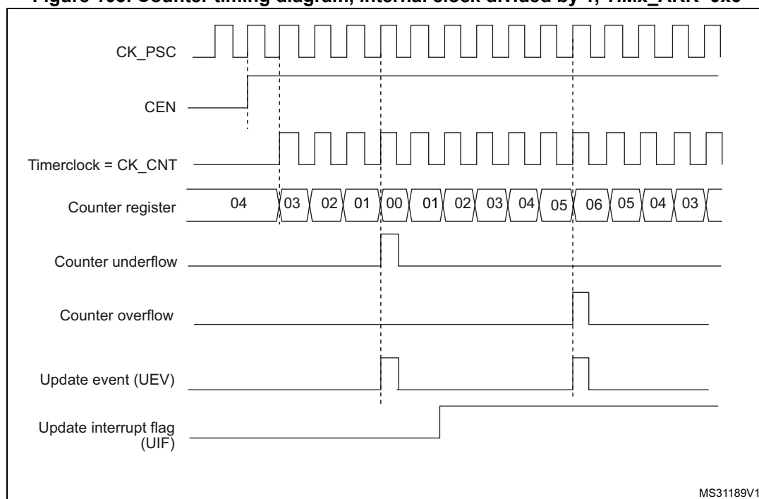
Figure 103. Counter timing diagram, internal clock divided by 1, TIMx_ARR=0x6
