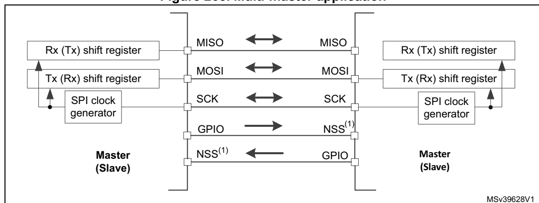
Figure 268. Multi-master application
