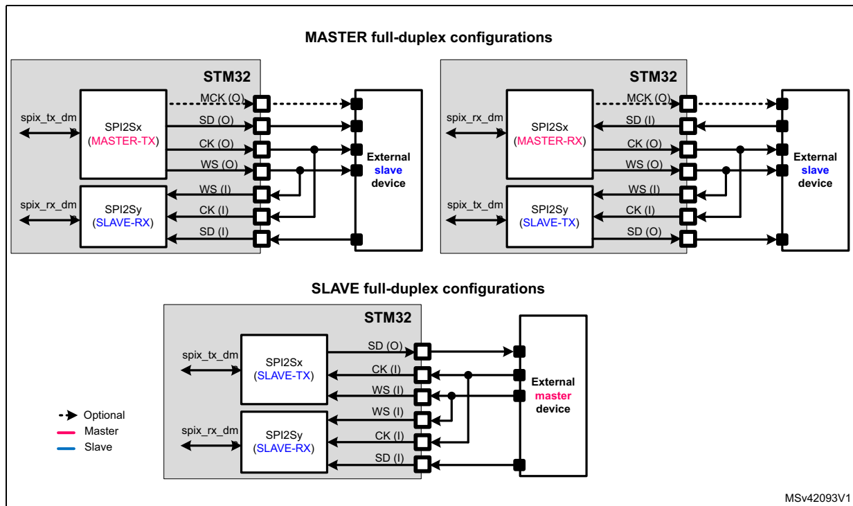
Figure 277. Full-duplex communication
