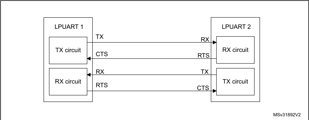
Figure 259. Hardware flow control between 2 LPUARTs
