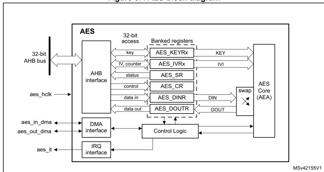
Figure 67. AES block diagram
