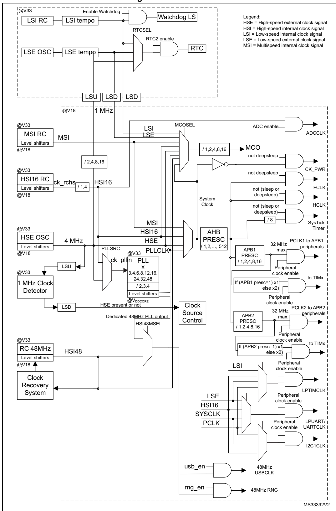
Figure 17. Clock tree
