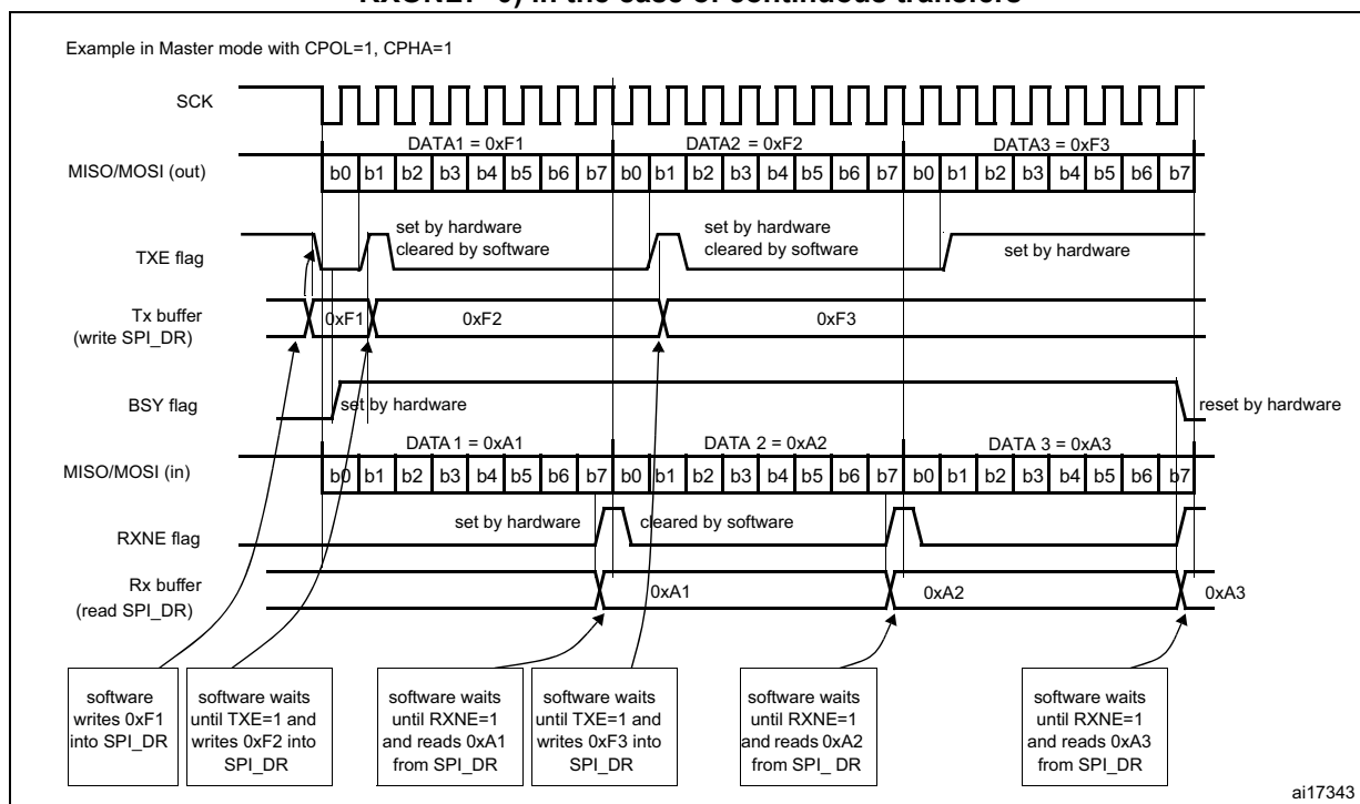
Figure 271. TXE/RXNE/BSY behavior in master / full-duplex mode (BIDIMODE=0, RXONLY=0) in the case of continuous transfers
