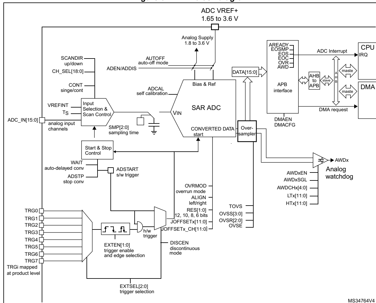
Figure 31. ADC block diagram
