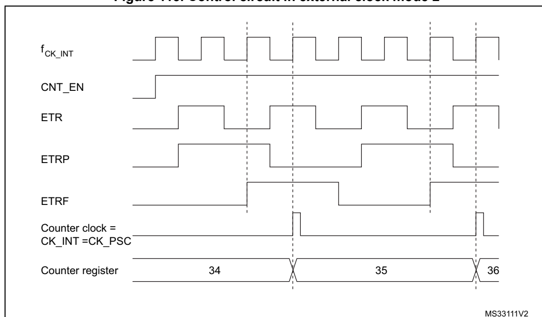
Figure 113. Control circuit in external clock mode 2
