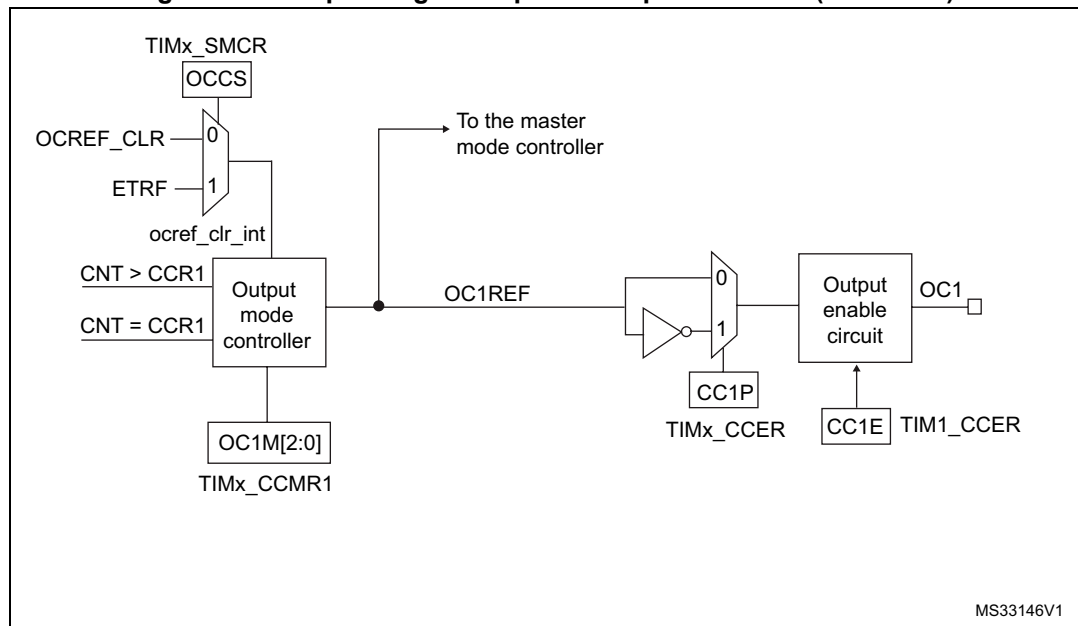
Figure 116. Output stage of capture/compare channel (channel 1)
