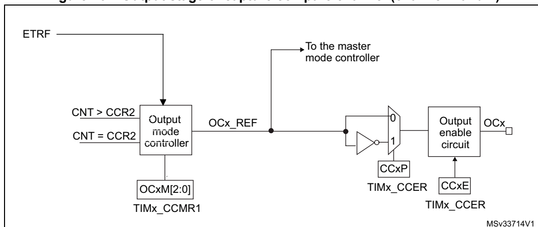
Figure 161. Output stage of capture/compare channel (channel 1 and 2)
