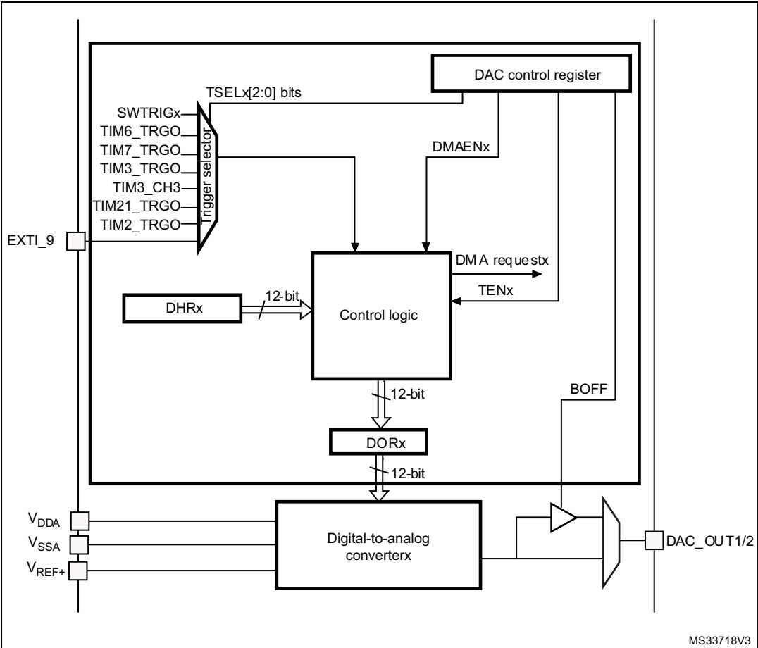
Figure 53. DAC block diagram
