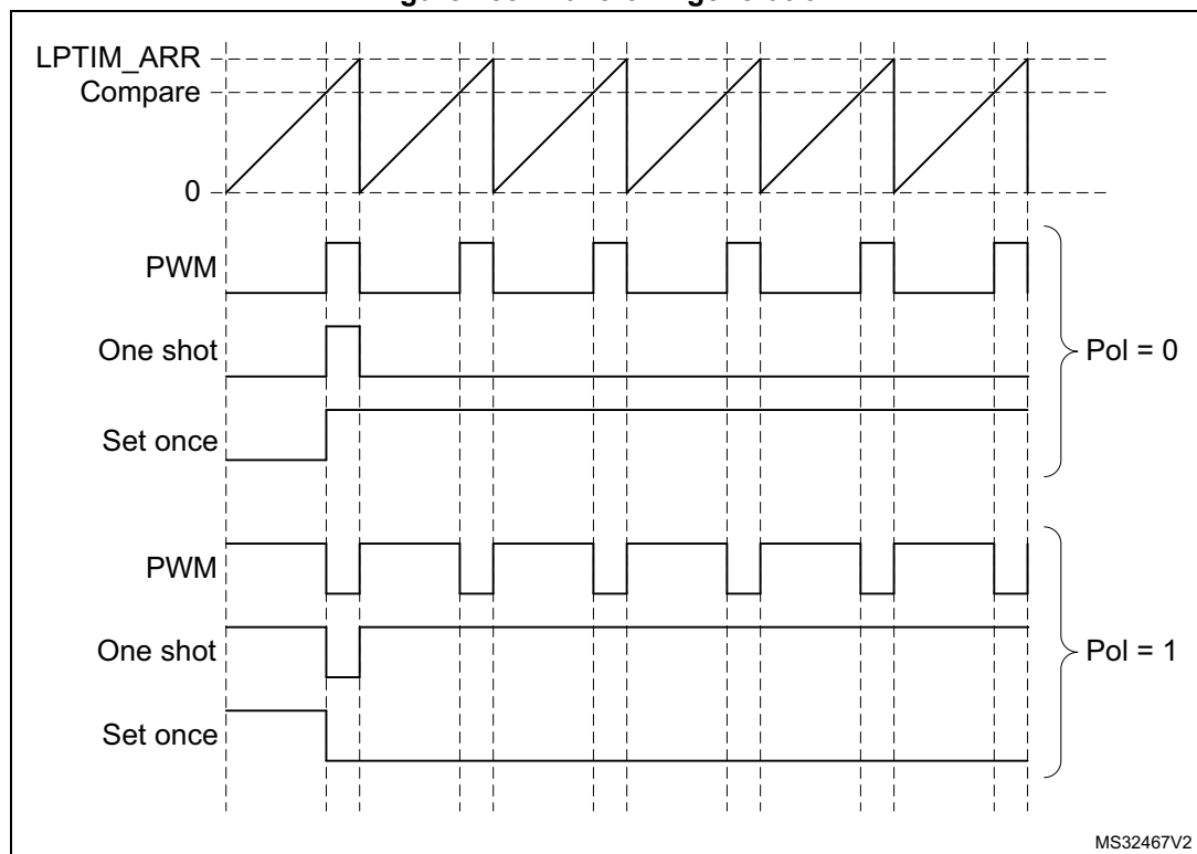
Figure 188. Waveform generation
