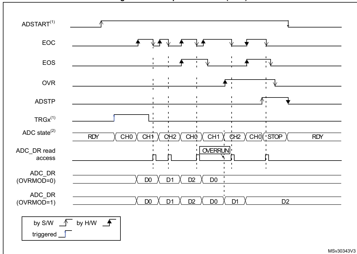
Figure 44. Example of overrun (OVR)
