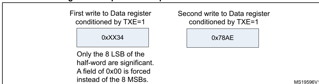
Figure 289. Operations required to transmit 0x3478AE
