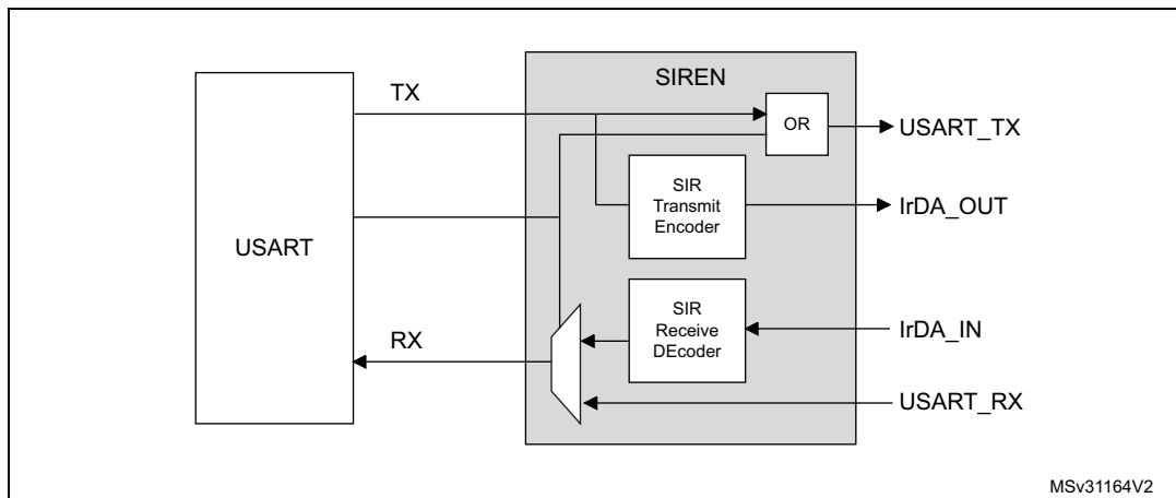
Figure 243. IrDA SIR ENDEC- block diagram
