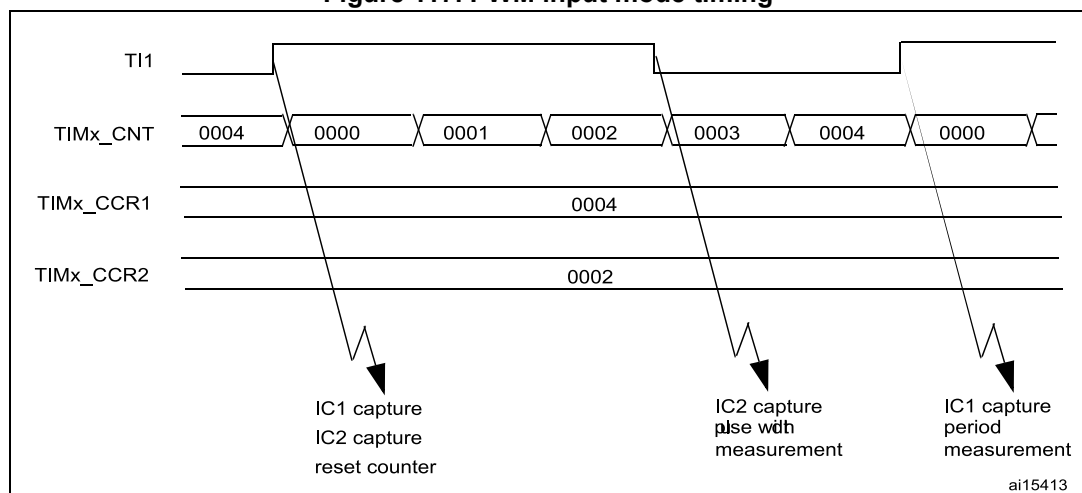
Figure 117. PWM input mode timing
