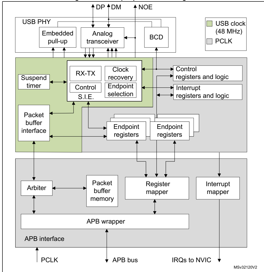
Figure 297. USB peripheral block diagram
