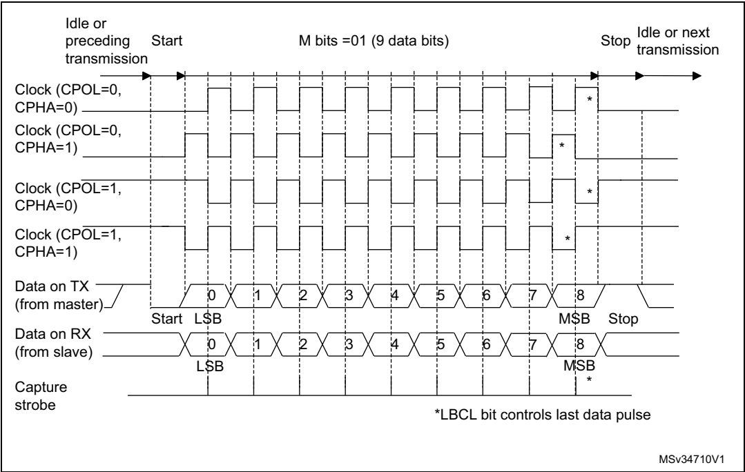
Figure 239. USART data clock timing diagram (M bits = 01)
