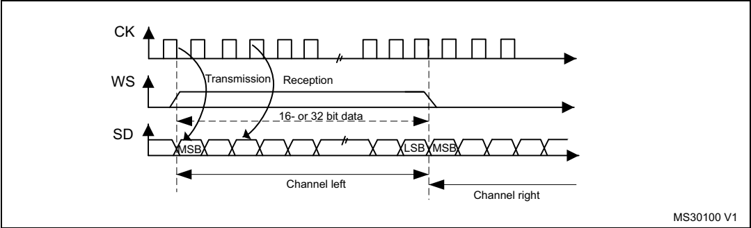
Figure 284. MSB Justified 16-bit or 32-bit full-accuracy length with CPOL = 0
