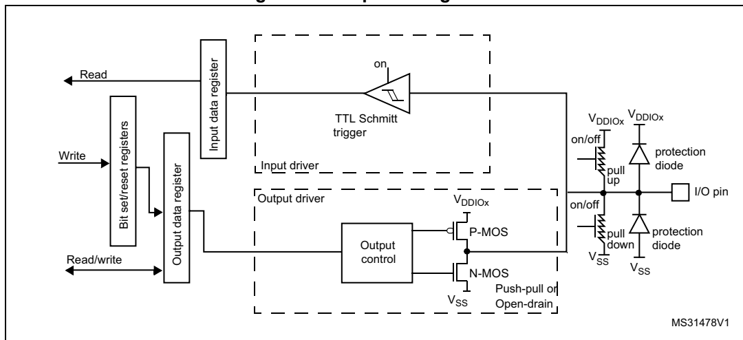
Figure 24. Output configuration
