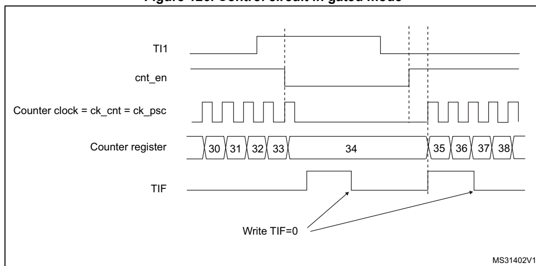
Figure 126. Control circuit in gated mode
