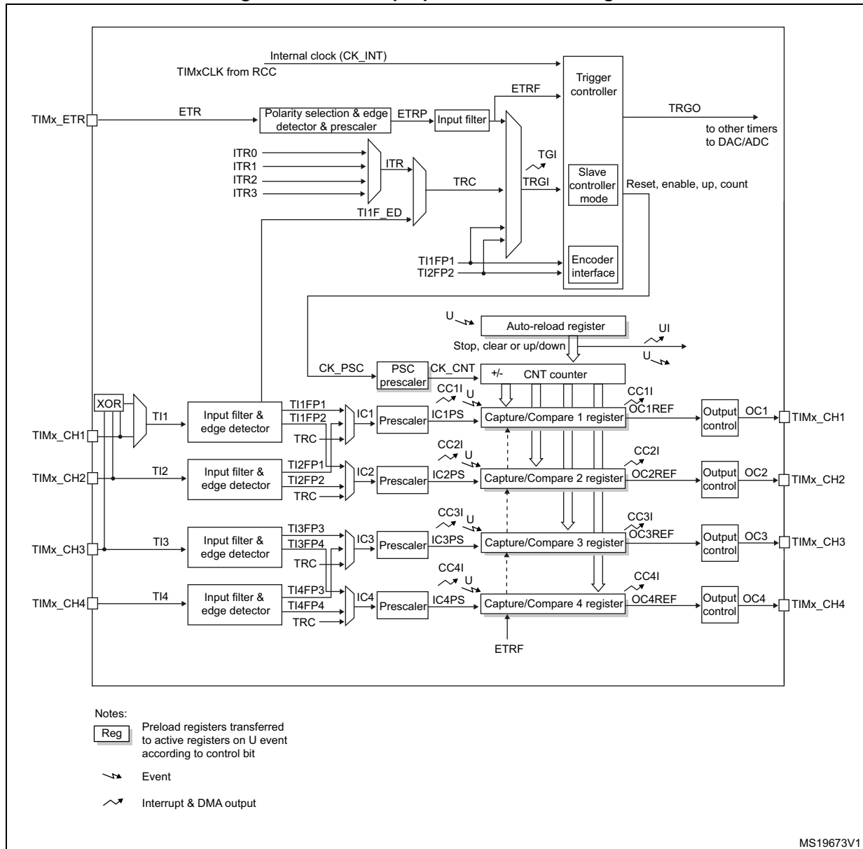
Figure 89. General-purpose timer block diagram
