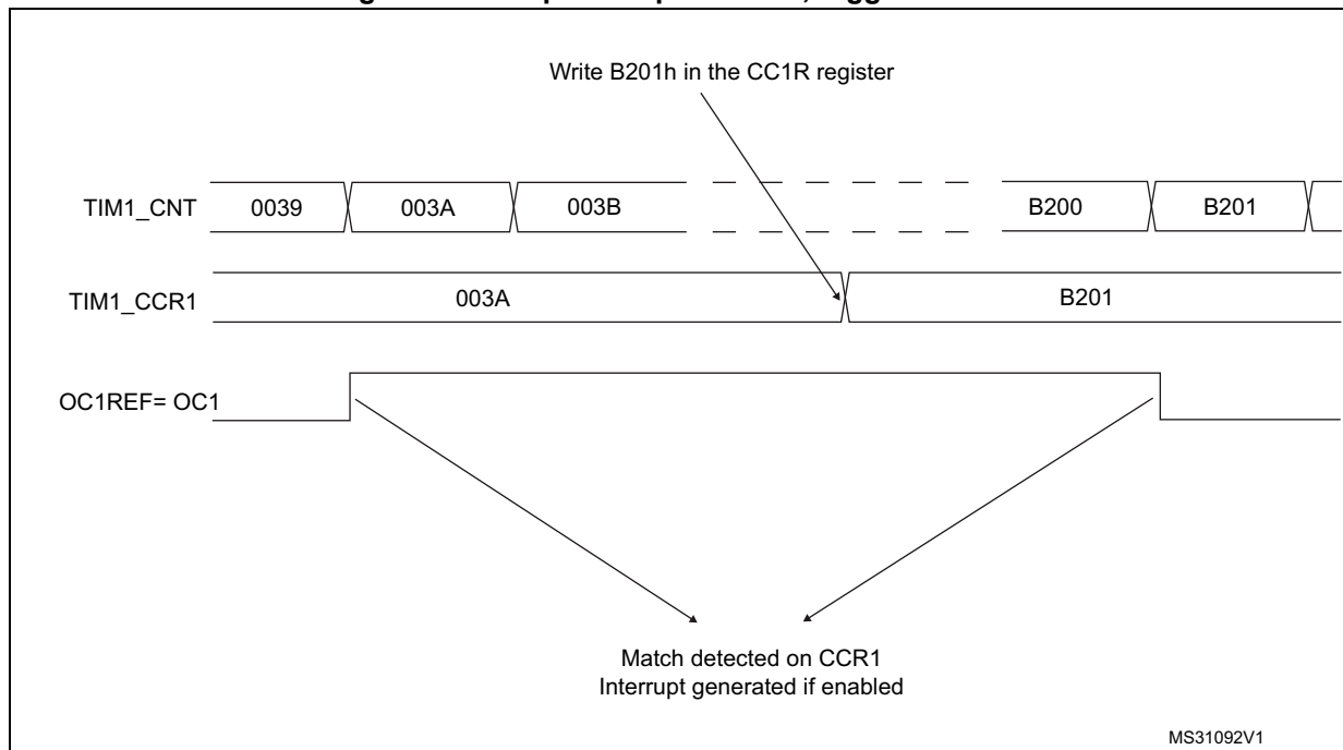
Figure 118. Output compare mode, toggle on OC1.
