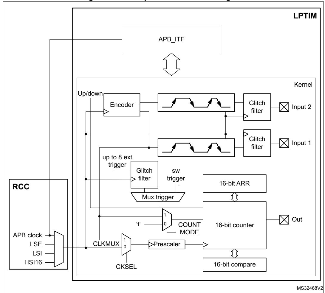
Figure 183. Low-power timer block diagram
