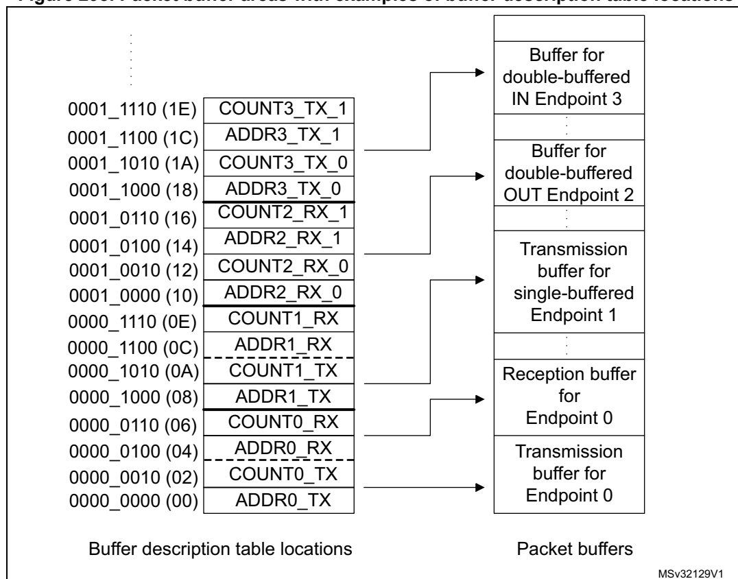
Figure 298. Packet buffer areas with examples of buffer description table locations
