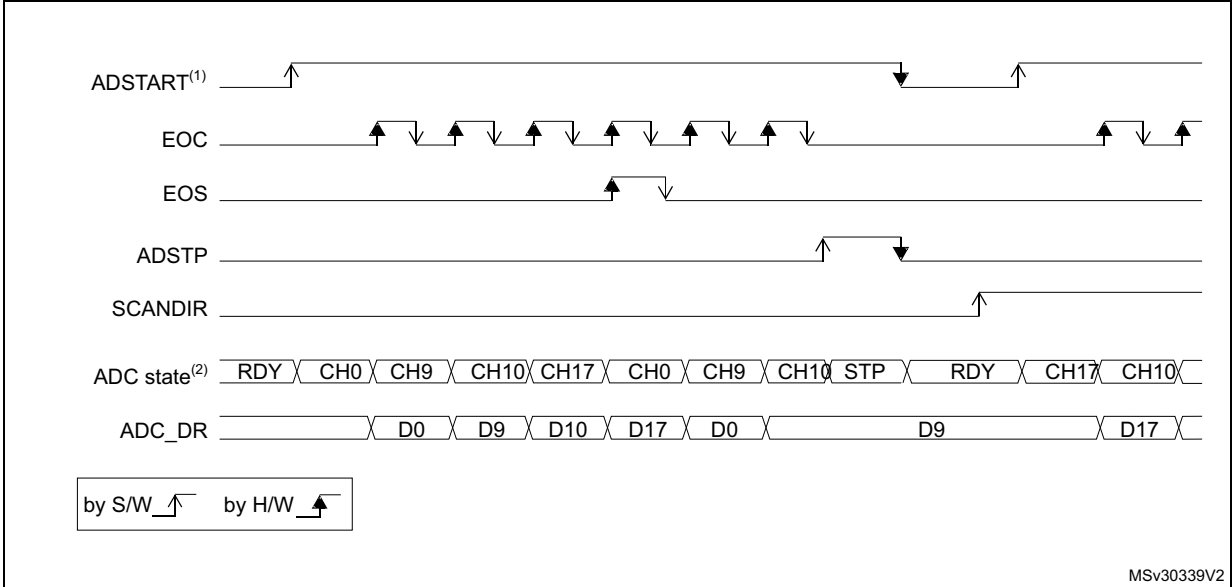
Figure 40. Continuous conversion of a sequence, software trigger
