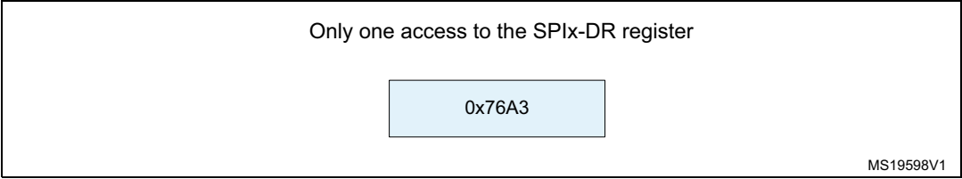
Figure 292. Example of 16-bit data frame extended to 32-bit channel frame
