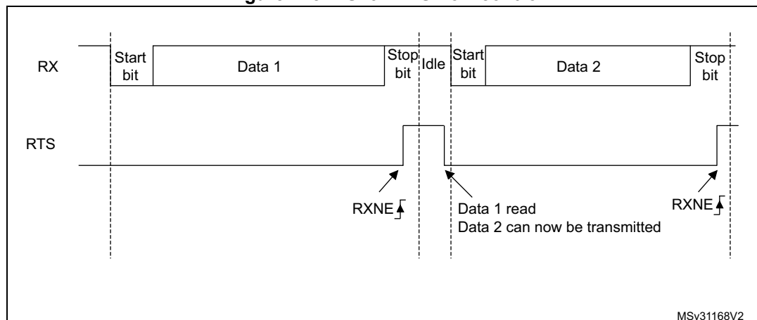
Figure 248. RS232 RTS flow control
