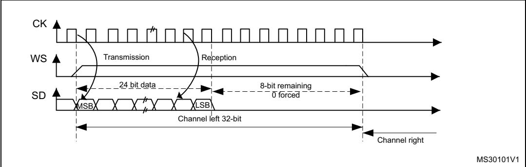
Figure 285. MSB justified 24-bit frame length with CPOL = 0
