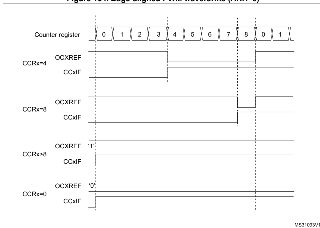
Figure 164. Edge-aligned PWM waveforms (ARR=8)
