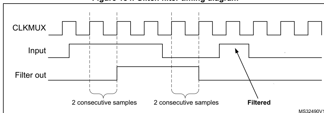
Figure 184. Glitch filter timing diagram
