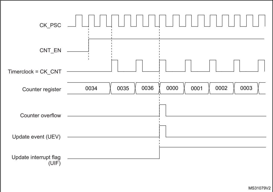
Figure 139. Counter timing diagram, internal clock divided by 2
