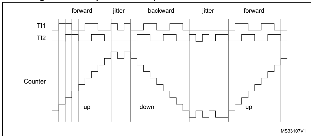
Figure 123. Example of counter operation in encoder interface mode
