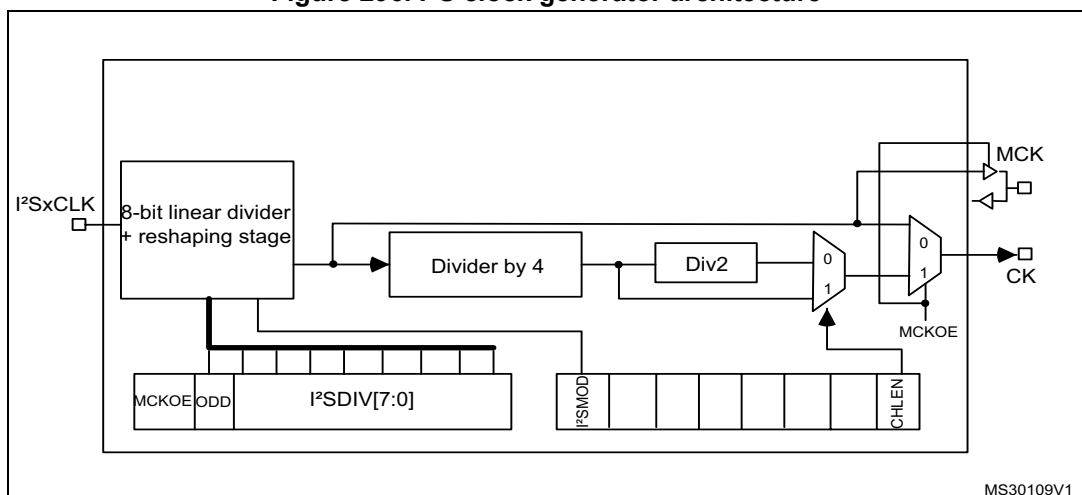
Figure 296. I 2 S clock generator architecture
