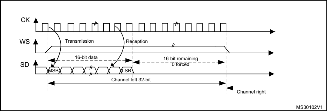
Figure 286. MSB justified 16-bit extended to 32-bit packet frame with CPOL = 0
