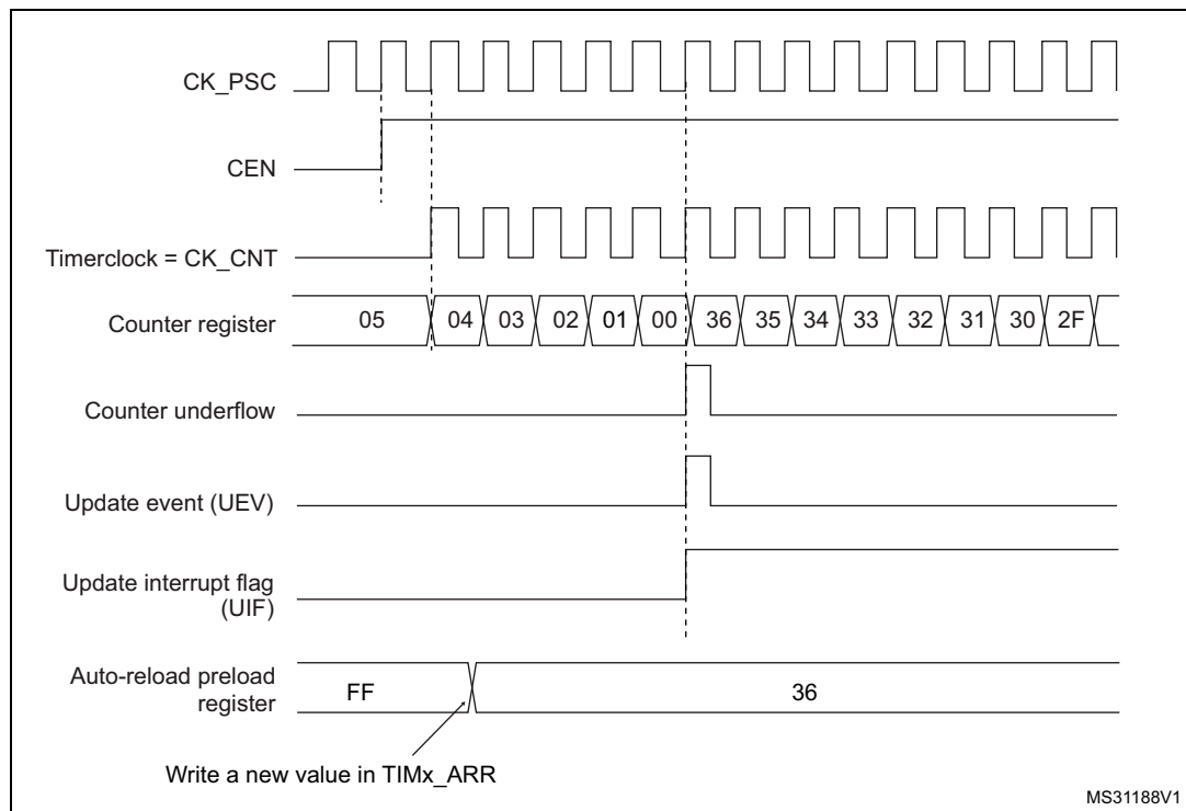
Figure 102. Counter timing diagram, Update event when repetition counter is not used
