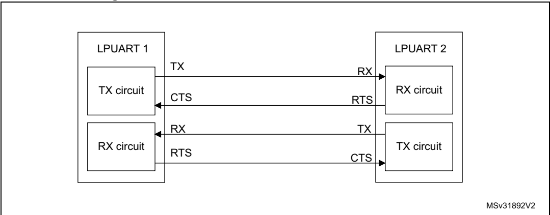
Figure 242. Hardware flow control between 2 LPUARTs
