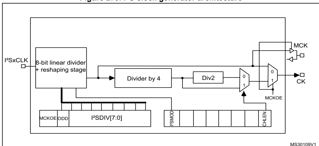
Figure 279. I 2 S clock generator architecture
