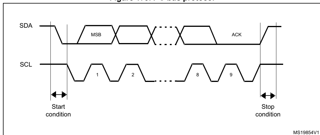
Figure 179. I 2 C bus protocol
