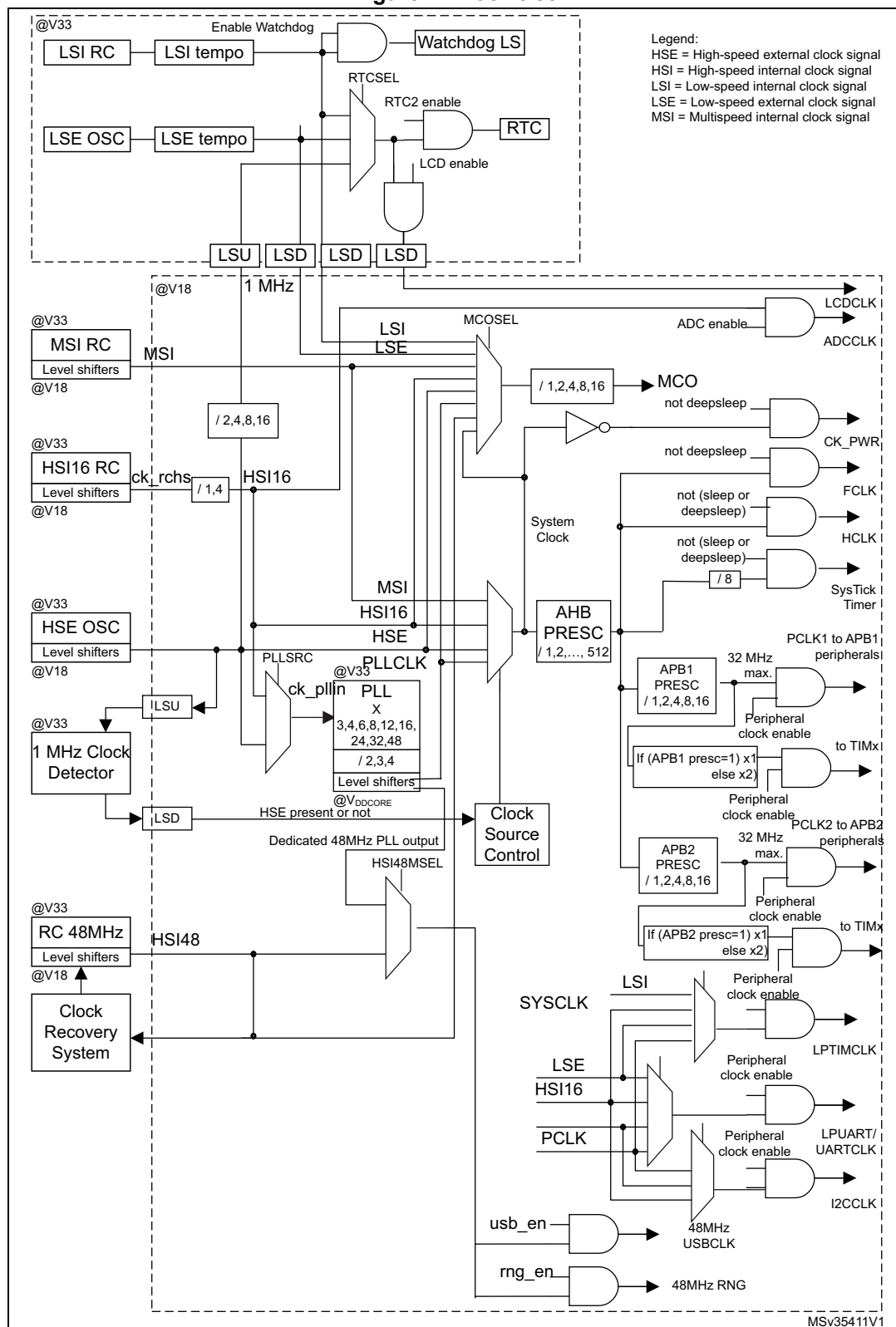
Figure 2. Clock tree
