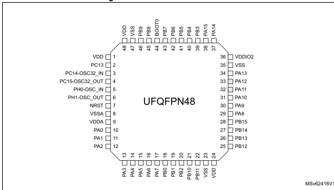
Figure 4. STM32L081xx UFQFPN48
