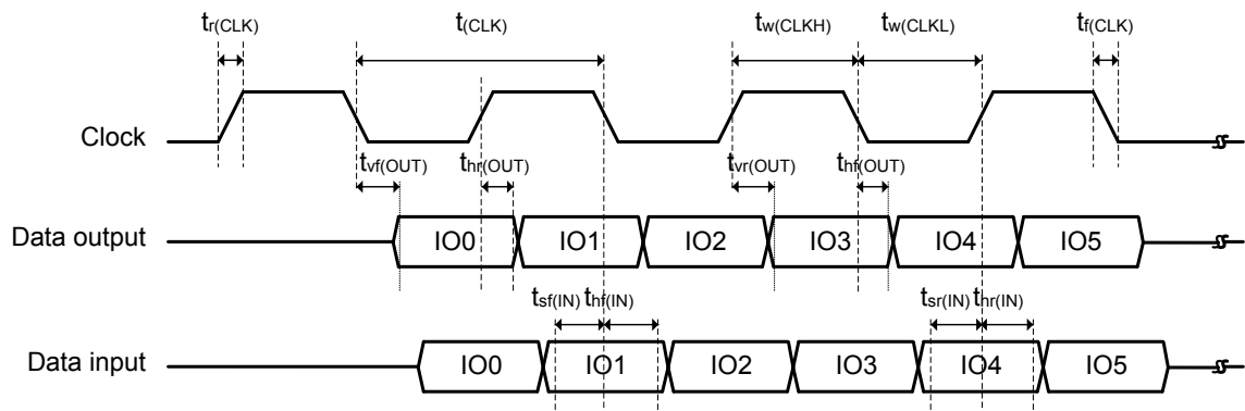
Figure 75. DDR mode
