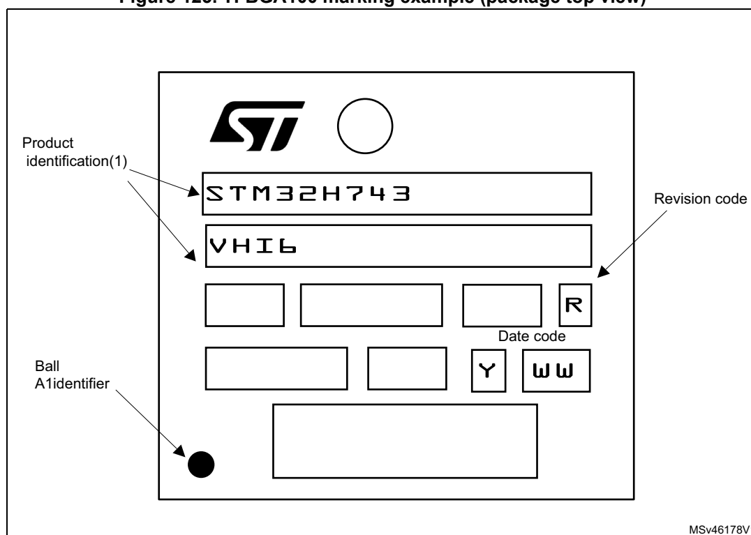
Figure 125. TFBGA100 marking example (package top view)
