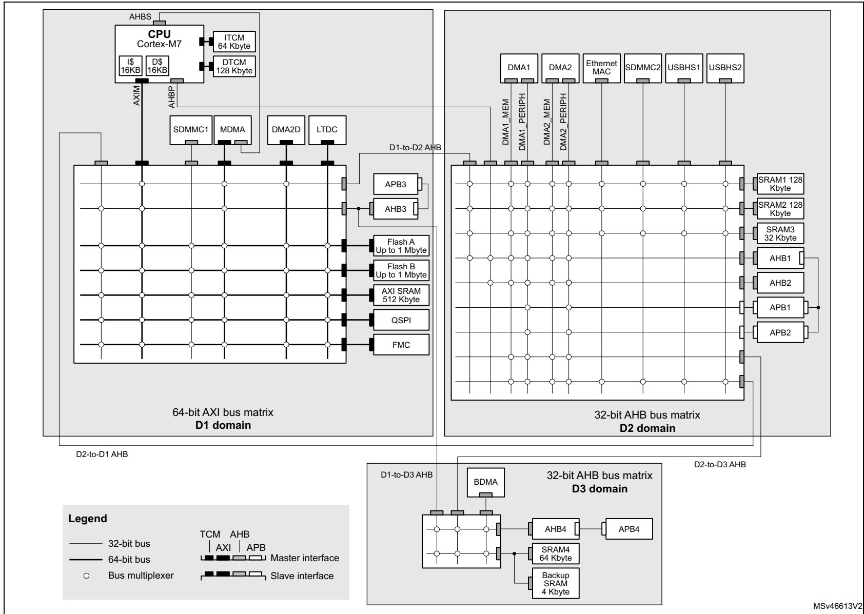
Figure 4. STM32H743xI/G bus matrix
