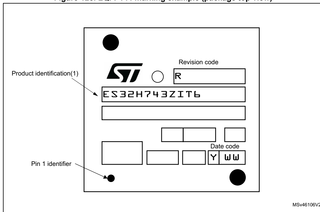
Figure 128. LQFP144 marking example (package top view)
