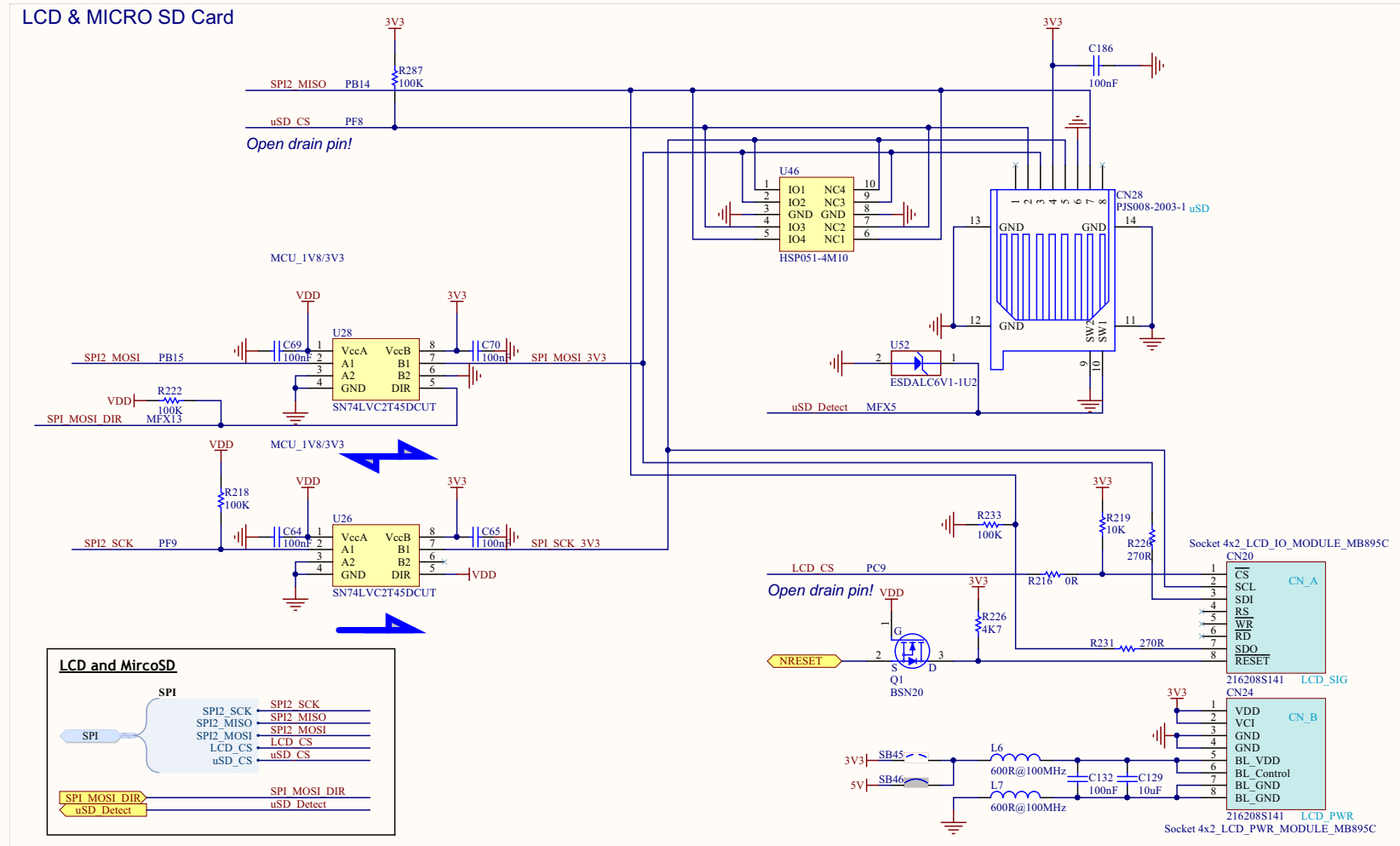
Figure 33. LCD and SD card
