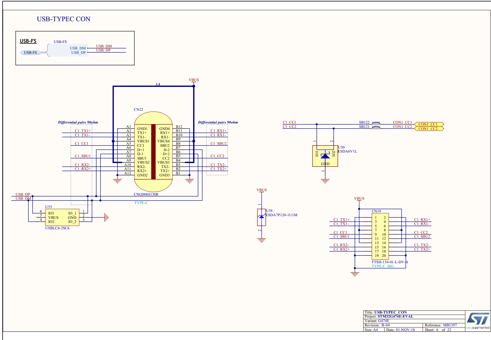
Figure 29. USB-TYPEC_CON
