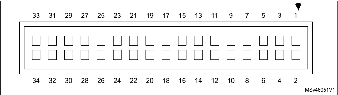
Figure 10. Motor control connector CN2 and CN4 (top view)
