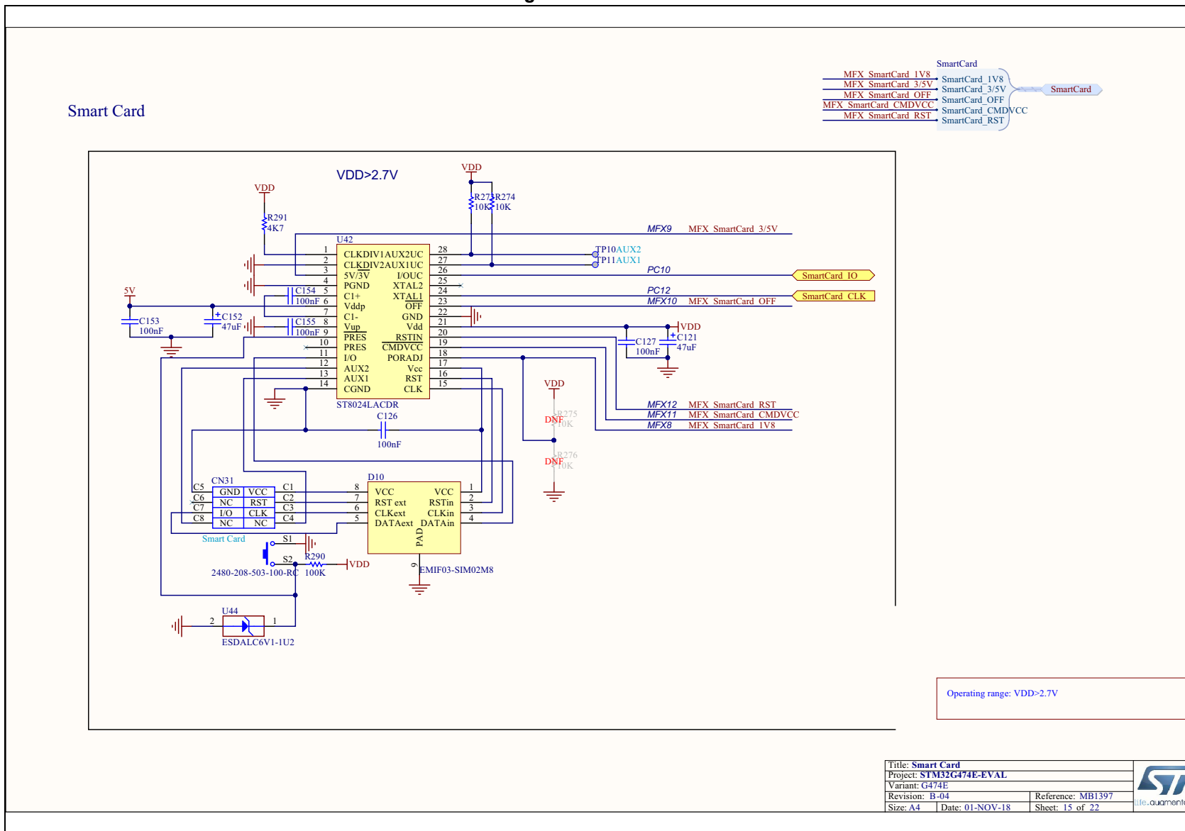
Figure 38. Smartcard
