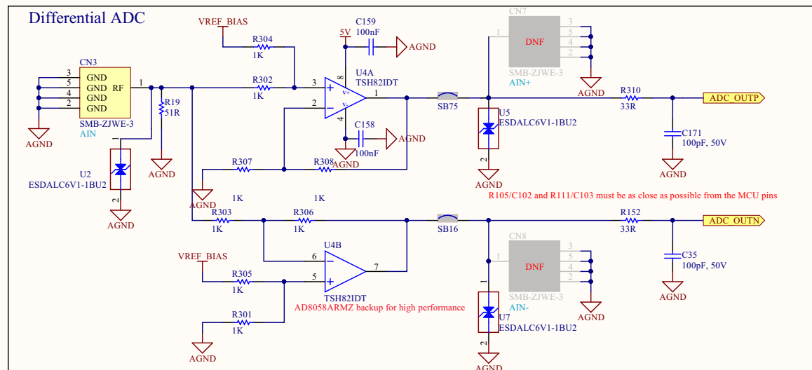
Figure 36. Analog interfaces
