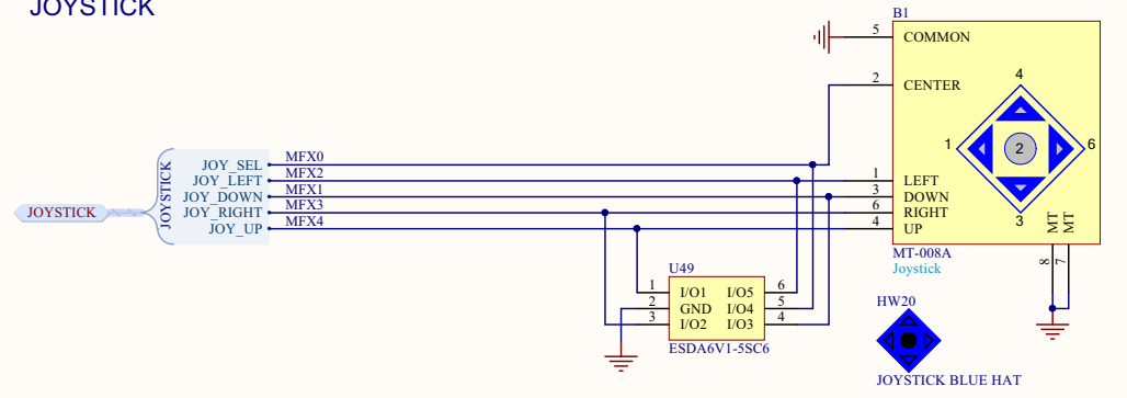
Figure 37. Peripherals
