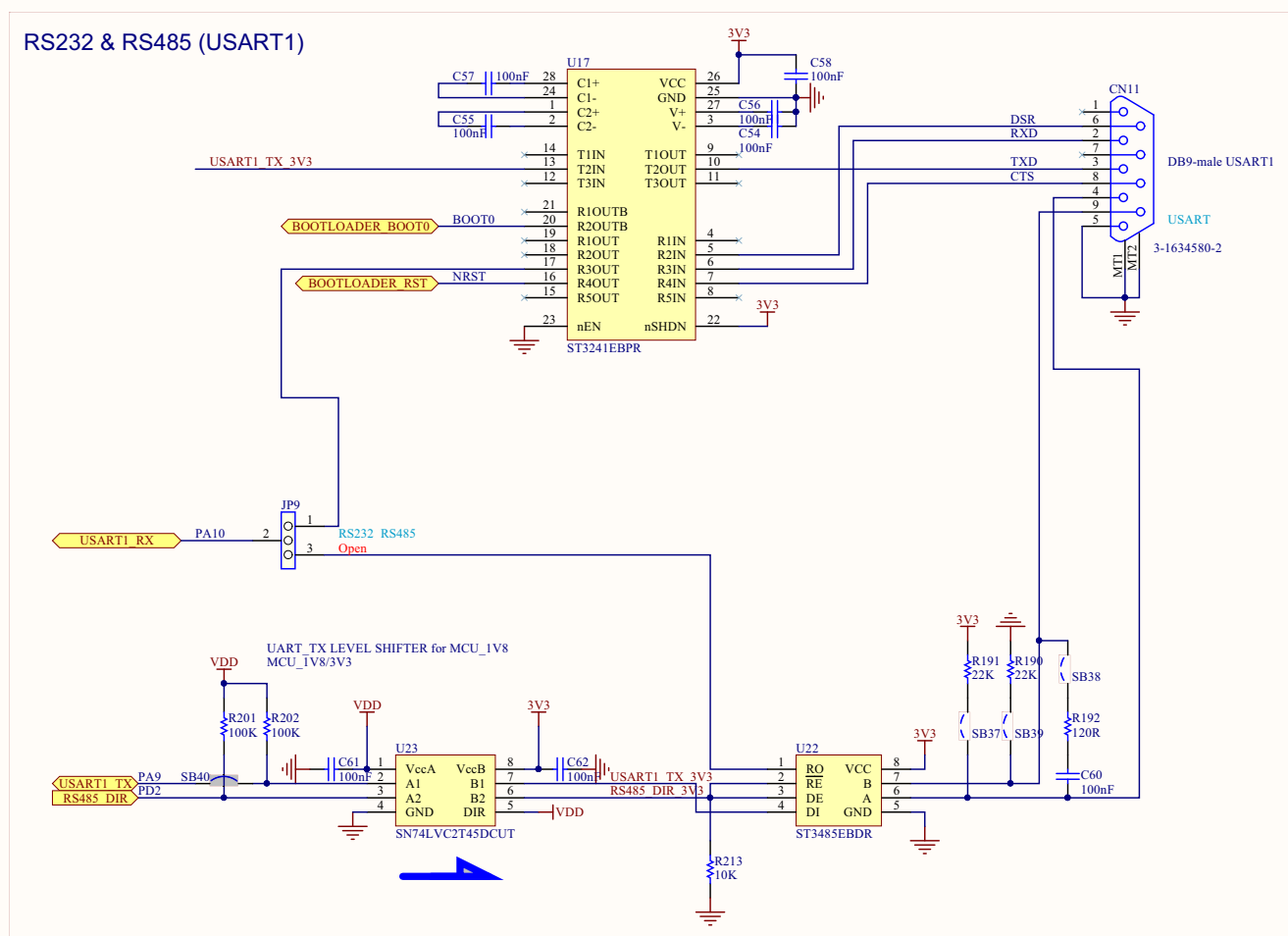
Figure 34. RS232 and RS485
