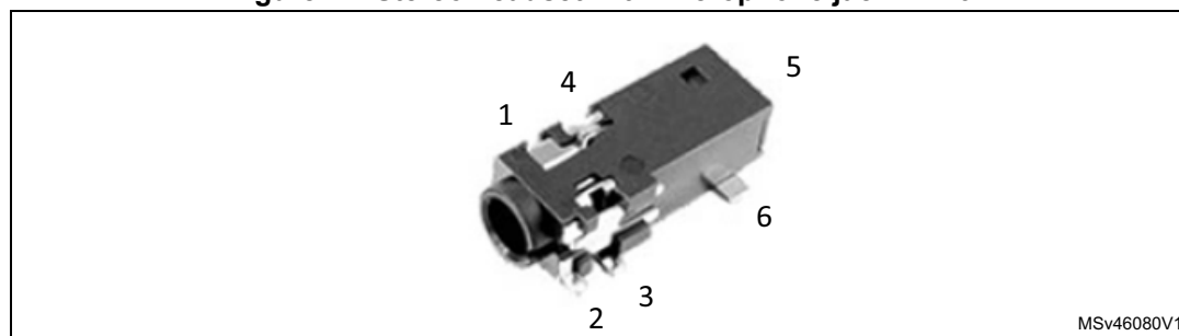
Figure 21. Stereo headset with microphone jack CN26
