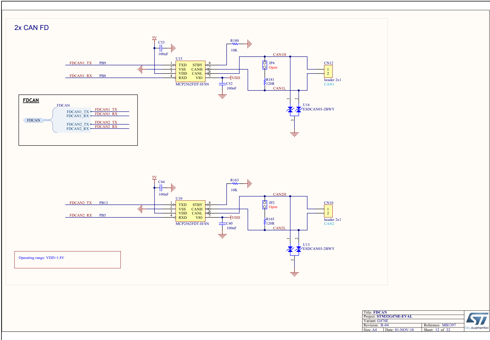
Figure 35. FDCAN
