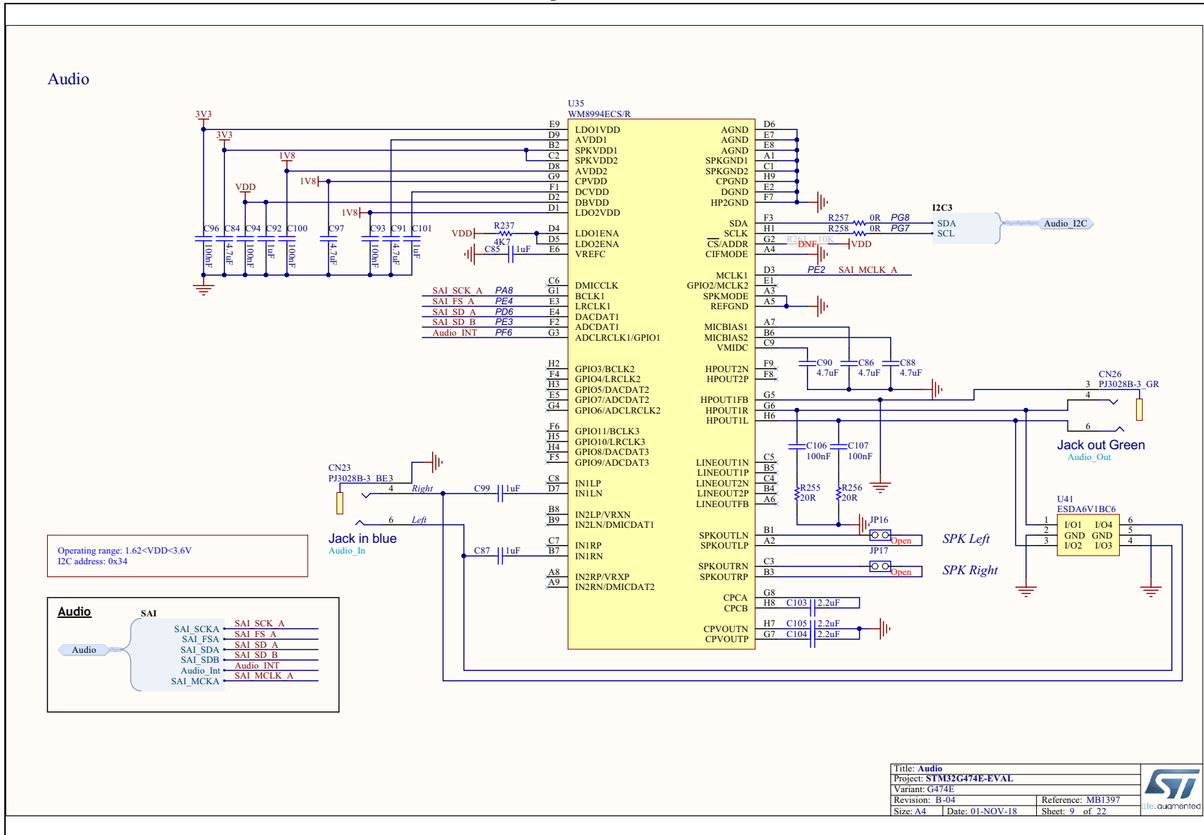
Figure 32. Audio
