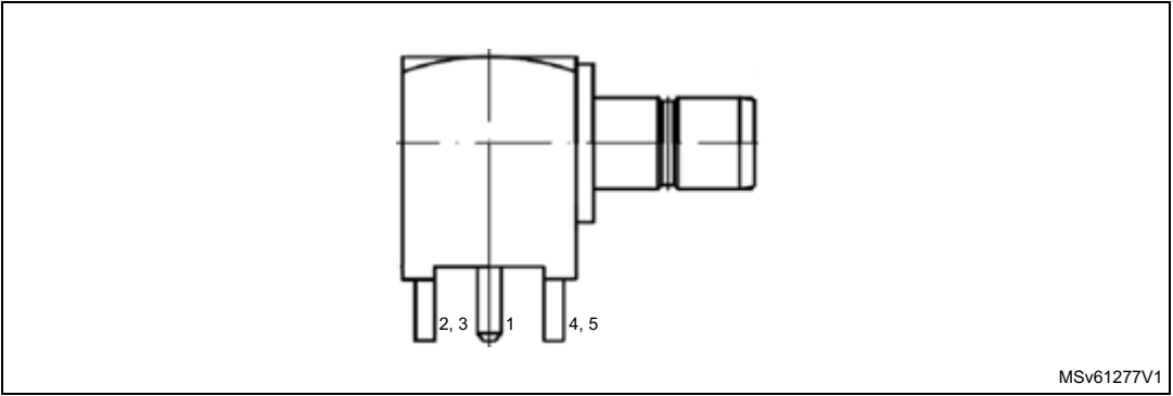
Figure 11. SMB connector (front view)
