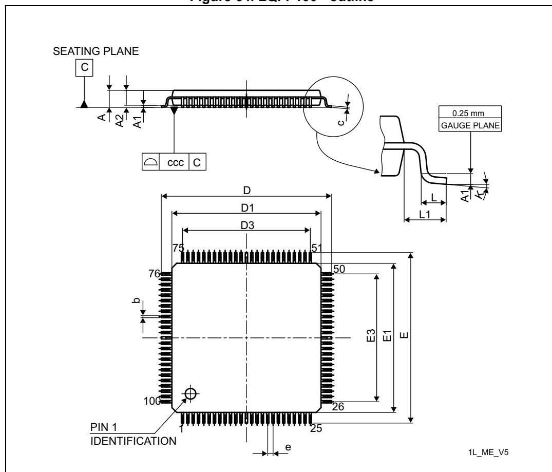
Figure 64. LQFP100 - outline
