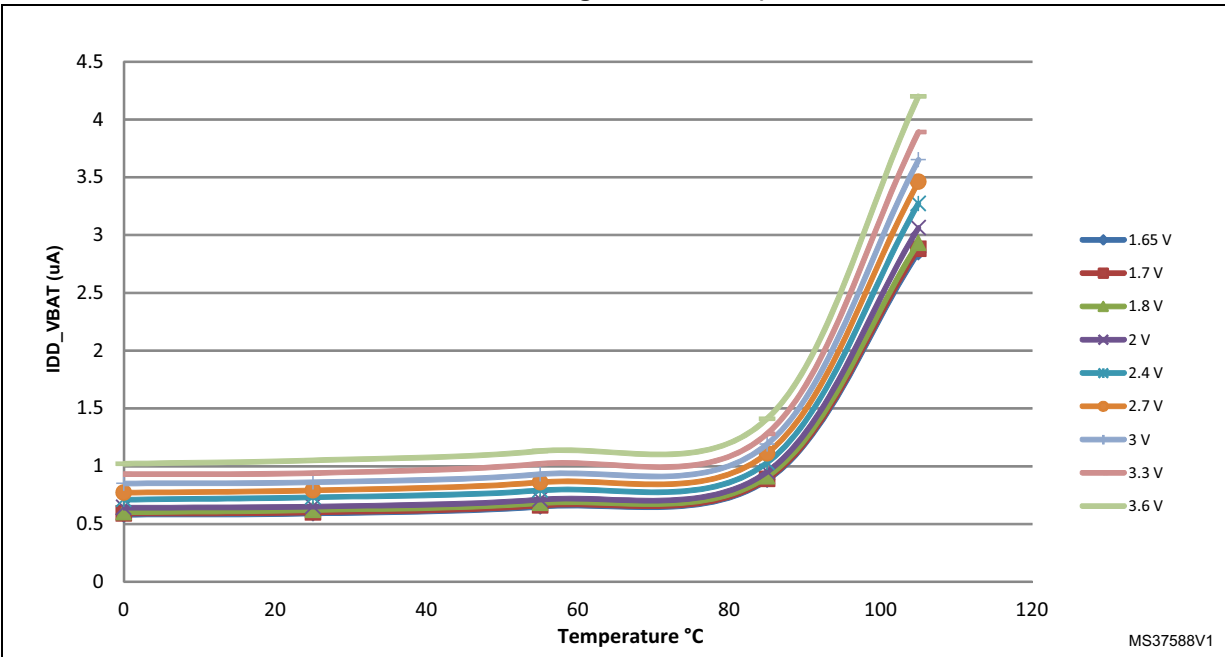
Figure 22. Typical V_{BAT} current consumption (RTC ON/BKP SRAM OFF and LSE in high drive mode)
