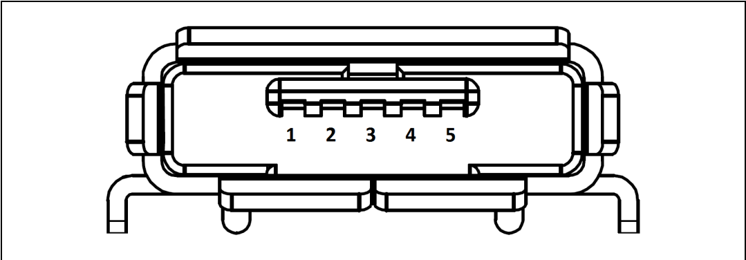
Figure 15. USB OTG Micro-AB connector CN12 (front view)
