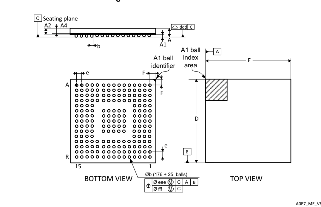
Figure 95. UFBGA176 outline
