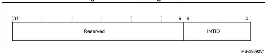
Figure 23. STIR bit assignments
