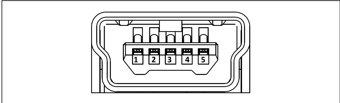
Figure 11. USB Mini-B connector CN1 (front view)
