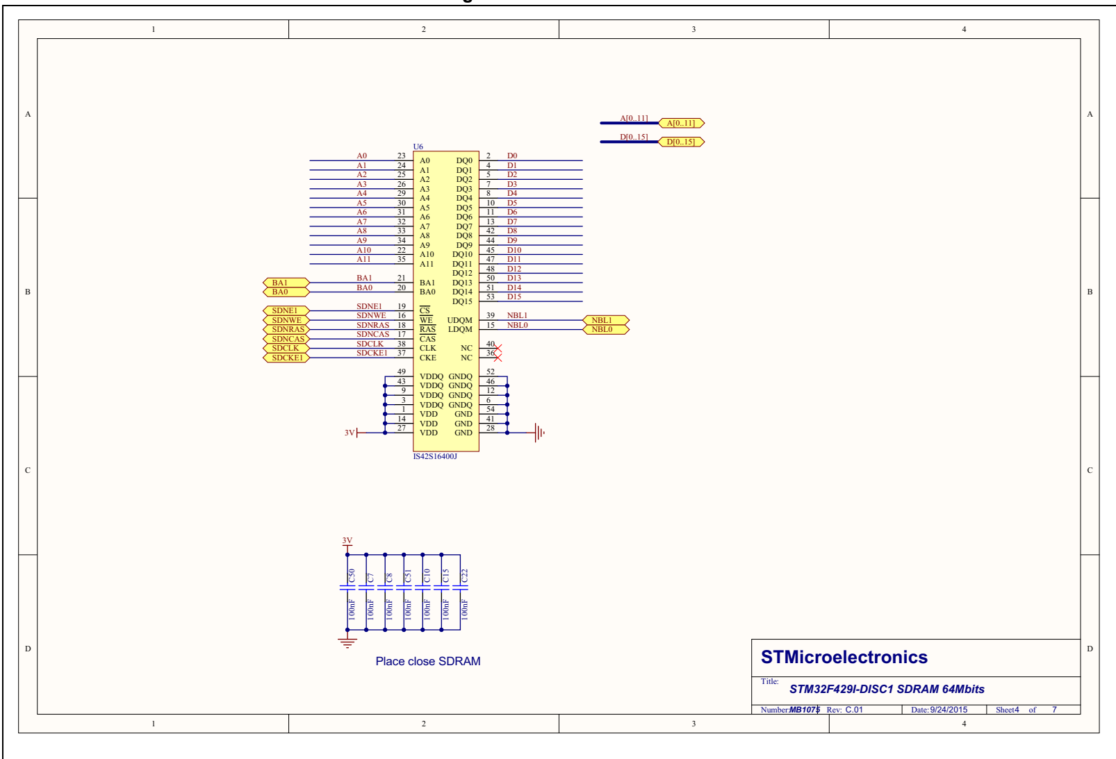
Figure 12. 64-Mbit SDRAM
