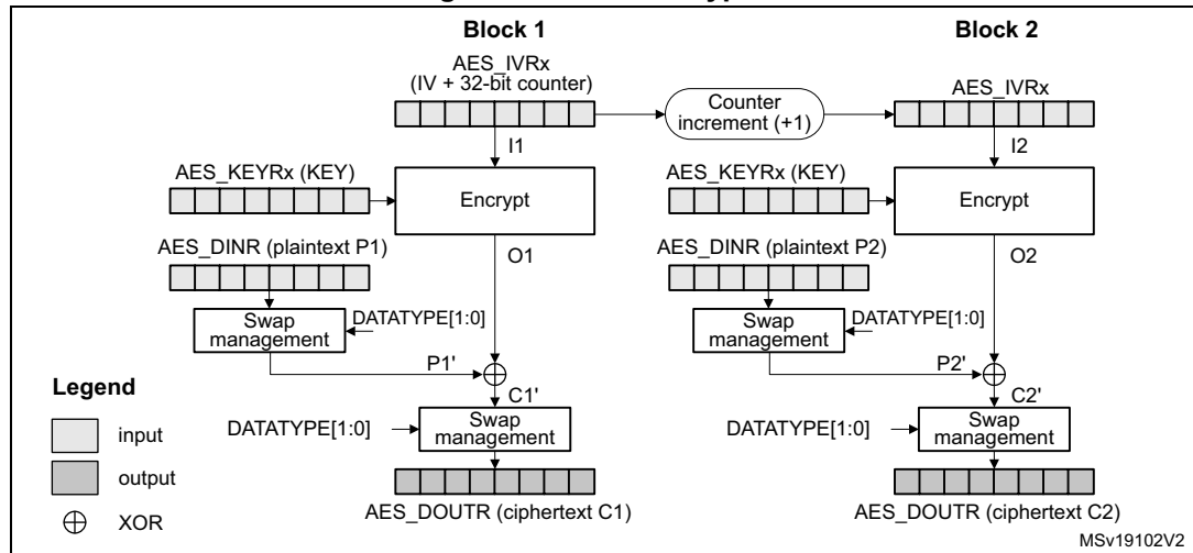
Figure 242. CTR encryption
