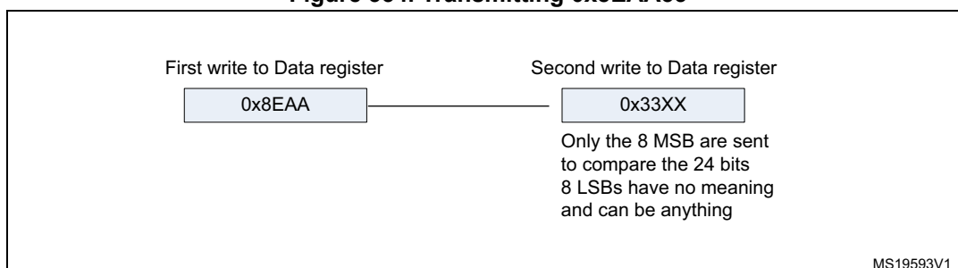
Figure 334. Transmitting 0x8EAA33
