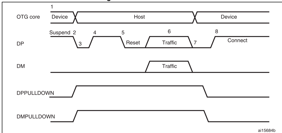
Figure 419. B-device HNP
