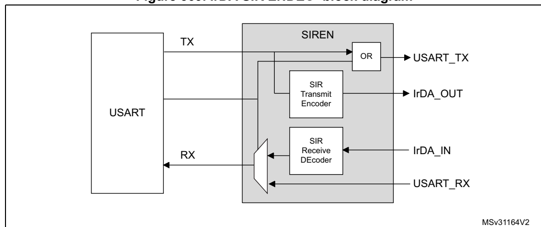
Figure 309. IrDA SIR ENDEC- block diagram
