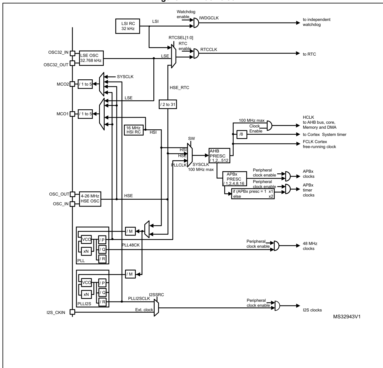
Figure 12. Clock tree
