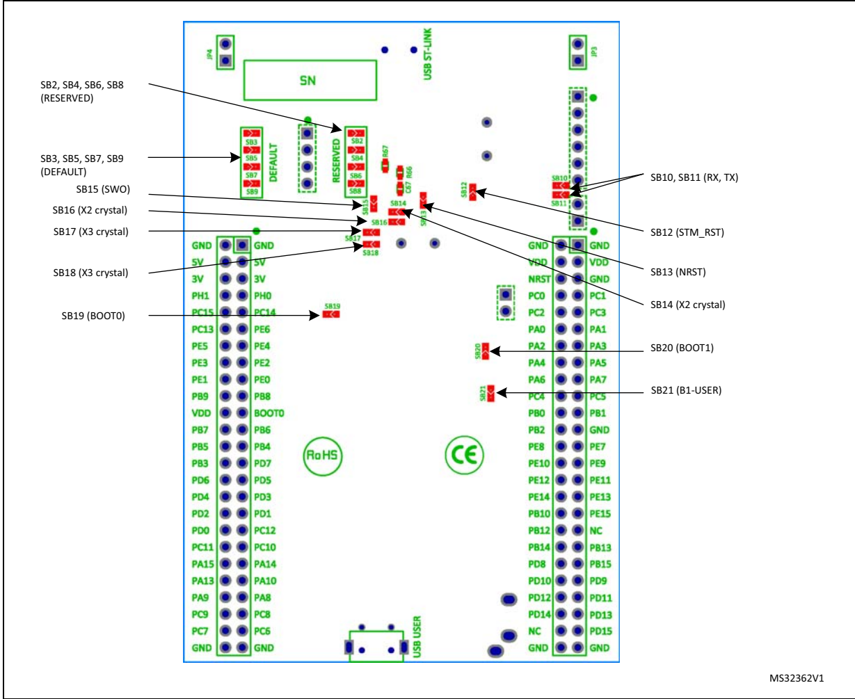
Figure 4. Bottom layout
