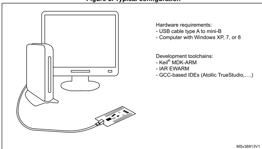
Figure 5. Typical configuration
